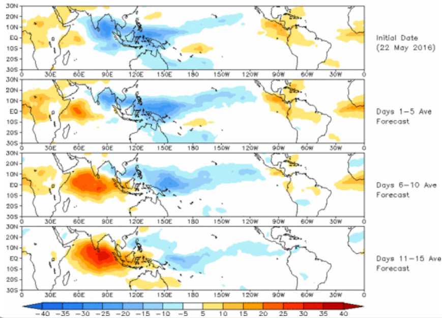
OLR prediction of MJO-related anomalies using CA model reconstruction by RMM1 & RMM2 (22 May 2016)
