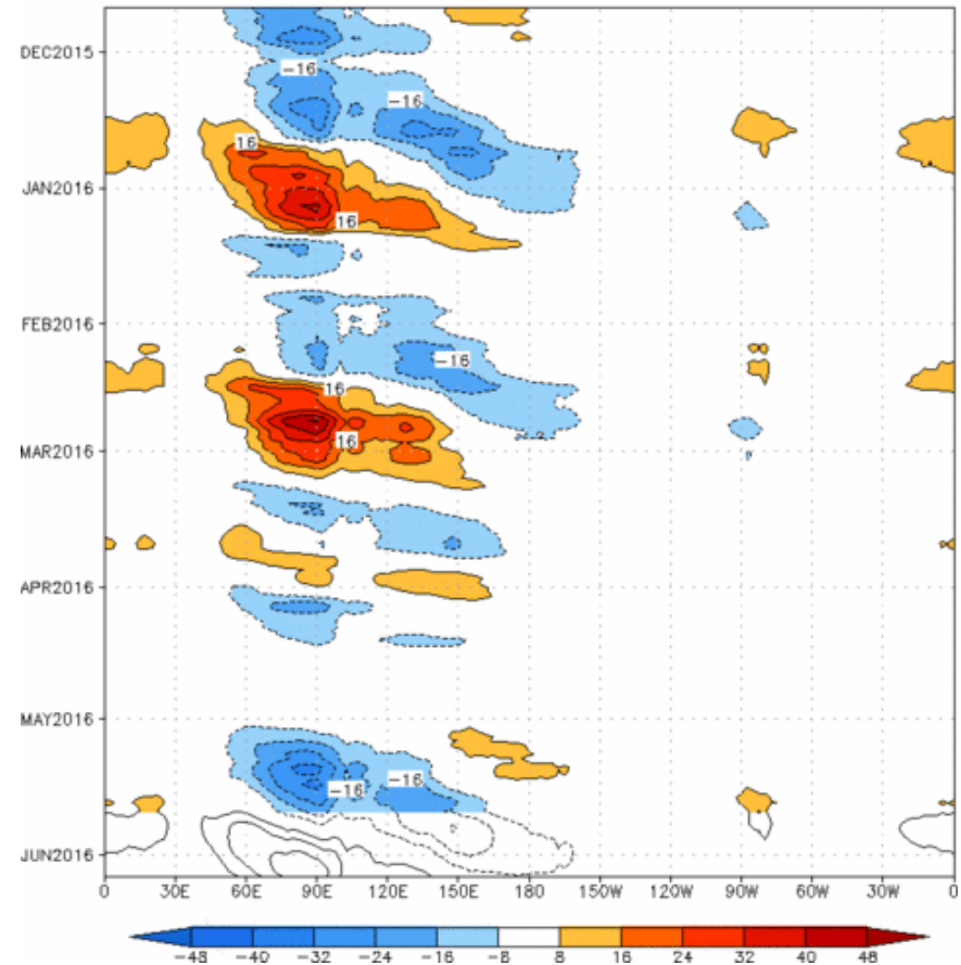
Reconstructed anomaly field associated with the MJO using RMM1 & RMM2 OLR [ 7.5^{\circ} S, 7.5^{\circ} N] (cont:4Wm -2 ) Period:21-Nov-2015 to 22-May-2016 The unfilled contours are CA forecast reconstructed anomaly for 15 days
