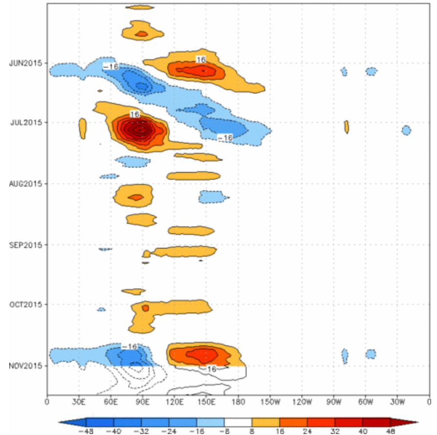
Reconstructed anomaly field associated with the MJO using RMM1 & RMM2 OLR [7.5°S,7.5°N] (cont:4Wm -2 ) Period:02-May-2015 to 01-Nov-2015 The unfilled contours are GEFS forecast reconstructed anomaly for 15 days
