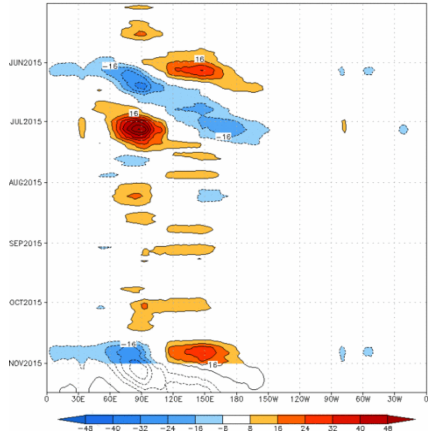
Reconstructed anomaly field associated with the MJO using RMM1 & RMM2 OLR [7.5°S,7.5°N] (cont:4Wm -2 ) Period:02-May-2015 to 01-Nov-2015 The unfilled contours are CA forecast reconstructed anomaly for 15 days
