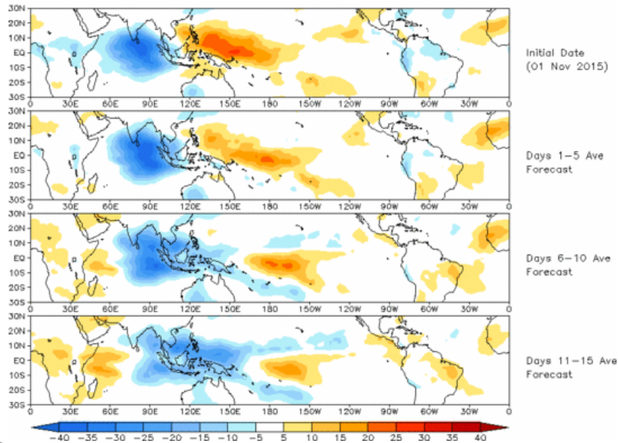
OLR prediction of MJO-related anomalies using CA model reconstruction by RMM1 & RMM2 (01 Nov 2015)
