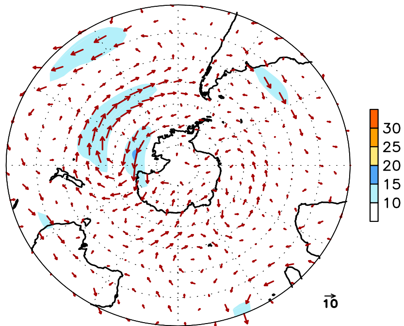
FIGURE E16. Southern Hemisphere mean (left) and anomalous (right) 300-hPa vector wind (CDAS/Reanalysis) for SEP 2020. Mean (anomaly) isotach contour interval is 10 (5) \text{ms}^{-1} . Values greater than 30 \text{ms}^{-1} (left) and 10 \text{ms}^{-1} (rights) are shaded. Anomalies are departures from the 1981-2010 base period monthly means.
