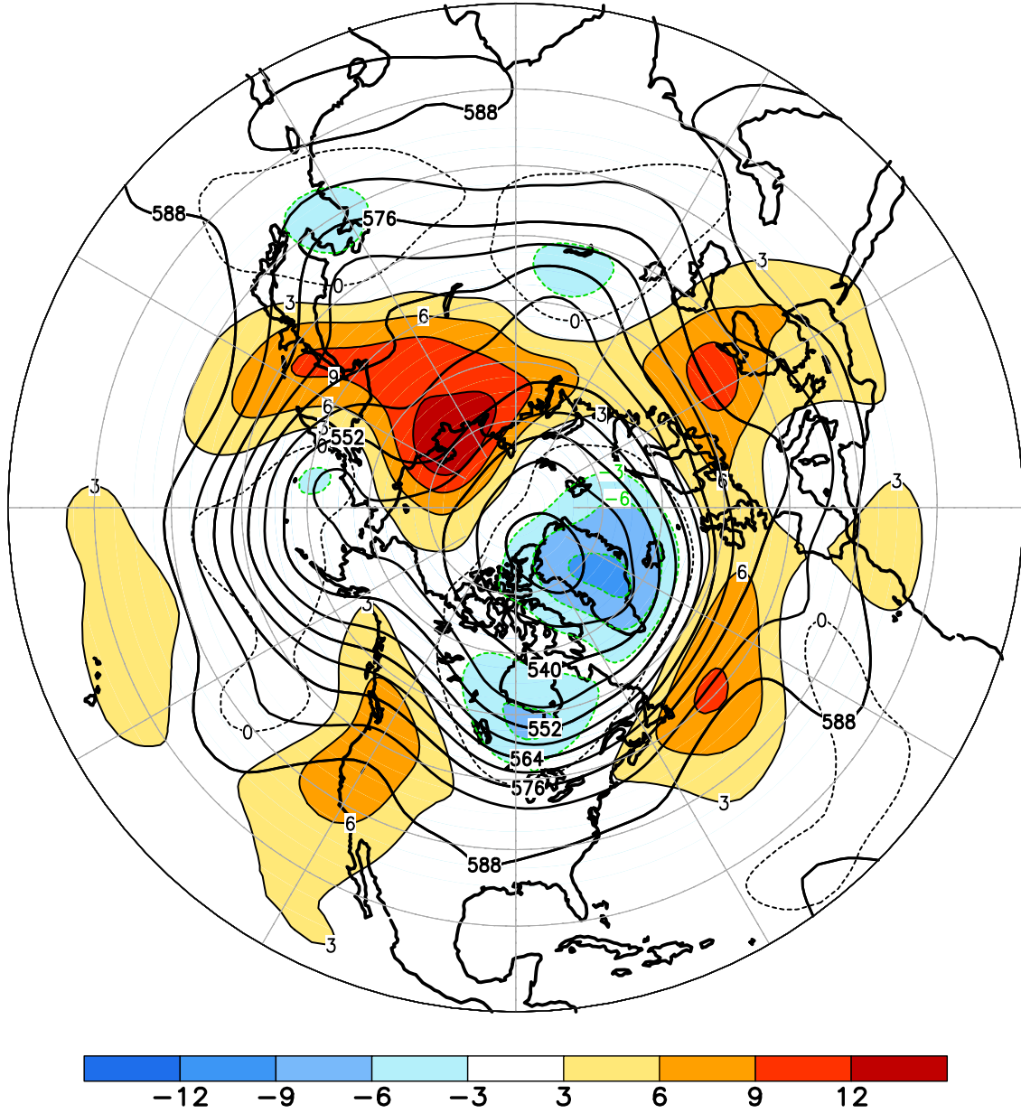
FIGURE E9. Northern Hemisphere mean and anomalous 500-hPa geopotential height (CDAS/Reanalysis) for SEP 2020. Mean heights are denoted by solid contours drawn at an interval of 6 dam. Anomaly contour interval is 3 dam with values less (greater) than -3 dam (3 dam) indicated by dark (light) shading. Anomalies are calculated as departures from the 1981-2010 base period monthly means.
