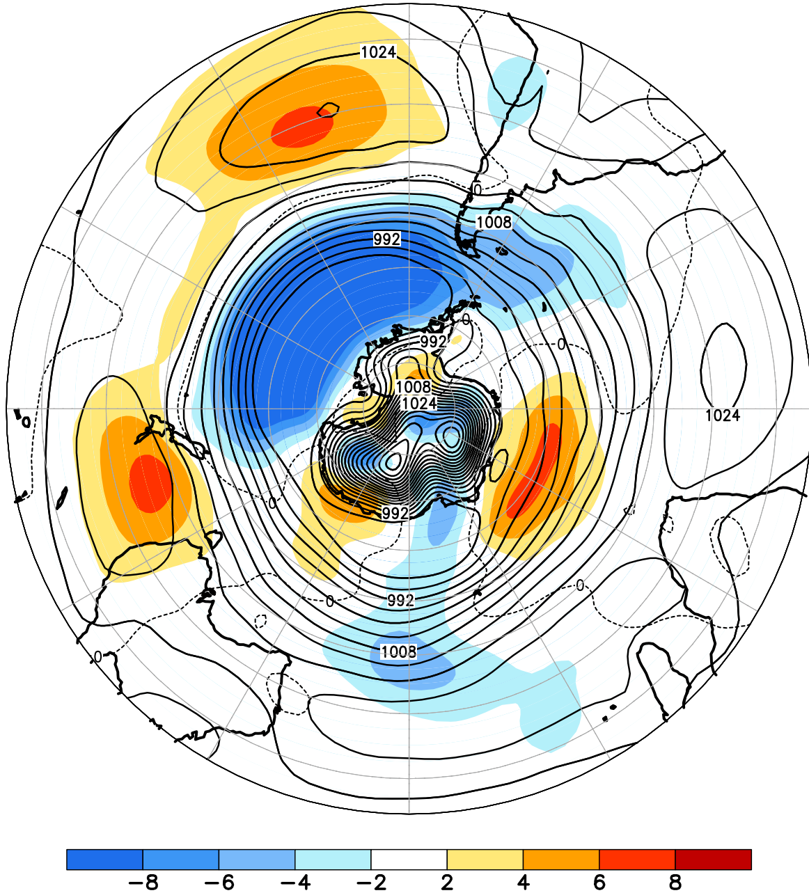
FIGURE E14. Southern Hemisphere mean and anomalous sea level pressure(CDAS/Reanalysis) for SEP 2020. Mean values are denoted by solid contours drawn at an interval of 4 hPa. Anomaly contour interval is 2 hPa with values less (greater) than -2 hPa (2 hPa) indicated by dark (light) shading. Anomalies are calculated as departures from the 1981-2010 base period monthly means.
