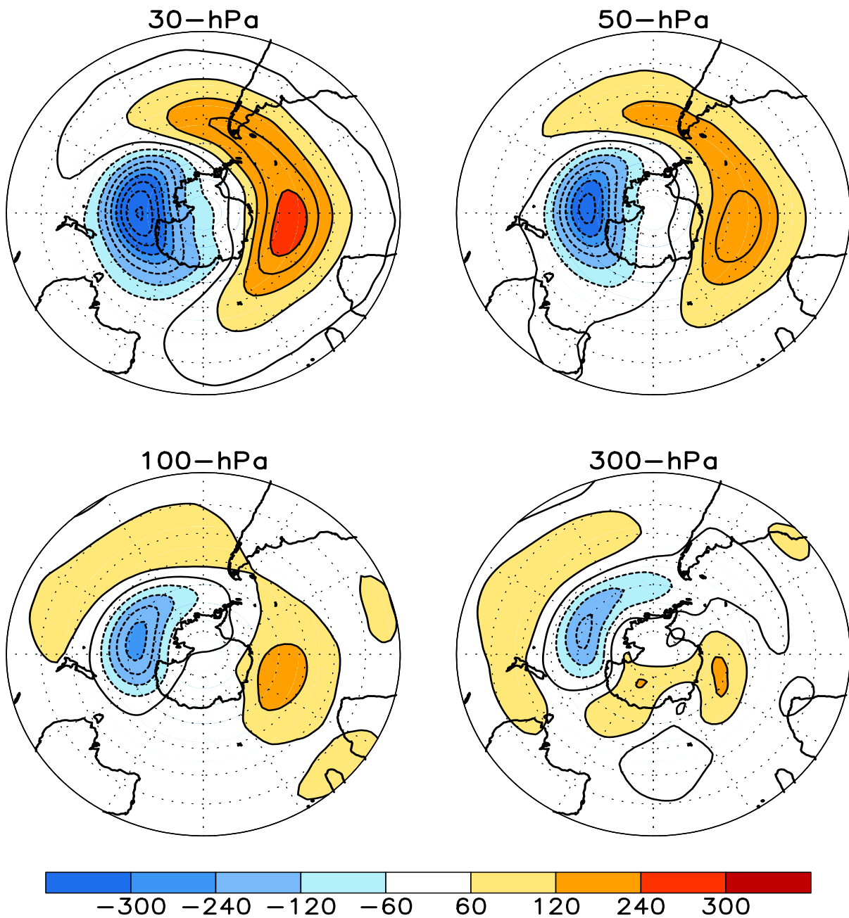
FIGURE S1. Stratospheric height anomalies (m) at selected levels for SEP 2020. Positive values are indicated by solid contours and dark shading. Negative values are indicated by dashed contours and light shading. Contour interval is 60 m. Anomalies are calculated from the 1981-2010 base period means. Winter Hemisphere is shown.
