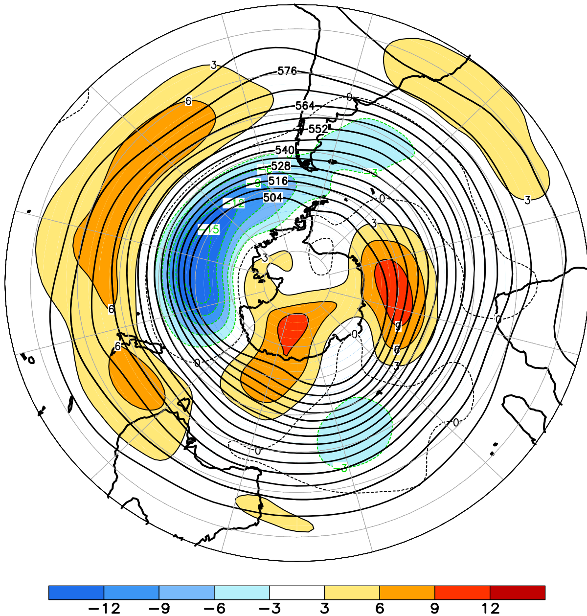
FIGURE E15. Southern Hemisphere mean and anomalous 500-hPa geopotential height (CDAS/Reanalysis) for SEP 2020. Mean heights are denoted by solid contours drawn at an interval of 6 dam. Anomaly contour interval is 3 dam with values less (greater) than -3 dam (3 dam) indicated by dark (light) shading. Anomalies are calculated as departures from the 1981-2010 base period monthly means.
