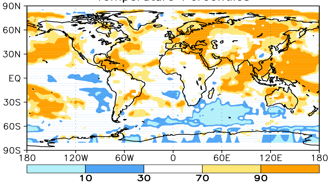
FIGURE E1. Surface temperature anomalies ( ^{\circ}\text{C} , top) and surface temperature expressed as percentiles of the normal (Gaussian) distribution fit to the 1981–2010 base period data (bottom) for SEP 2020. Analysis is based on station data over land and on SST data over the oceans (top). Anomalies for station data are departures from the 1981–2010 base period means, while SST anomalies are departures from the 1981–2010 adjusted OI climatology. (Smith and Reynolds 1998, J. Climate , 11 , 3320-3323). Regions with insufficient data for analysis in both figures are indicated by shading in the top figure only.
