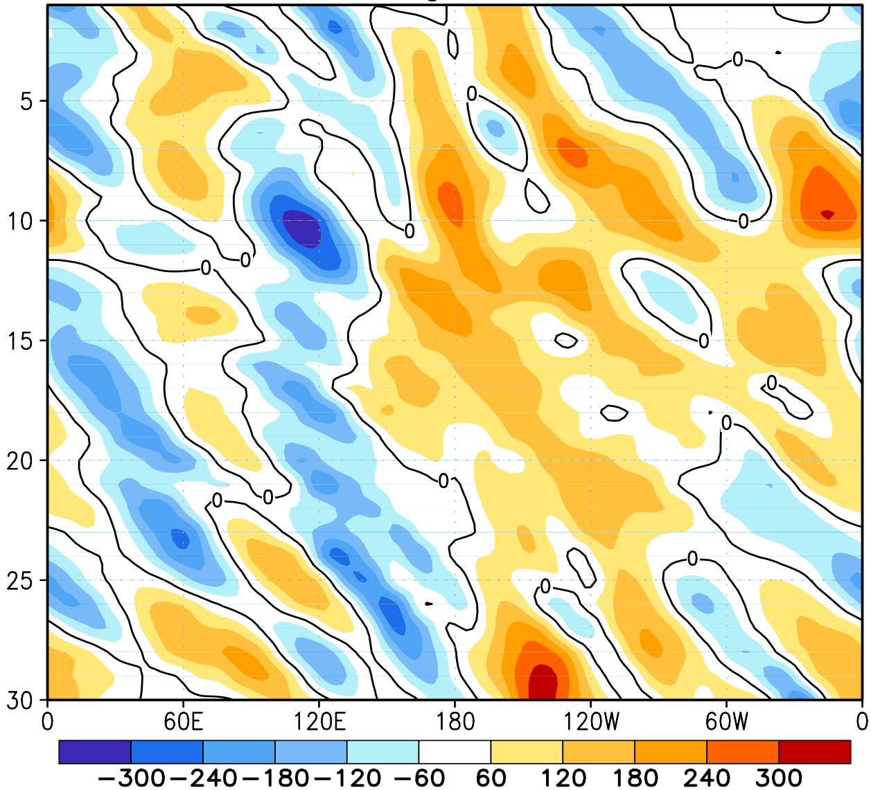
FIGURE E18. Southern Hemisphere: Daily 500-hPa height anomalies for SEP 2009 averaged over the 5° latitude band centered on 40°S. Positive values are indicated by solid contours and dark shading. Negative values are indicated by dashed contours and light shading. Contour interval is 60 m. Anomalies are departures from the 1979-95 base period daily means.
