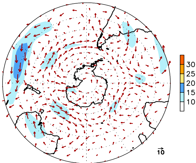
FIGURE E16. Southern Hemisphere mean (left) and anomalous (right) 300-hPa vector wind (CDAS/Reanalysis) for SEP 2009. Mean (anomaly) isotach contour interval is 10 (5) \text{ms}^{-1} . Values greater than 30 \text{ms}^{-1} (left) and 10 \text{ms}^{-1} (rights) are shaded. Anomalies are departures from the 1979-95 base period monthly means.
