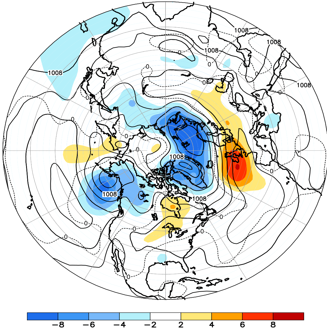
FIGURE E8. Northern Hemisphere mean and anomalous sea level pressure (CDAS/Reanalysis) for SEP 2009. Mean values are denoted by solid contours drawn at an interval of 4 hPa. Anomaly contour interval is 2 hPa with values less (greater) than -2 hPa (2 hPa) indicated by dark (light) shading. Anomalies are calculated as departures from the 1979-95 base period monthly means.
