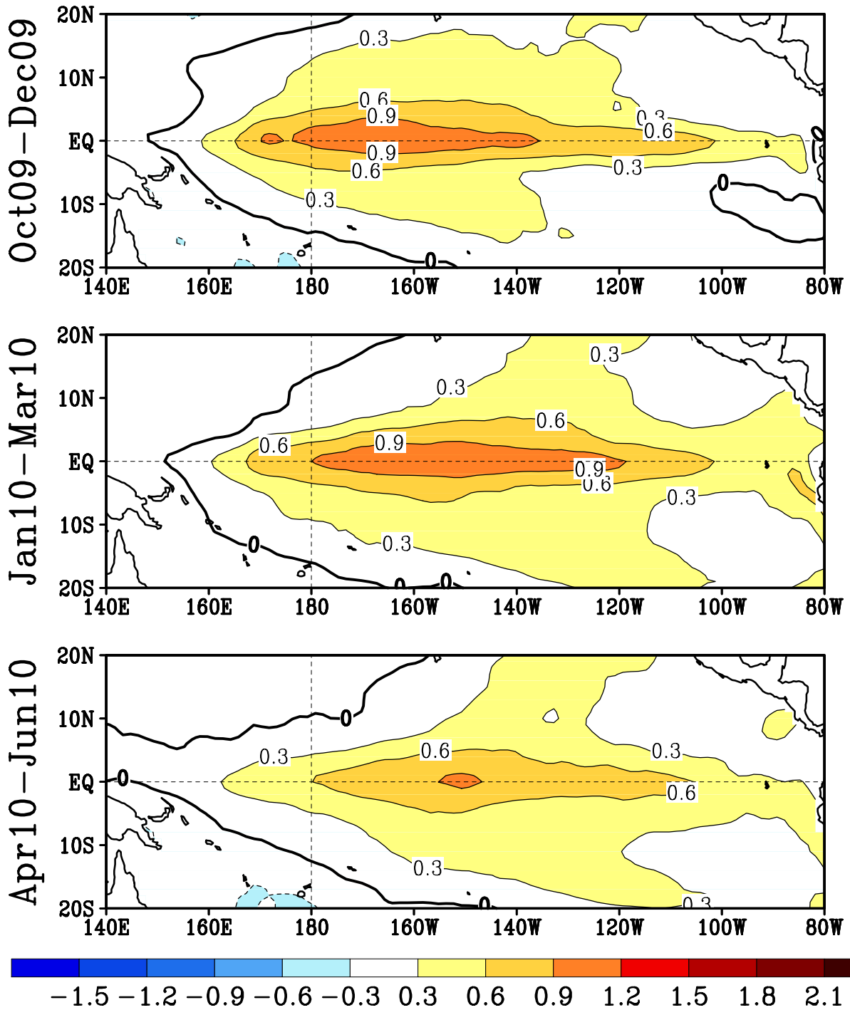
FIGURE F5. Predicted 3-month average sea surface temperature anomalies from the NCEP/CPC Markov model (Xue et al. 2000, J. Climate , 13 , 849-871). The forecast is initiated in SEP 2009. Contour interval is 0.3C and negative anomalies are indicated by dashed contours. Anomalies are calculated relative to the 1971-2000 climatology.
