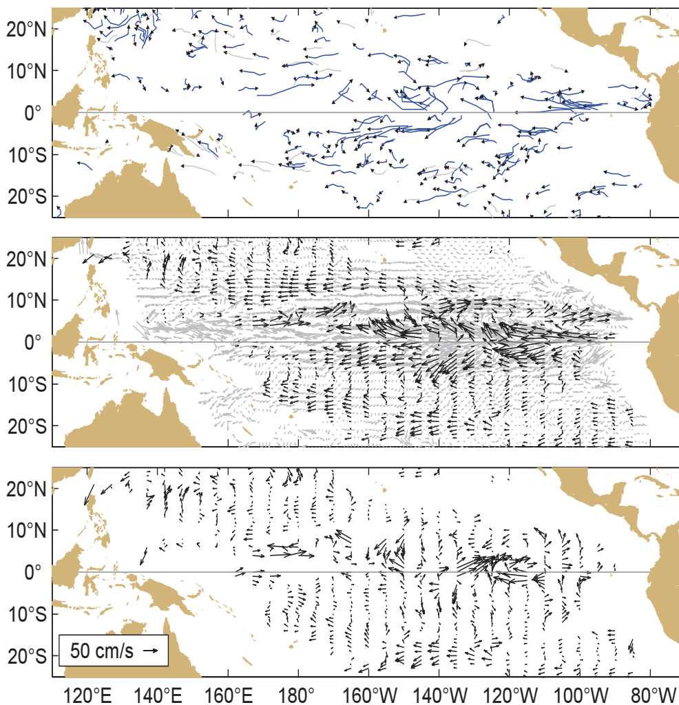
Figure A1.1 Top: Movements of drifting buoys in the tropical Pacific Ocean during September 2009. The linear segments of each trajectory represent a one week displacement. Trajectories of buoys which have lost their subsurface drogues are gray; those with drogues are black.
