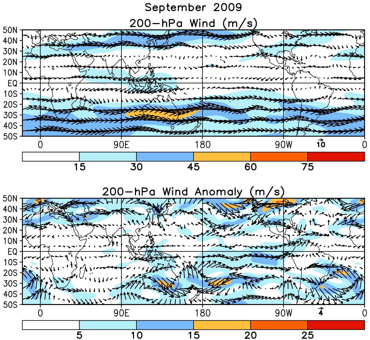
FIGURE T21. Mean (top) and anomalous (bottom) 200-hPa vector wind (CDAS/Reanalysis) for SEP 2009. Contour interval for isotachs is 15 \text{ ms}^{-1} (top) and 5 \text{ ms}^{-1} (bottom). Anomalies are departures from 1979–95 base period monthly means.
