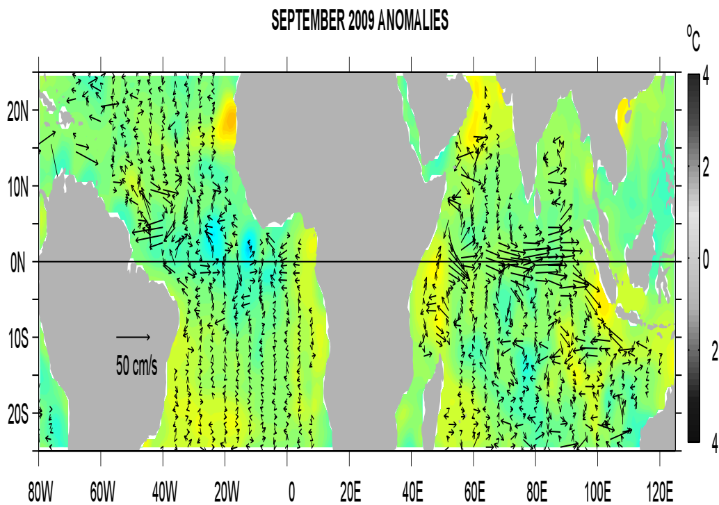
FIGURE A1.8. Ocean Surface Current Analysis-Real-time (OSCAR) for SEP 2009 (Bonjean and Lagerloef 2002, J. Phys. Oceanogr. , Vol. 32, No. 10, 2938-2954; Lagerloef et al. 1999, JGR-Oceans , 104, 23313-23326). (top) Total velocity. Satellite data included SEP 2009 Jason sea level anomalies and QuickScat winds. (bottom) Velocity anomalies. The subtracted climatology was based on SSM/I and QuickScat winds and Topex/Poseidon and Jason from 1993-2003. See also http://www.oscar.noaa.gov .
