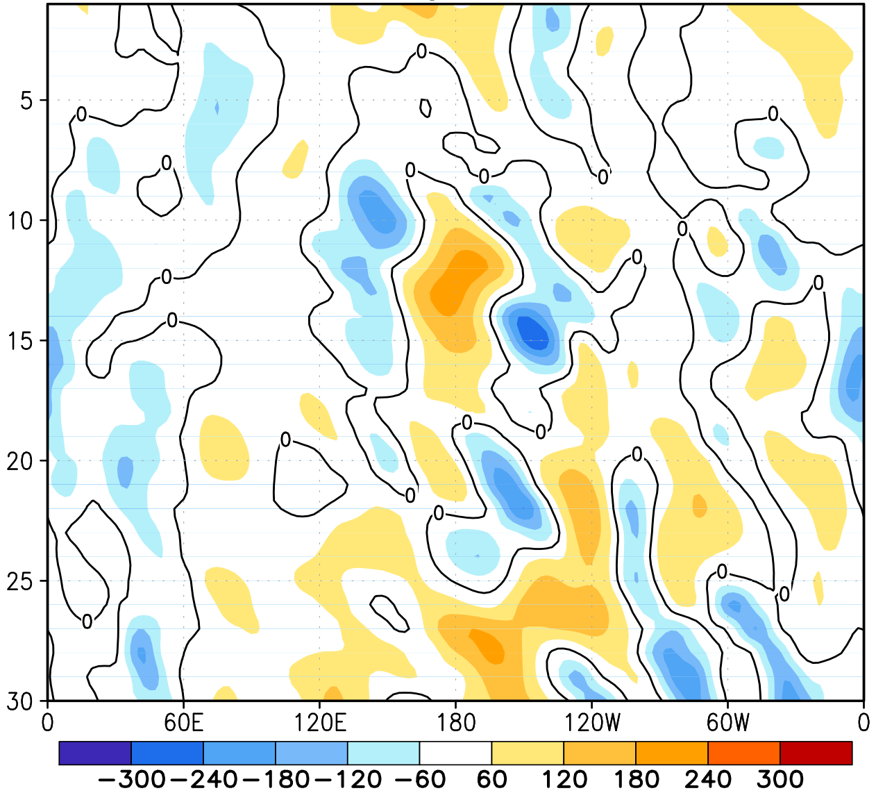
FIGURE E12. Northern Hemisphere: Daily 500-hPa height anomalies for SEP 2009 averaged over the 5° latitude band centered on 40°N. Positive values are indicated by solid contours and dark shading. Negative values are indicated by dashed contours and light shading. Contour interval is 60 m. Anomalies are departures from the 1979-95 base period daily means.
