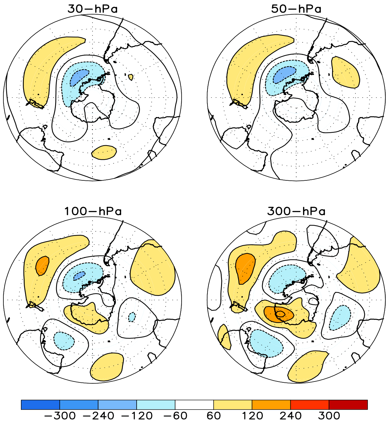
FIGURE S1. Stratospheric height anomalies (m) at selected levels for SEP 2009. Positive values are indicated by solid contours and dark shading. Negative values are indicated by dashed contours and light shading. Contour interval is 60 m. Anomalies are calculated from the 1979–95 base period means. Winter Hemisphere is shown.
