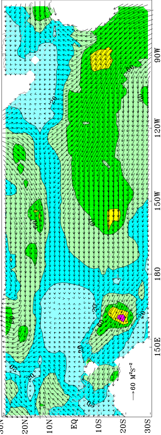
Near-real-time Objective FSU Pseudo-stress Magnitude and Vectors (10m) September 2009
