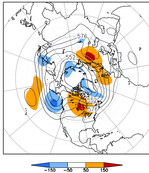
500-hPa Height (dm) & Anomalies (m) (Sep 1–15, 2009)
