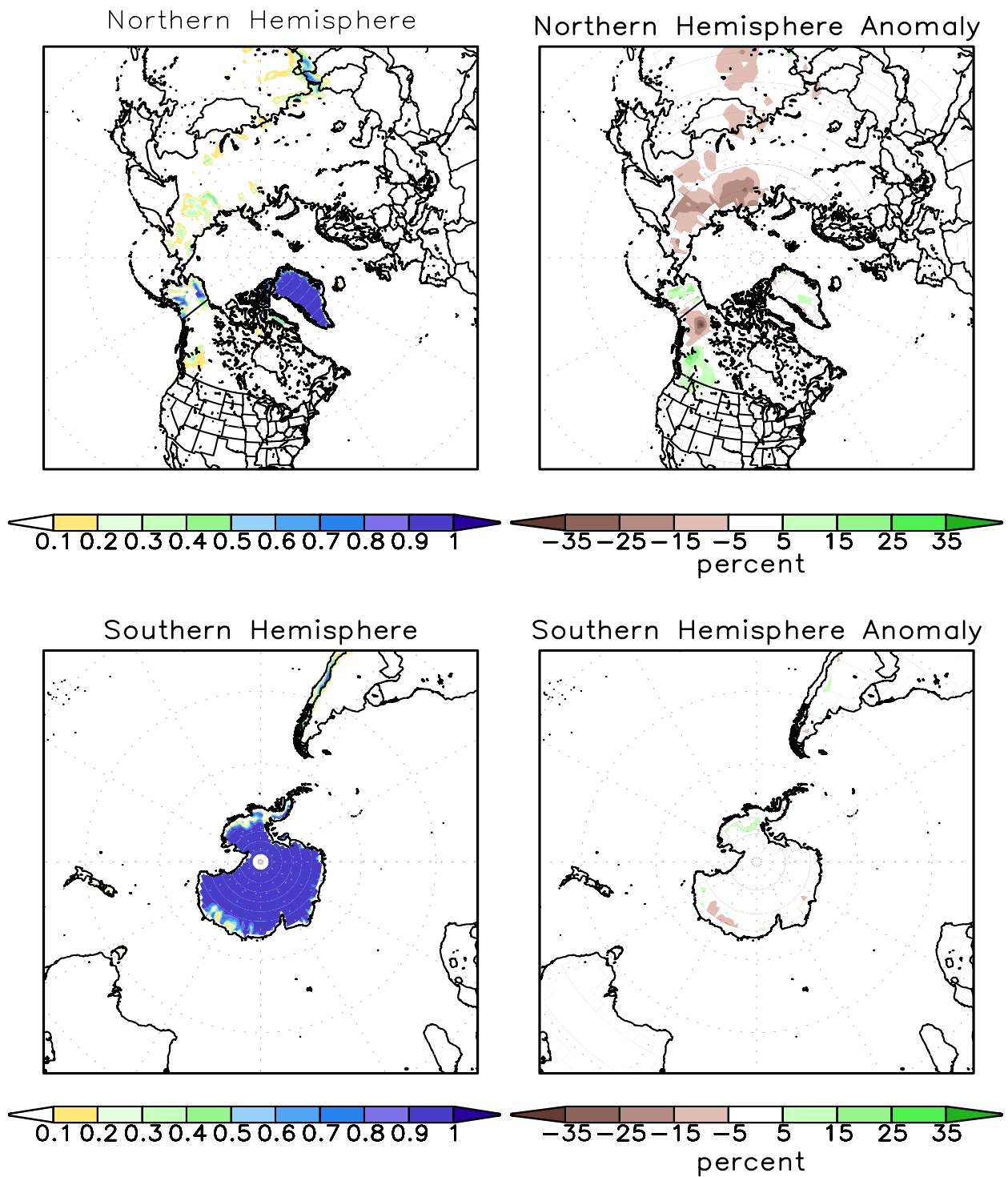
FIGURE A2.2. SSM/I derived snow cover frequency (%) (left) and snow cover anomaly (%) (right) for the month of SEP 2009 based on 1987 - 2006 base period for the Northern Hemisphere (top) and Southern Hemisphere (bottom). It is generated using the algorithm described by Ferraro et. al, 1996, Bull. Amer. Meteor. Soc., vol 77, 891-905.
