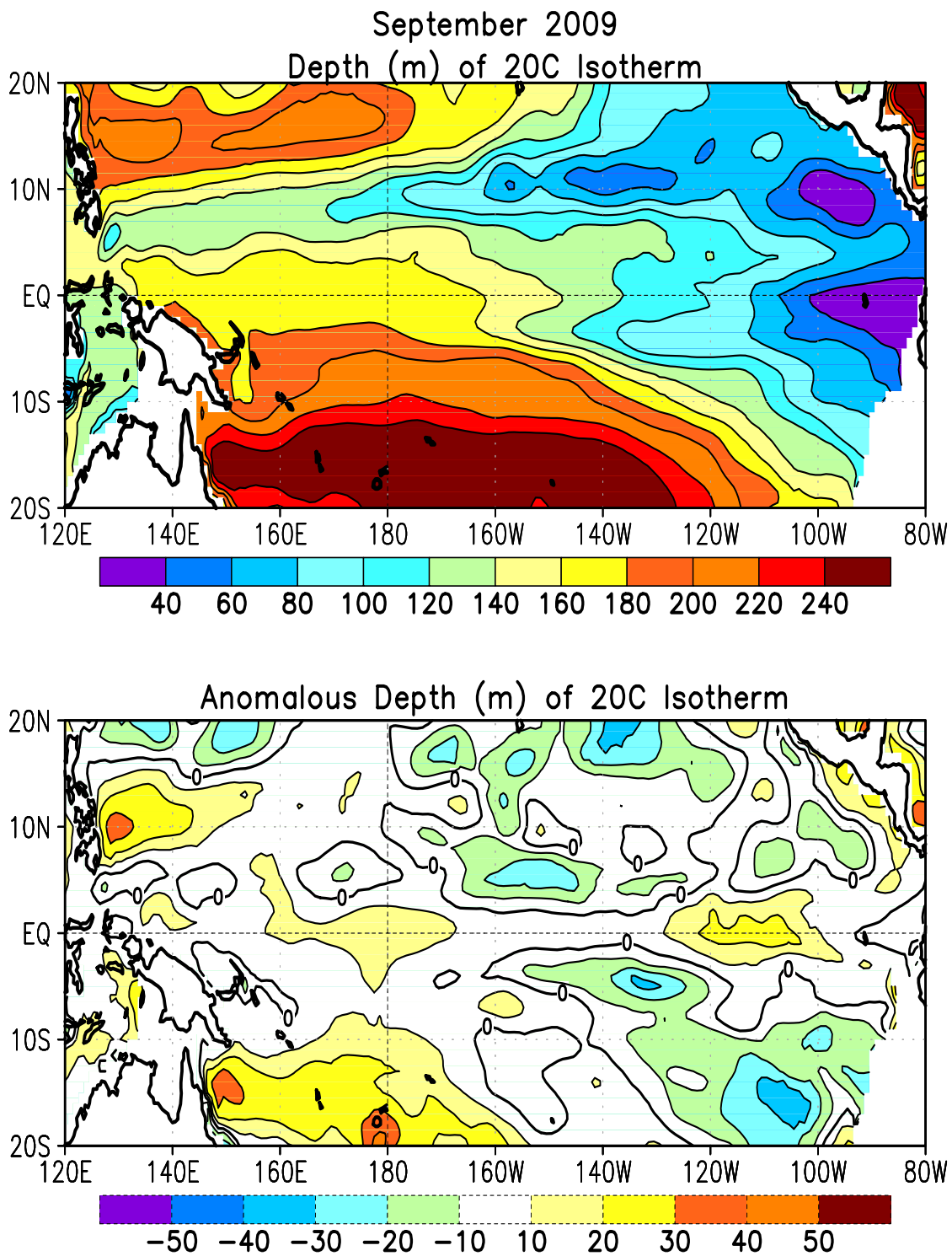
FIGURE T16. Mean (top) and anomalous (bottom) depth of the 20°C isotherm for SEP 2009. Contour interval is 40 m (top) and 10 m (bottom). Dashed contours in bottom panel indicate negative anomalies. Data are derived from the NCEP’s global ocean data assimilation system version 2 which assimilates oceanic observations into an oceanic GCM (Xue, Y. and Behringer, D.W., 2006: Operational global ocean data assimilation system at NCEP, to be submitted to BAMS). Anomalies are departures from the 1982–2004 base period means.
