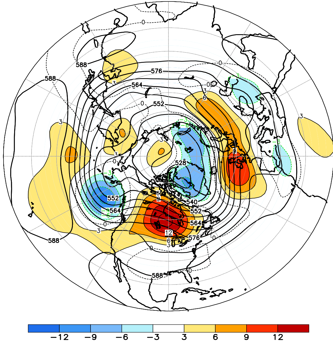
FIGURE E9. Northern Hemisphere mean and anomalous 500-hPa geopotential height (CDAS/Reanalysis) for SEP 2009. Mean heights are denoted by solid contours drawn at an interval of 6 dam. Anomaly contour interval is 3 dam with values less (greater) than -3 dam (3 dam) indicated by dark (light) shading. Anomalies are calculated as departures from the 1979-95 base period monthly means.
