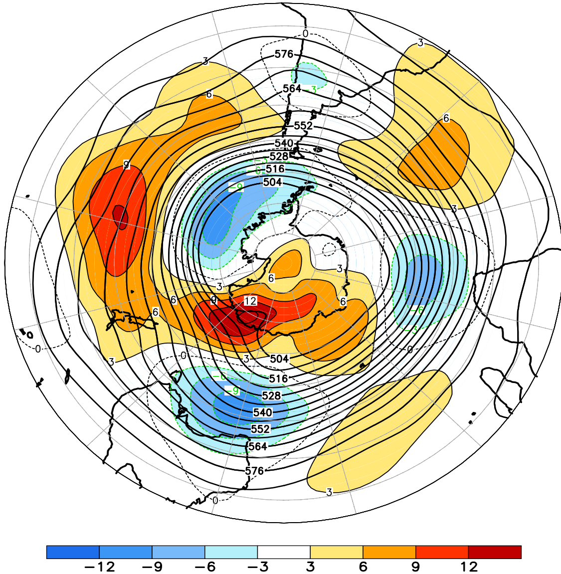
FIGURE E15. Southern Hemisphere mean and anomalous 500-hPa geopotential height (CDAS/Reanalysis) for SEP 2009. Mean heights are denoted by solid contours drawn at an interval of 6 dam. Anomaly contour interval is 3 dam with values less (greater) than -3 dam (3 dam) indicated by dark (light) shading. Anomalies are calculated as departures from the 1979-95 base period monthly means.
