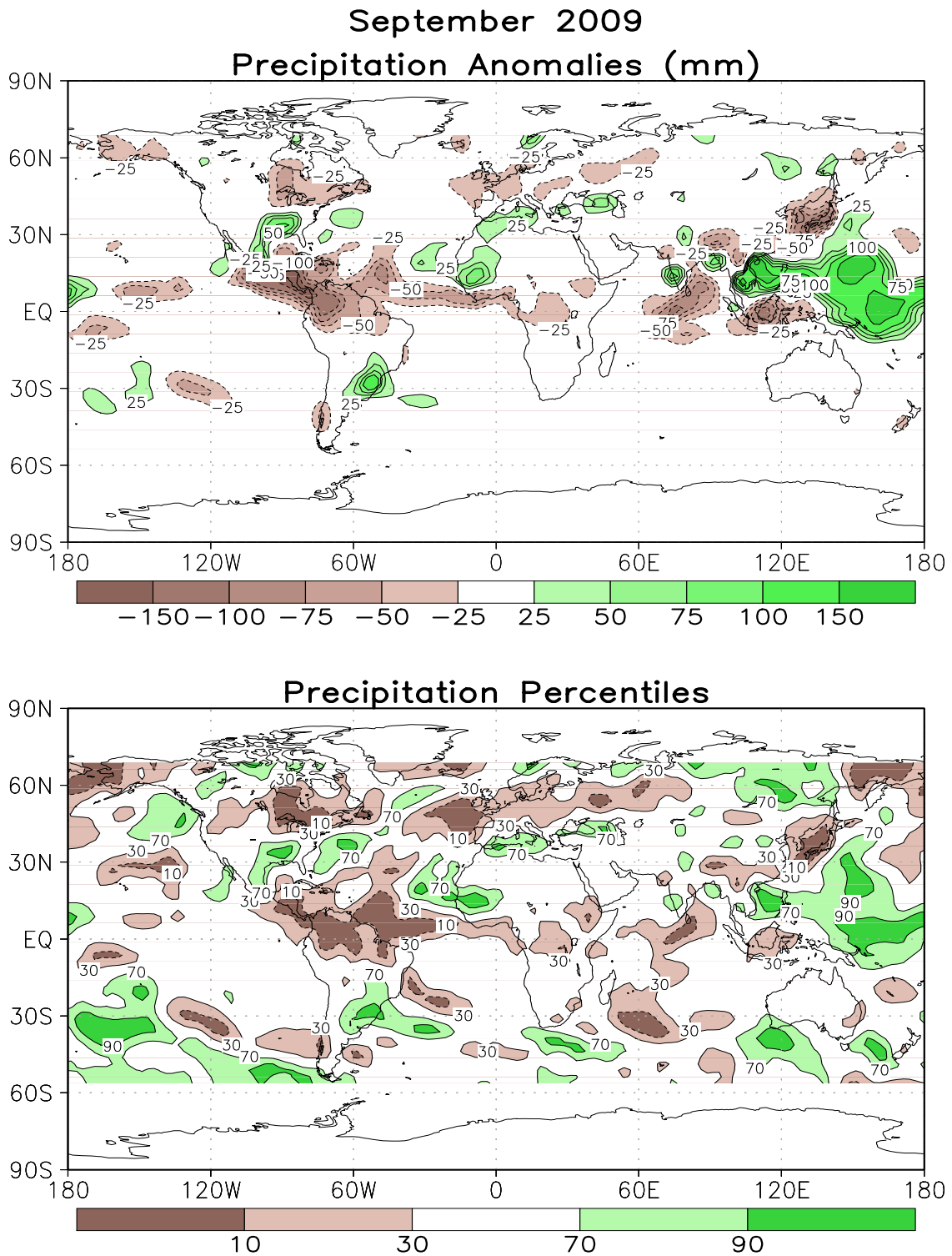
FIGURE E3. Anomalous precipitation (mm, top) and precipitation percentiles based on a Gamma distribution fit to the 1979–2000 base period data (bottom) for SEP 2009. Data are obtained from a merge of raingauge observations and satellite-derived precipitation estimates (Janowiak and Xie 1999, J. Climate , 12 , 3335–3342). Contours are drawn at 200, 100, 50, 25, -25, -50, -100, and -200 mm in top panel. Percentiles are not plotted in regions where mean monthly precipitation is <5mm/month.
