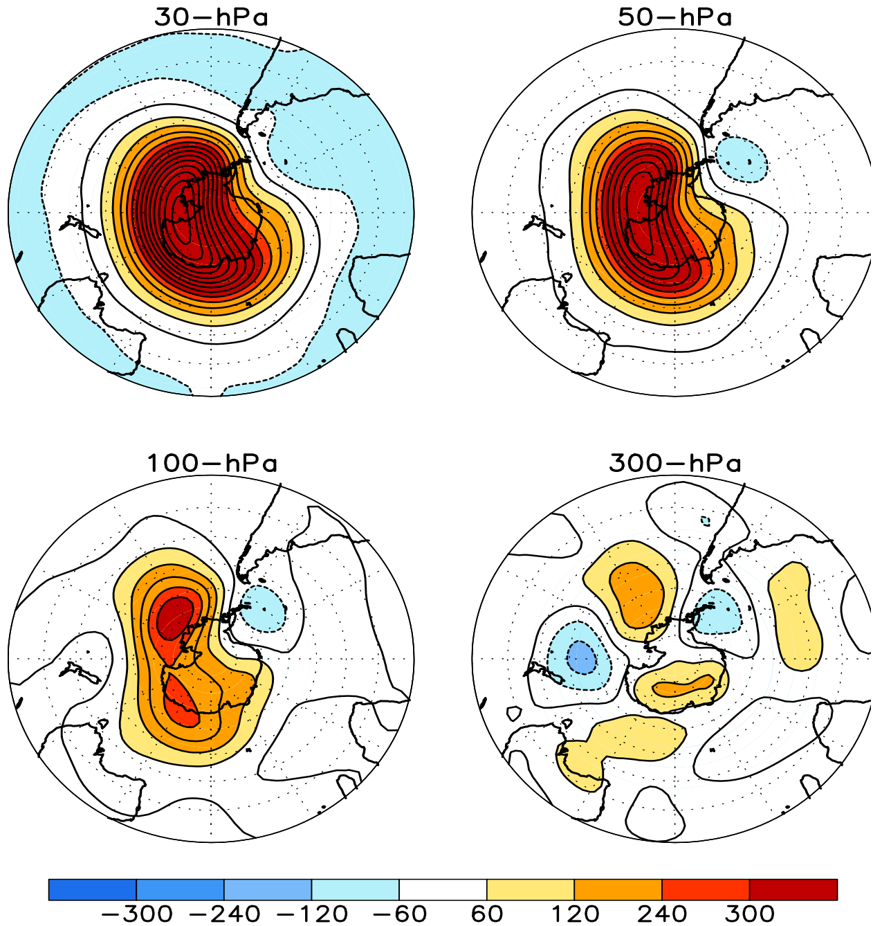
FIGURE S1. Stratospheric height anomalies (m) at selected levels for OCT 2012. Positive values are indicated by solid contours and dark shading. Negative values are indicated by dashed contours and light shading. Contour interval is 60 m. Anomalies are calculated from the 1981-2010 base period means. Winter Hemisphere is shown.
