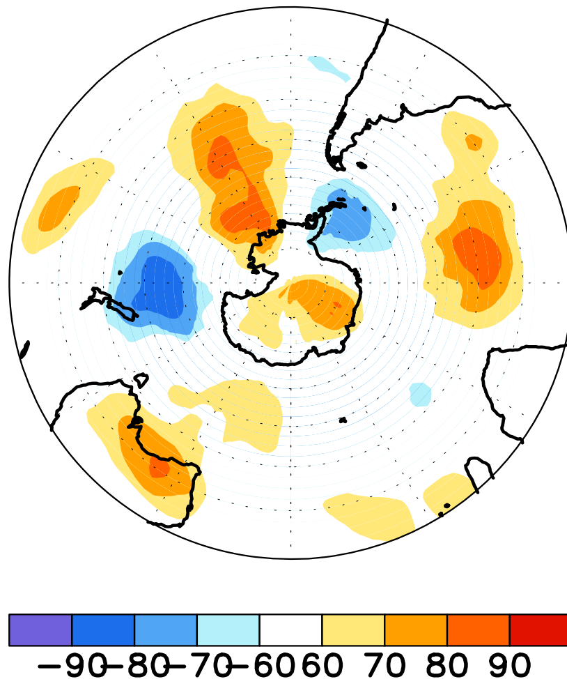
FIGURE E17. Southern Hemisphere percentage of days during OCT 2012 in which 500-hPa height anomalies greater than 15 m (red) and less than -15 m (blue) were observed. Values greater than 70% are shaded and contour in-
