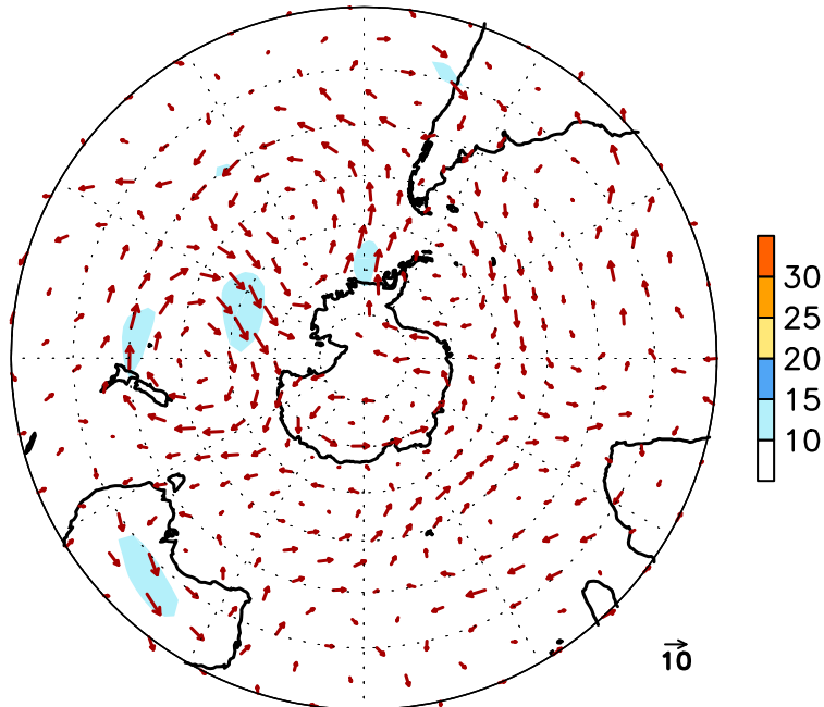
FIGURE E16. Southern Hemisphere mean (left) and anomalous (right) 300-hPa vector wind (CDAS/Reanalysis) for OCT 2012. Mean (anomaly) isotach contour interval is 10 (5) ms -1 . Values greater than 30 ms -1 (left) and 10 ms -1 (rights) are shaded. Anomalies are departures from the 1981-2010 base period monthly means.
