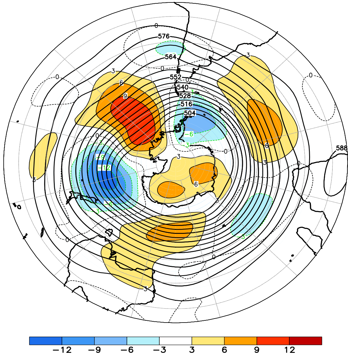
FIGURE E15. Southern Hemisphere mean and anomalous 500-hPa geopotential height (CDAS/Reanalysis) for OCT 2012. Mean heights are denoted by solid contours drawn at an interval of 6 dam. Anomaly contour interval is 3 dam with values less (greater) than -3 dam (3 dam) indicated by dark (light) shading. Anomalies are calculated as departures from the 1981-2010 base period monthly means.
