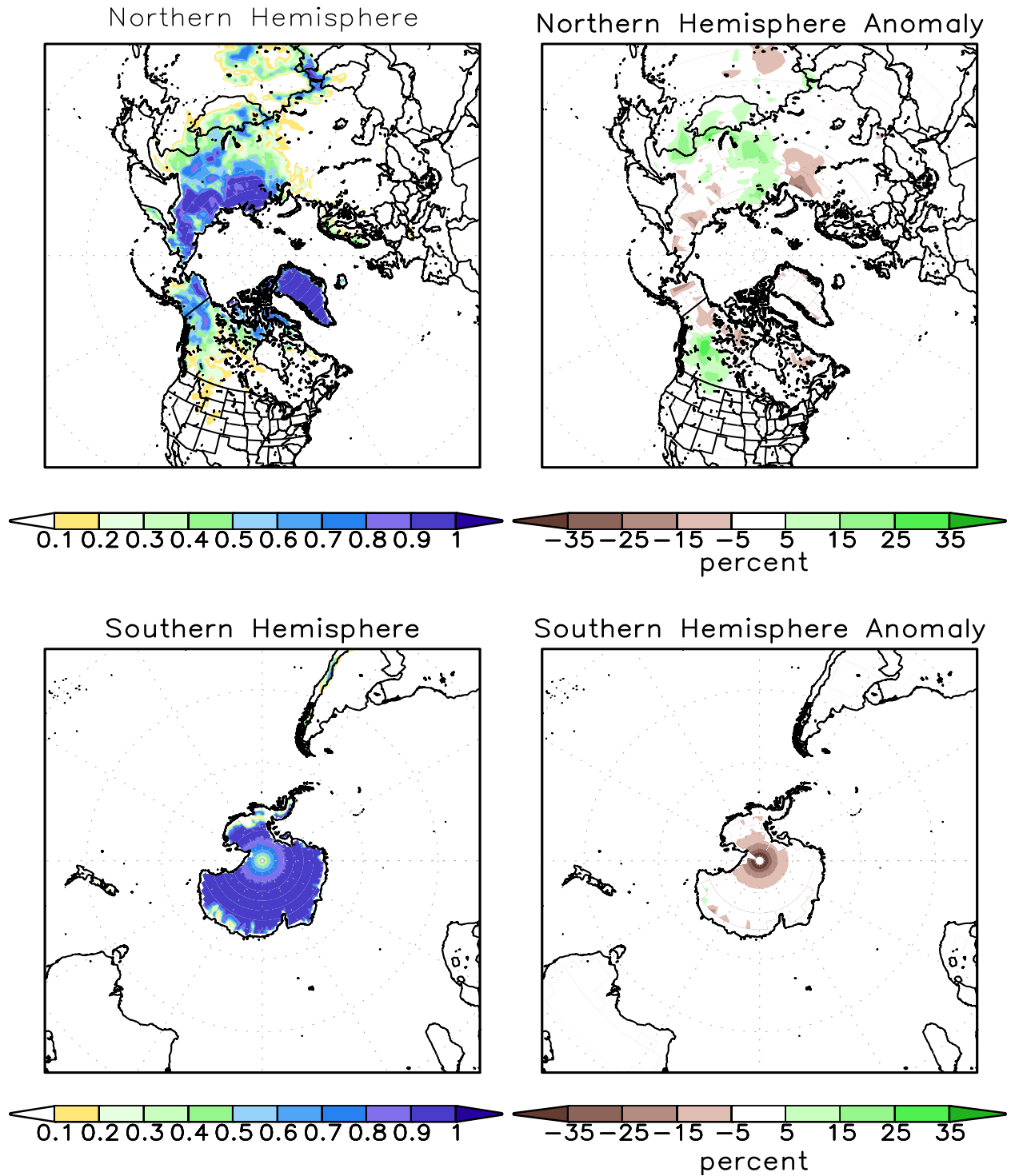
FIGURE A2.2. SSM/I derived snow cover frequency (%) (left) and snow cover anomaly (%) (right) for the month of OCT 2012 based on 1987 - 2010 base period for the Northern Hemisphere (top) and Southern Hemisphere (bottom). It is generated using the algorithm described by Ferraro et. al, 1996, Bull. Amer. Meteor. Soc., vol 77, 891-905.
