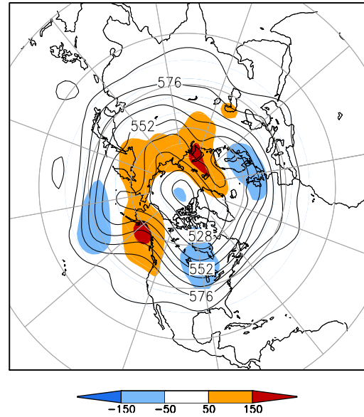
500-hPa Height (dm) & Anomalies (m) (Oct 1–15, 2012)
