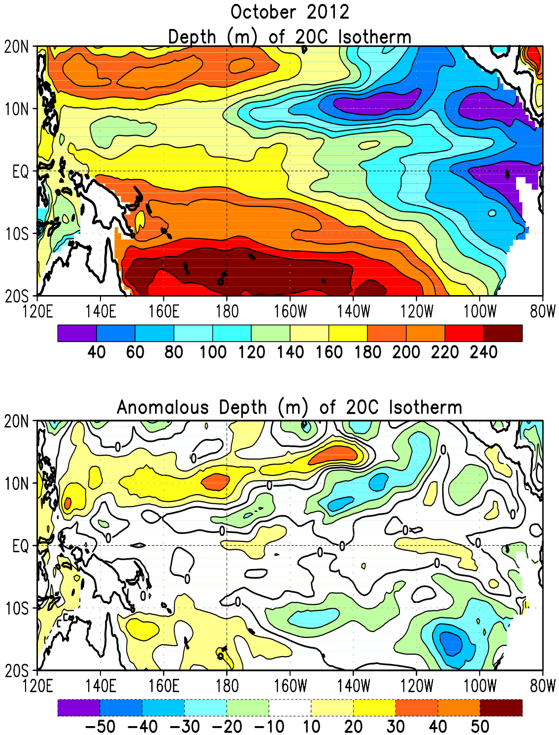
FIGURE T16. Mean (top) and anomalous (bottom) depth of the 20°C isotherm for OCT 2012. Contour interval is 40 m (top) and 10 m (bottom). Dashed contours in bottom panel indicate negative anomalies. Data are derived from the NCEP's global ocean data assimilation system version 2 which assimilates oceanic observations into an oceanic GCM (Xue, Y. and Behringer, D.W., 2006: Operational global ocean data assimilation system at NCEP, to be submitted to BAMS). Anomalies are departures from the 1981–2010 base period means.
