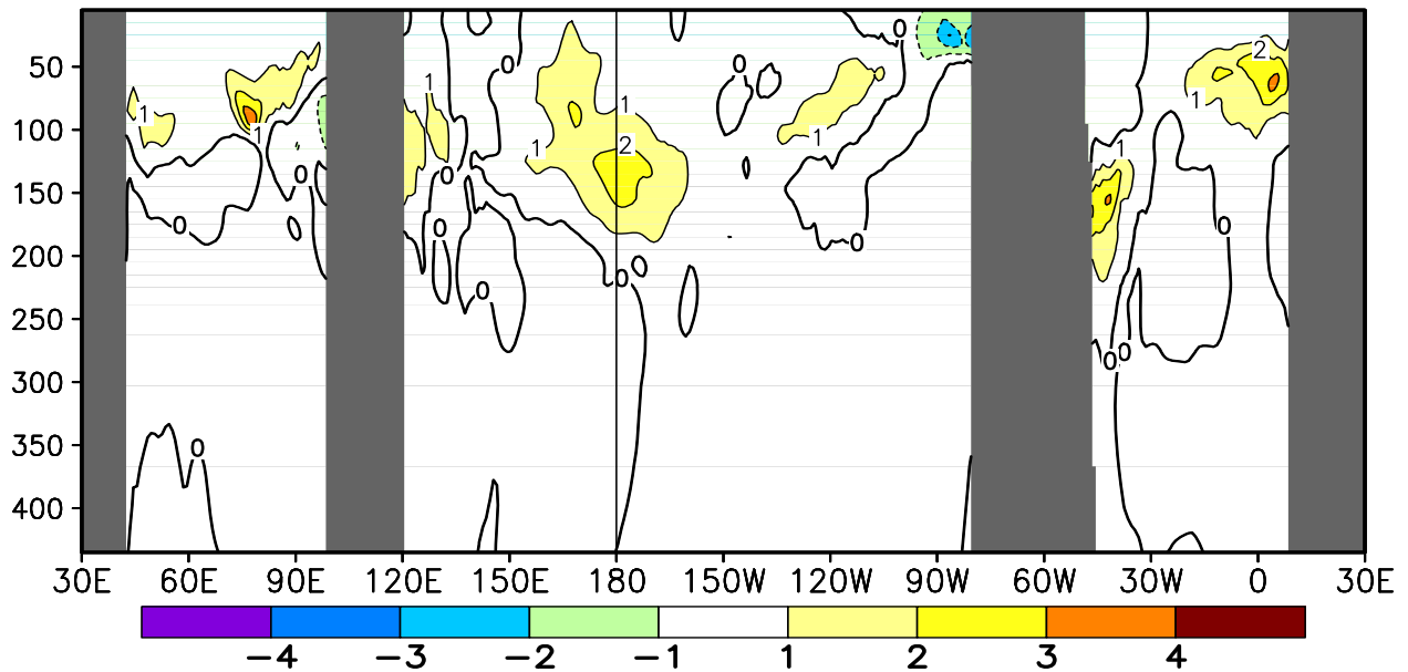
FIGURE T17. Equatorial depth–longitude section of ocean temperature (top) and ocean temperature anomalies (bottom) for OCT 2012. Contour interval is 1°C. Dashed contours in bottom panel indicate negative anomalies. Data are derived from the NCEP’s global ocean data assimilation system version 2 which assimilates oceanic observations into an oceanic GCM (Xue, Y. and Behringer, D.W., 2006: Operational global ocean data assimilation system at NCEP, to be submitted to BAMS). Anomalies are departures from the 1981–2010 base period means.
