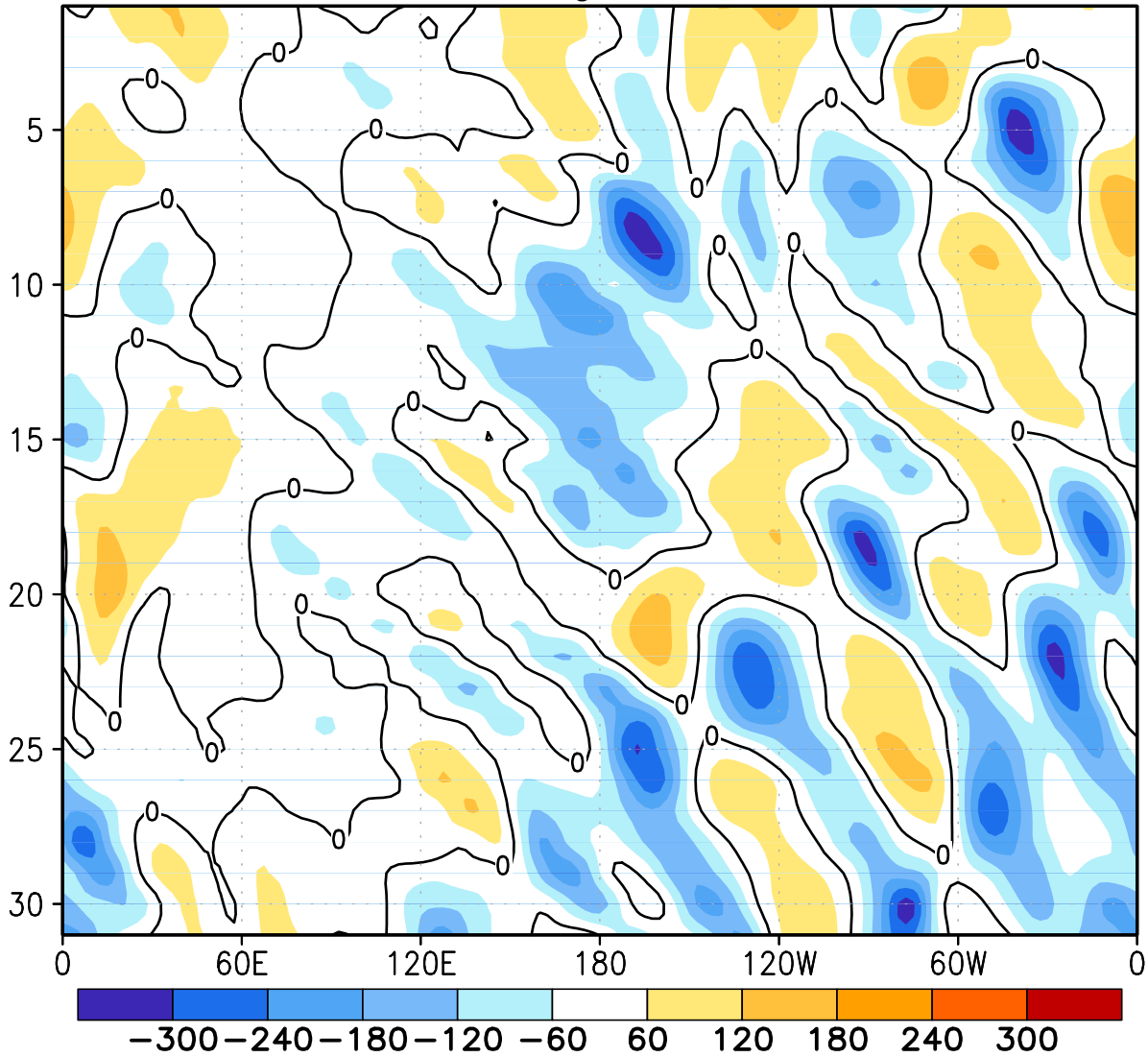
FIGURE E12. Northern Hemisphere: Daily 500-hPa height anomalies for OCT 2012 averaged over the 5° latitude band centered on 40°N. Positive values are indicated by solid contours and dark shading. Negative values are indicated by dashed contours and light shading. Contour interval is 60 m. Anomalies are departures from the 1981-2010 base period daily means.
