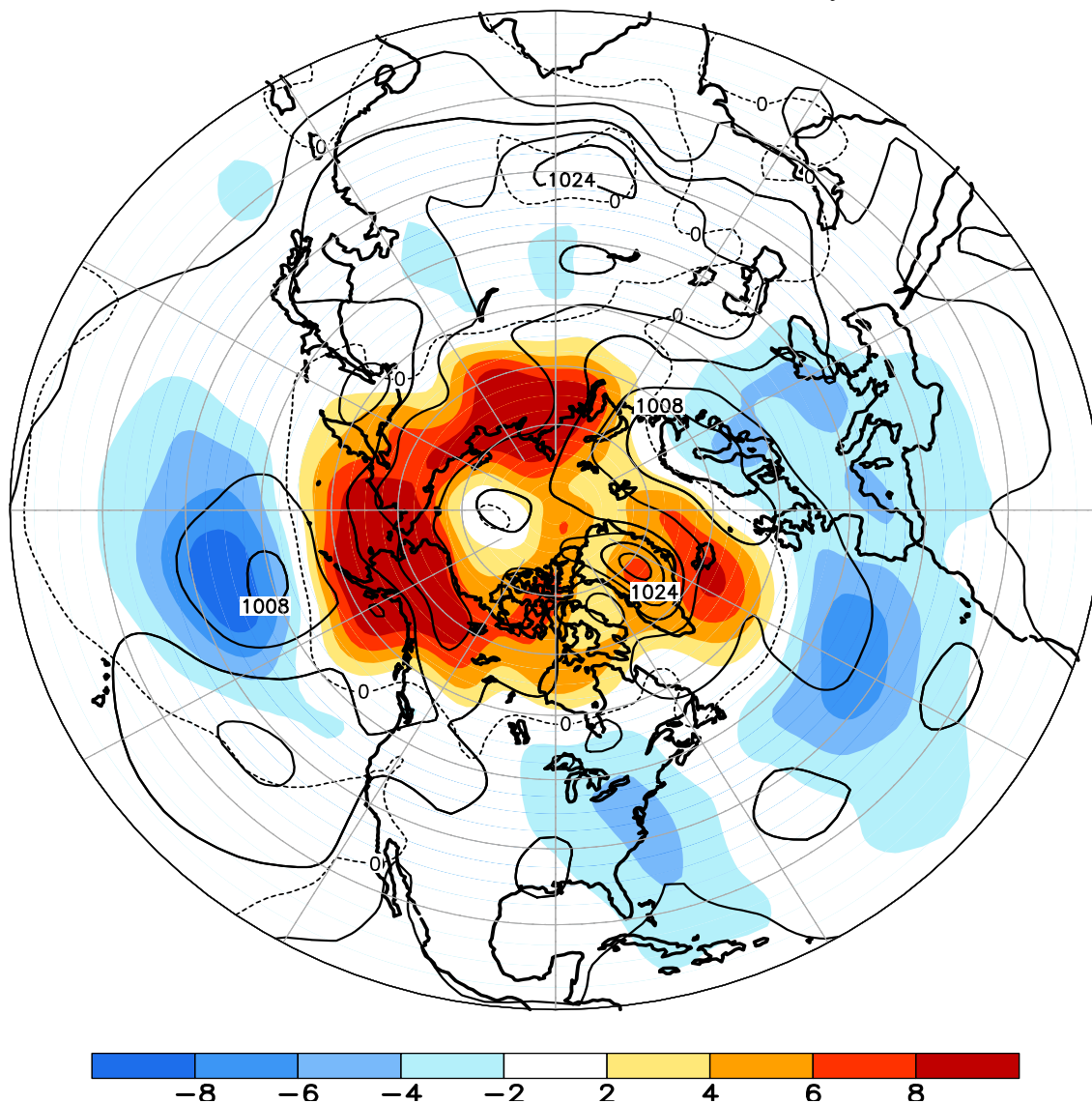
FIGURE E8. Northern Hemisphere mean and anomalous sea level pressure (CDAS/Reanalysis) for OCT 2012. Mean values are denoted by solid contours drawn at an interval of 4 hPa. Anomaly contour interval is 2 hPa with values less (greater) than -2 hPa (2 hPa) indicated by dark (light) shading. Anomalies are calculated as departures from the 1981-2010 base period monthly means.
