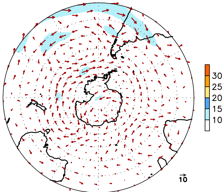
FIGURE E16. Southern Hemisphere mean (left) and anomalous (right) 300-hPa vector wind (CDAS/Reanalysis) for NOV 2015. Mean (anomaly) isotach contour interval is 10 (5) ms -1 . Values greater than 30 ms -1 (left) and 10 ms -1 (rights) are shaded. Anomalies are departures from the 1981-2010 base period monthly means.
