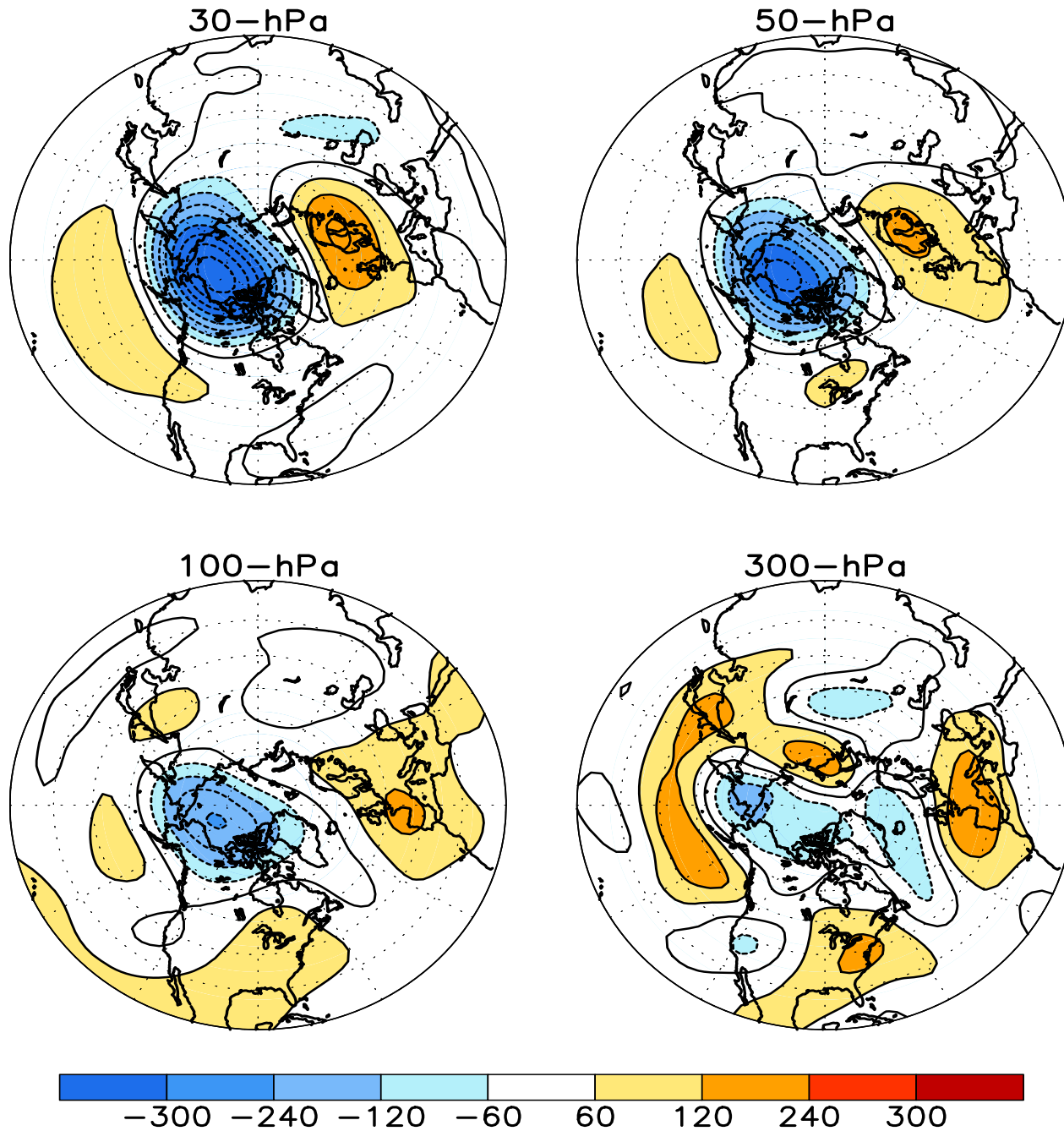
FIGURE S1. Stratospheric height anomalies (m) at selected levels for NOV 2015. Positive values are indicated by solid contours and dark shading. Negative values are indicated by dashed contours and light shading. Contour interval is 60 m. Anomalies are calculated from the 1981-2010 base period means. Winter Hemisphere is shown.
