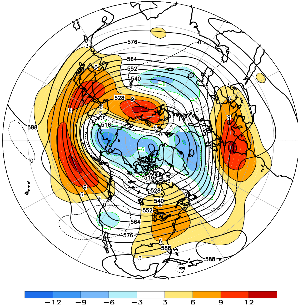
FIGURE E9. Northern Hemisphere mean and anomalous 500-hPa geopotential height (CDAS/Reanalysis) for NOV 2015. Mean heights are denoted by solid contours drawn at an interval of 6 dam. Anomaly contour interval is 3 dam with values less (greater) than -3 dam (3 dam) indicated by dark (light) shading. Anomalies are calculated as departures from the 1981-2010 base period monthly means.
