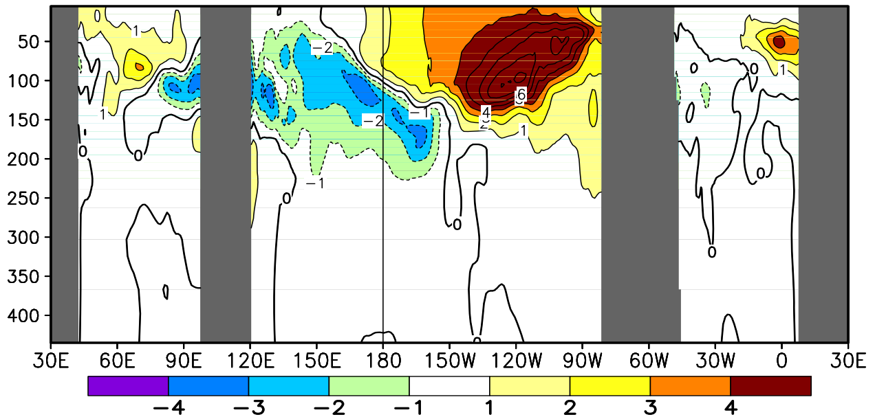
FIGURE T17. Equatorial depth–longitude section of ocean temperature (top) and ocean temperature anomalies (bottom) for NOV 2015. Contour interval is 1°C. Dashed contours in bottom panel indicate negative anomalies. Data are derived from the NCEP’s global ocean data assimilation system version 2 which assimilates oceanic observations into an oceanic GCM (Xue, Y. and Behringer, D.W., 2006: Operational global ocean data assimilation system at NCEP, to be submitted to BAMS). Anomalies are departures from the 1981–2010 base period means.
