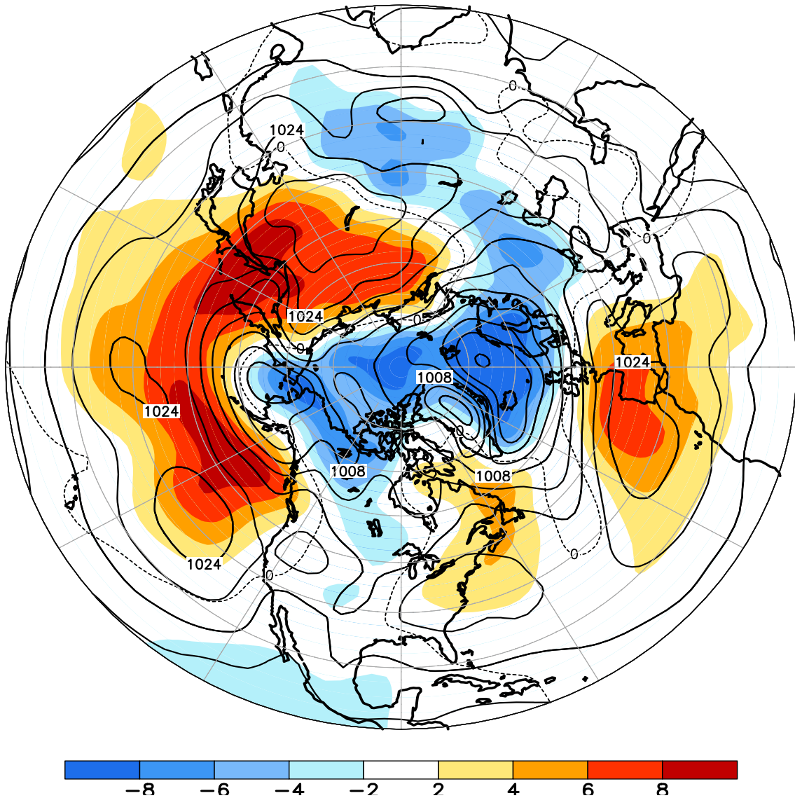
FIGURE E8. Northern Hemisphere mean and anomalous sea level pressure (CDAS/Reanalysis) for NOV 2015. Mean values are denoted by solid contours drawn at an interval of 4 hPa. Anomaly contour interval is 2 hPa with values less (greater) than -2 hPa (2 hPa) indicated by dark (light) shading. Anomalies are calculated as departures from the 1981-2010 base period monthly means.
