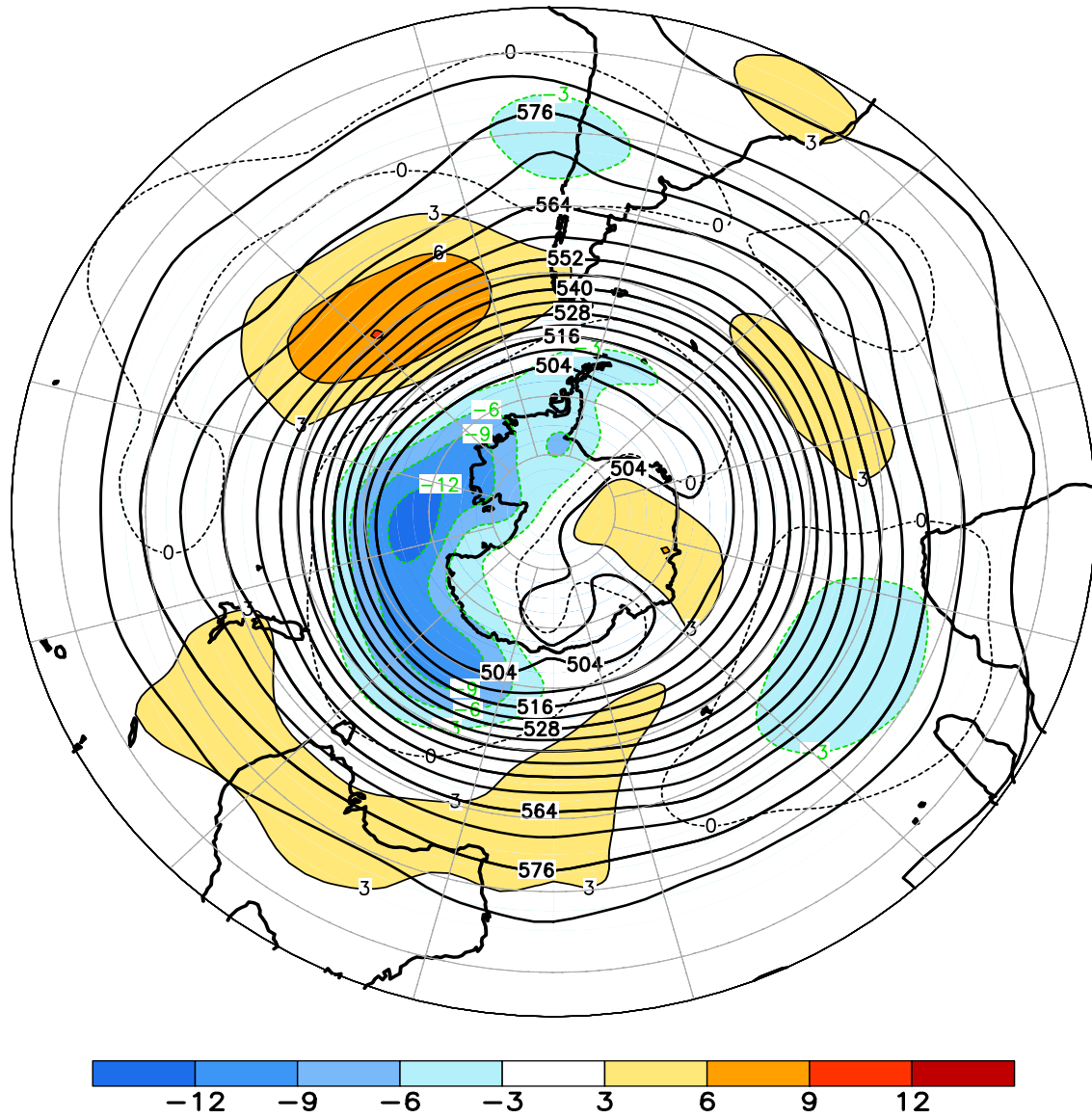
FIGURE E15. Southern Hemisphere mean and anomalous 500-hPa geopotential height (CDAS/Reanalysis) for NOV 2015. Mean heights are denoted by solid contours drawn at an interval of 6 dam. Anomaly contour interval is 3 dam with values less (greater) than -3 dam (3 dam) indicated by dark (light) shading. Anomalies are calculated as departures from the 1981-2010 base period monthly means.
