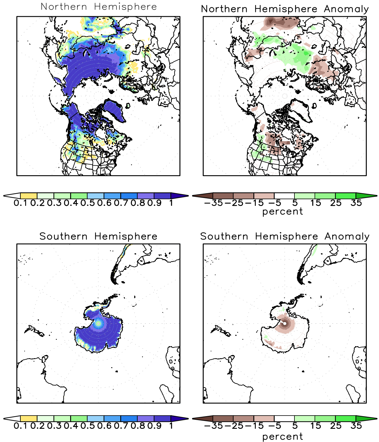
FIGURE A2.2. SSM/I derived snow cover frequency (%) (left) and snow cover anomaly (%) (right) for the month of NOV 2015 based on 1987 - 2010 base period for the Northern Hemisphere (top) and Southern Hemisphere (bottom). It is generated using the algorithm described by Ferraro et. al, 1996, Bull. Amer. Meteor. Soc., vol 77, 891-905.
