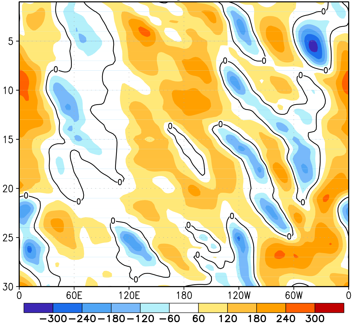
FIGURE E12. Northern Hemisphere: Daily 500-hPa height anomalies for NOV 2015 averaged over the 5° latitude band centered on 40°N. Positive values are indicated by solid contours and dark shading. Negative values are indicated by dashed contours and light shading. Contour interval is 60 m. Anomalies are departures from the 1981-2010 base period daily means.
