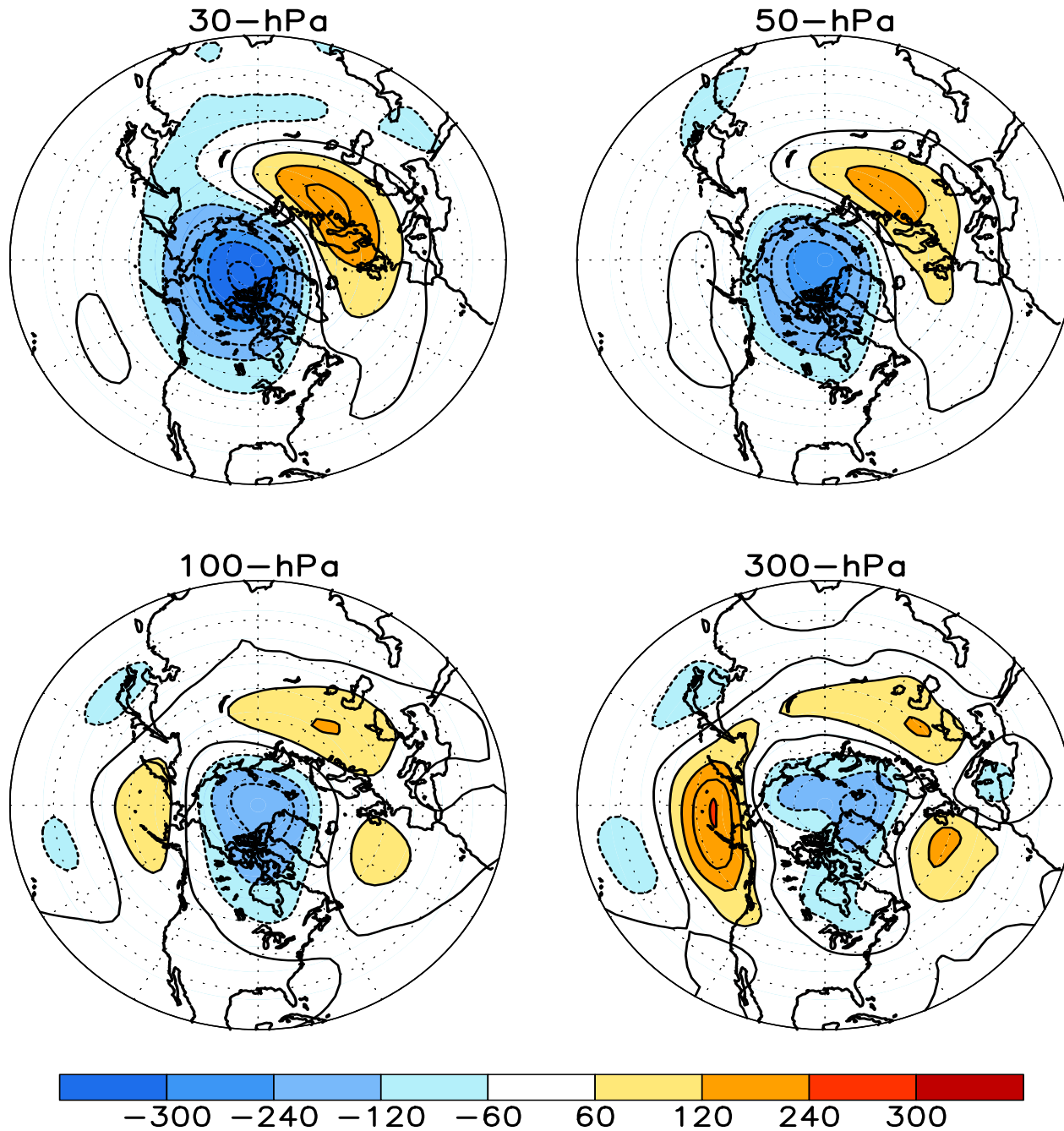
FIGURE S1. Stratospheric height anomalies (m) at selected levels for NOV 2013. Positive values are indicated by solid contours and dark shading. Negative values are indicated by dashed contours and light shading. Contour interval is 60 m. Anomalies are calculated from the 1981-2010 base period means. Winter Hemisphere is shown.
