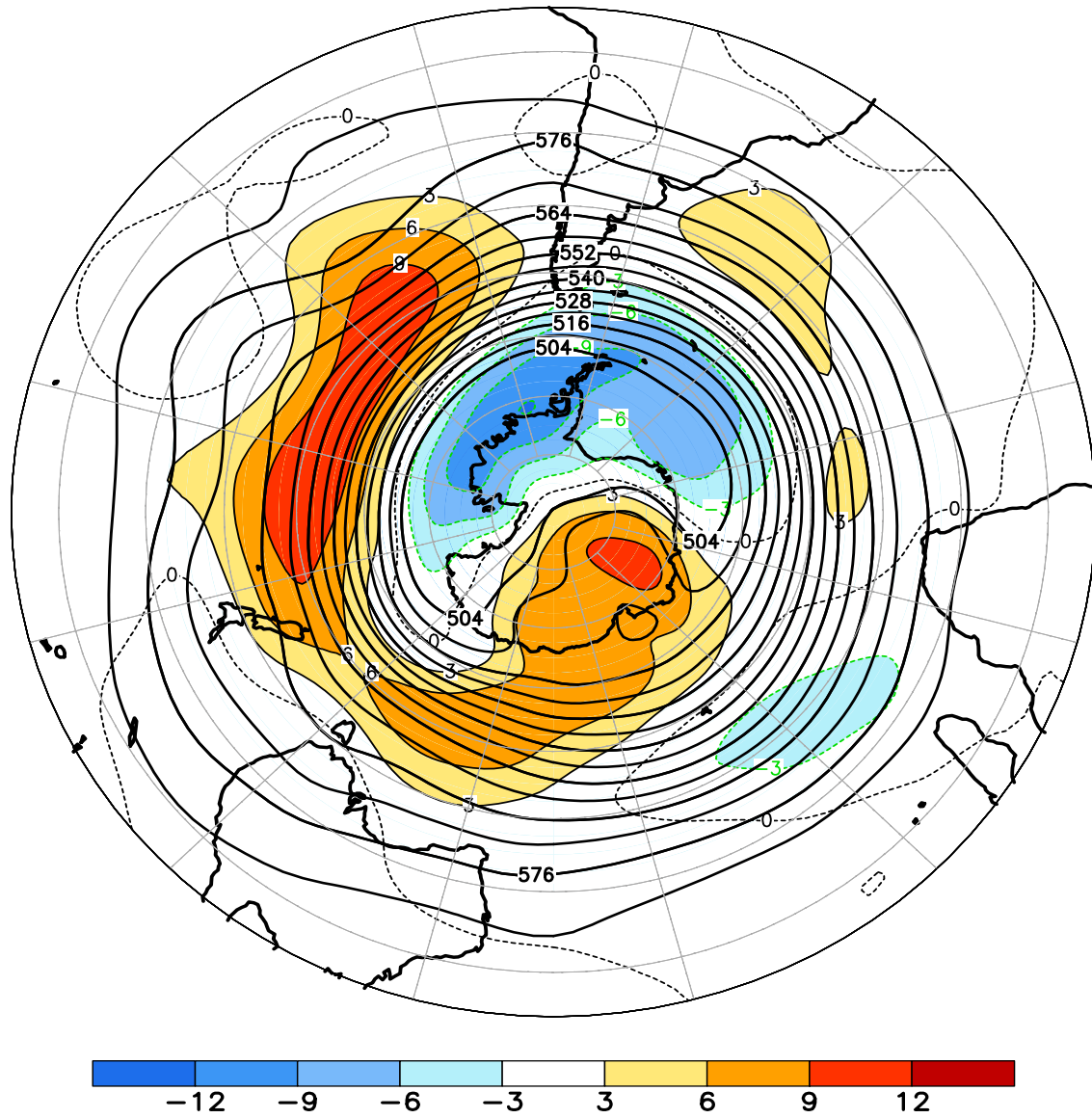
FIGURE E15. Southern Hemisphere mean and anomalous 500-hPa geopotential height (CDAS/Reanalysis) for NOV 2013. Mean heights are denoted by solid contours drawn at an interval of 6 dam. Anomaly contour interval is 3 dam with values less (greater) than -3 dam (3 dam) indicated by dark (light) shading. Anomalies are calculated as departures from the 1981-2010 base period monthly means.
