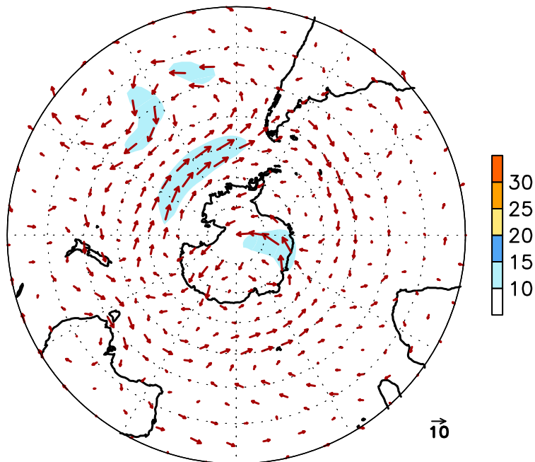
FIGURE E16. Southern Hemisphere mean (left) and anomalous (right) 300-hPa vector wind (CDAS/Reanalysis) for NOV 2013. Mean (anomaly) isotach contour interval is 10 (5) \text{ms}^{-1} . Values greater than 30 \text{ms}^{-1} (left) and 10 \text{ms}^{-1} (rights) are shaded. Anomalies are departures from the 1981-2010 base period monthly means.
