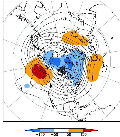
500-hPa Height (dm) & Anomalies (m) (Nov 1–15, 2013)
