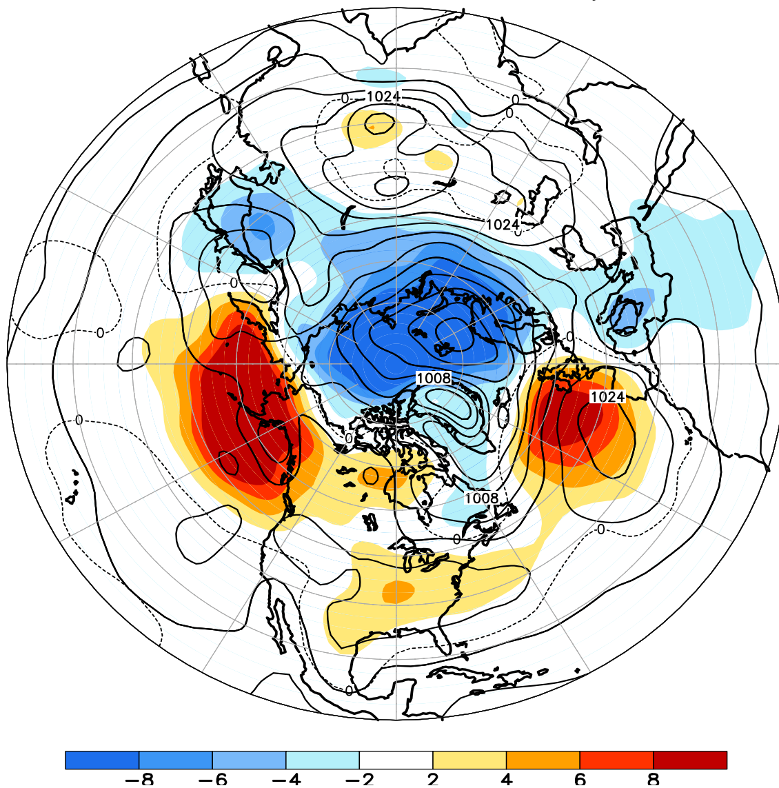
FIGURE E8. Northern Hemisphere mean and anomalous sea level pressure (CDAS/Reanalysis) for NOV 2013. Mean values are denoted by solid contours drawn at an interval of 4 hPa. Anomaly contour interval is 2 hPa with values less (greater) than -2 hPa (2 hPa) indicated by dark (light) shading. Anomalies are calculated as departures from the 1981-2010 base period monthly means.
