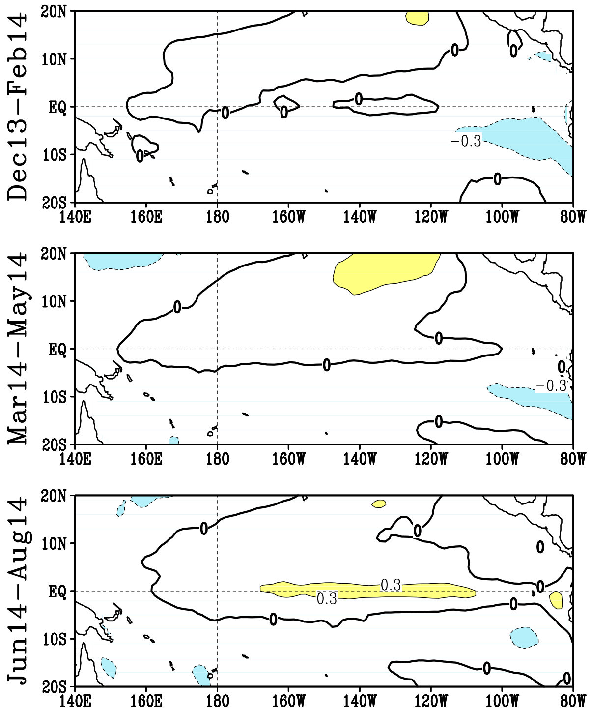
FIGURE F5. Predicted 3-month average sea surface temperature anomalies from the NCEP/CPC Markov model (Xue et al. 2000, J. Climate , 13 , 849-871). The forecast is initiated in NOV 2013 . Contour interval is 0.3C and negative anomalies are indicated by dashed contours. Anomalies are calculated relative to the 1971-2000 climatology.
