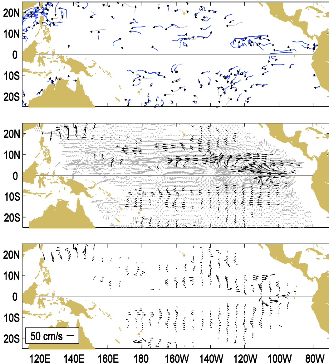
Figure A1.1 Top: Movements of drifting buoys in the tropical Pacific Ocean during November 2013. The linear segments of each trajectory represent a one week displacement. Trajectories of buoys which have lost their subsurface drogues are gray; those with drogues are black. Middle: Monthly mean currents calculated from all buoys 1993-2002 (gray), and currents measured by the drogued
