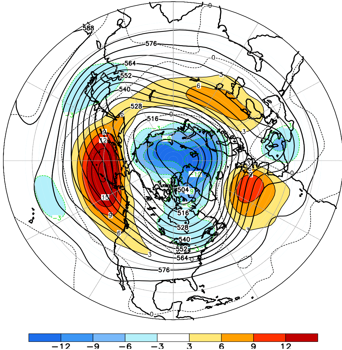
FIGURE E9. Northern Hemisphere mean and anomalous 500-hPa geopotential height (CDAS/Reanalysis) for NOV 2013. Mean heights are denoted by solid contours drawn at an interval of 6 dam. Anomaly contour interval is 3 dam with values less (greater) than -3 dam (3 dam) indicated by dark (light) shading. Anomalies are calculated as departures from the 1981-2010 base period monthly means.
