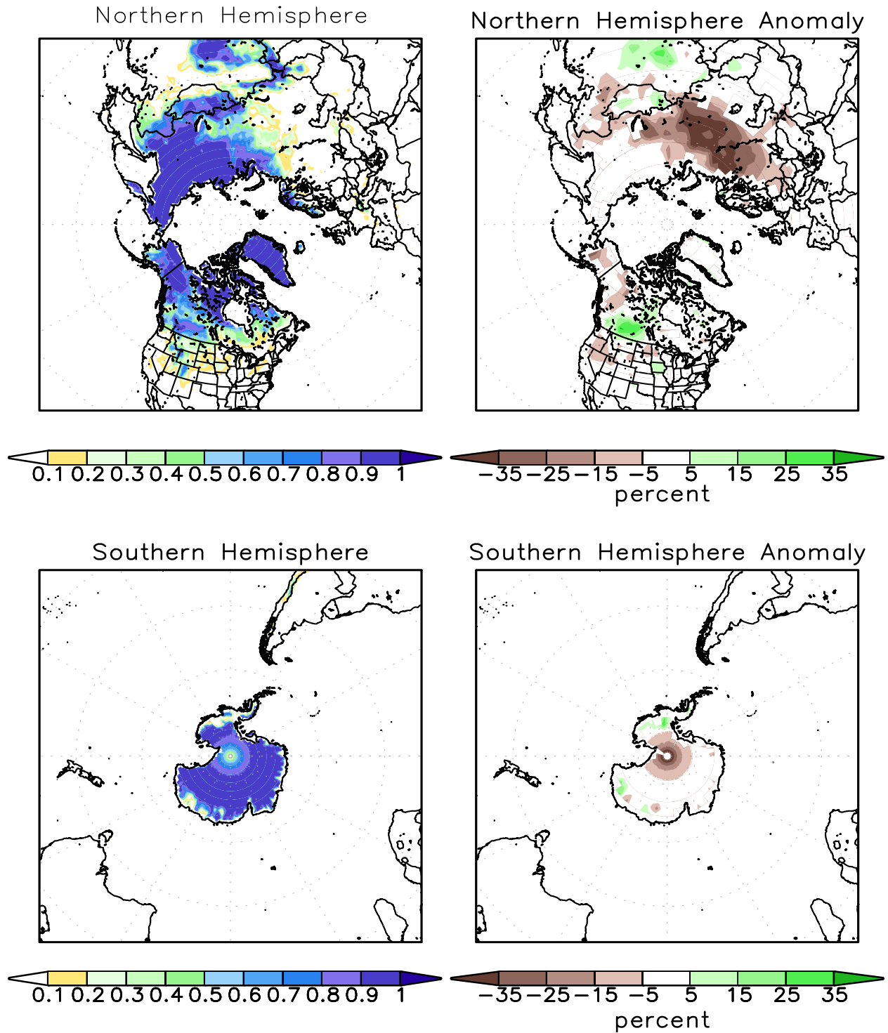
FIGURE A2.2. SSM/I derived snow cover frequency (%) (left) and snow cover anomaly (%) (right) for the month of NOV 2013 based on 1987 - 2010 base period for the Northern Hemisphere (top) and Southern Hemisphere (bottom). It is generated using the algorithm described by Ferraro et. al, 1996, Bull. Amer. Meteor. Soc., vol 77, 891-905.
