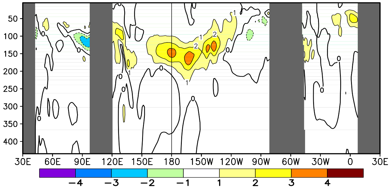
FIGURE T17. Equatorial depth–longitude section of ocean temperature (top) and ocean temperature anomalies (bottom) for NOV 2013. Contour interval is 1°C. Dashed contours in bottom panel indicate negative anomalies. Data are derived from the NCEP’s global ocean data assimilation system version 2 which assimilates oceanic observations into an oceanic GCM (Xue, Y. and Behringer, D.W., 2006: Operational global ocean data assimilation system at NCEP, to be submitted to BAMS). Anomalies are departures from the 1981–2010 base period means.
