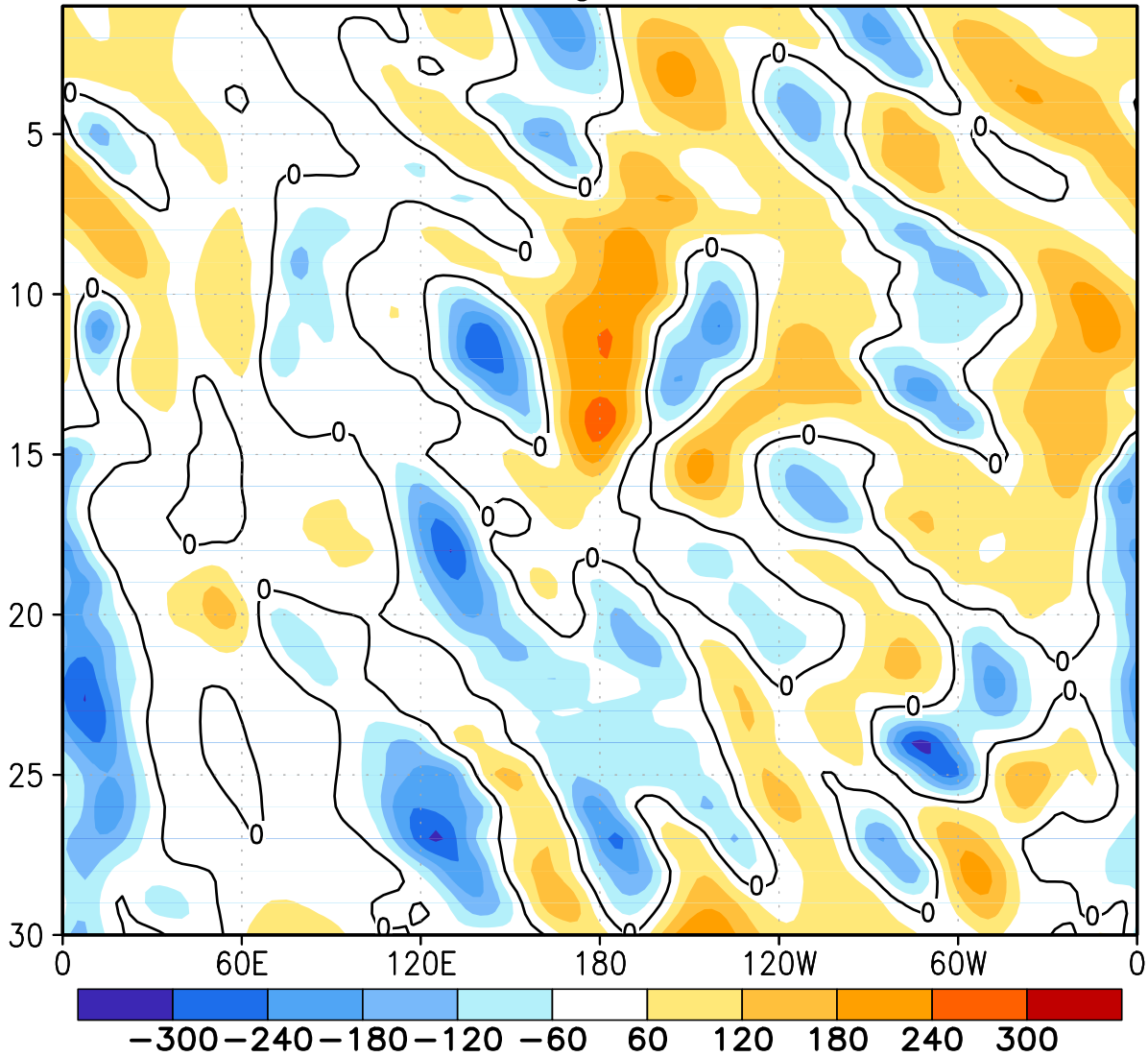
FIGURE E12. Northern Hemisphere: Daily 500-hPa height anomalies for NOV 2013 averaged over the 5° latitude band centered on 40°N. Positive values are indicated by solid contours and dark shading. Negative values are indicated by dashed contours and light shading. Contour interval is 60 m. Anomalies are departures from the 1981-2010 base period daily means.
