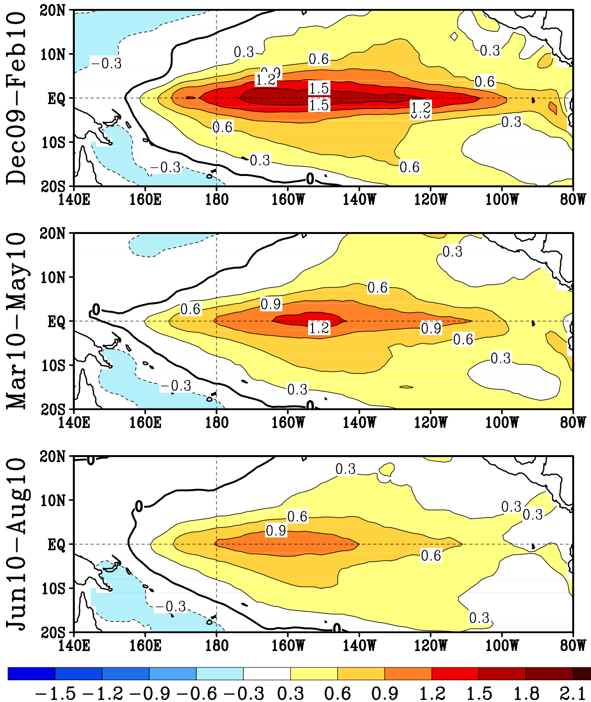
FIGURE F5. Predicted 3-month average sea surface temperature anomalies from the NCEP/CPC Markov model (Xue et al. 2000, J. Climate , 13 , 849-871). The forecast is initiated in NOV 2009 . Contour interval is 0.3C and negative anomalies are indicated by dashed contours. Anomalies are calculated relative to the 1971-2000 climatology.
