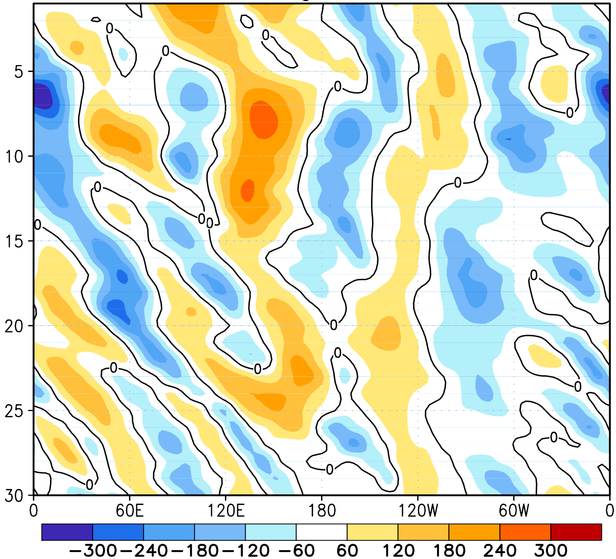
FIGURE E18. Southern Hemisphere: Daily 500-hPa height anomalies for NOV 2009 averaged over the 5° latitude band centered on 40°S. Positive values are indicated by solid contours and dark shading. Negative values are indicated by dashed contours and light shading. Contour interval is 60 m. Anomalies are departures from the 1979-95 base period daily means.
