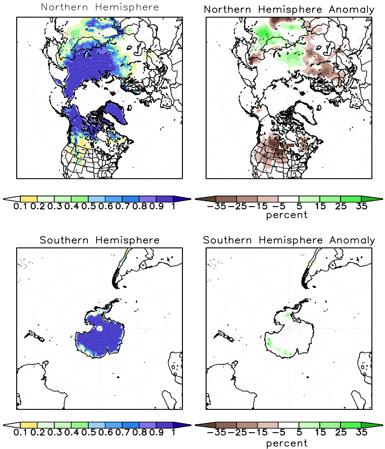
FIGURE A2.2. SSM/I derived snow cover frequency (%) (left) and snow cover anomaly (%) (right) for the month of NOV 2009 based on 1987 - 2006 base period for the Northern Hemisphere (top) and Southern Hemisphere (bottom). It is generated using the algorithm described by Ferraro et. al, 1996, Bull. Amer. Meteor. Soc., vol 77, 891-905.
