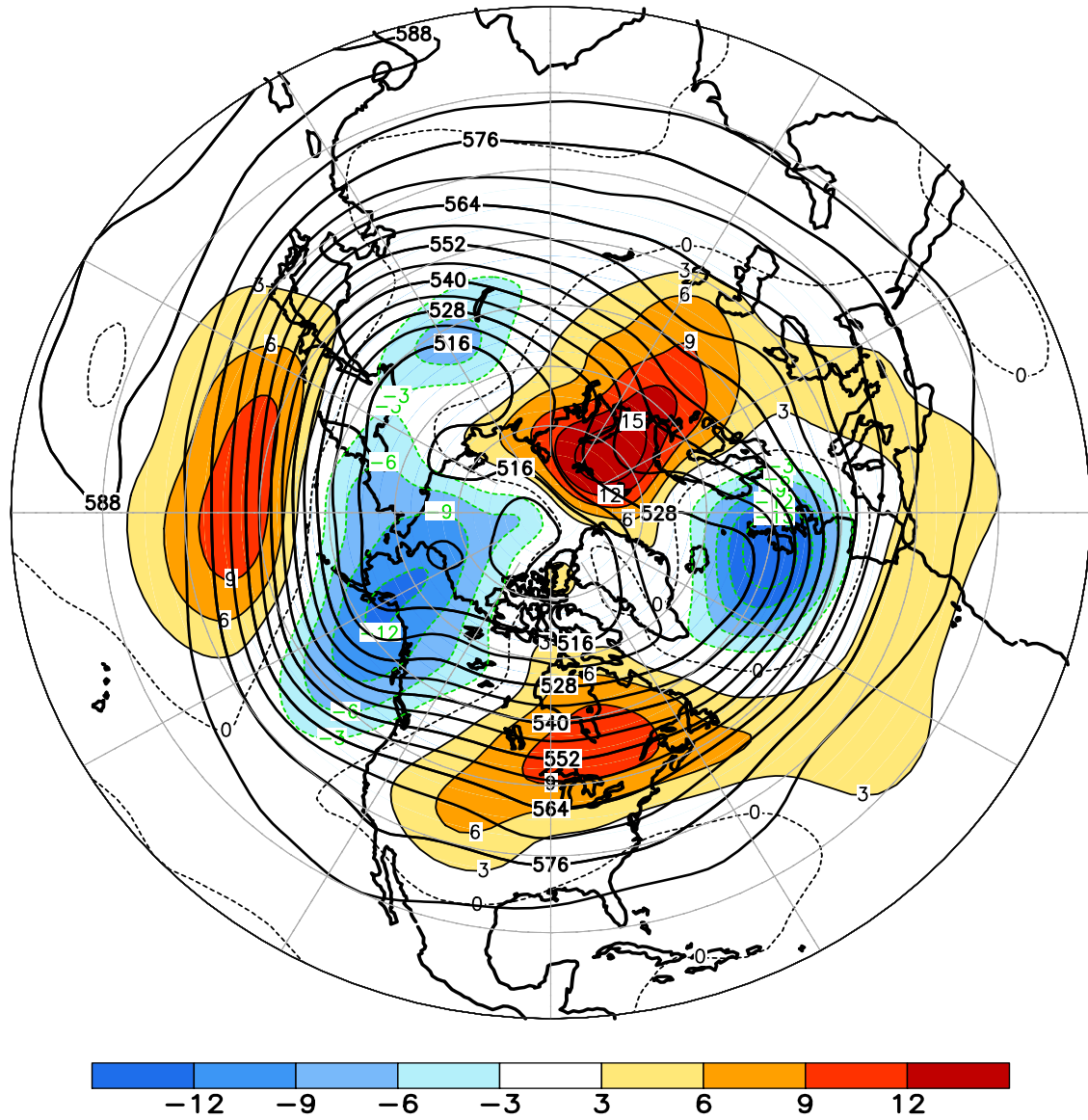
FIGURE E9. Northern Hemisphere mean and anomalous 500-hPa geopotential height (CDAS/Reanalysis) for NOV 2009. Mean heights are denoted by solid contours drawn at an interval of 6 dam. Anomaly contour interval is 3 dam with values less (greater) than -3 dam (3 dam) indicated by dark (light) shading. Anomalies are calculated as departures from the 1979-95 base period monthly means.
