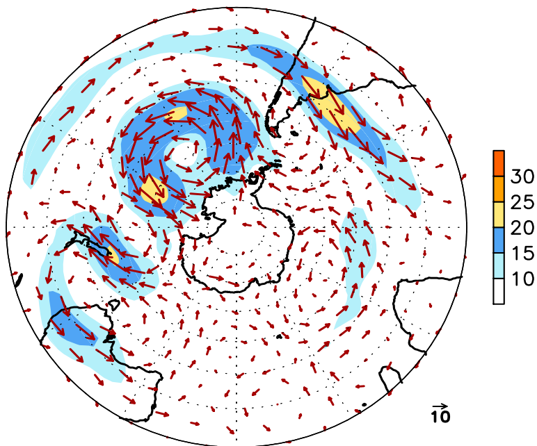
FIGURE E16. Southern Hemisphere mean (left) and anomalous (right) 300-hPa vector wind (CDAS/Reanalysis) for NOV 2009. Mean (anomaly) isotach contour interval is 10 (5) \text{ms}^{-1} . Values greater than 30 \text{ms}^{-1} (left) and 10 \text{ms}^{-1} (rights) are shaded. Anomalies are departures from the 1979-95 base period monthly means.
