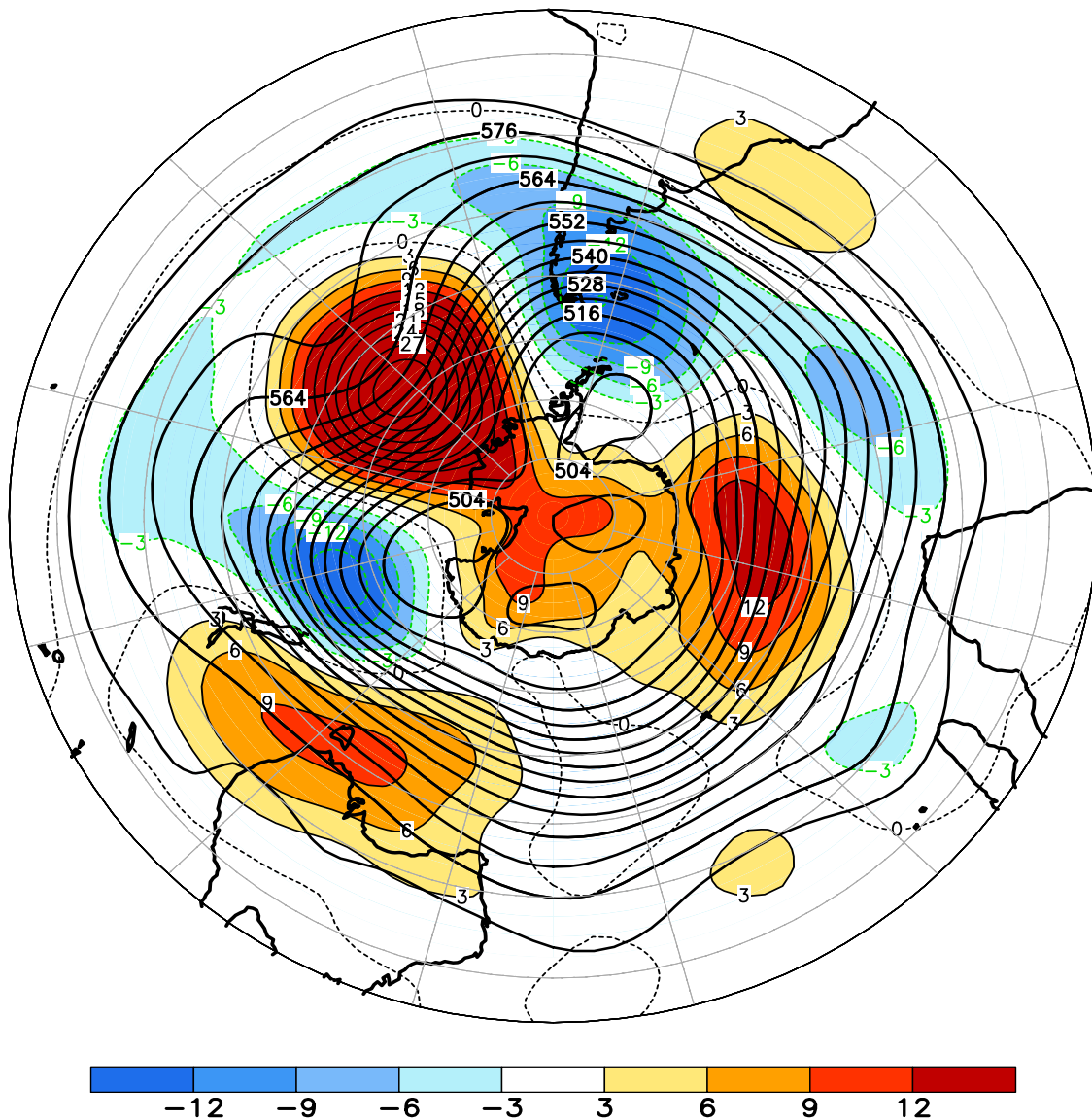
FIGURE E15. Southern Hemisphere mean and anomalous 500-hPa geopotential height (CDAS/Reanalysis) for NOV 2009. Mean heights are denoted by solid contours drawn at an interval of 6 dam. Anomaly contour interval is 3 dam with values less (greater) than -3 dam (3 dam) indicated by dark (light) shading. Anomalies are calculated as departures from the 1979-95 base period monthly means.
