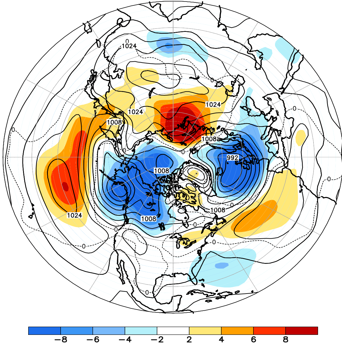
FIGURE E8. Northern Hemisphere mean and anomalous sea level pressure (CDAS/Reanalysis) for NOV 2009. Mean values are denoted by solid contours drawn at an interval of 4 hPa. Anomaly contour interval is 2 hPa with values less (greater) than -2 hPa (2 hPa) indicated by dark (light) shading. Anomalies are calculated as departures from the 1979-95 base period monthly means.
