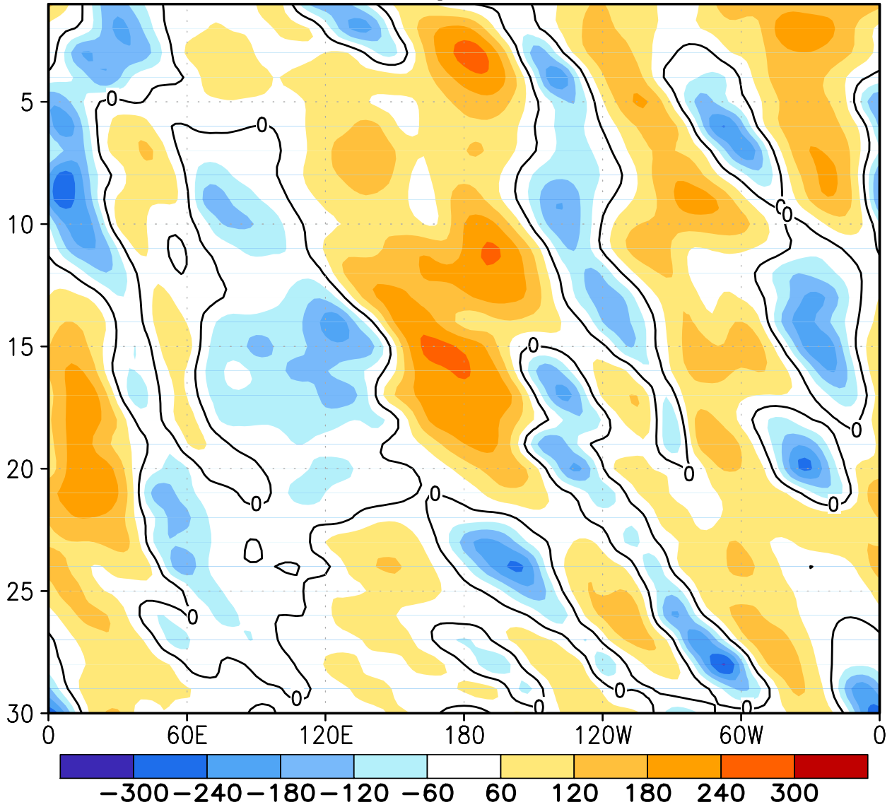
FIGURE E12. Northern Hemisphere: Daily 500-hPa height anomalies for NOV 2009 averaged over the 5° latitude band centered on 40°N. Positive values are indicated by solid contours and dark shading. Negative values are indicated by dashed contours and light shading. Contour interval is 60 m. Anomalies are departures from the 1979-95 base period daily means.
