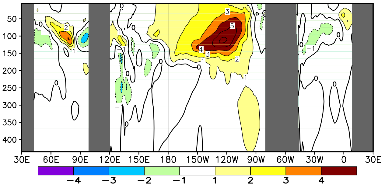
FIGURE T17. Equatorial depth–longitude section of ocean temperature (top) and ocean temperature anomalies (bottom) for NOV 2009. Contour interval is 1°C. Dashed contours in bottom panel indicate negative anomalies. Data are derived from the NCEP’s global ocean data assimilation system version 2 which assimilates oceanic observations into an oceanic GCM (Xue, Y. and Behringer, D.W., 2006: Operational global ocean data assimilation system at NCEP, to be submitted to BAMS). Anomalies are departures from the 1982–2004 base period means.
