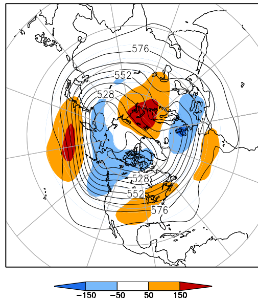
500-hPa Height (dm) & Anomalies (m) (Nov 1–15, 2009)
