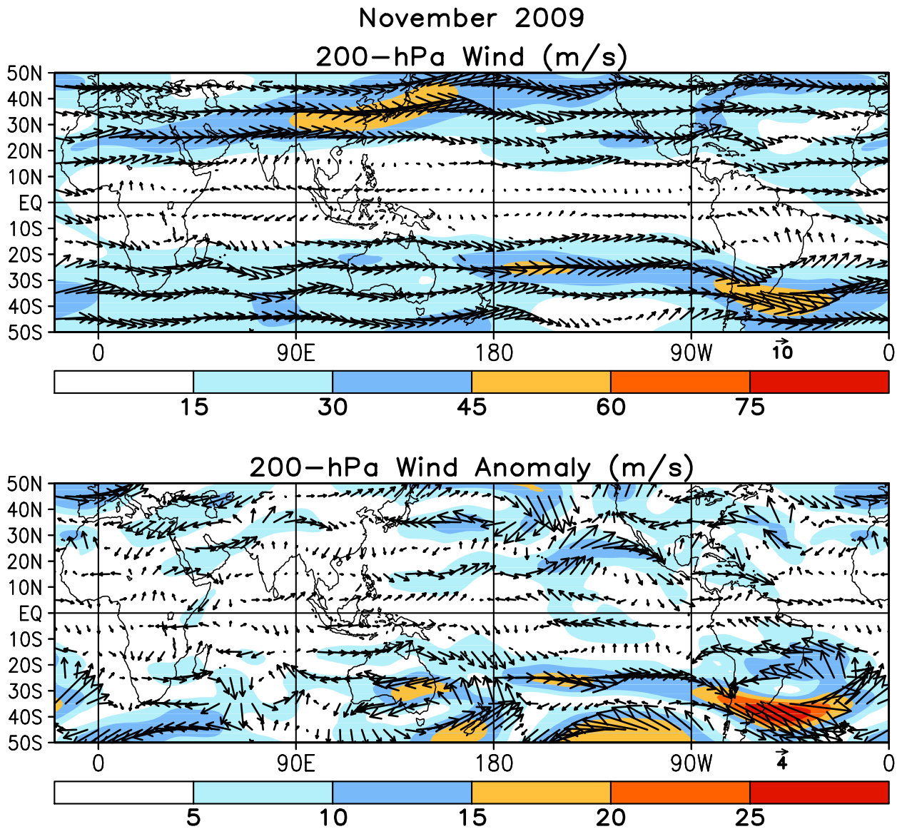
FIGURE T21. Mean (top) and anomalous (bottom) 200-hPa vector wind (CDAS/Reanalysis) for NOV 2009. Contour interval for isotachs is 15 \text{ ms}^{-1} (top) and 5 \text{ ms}^{-1} (bottom). Anomalies are departures from 1979–95 base period monthly means.
