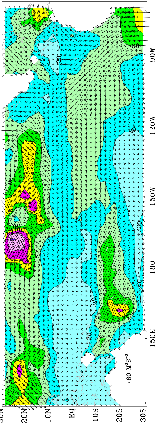
Near-real-time Objective FSU Pseudo-stress Magnitude and Vectors (10m) November 2009
