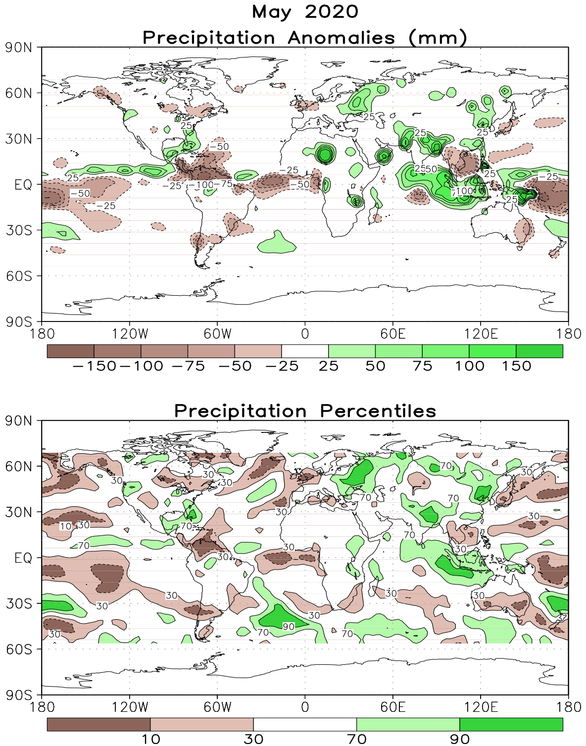
FIGURE E3. Anomalous precipitation (mm, top) and precipitation percentiles based on a Gamma distribution fit to the 1981–2010 base period data (bottom) for MAY 2020. Data are obtained from a merge of raingauge observations and satellite-derived precipitation estimates (Janowiak and Xie 1999, J. Climate , 12, 3335–3342). Contours are drawn at 200, 100, 50, 25, -25, -50, -100, and -200 mm in top panel. Percentiles are not plotted in regions where mean monthly precipitation is <5mm/month.
