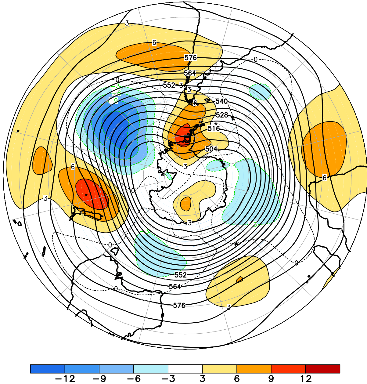
FIGURE E15. Southern Hemisphere mean and anomalous 500-hPa geopotential height (CDAS/Reanalysis) for MAY 2020. Mean heights are denoted by solid contours drawn at an interval of 6 dam. Anomaly contour interval is 3 dam with values less (greater) than -3 dam (3 dam) indicated by dark (light) shading. Anomalies are calculated as departures from the 1981-2010 base period monthly means.
