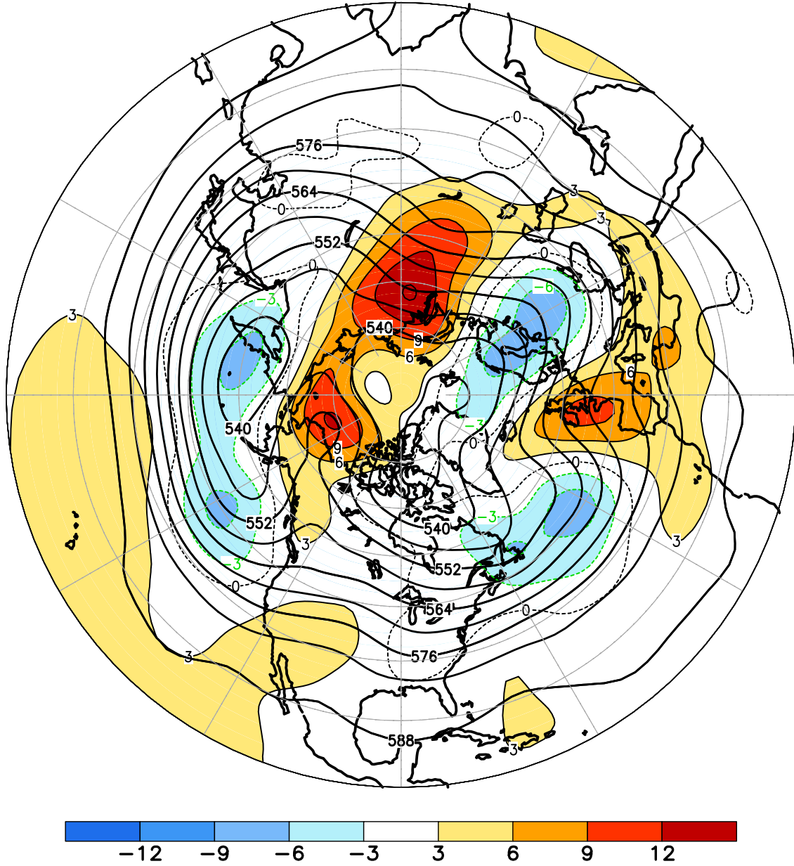
FIGURE E9. Northern Hemisphere mean and anomalous 500-hPa geopotential height (CDAS/Reanalysis) for MAY 2020. Mean heights are denoted by solid contours drawn at an interval of 6 dam. Anomaly contour interval is 3 dam with values less (greater) than -3 dam (3 dam) indicated by dark (light) shading. Anomalies are calculated as departures from the 1981-2010 base period monthly means.
