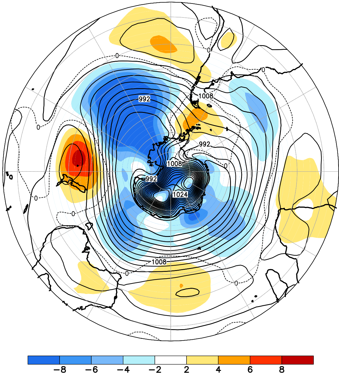
FIGURE E14. Southern Hemisphere mean and anomalous sea level pressure(CDAS/Reanalysis) for MAY 2020. Mean values are denoted by solid contours drawn at an interval of 4 hPa. Anomaly contour interval is 2 hPa with values less (greater) than -2 hPa (2 hPa) indicated by dark (light) shading. Anomalies are calculated as departures from the 1981-2010 base period monthly means.
