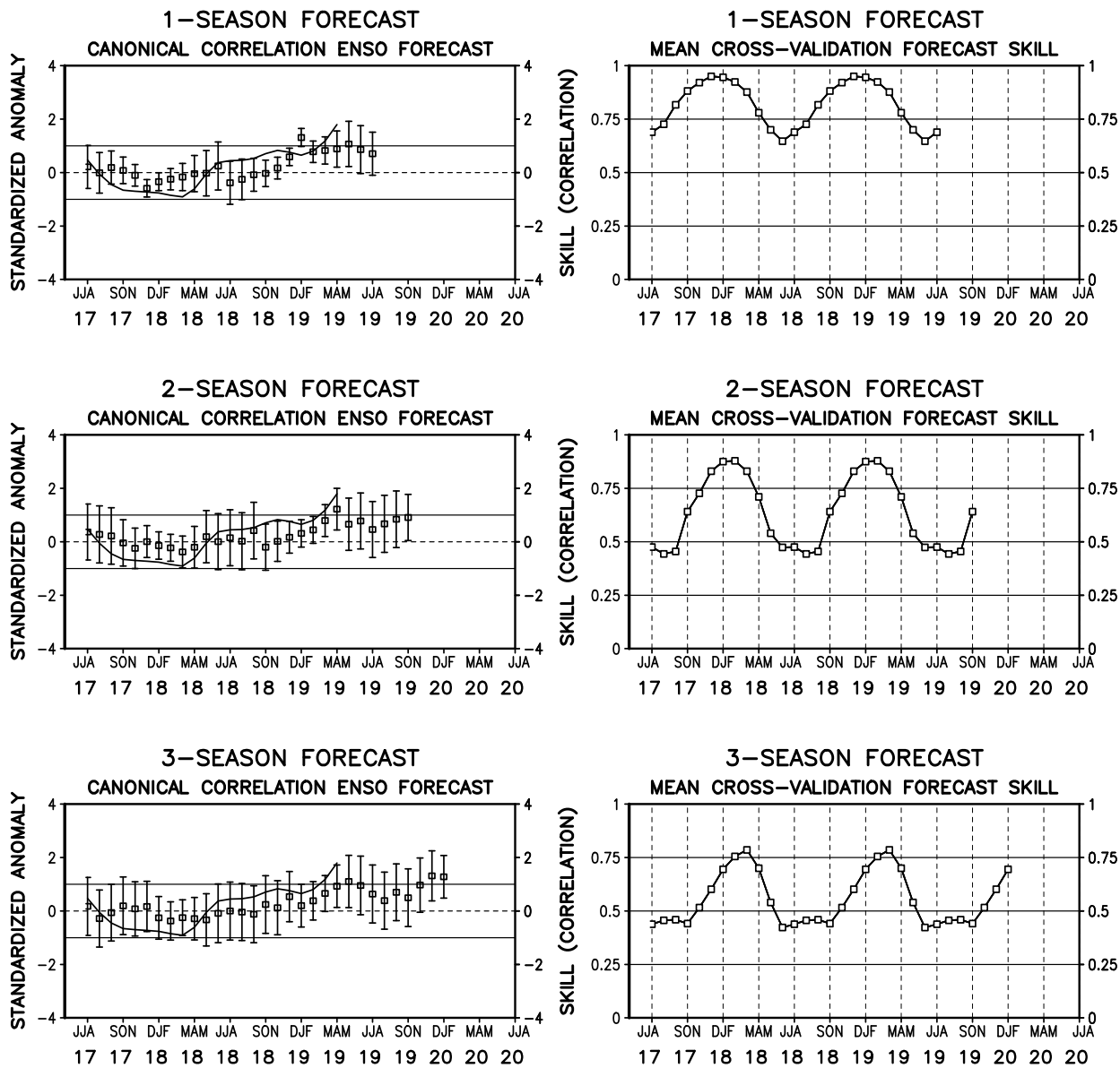
FIGURE F1. Canonical correlation analysis (CCA) sea surface temperature (SST) anomaly prediction for the central Pacific (5°N to 5°S, 120°W to 170°W (Barnston and Ropelewski, 1992, J. Climate , 5 , 1316-1345). The three plots on the left hand side are, from top to bottom, the 1-season, 2-season, and 3-season lead forecasts. The solid line in each forecast represents the observed SST standardized anomaly through the latest month. The small squares at the mid-points of the forecast bars represent the real-time CCA predictions based on the anomalies of quasi-global sea level pressure and on the anomalies of tropical Pacific SST, depth of the 20°C isotherm and sea level height over the prior four seasons. The vertical lines represent the one standard deviation error bars for the predictions based on past performance. The three plots on the right side are skills, corresponding to the predicted and observed SST. The skills are derived from cross-correlation tests from 1956 to present. These skills show a clear annual cycle and are inversely proportional to the length of the error bars depicted in the forecast time series.
