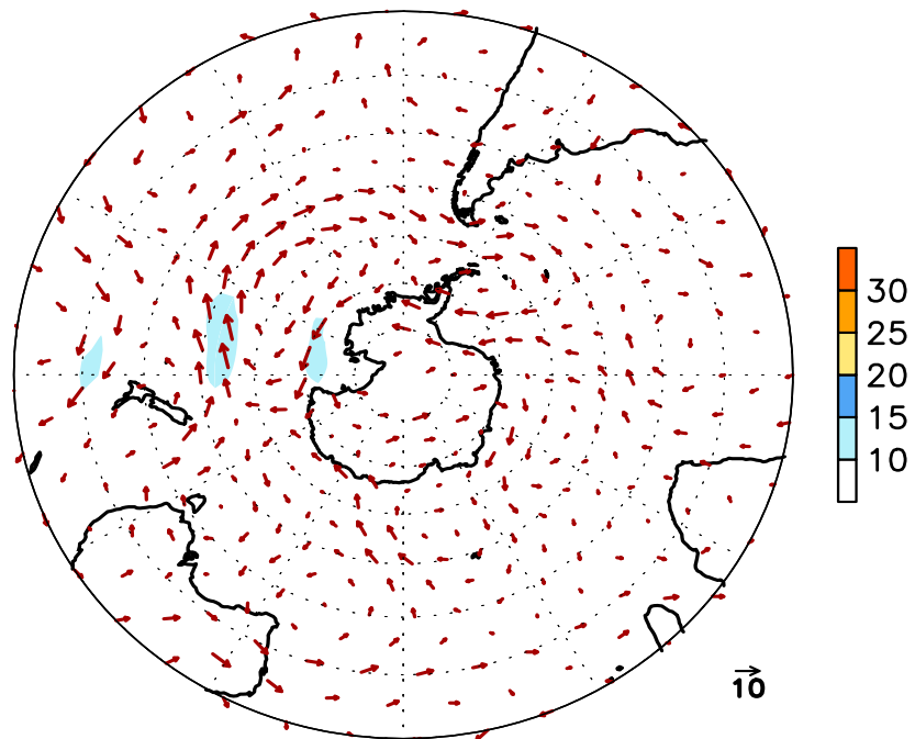
FIGURE E16. Southern Hemisphere mean (left) and anomalous (right) 300-hPa vector wind (CDAS/Reanalysis) for APR 2019. Mean (anomaly) isotach contour interval is 10 (5) \text{ms}^{-1} . Values greater than 30 \text{ms}^{-1} (left) and 10 \text{ms}^{-1} (rights) are shaded. Anomalies are departures from the 1981-2010 base period monthly means.
