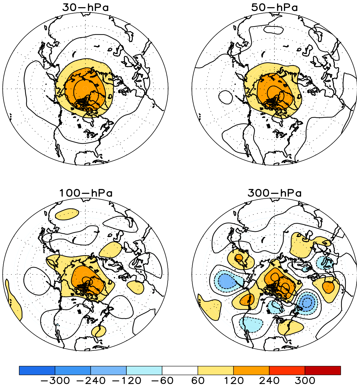
FIGURE S1. Stratospheric height anomalies (m) at selected levels for APR 2019. Positive values are indicated by solid contours and dark shading. Negative values are indicated by dashed contours and light shading. Contour interval is 60 m. Anomalies are calculated from the 1981-2010 base period means. Winter Hemisphere is shown.
