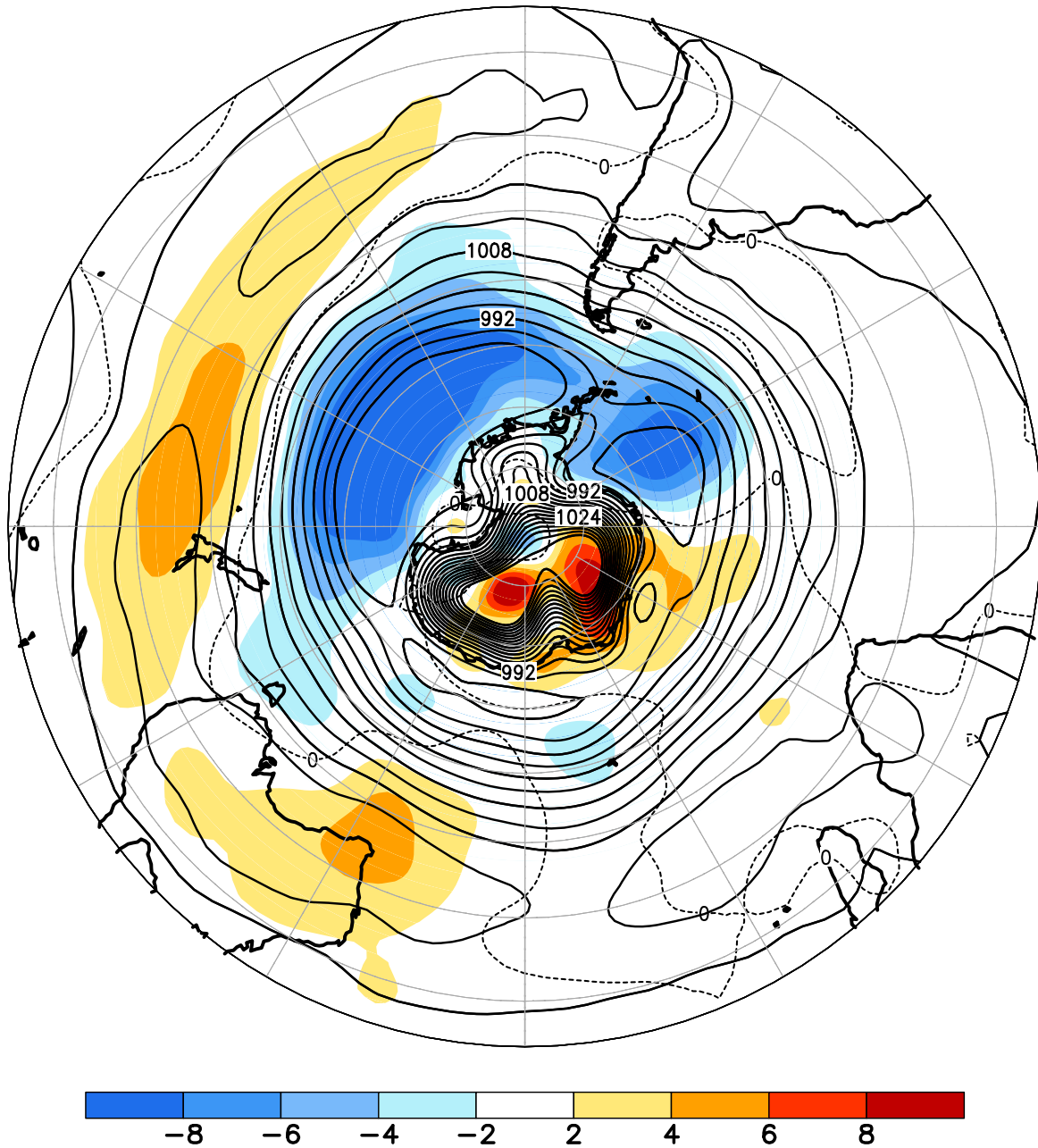
FIGURE E14. Southern Hemisphere mean and anomalous sea level pressure(CDAS/Reanalysis) for APR 2019. Mean values are denoted by solid contours drawn at an interval of 4 hPa. Anomaly contour interval is 2 hPa with values less (greater) than -2 hPa (2 hPa) indicated by dark (light) shading. Anomalies are calculated as departures from the 1981-2010 base period monthly means.
