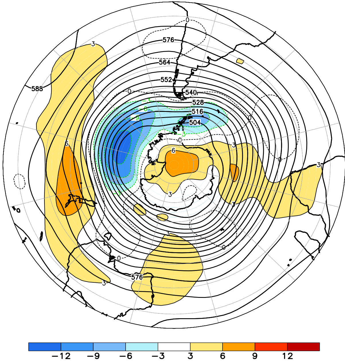
FIGURE E15. Southern Hemisphere mean and anomalous 500-hPa geopotential height (CDAS/Reanalysis) for APR 2019. Mean heights are denoted by solid contours drawn at an interval of 6 dam. Anomaly contour interval is 3 dam with values less (greater) than -3 dam (3 dam) indicated by dark (light) shading. Anomalies are calculated as departures from the 1981-2010 base period monthly means.
