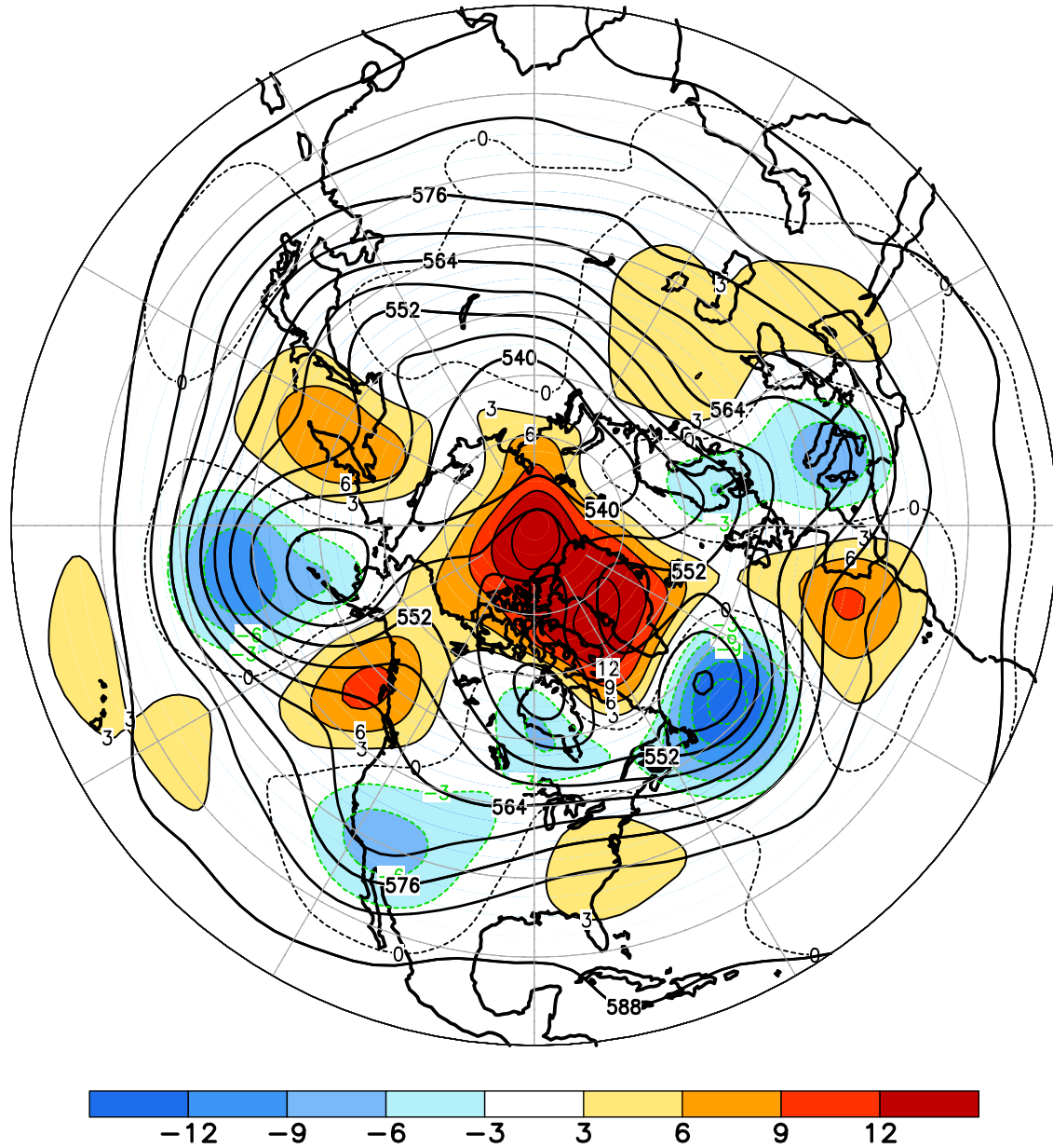
FIGURE E9. Northern Hemisphere mean and anomalous 500-hPa geopotential height (CDAS/Reanalysis) for APR 2019. Mean heights are denoted by solid contours drawn at an interval of 6 dam. Anomaly contour interval is 3 dam with values less (greater) than -3 dam (3 dam) indicated by dark (light) shading. Anomalies are calculated as departures from the 1981-2010 base period monthly means.
