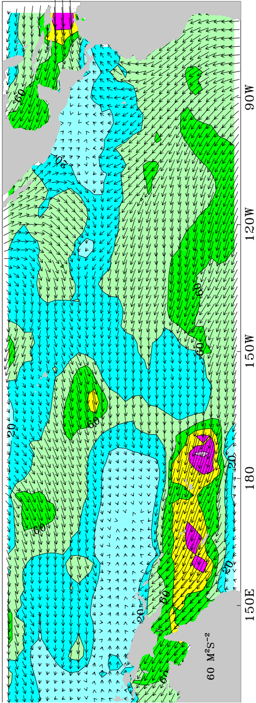
Near realtime Objective FSU Pseudostress Magnitude and Vectors (10m) May 2019
