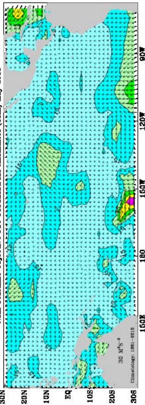
Near realtime Objective FSU Pseudostress Anomalies (10m) May 2016
