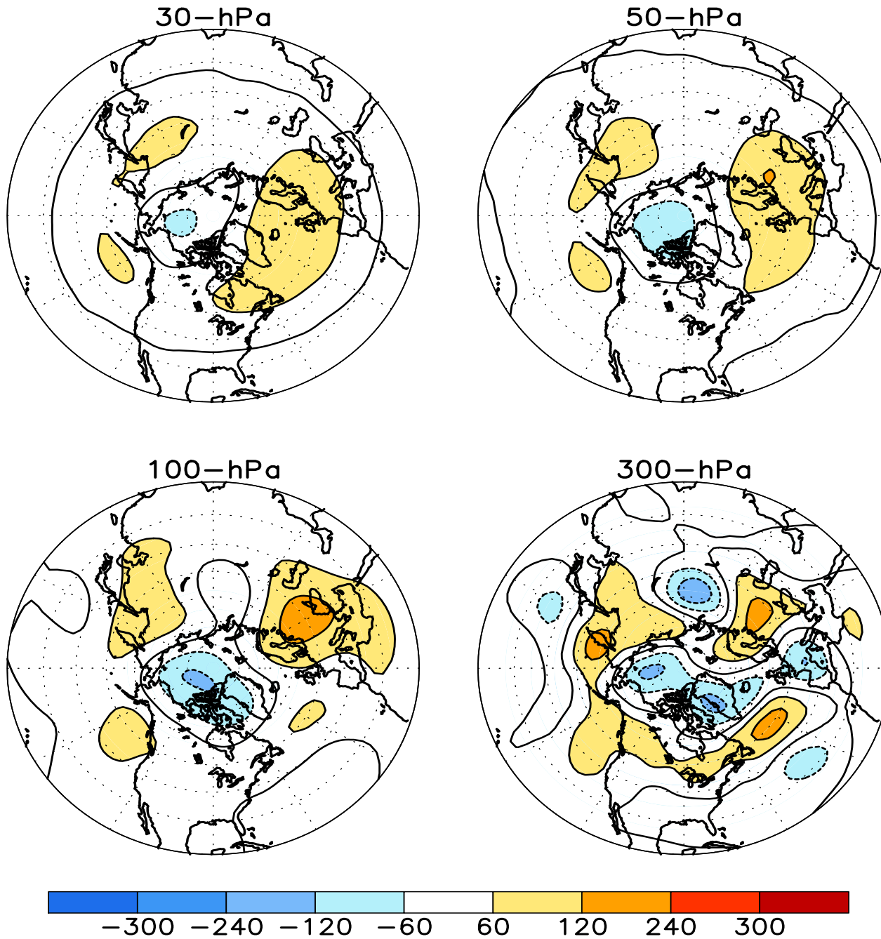
FIGURE S1. Stratospheric height anomalies (m) at selected levels for MAY 2013. Positive values are indicated by solid contours and dark shading. Negative values are indicated by dashed contours and light shading. Contour interval is 60 m. Anomalies are calculated from the 1981-2010 base period means. Winter Hemisphere is shown.
