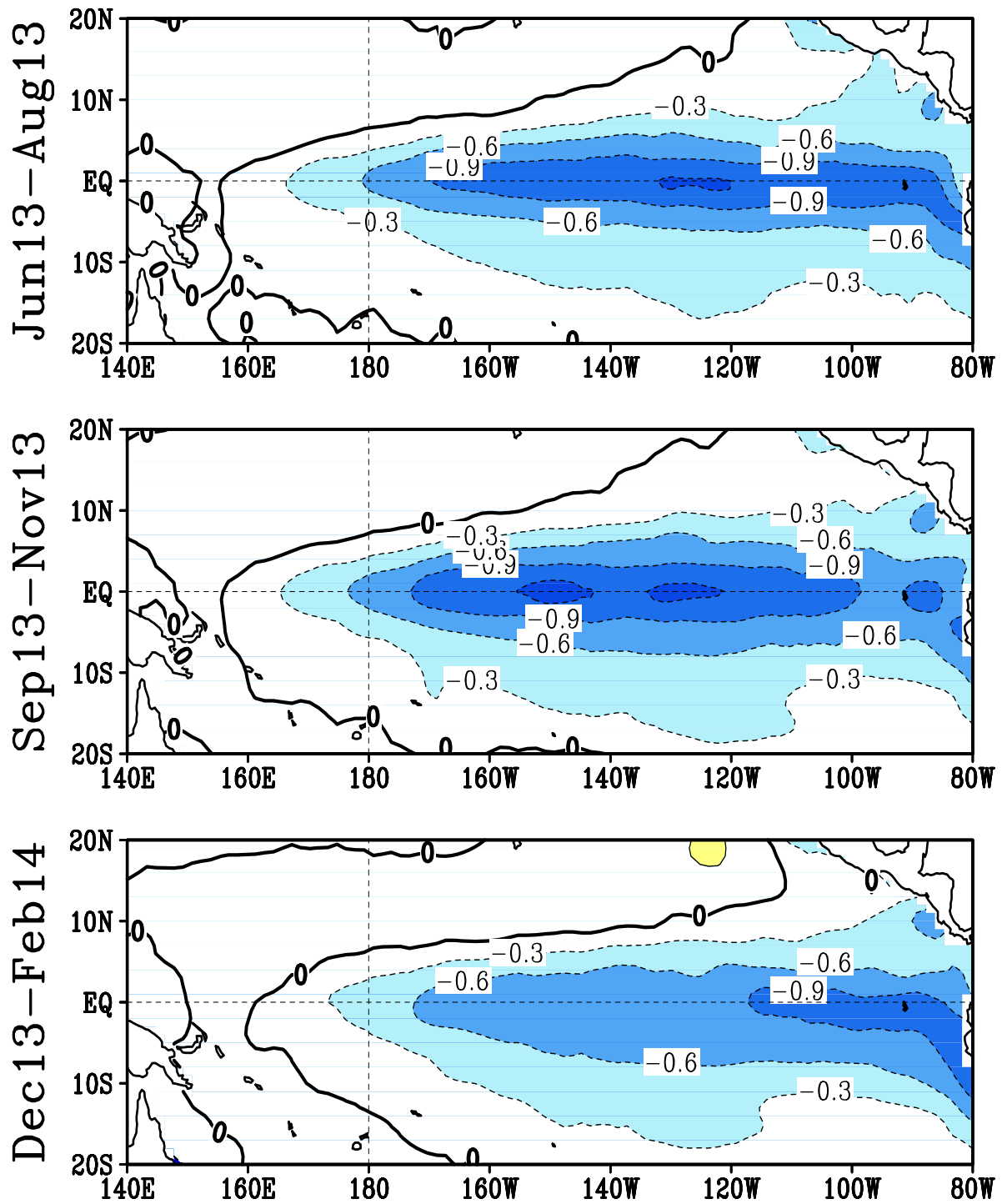
FIGURE F5. Predicted 3-month average sea surface temperature anomalies from the NCEP/CPC Markov model (Xue et al. 2000, J. Climate , 13 , 849-871). The forecast is initiated in MAY 2013 . Contour interval is 0.3C and negative anomalies are indicated by dashed contours. Anomalies are calculated relative to the 1971-2000 climatology.
