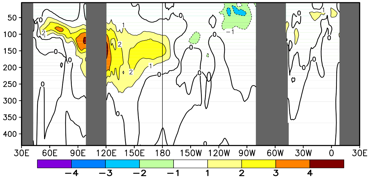
FIGURE T17. Equatorial depth–longitude section of ocean temperature (top) and ocean temperature anomalies (bottom) for MAY 2013. Contour interval is 1°C. Dashed contours in bottom panel indicate negative anomalies. Data are derived from the NCEP’s global ocean data assimilation system version 2 which assimilates oceanic observations into an oceanic GCM (Xue, Y. and Behringer, D.W., 2006: Operational global ocean data assimilation system at NCEP, to be submitted to BAMS). Anomalies are departures from the 1981–2010 base period means.
