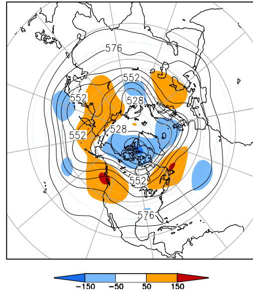
500-hPa Height (dm) & Anomalies (m) (May 1–15, 2013)
