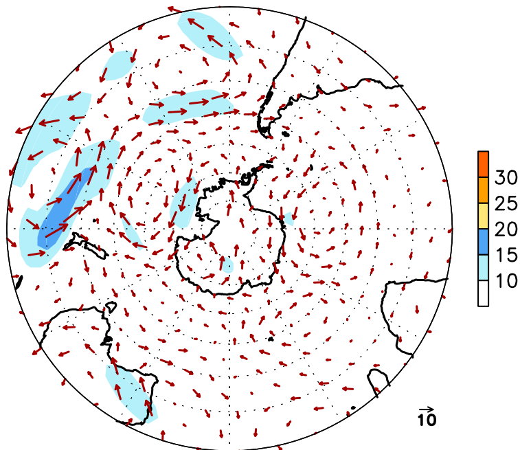
FIGURE E16. Southern Hemisphere mean (left) and anomalous (right) 300-hPa vector wind (CDAS/Reanalysis) for MAY 2013. Mean (anomaly) isotach contour interval is 10 (5) \text{ms}^{-1} . Values greater than 30 \text{ms}^{-1} (left) and 10 \text{ms}^{-1} (rights) are shaded. Anomalies are departures from the 1981-2010 base period monthly means.
