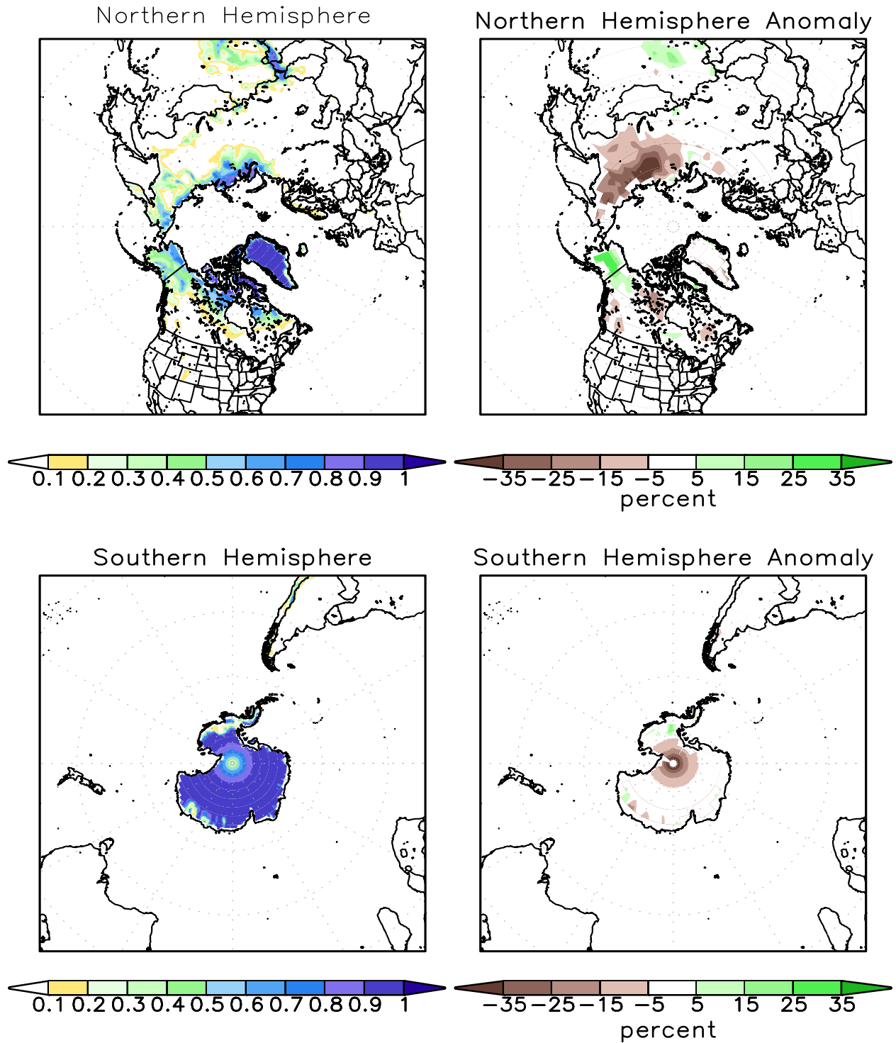
FIGURE A2.2. SSM/I derived snow cover frequency (%) (left) and snow cover anomaly (%) (right) for the month of MAY 2013 based on 1987 - 2010 base period for the Northern Hemisphere (top) and Southern Hemisphere (bottom). It is generated using the algorithm described by Ferraro et. al, 1996, Bull. Amer. Meteor. Soc., vol 77, 891-905.
