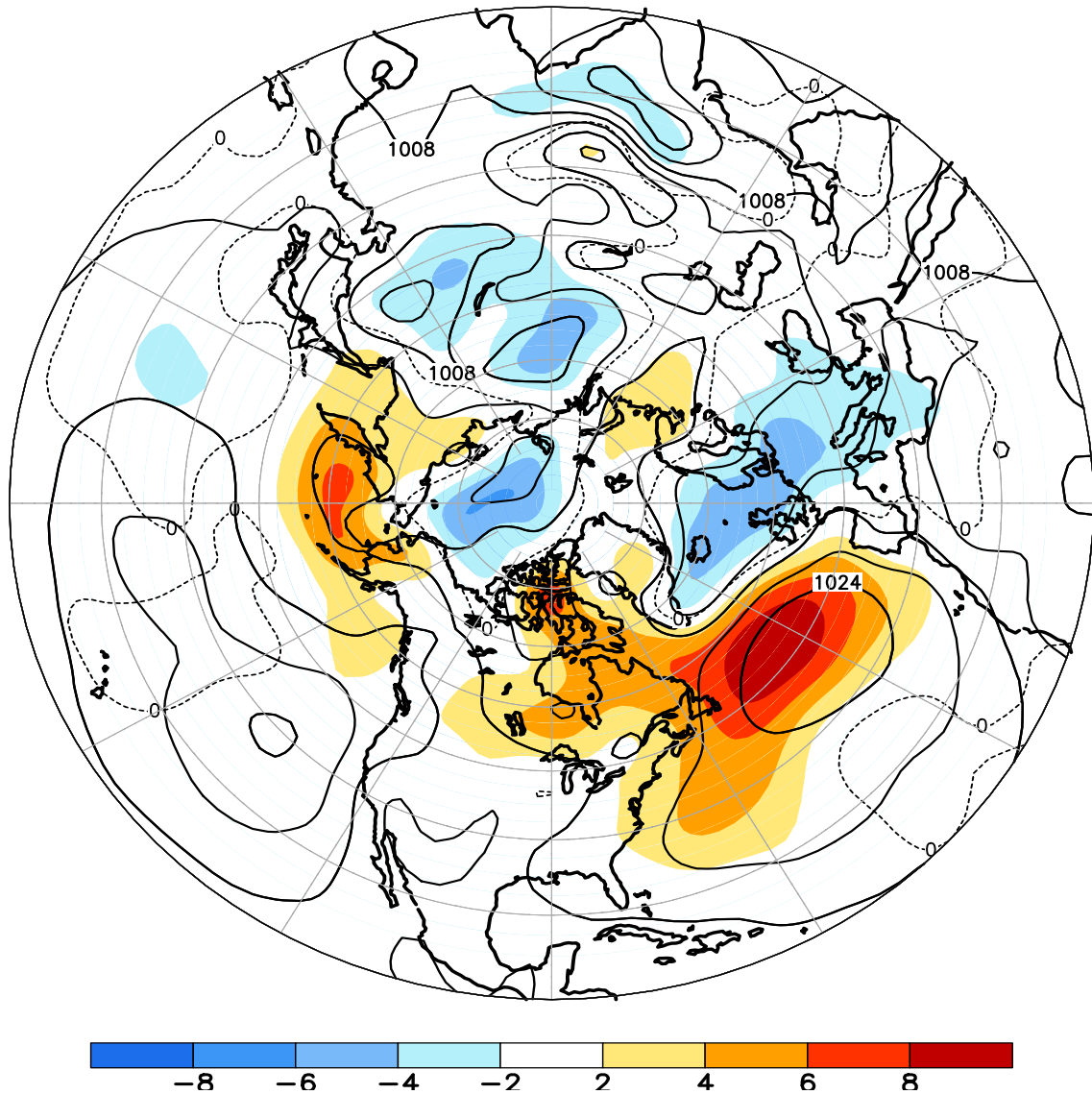
FIGURE E8. Northern Hemisphere mean and anomalous sea level pressure (CDAS/Reanalysis) for MAY 2013. Mean values are denoted by solid contours drawn at an interval of 4 hPa. Anomaly contour interval is 2 hPa with values less (greater) than -2 hPa (2 hPa) indicated by dark (light) shading. Anomalies are calculated as departures from the 1981-2010 base period monthly means.
