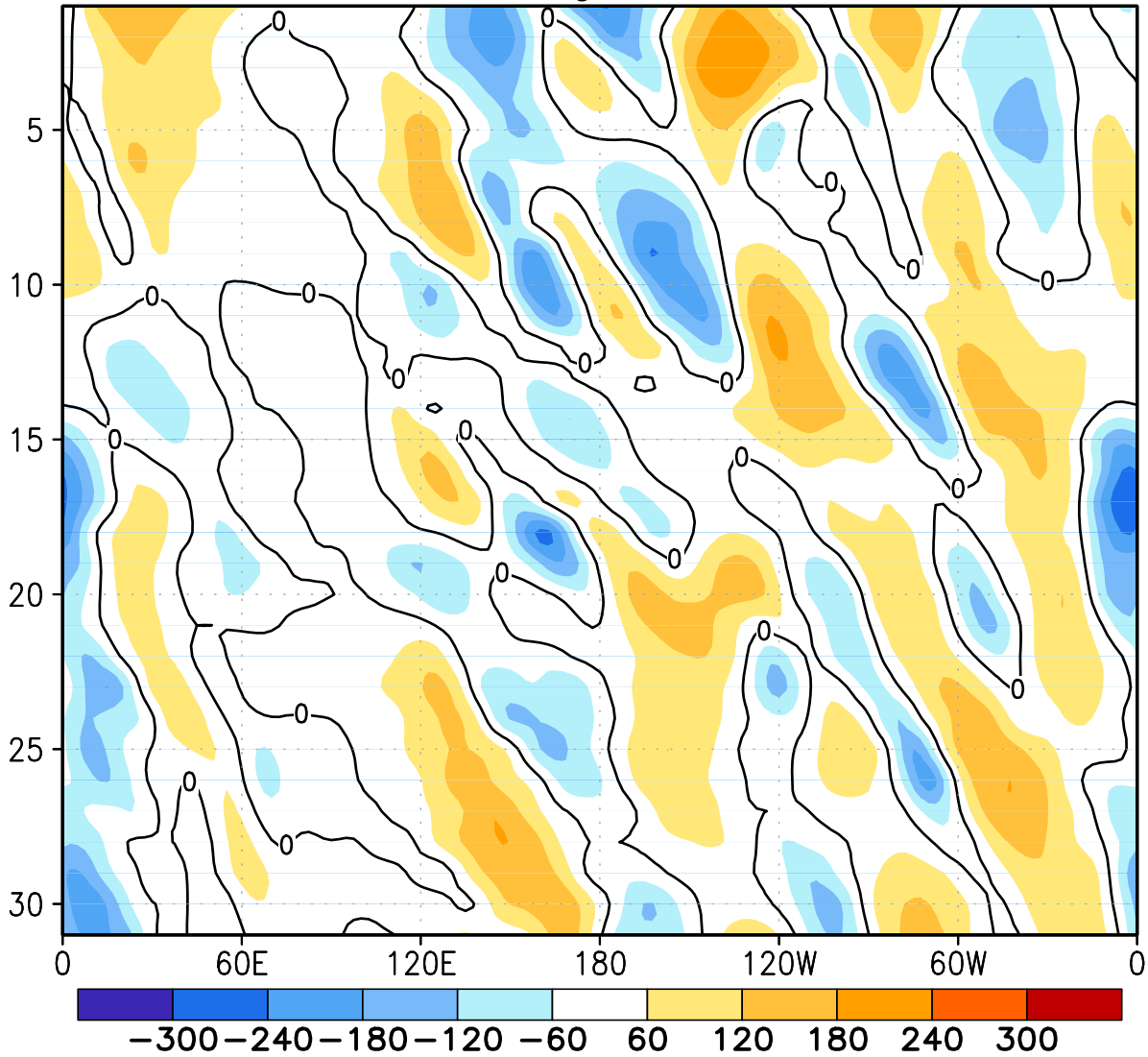
FIGURE E12. Northern Hemisphere: Daily 500-hPa height anomalies for MAY 2013 averaged over the 5° latitude band centered on 40°N. Positive values are indicated by solid contours and dark shading. Negative values are indicated by dashed contours and light shading. Contour interval is 60 m. Anomalies are departures from the 1981-2010 base period daily means.
