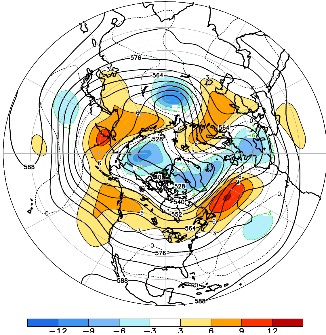
FIGURE E9. Northern Hemisphere mean and anomalous 500-hPa geopotential height (CDAS/Reanalysis) for MAY 2013. Mean heights are denoted by solid contours drawn at an interval of 6 dam. Anomaly contour interval is 3 dam with values less (greater) than -3 dam (3 dam) indicated by dark (light) shading. Anomalies are calculated as departures from the 1981-2010 base period monthly means.
