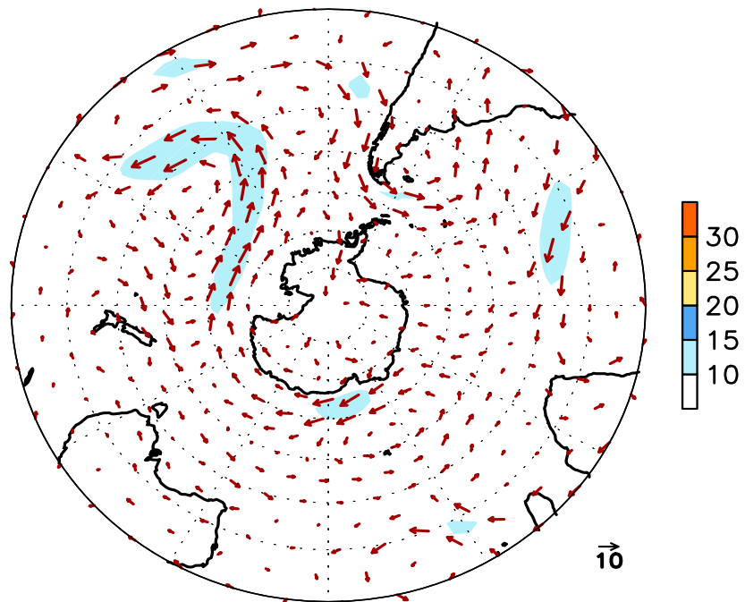
FIGURE E16. Southern Hemisphere mean (left) and anomalous (right) 300-hPa vector wind (CDAS/Reanalysis) for MAR 2020. Mean (anomaly) isotach contour interval is 10 (5) \text{ms}^{-1} . Values greater than 30 \text{ms}^{-1} (left) and 10 \text{ms}^{-1} (rights) are shaded. Anomalies are departures from the 1981-2010 base period monthly means.
