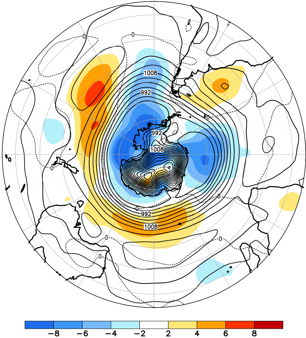
FIGURE E14. Southern Hemisphere mean and anomalous sea level pressure(CDAS/Reanalysis) for MAR 2020. Mean values are denoted by solid contours drawn at an interval of 4 hPa. Anomaly contour interval is 2 hPa with values less (greater) than -2 hPa (2 hPa) indicated by dark (light) shading. Anomalies are calculated as departures from the 1981-2010 base period monthly means.
