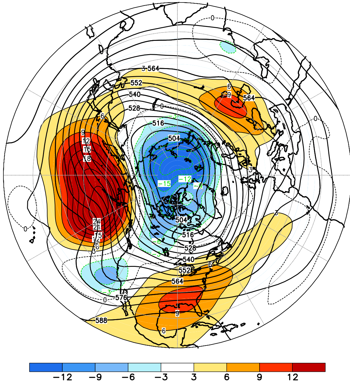
FIGURE E9. Northern Hemisphere mean and anomalous 500-hPa geopotential height (CDAS/Reanalysis) for MAR 2020. Mean heights are denoted by solid contours drawn at an interval of 6 dam. Anomaly contour interval is 3 dam with values less (greater) than -3 dam (3 dam) indicated by dark (light) shading. Anomalies are calculated as departures from the 1981-2010 base period monthly means.
