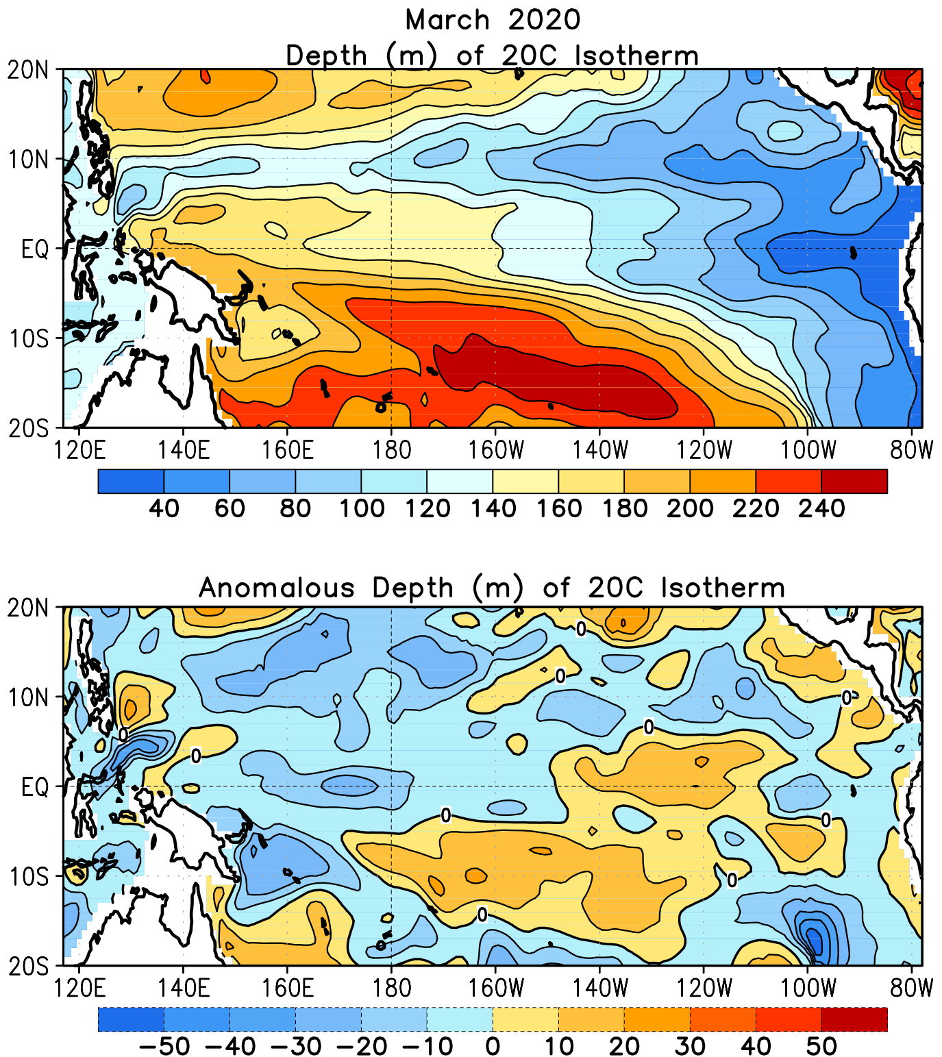
FIGURE T16. Mean (top) and anomalous (bottom) depth of the 20°C isotherm for MAR 2020. Contour interval is 40 m (top) and 10 m (bottom). Dashed contours in bottom panel indicate negative anomalies. Data are derived from the NCEP’s global ocean data assimilation system version 2 which assimilates oceanic observations into an oceanic GCM (Xue, Y. and Behringer, D.W., 2006: Operational global ocean data assimilation system at NCEP, to be submitted to BAMS). Anomalies are departures from the 1981–2010 base period means.
