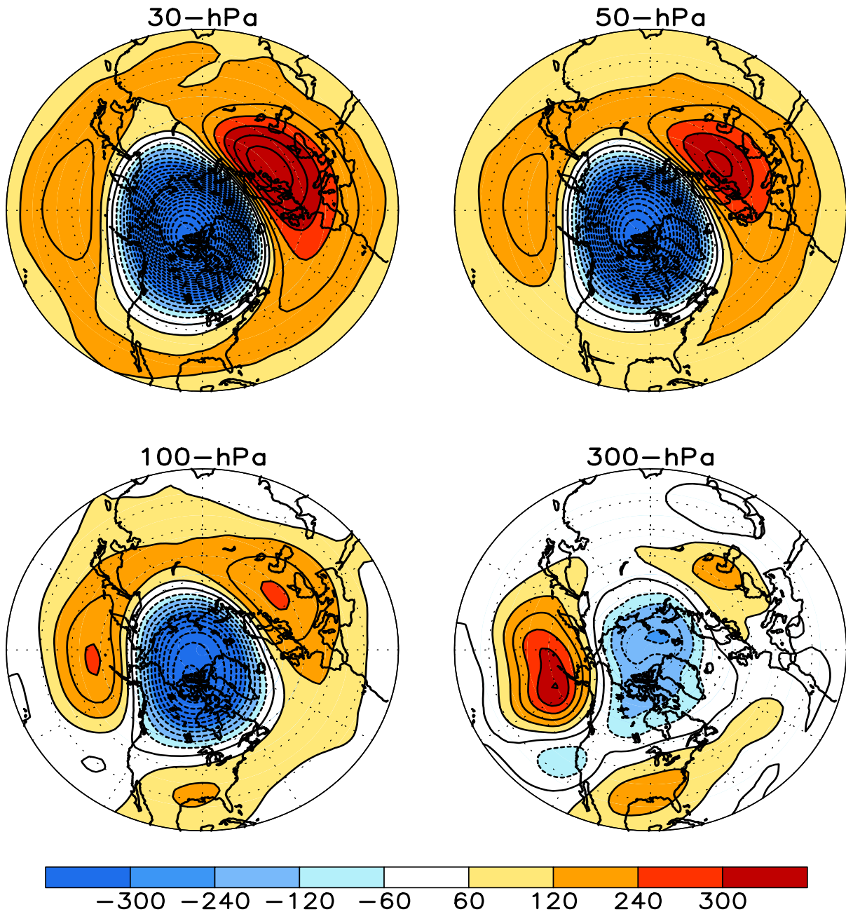
FIGURE S1. Stratospheric height anomalies (m) at selected levels for MAR 2020. Positive values are indicated by solid contours and dark shading. Negative values are indicated by dashed contours and light shading. Contour interval is 60 m. Anomalies are calculated from the 1981-2010 base period means. Winter Hemisphere is shown.
