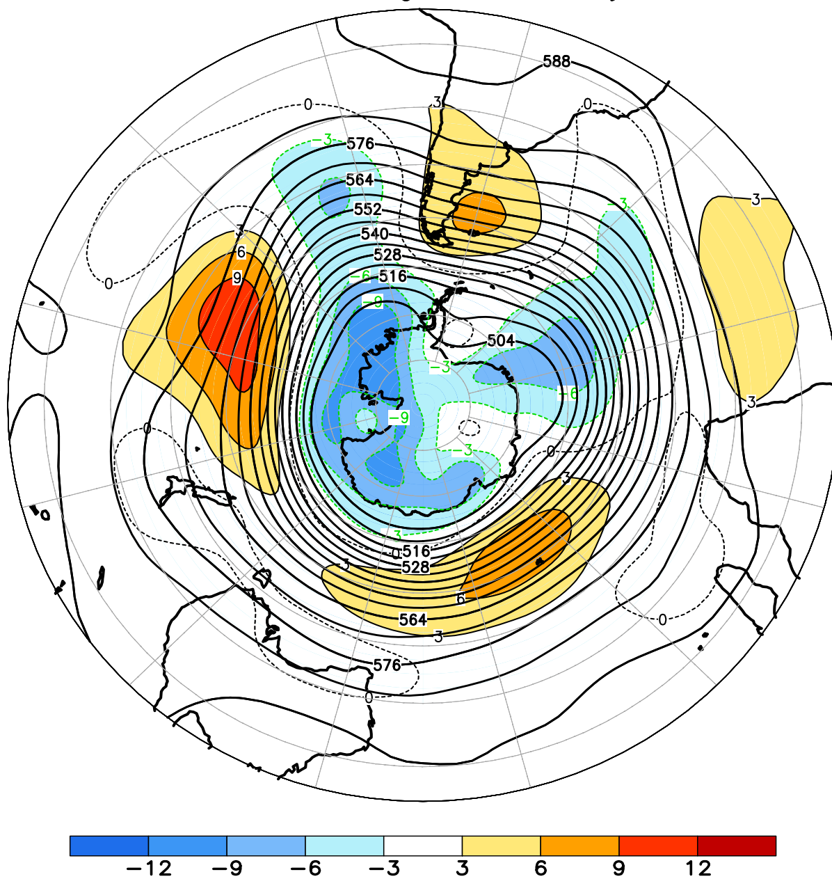
FIGURE E15. Southern Hemisphere mean and anomalous 500-hPa geopotential height (CDAS/Reanalysis) for MAR 2020. Mean heights are denoted by solid contours drawn at an interval of 6 dam. Anomaly contour interval is 3 dam with values less (greater) than -3 dam (3 dam) indicated by dark (light) shading. Anomalies are calculated as departures from the 1981-2010 base period monthly means.
