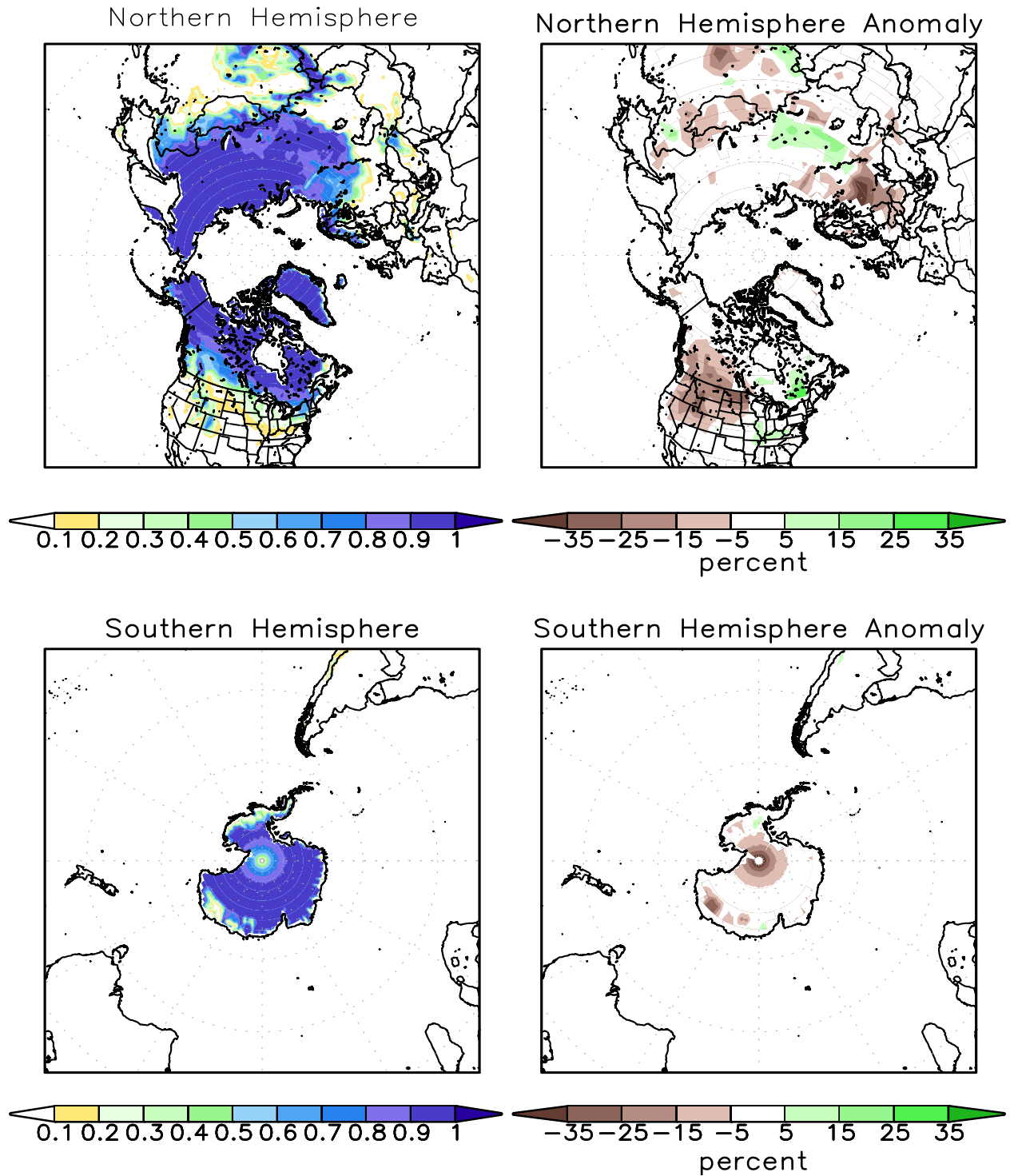
FIGURE A2.2. SSM/I derived snow cover frequency (%) (left) and snow cover anomaly (%) (right) for the month of MAR 2015 based on 1987 - 2010 base period for the Northern Hemisphere (top) and Southern Hemisphere (bottom). It is generated using the algorithm described by Ferraro et. al, 1996, Bull. Amer. Meteor. Soc., vol 77, 891-905.
