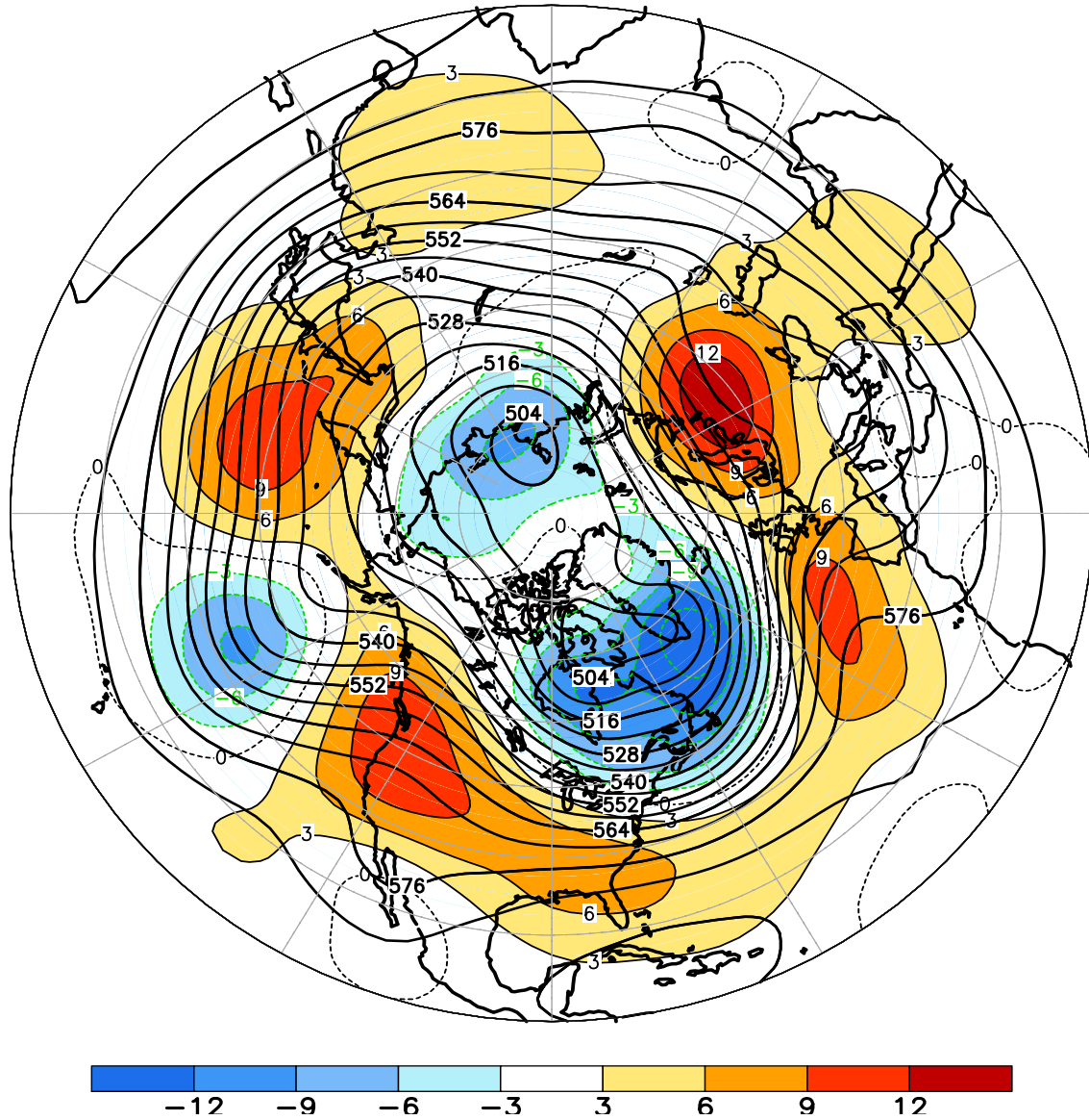
FIGURE E9. Northern Hemisphere mean and anomalous 500-hPa geopotential height (CDAS/Reanalysis) for MAR 2015. Mean heights are denoted by solid contours drawn at an interval of 6 dam. Anomaly contour interval is 3 dam with values less (greater) than -3 dam (3 dam) indicated by dark (light) shading. Anomalies are calculated as departures from the 1981-2010 base period monthly means.
