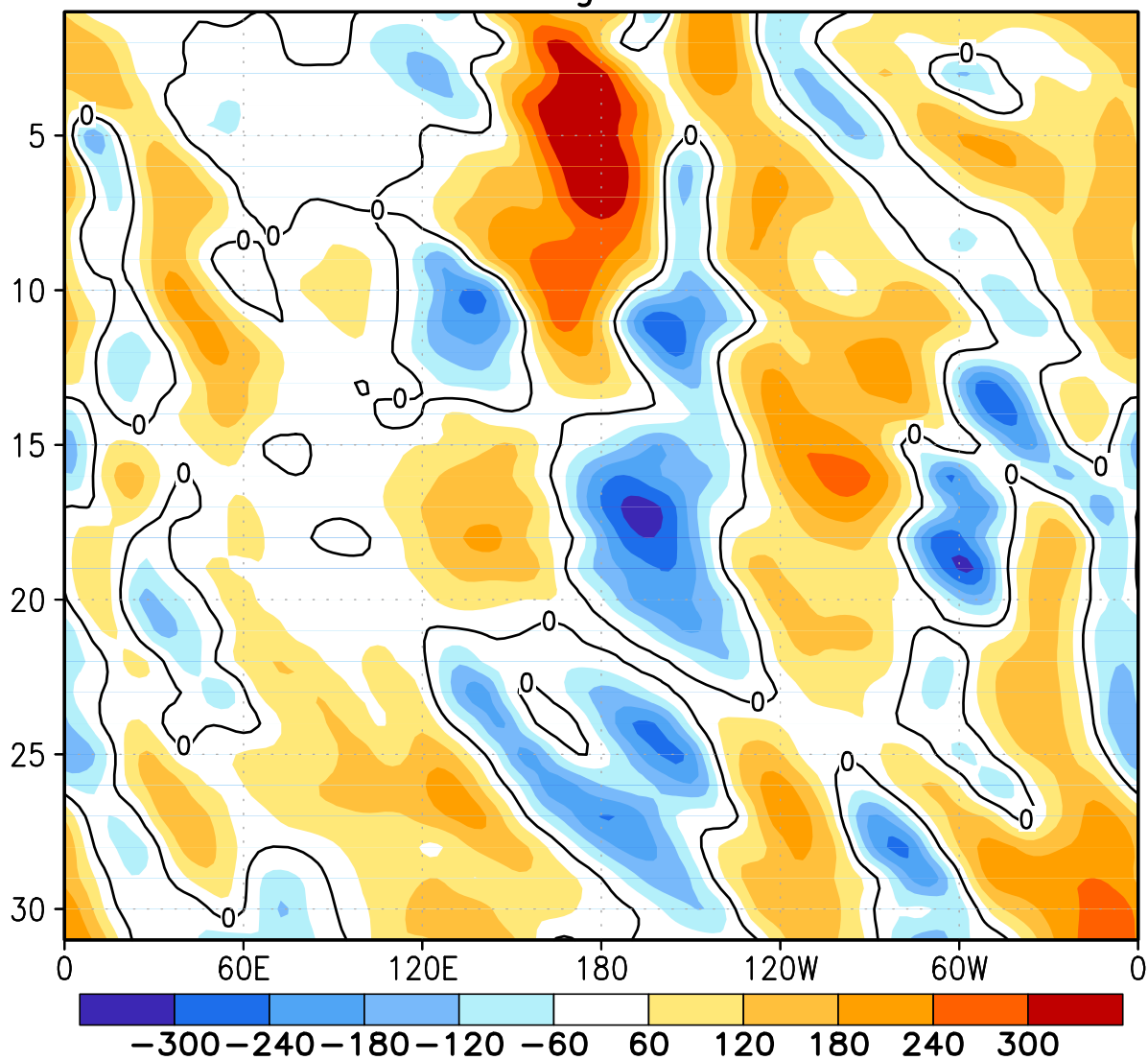
FIGURE E12. Northern Hemisphere: Daily 500-hPa height anomalies for MAR 2015 averaged over the 5° latitude band centered on 40°N. Positive values are indicated by solid contours and dark shading. Negative values are indicated by dashed contours and light shading. Contour interval is 60 m. Anomalies are departures from the 1981-2010 base period daily means.
