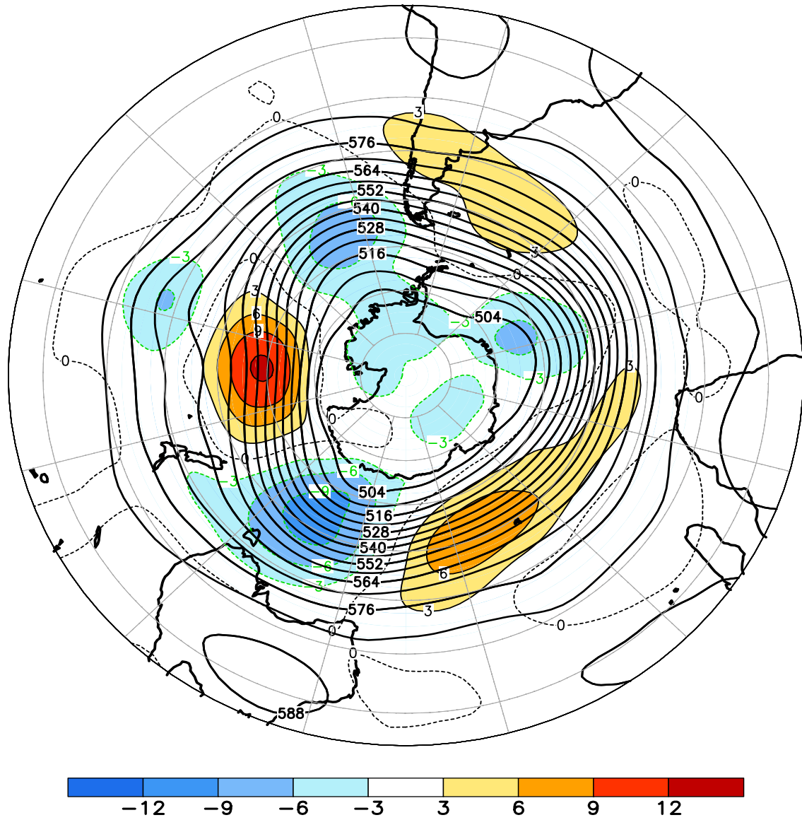
FIGURE E15. Southern Hemisphere mean and anomalous 500-hPa geopotential height (CDAS/Reanalysis) for MAR 2015. Mean heights are denoted by solid contours drawn at an interval of 6 dam. Anomaly contour interval is 3 dam with values less (greater) than -3 dam (3 dam) indicated by dark (light) shading. Anomalies are calculated as departures from the 1981-2010 base period monthly means.
