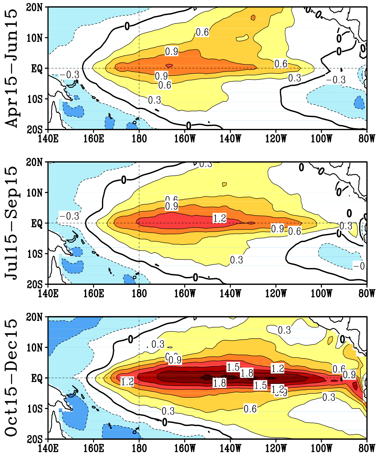
FIGURE F5. Predicted 3-month average sea surface temperature anomalies from the NCEP/CPC Markov model (Xue et al. 2000, J. Climate , 13 , 849-871). The forecast is initiated in MAR 2015. Contour interval is 0.3C and negative anomalies are indicated by dashed contours. Anomalies are calculated relative to the 1971-2000 climatology.
