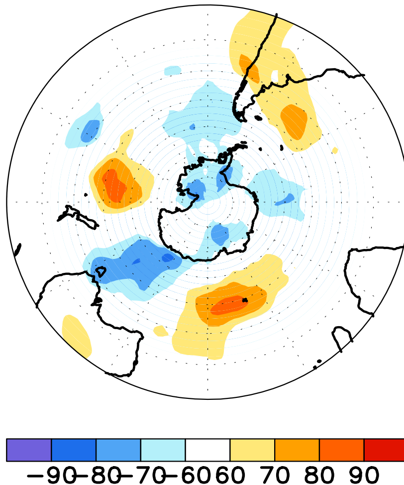
FIGURE E17. Southern Hemisphere percentage of days during MAR 2015 in which 500-hPa height anomalies greater than 15 m (red) and less than -15 m (blue) were observed. Values greater than 70% are shaded and contour interval
