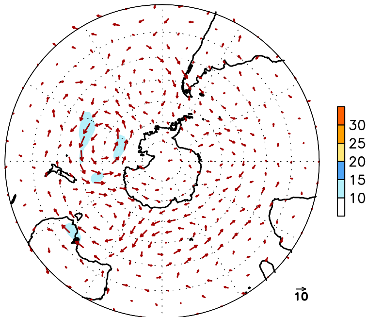
FIGURE E16. Southern Hemisphere mean (left) and anomalous (right) 300-hPa vector wind (CDAS/Reanalysis) for MAR 2015. Mean (anomaly) isotach contour interval is 10 (5) \text{ms}^{-1} . Values greater than 30 \text{ms}^{-1} (left) and 10 \text{ms}^{-1} (rights) are shaded. Anomalies are departures from the 1981-2010 base period monthly means.
