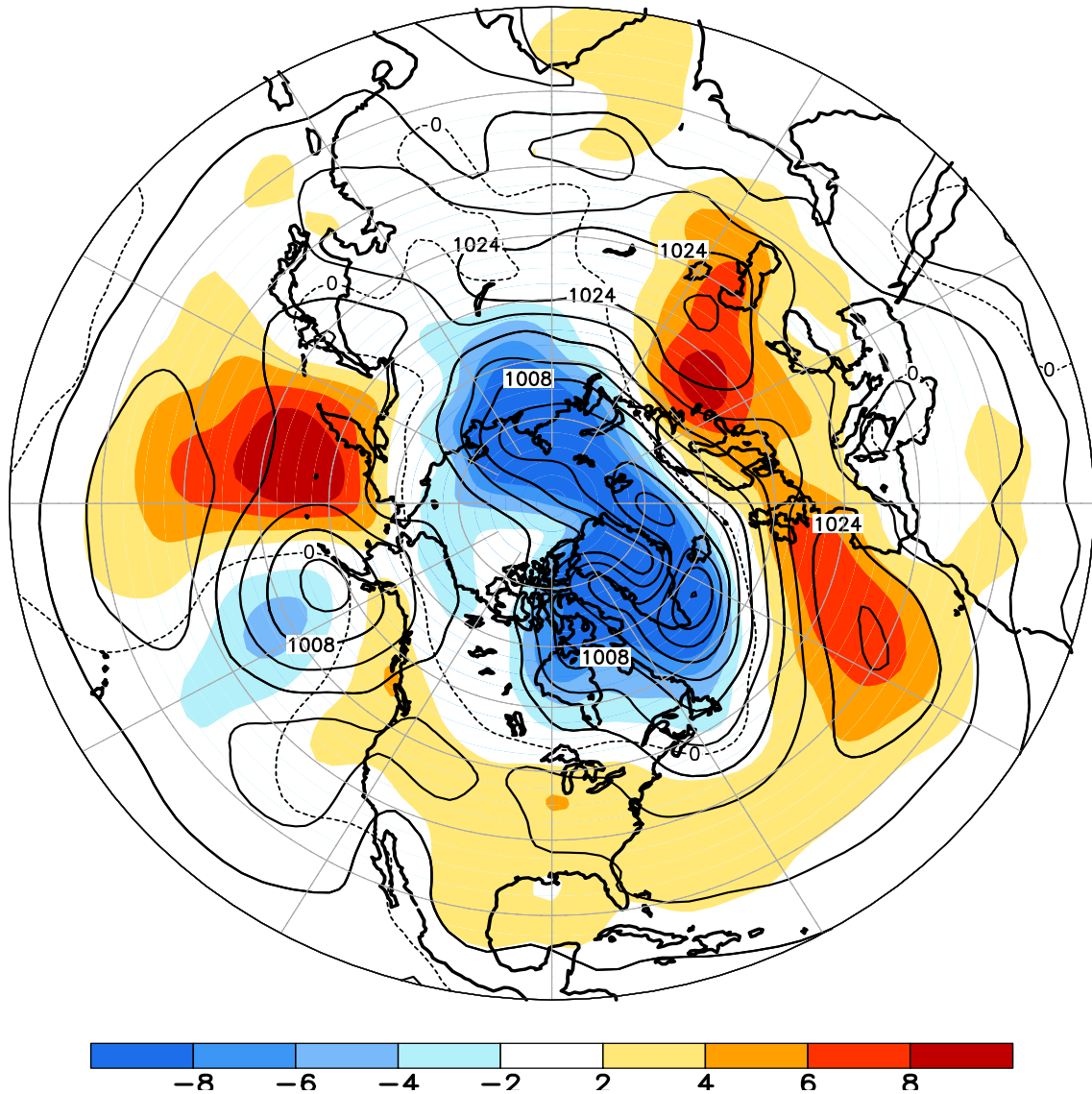
FIGURE E8. Northern Hemisphere mean and anomalous sea level pressure (CDAS/Reanalysis) for MAR 2015. Mean values are denoted by solid contours drawn at an interval of 4 hPa. Anomaly contour interval is 2 hPa with values less (greater) than -2 hPa (2 hPa) indicated by dark (light) shading. Anomalies are calculated as departures from the 1981-2010 base period monthly means.
