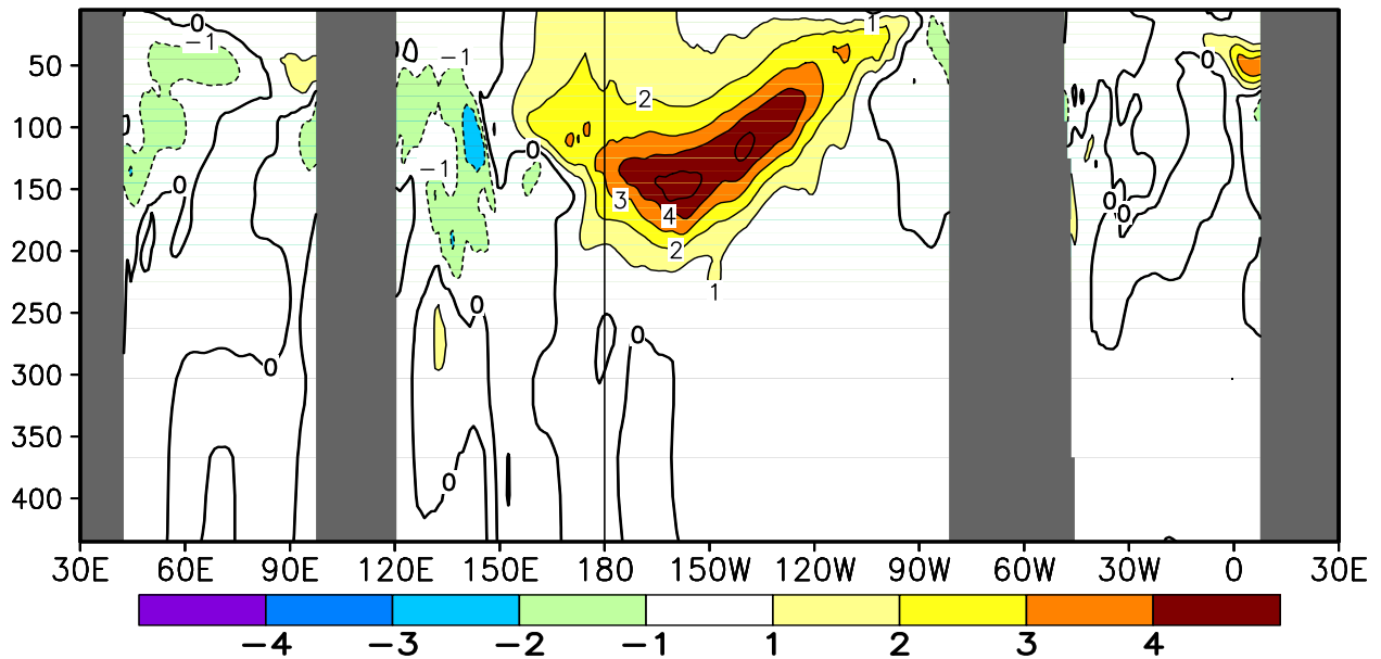
FIGURE T17. Equatorial depth–longitude section of ocean temperature (top) and ocean temperature anomalies (bottom) for MAR 2015. Contour interval is 1°C. Dashed contours in bottom panel indicate negative anomalies. Data are derived from the NCEP’s global ocean data assimilation system version 2 which assimilates oceanic observations into an oceanic GCM (Xue, Y. and Behringer, D.W., 2006: Operational global ocean data assimilation system at NCEP, to be submitted to BAMS). Anomalies are departures from the 1981–2010 base period means.
