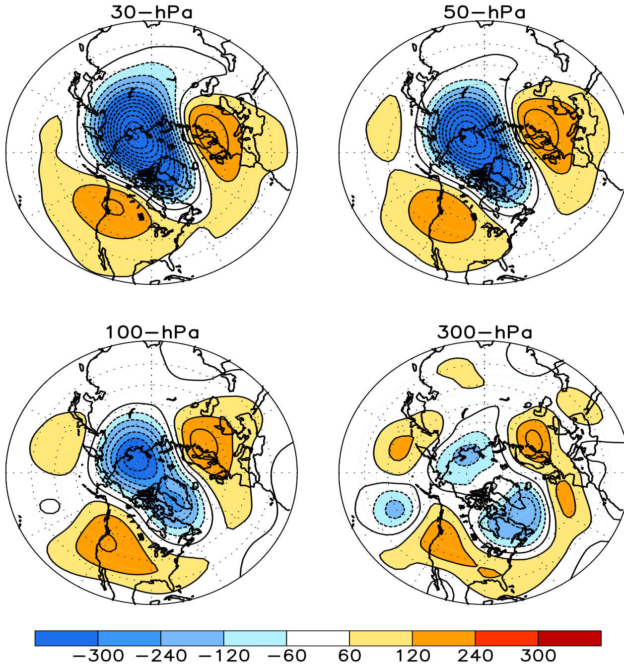
FIGURE S1. Stratospheric height anomalies (m) at selected levels for MAR 2015. Positive values are indicated by solid contours and dark shading. Negative values are indicated by dashed contours and light shading. Contour interval is 60 m. Anomalies are calculated from the 1981-2010 base period means. Winter Hemisphere is shown.
