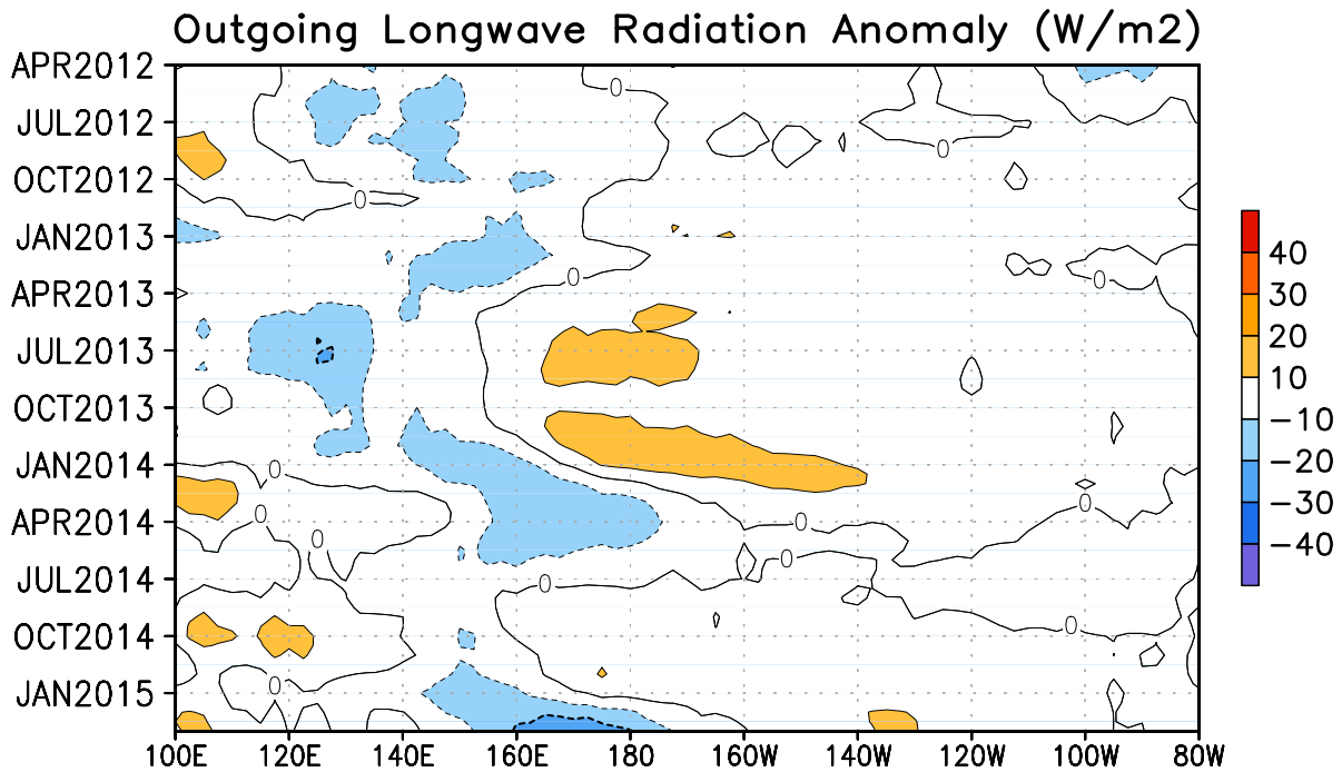
FIGURE T8. Time-longitude section of mean (top) and anomalous (bottom) outgoing longwave radiation (OLR) averaged between 5N-5S. Contour interval is 10 \text{ Wm}^{-2} . Dashed contours in bottom panel indicate negative OLR anomalies. Anomalies are departures from the 1981-2010 base period monthly means. The data are smoothed temporally using a 3-month running average.
