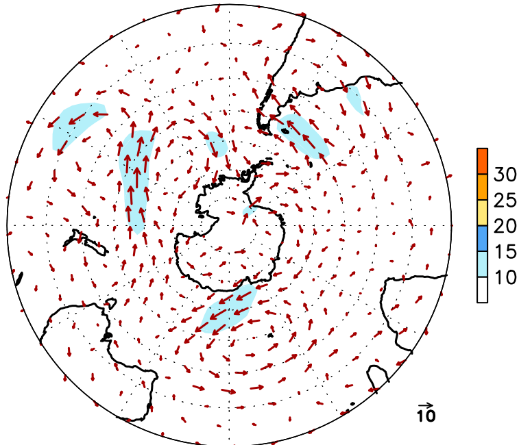
FIGURE E16. Southern Hemisphere mean (left) and anomalous (right) 300-hPa vector wind (CDAS/Reanalysis) for MAR 2013. Mean (anomaly) isotach contour interval is 10 (5) ms -1 . Values greater than 30 ms -1 (left) and 10 ms -1 (rights) are shaded. Anomalies are departures from the 1981-2010 base period monthly means.
