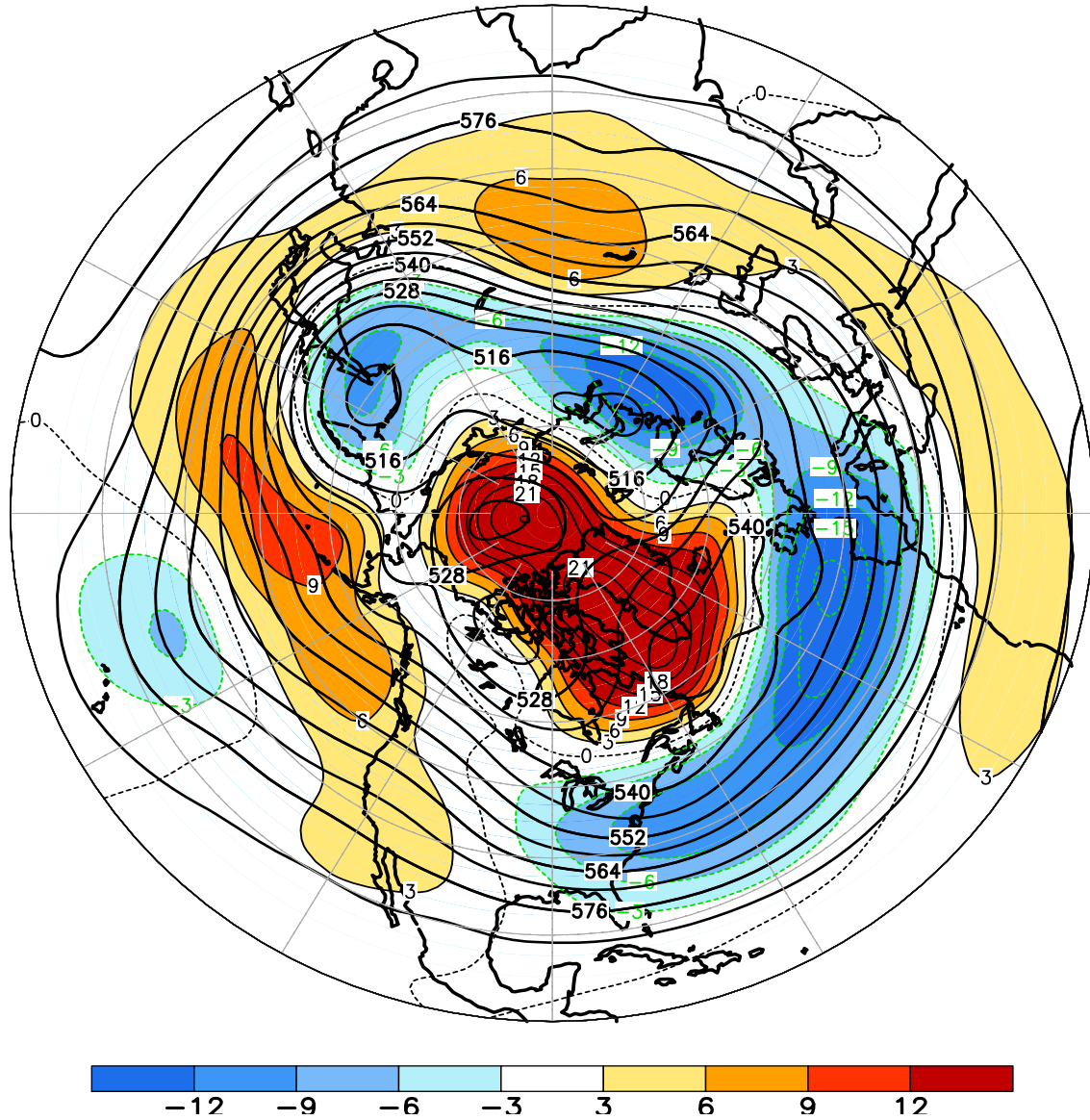
FIGURE E9. Northern Hemisphere mean and anomalous 500-hPa geopotential height (CDAS/Reanalysis) for MAR 2013. Mean heights are denoted by solid contours drawn at an interval of 6 dam. Anomaly contour interval is 3 dam with values less (greater) than -3 dam (3 dam) indicated by dark (light) shading. Anomalies are calculated as departures from the 1981-2010 base period monthly means.
