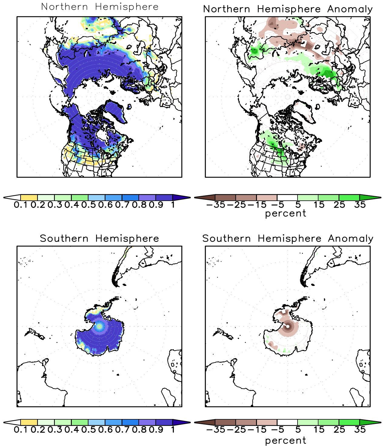
FIGURE A2.2. SSM/I derived snow cover frequency (%) (left) and snow cover anomaly (%) (right) for the month of MAR 2013 based on 1987 - 2010 base period for the Northern Hemisphere (top) and Southern Hemisphere (bottom). It is generated using the algorithm described by Ferraro et. al, 1996, Bull. Amer. Meteor. Soc., vol 77, 891-905.
