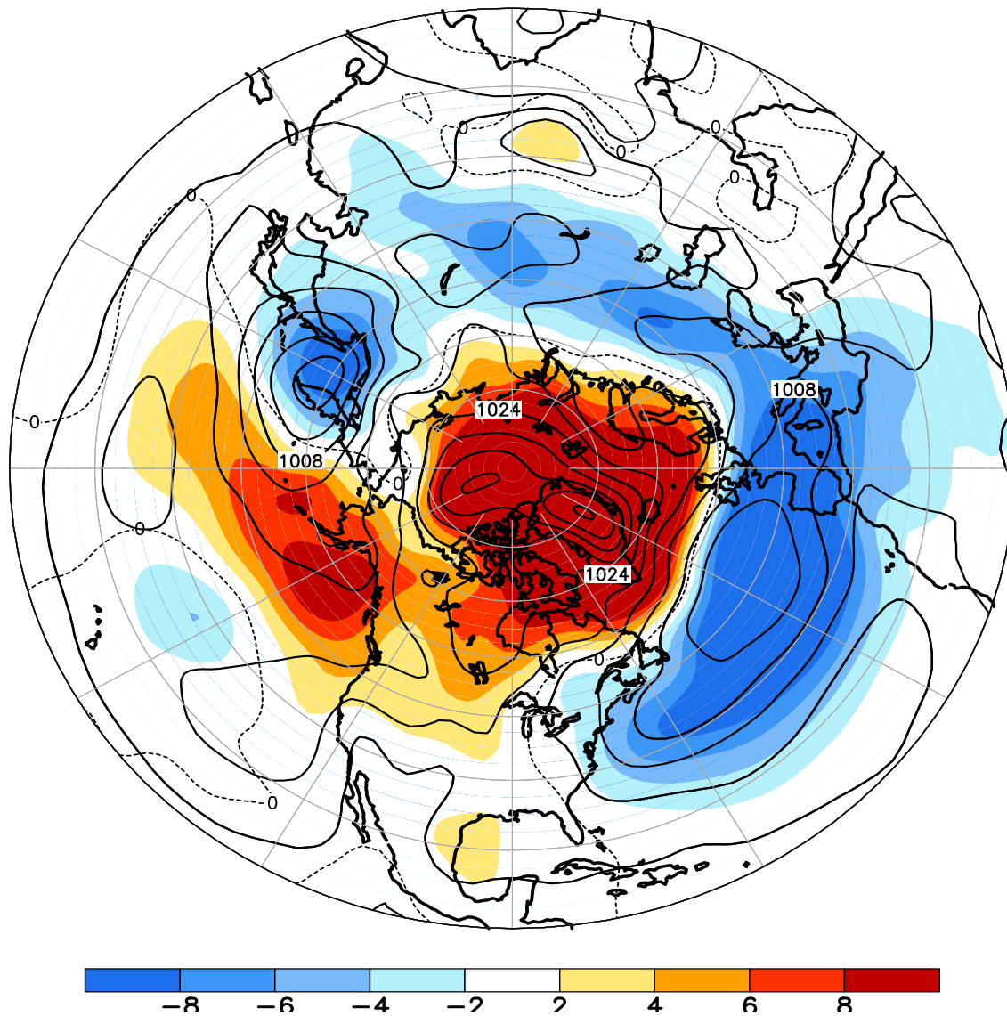
FIGURE E8. Northern Hemisphere mean and anomalous sea level pressure (CDAS/Reanalysis) for MAR 2013. Mean values are denoted by solid contours drawn at an interval of 4 hPa. Anomaly contour interval is 2 hPa with values less (greater) than -2 hPa (2 hPa) indicated by dark (light) shading. Anomalies are calculated as departures from the 1981-2010 base period monthly means.
