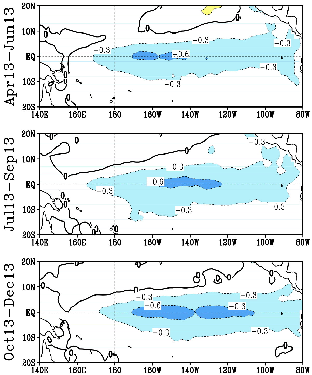
FIGURE F5. Predicted 3-month average sea surface temperature anomalies from the NCEP/CPC Markov model (Xue et al. 2000, J. Climate , 13 , 849-871). The forecast is initiated in MAR 2013. Contour interval is 0.3C and negative anomalies are indicated by dashed contours. Anomalies are calculated relative to the 1971-2000 climatology.
