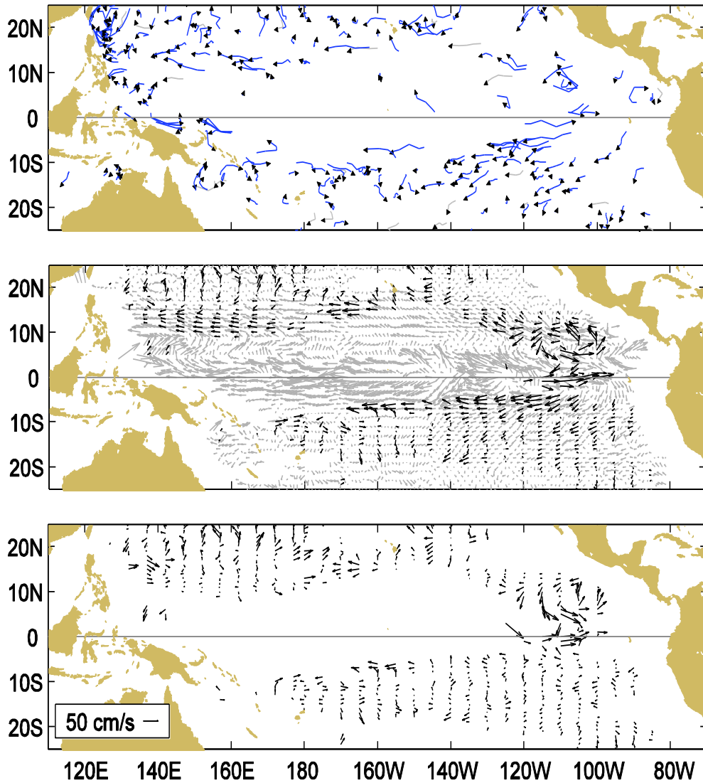
Figure A1.1 Top: Movements of drifting buoys in the tropical Pacific Ocean during April 2013. The linear segments of each trajectory represent a one week displacement. Trajectories of buoys which have lost their subsurface drogues are gray; those with drogues are black.
