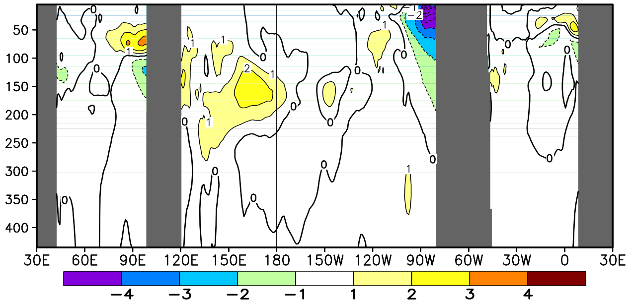
FIGURE T17. Equatorial depth–longitude section of ocean temperature (top) and ocean temperature anomalies (bottom) for MAR 2013. Contour interval is 1°C. Dashed contours in bottom panel indicate negative anomalies. Data are derived from the NCEP’s global ocean data assimilation system version 2 which assimilates oceanic observations into an oceanic GCM (Xue, Y. and Behringer, D.W., 2006: Operational global ocean data assimilation system at NCEP, to be submitted to BAMS). Anomalies are departures from the 1981–2010 base period means.
