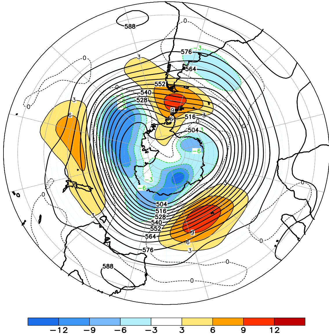
FIGURE E15. Southern Hemisphere mean and anomalous 500-hPa geopotential height (CDAS/Reanalysis) for MAR 2013. Mean heights are denoted by solid contours drawn at an interval of 6 dam. Anomaly contour interval is 3 dam with values less (greater) than -3 dam (3 dam) indicated by dark (light) shading. Anomalies are calculated as departures from the 1981-2010 base period monthly means.
