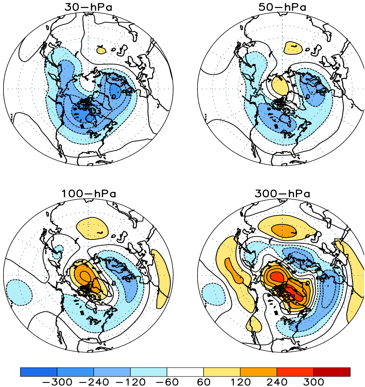
FIGURE S1. Stratospheric height anomalies (m) at selected levels for MAR 2013. Positive values are indicated by solid contours and dark shading. Negative values are indicated by dashed contours and light shading. Contour interval is 60 m. Anomalies are calculated from the 1981-2010 base period means. Winter Hemisphere is shown.
