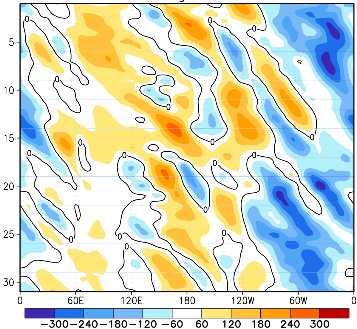
FIGURE E12. Northern Hemisphere: Daily 500-hPa height anomalies for MAR 2013 averaged over the 5° latitude band centered on 40°N. Positive values are indicated by solid contours and dark shading. Negative values are indicated by dashed contours and light shading. Contour interval is 60 m. Anomalies are departures from the 1981-2010 base period daily means.
