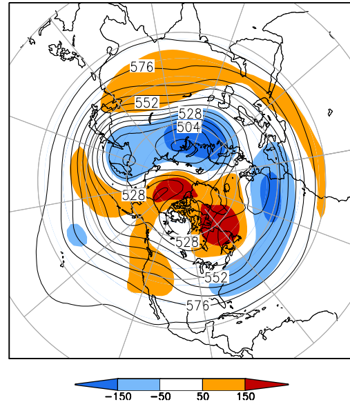
500-hPa Height (dm) & Anomalies (m) (Mar 1–15, 2013)
