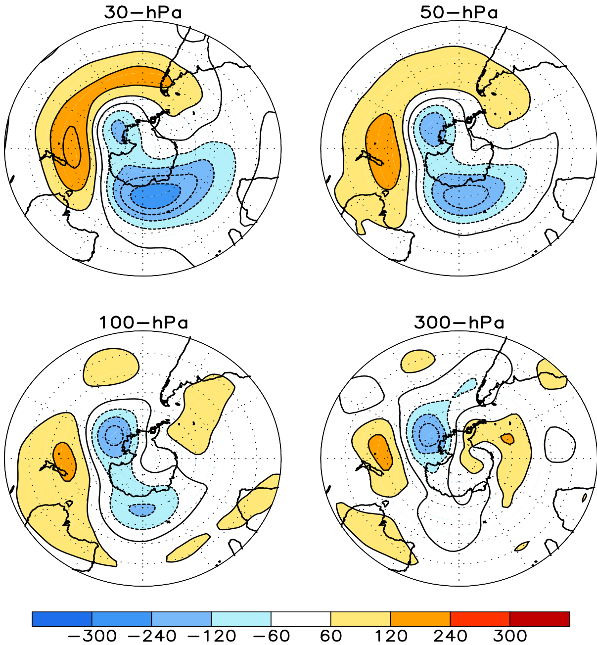
FIGURE S1. Stratospheric height anomalies (m) at selected levels for JUN 2020. Positive values are indicated by solid contours and dark shading. Negative values are indicated by dashed contours and light shading. Contour interval is 60 m. Anomalies are calculated from the 1981-2010 base period means. Winter Hemisphere is shown.
