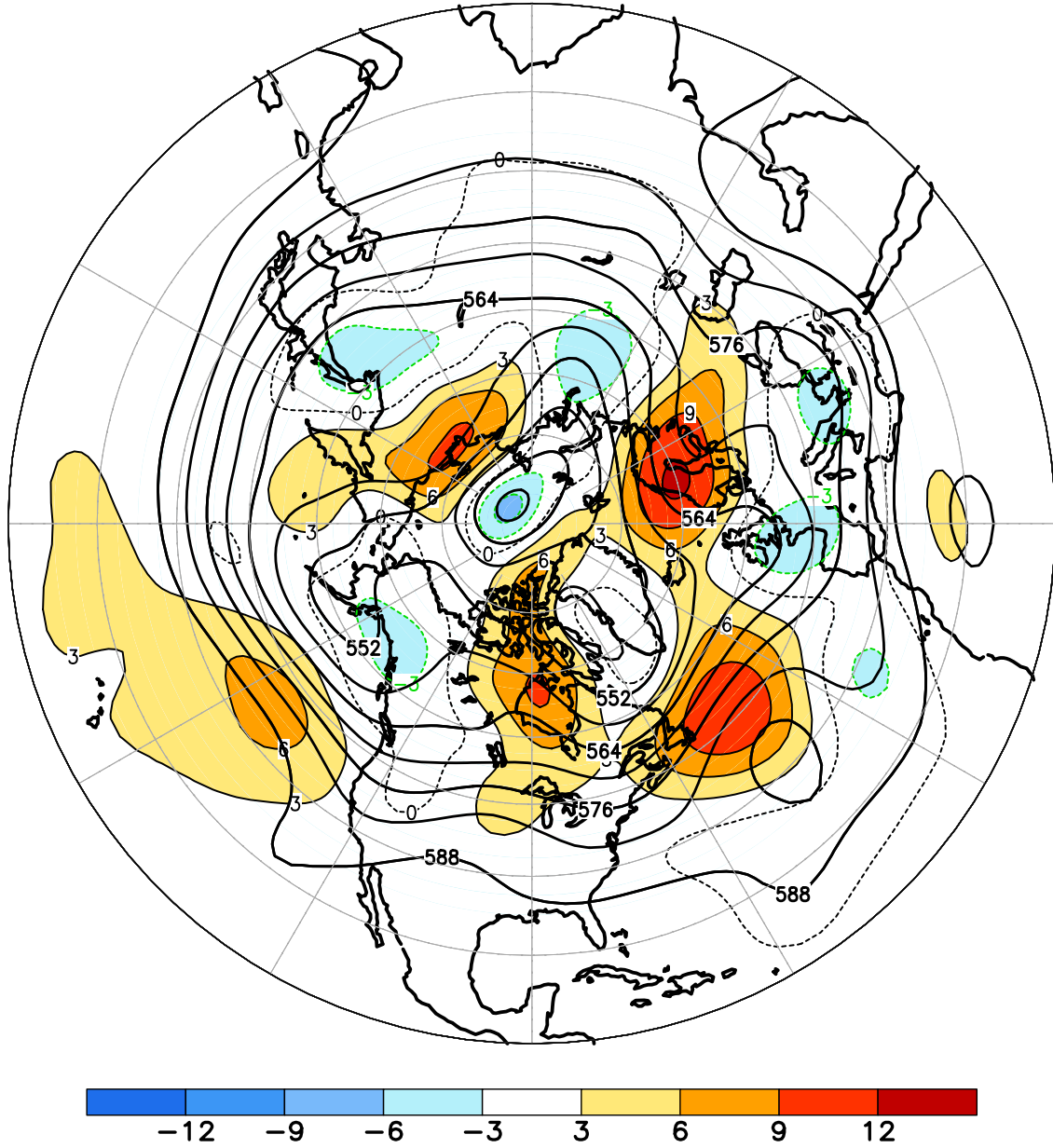
FIGURE E9. Northern Hemisphere mean and anomalous 500-hPa geopotential height (CDAS/Reanalysis) for JUN 2020. Mean heights are denoted by solid contours drawn at an interval of 6 dam. Anomaly contour interval is 3 dam with values less (greater) than -3 dam (3 dam) indicated by dark (light) shading. Anomalies are calculated as departures from the 1981-2010 base period monthly means.
