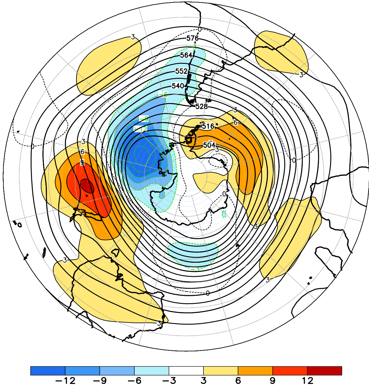
FIGURE E15. Southern Hemisphere mean and anomalous 500-hPa geopotential height (CDAS/Reanalysis) for JUN 2020. Mean heights are denoted by solid contours drawn at an interval of 6 dam. Anomaly contour interval is 3 dam with values less (greater) than -3 dam (3 dam) indicated by dark (light) shading. Anomalies are calculated as departures from the 1981-2010 base period monthly means.
