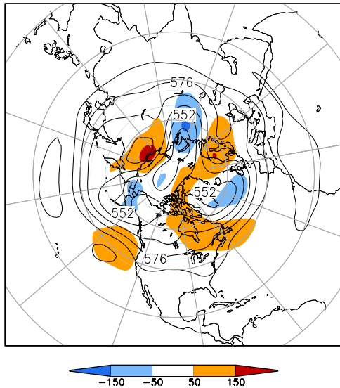
500-hPa Height (dm) & Anomalies (m) (Jun 16–30, 2020)
