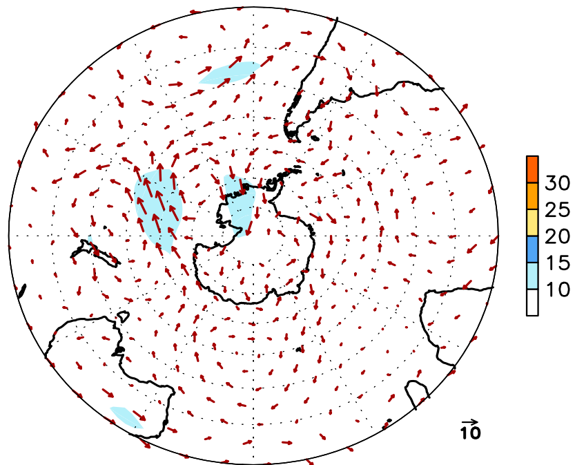
FIGURE E16. Southern Hemisphere mean (left) and anomalous (right) 300-hPa vector wind (CDAS/Reanalysis) for JUN 2020. Mean (anomaly) isotach contour interval is 10 (5) \text{ms}^{-1} . Values greater than 30 \text{ ms}^{-1} (left) and 10 \text{ ms}^{-1} (rights) are shaded. Anomalies are departures from the 1981-2010 base period monthly means.
