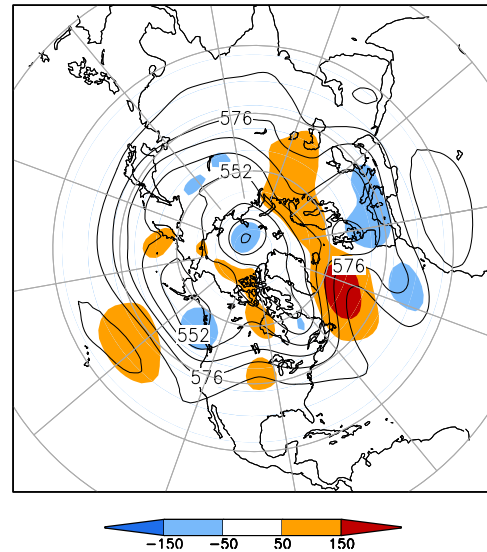
500-hPa Height (dm) & Anomalies (m) (Jun 1–15, 2020)
