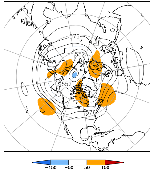
500-hPa Height (dm) & Anomalies (m) (Jun 1–30, 2020)
