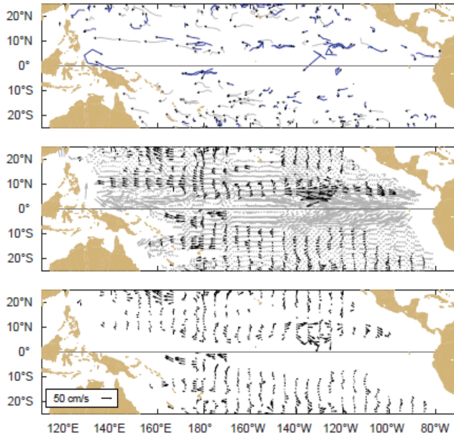
Figure A1.1 Top: Movements of drifting buoys in the tropical Pacific Ocean during June 2020. The linear segments of each trajectory represent a one week displacement. Trajectories of buoys which have lost their subsurface drogues are gray; those with drogues are black.
