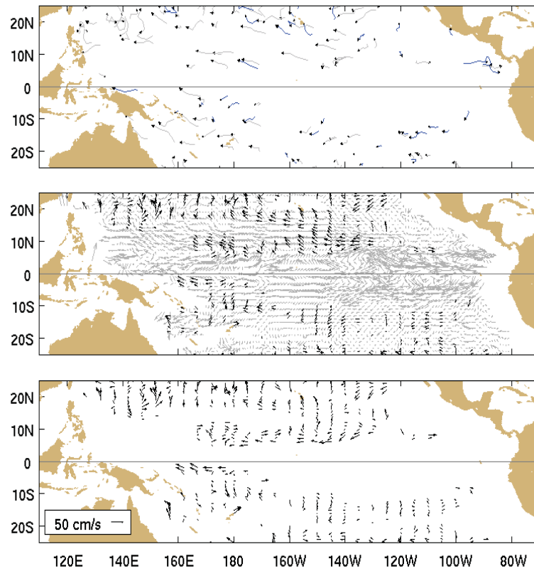
Figure A1.1 Top: Movements of drifting buoys in the tropical Pacific Ocean during June 2017. The linear segments of each trajectory represent a one week displacement. Trajectories of buoys which have lost their subsurface drogues are gray; those with drogues are black.
