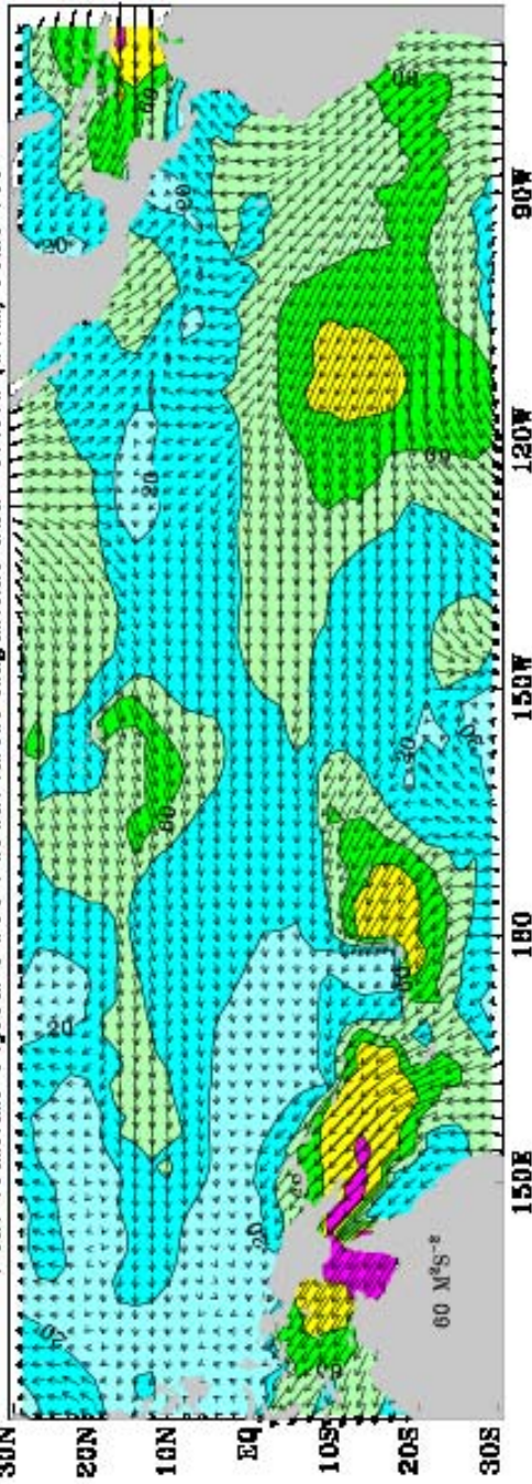
Near realtime Objective FSU Pseudostress Magnitude and Vectors (10m) June 2017
