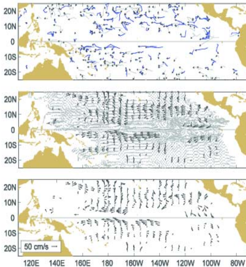
Figure A1.1 Top: Movements of drifting buoys in the tropical Pacific Ocean during June 2016. The linear segments of each trajectory represent a one week displacement. Trajectories of buoys which have lost their subsurface drogues are gray; those with drogues are black. Middle: Monthly mean currents calculated from all buoys 1993-2002 (gray), and currents measured by the drogued buoys this month (black) smoothed by an optimal filter. Bottom: Anomalies from the climatological monthly mean currents for this month.
