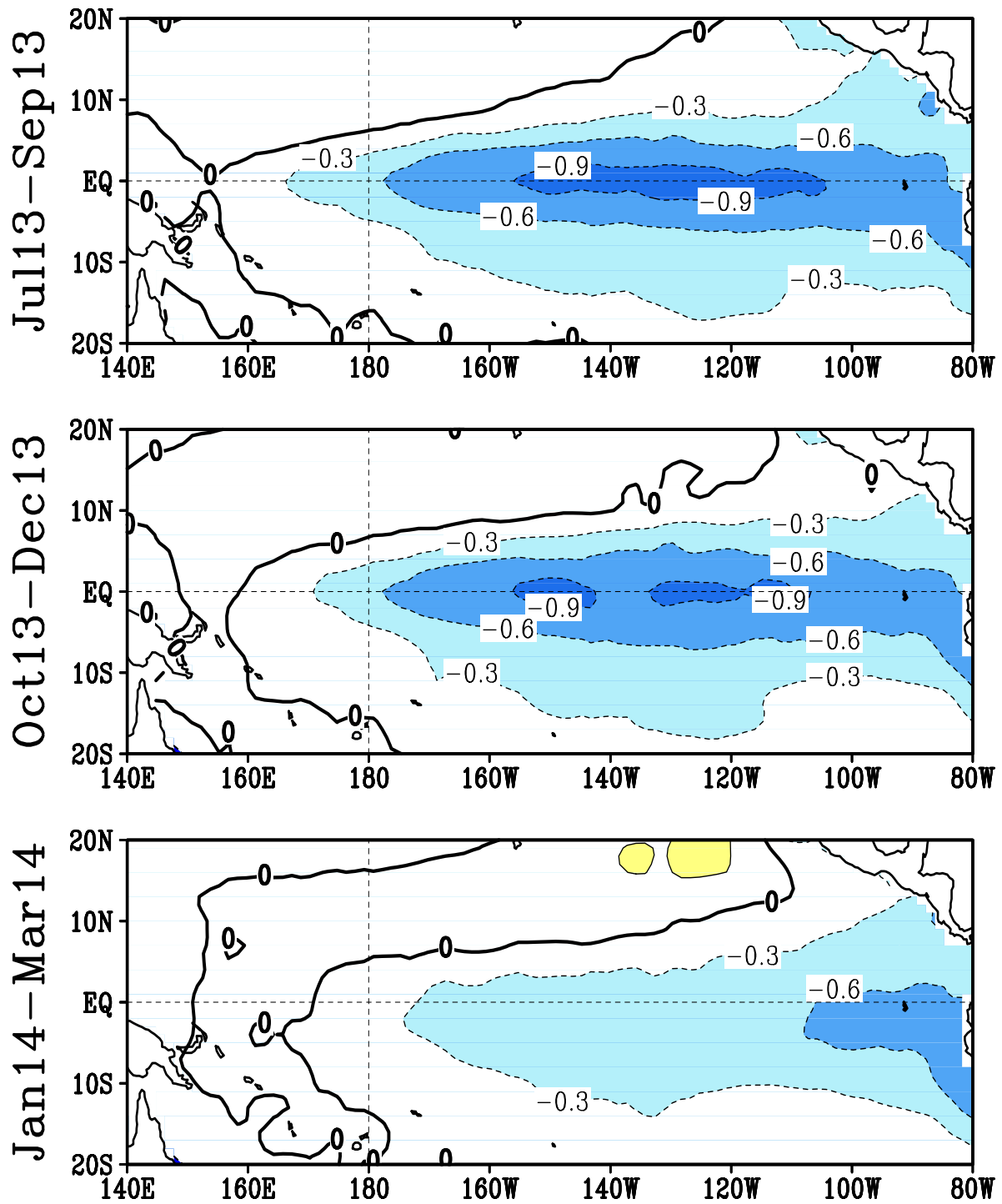
FIGURE F5. Predicted 3-month average sea surface temperature anomalies from the NCEP/CPC Markov model (Xue et al. 2000, J. Climate , 13 , 849-871). The forecast is initiated in JUN 2013 . Contour interval is 0.3C and negative anomalies are indicated by dashed contours. Anomalies are calculated relative to the 1971-2000 climatology.
