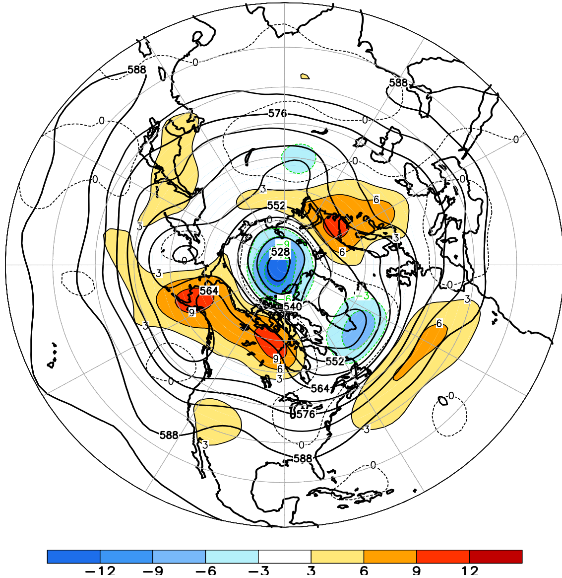
FIGURE E9. Northern Hemisphere mean and anomalous 500-hPa geopotential height (CDAS/Reanalysis) for JUN 2013. Mean heights are denoted by solid contours drawn at an interval of 6 dam. Anomaly contour interval is 3 dam with values less (greater) than -3 dam (3 dam) indicated by dark (light) shading. Anomalies are calculated as departures from the 1981-2010 base period monthly means.
