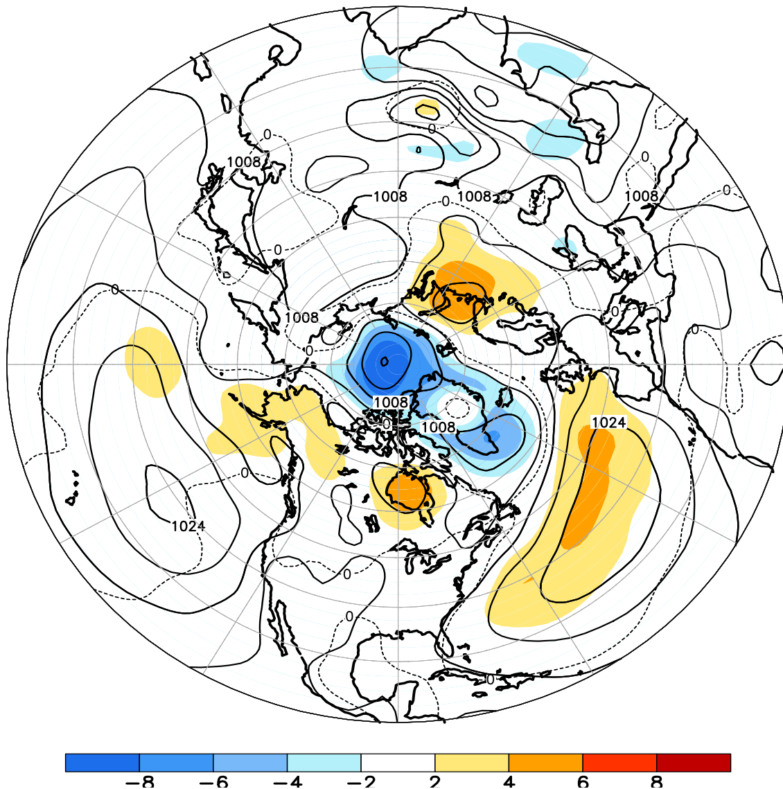
FIGURE E8. Northern Hemisphere mean and anomalous sea level pressure (CDAS/Reanalysis) for JUN 2013. Mean values are denoted by solid contours drawn at an interval of 4 hPa. Anomaly contour interval is 2 hPa with values less (greater) than -2 hPa (2 hPa) indicated by dark (light) shading. Anomalies are calculated as departures from the 1981-2010 base period monthly means.
