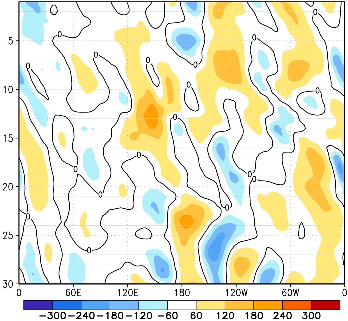
FIGURE E12. Northern Hemisphere: Daily 500-hPa height anomalies for JUN 2013 averaged over the 5° latitude band centered on 40°N. Positive values are indicated by solid contours and dark shading. Negative values are indicated by dashed contours and light shading. Contour interval is 60 m. Anomalies are departures from the 1981-2010 base period daily means.
