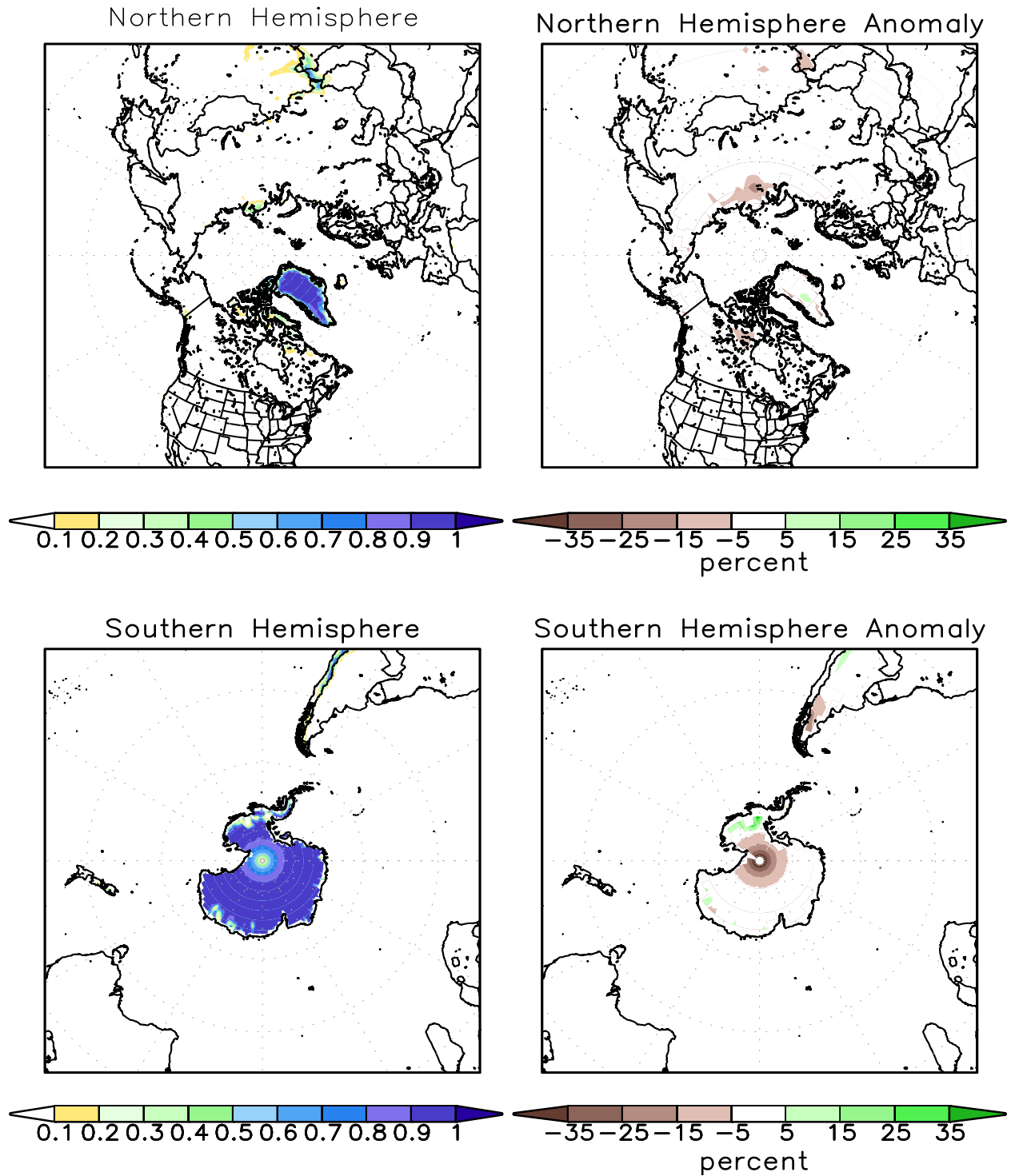
FIGURE A2.2. SSM/I derived snow cover frequency (%) (left) and snow cover anomaly (%) (right) for the month of JUN 2013 based on 1987 - 2010 base period for the Northern Hemisphere (top) and Southern Hemisphere (bottom). It is generated using the algorithm described by Ferraro et. al, 1996, Bull. Amer. Meteor. Soc., vol 77, 891-905.
