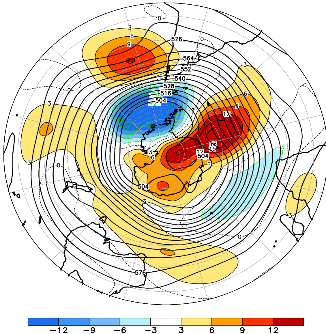
FIGURE E15. Southern Hemisphere mean and anomalous 500-hPa geopotential height (CDAS/Reanalysis) for JUN 2013. Mean heights are denoted by solid contours drawn at an interval of 6 dam. Anomaly contour interval is 3 dam with values less (greater) than -3 dam (3 dam) indicated by dark (light) shading. Anomalies are calculated as departures from the 1981-2010 base period monthly means.
