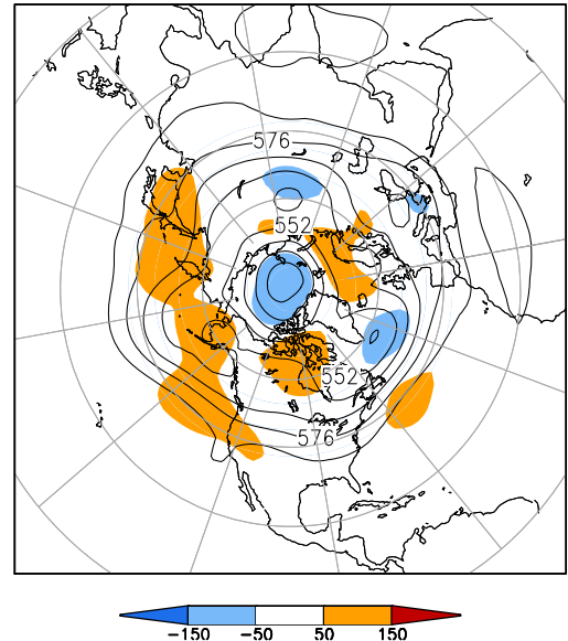
500-hPa Height (dm) & Anomalies (m) (Jun 1–15, 2013)
