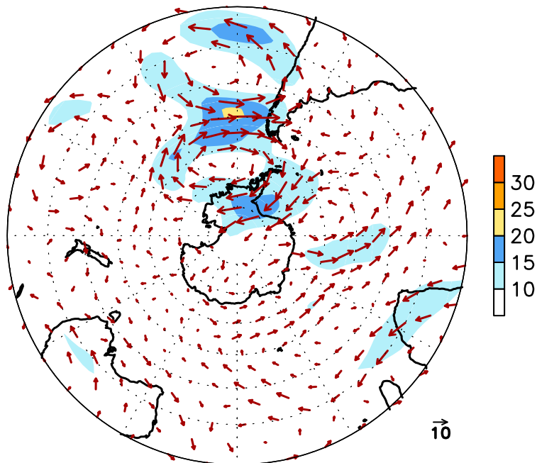
FIGURE E16. Southern Hemisphere mean (left) and anomalous (right) 300-hPa vector wind (CDAS/Reanalysis) for JUN 2013. Mean (anomaly) isotach contour interval is 10 (5) \text{ms}^{-1} . Values greater than 30 \text{ms}^{-1} (left) and 10 \text{ms}^{-1} (rights) are shaded. Anomalies are departures from the 1981-2010 base period monthly means.
