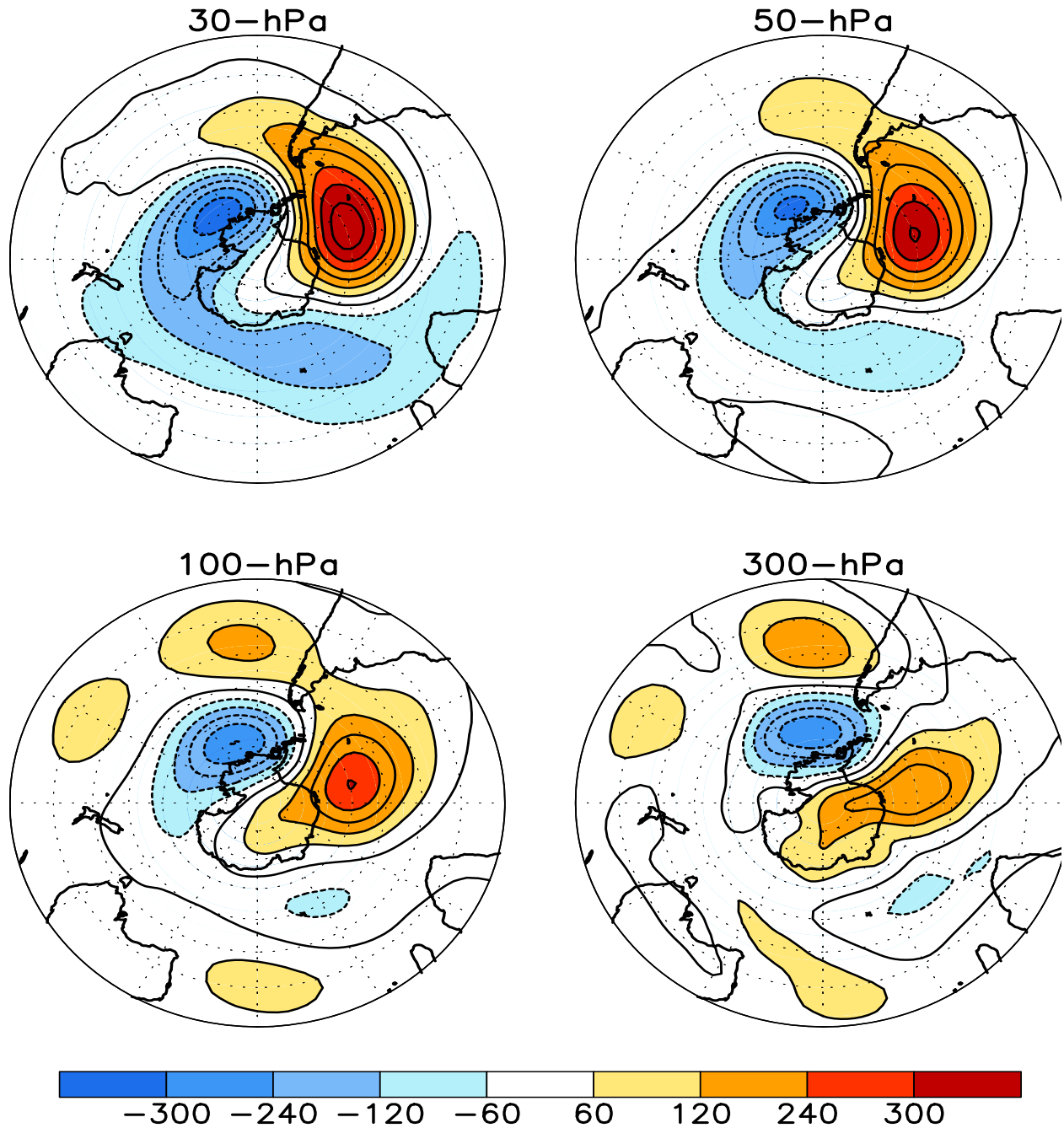
FIGURE S1. Stratospheric height anomalies (m) at selected levels for JUN 2013. Positive values are indicated by solid contours and dark shading. Negative values are indicated by dashed contours and light shading. Contour interval is 60 m. Anomalies are calculated from the 1981-2010 base period means. Winter Hemisphere is shown.
