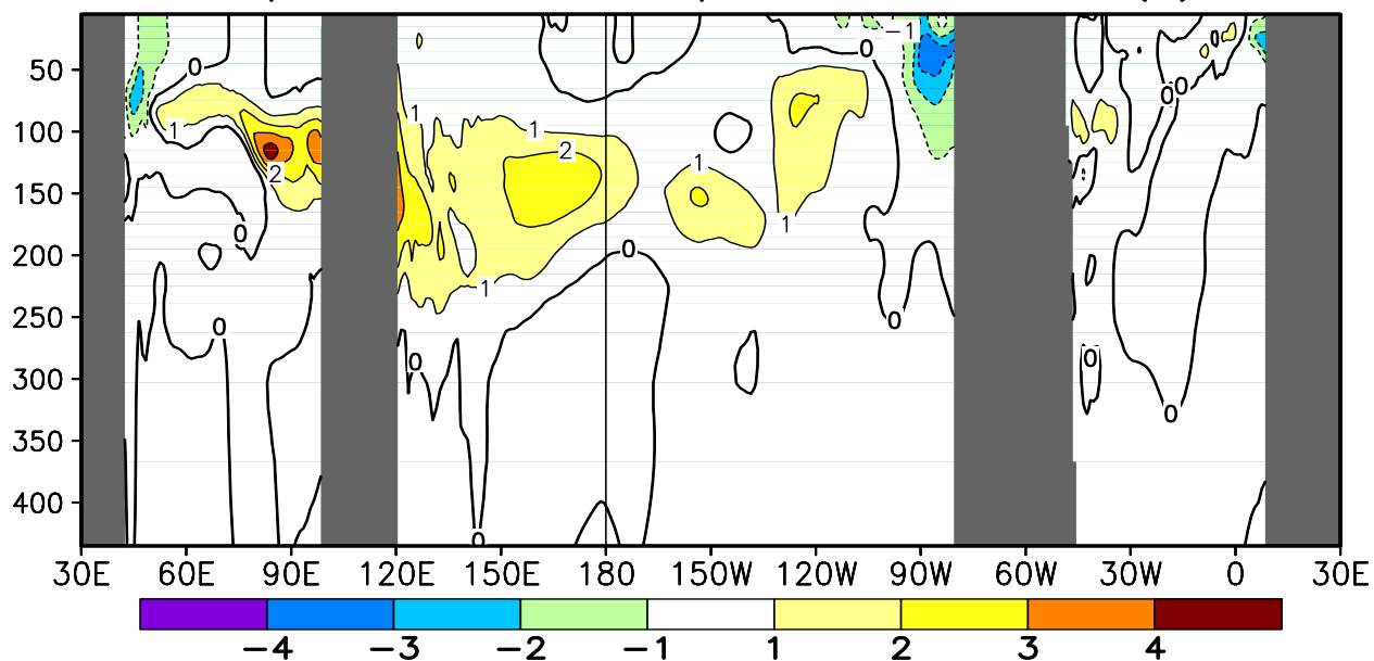
FIGURE T17. Equatorial depth–longitude section of ocean temperature (top) and ocean temperature anomalies (bottom) for JUN 2013. Contour interval is 1°C. Dashed contours in bottom panel indicate negative anomalies. Data are derived from the NCEP’s global ocean data assimilation system version 2 which assimilates oceanic observations into an oceanic GCM (Xue, Y. and Behringer, D.W., 2006: Operational global ocean data assimilation system at NCEP, to be submitted to BAMS). Anomalies are departures from the 1981–2010 base period means.
