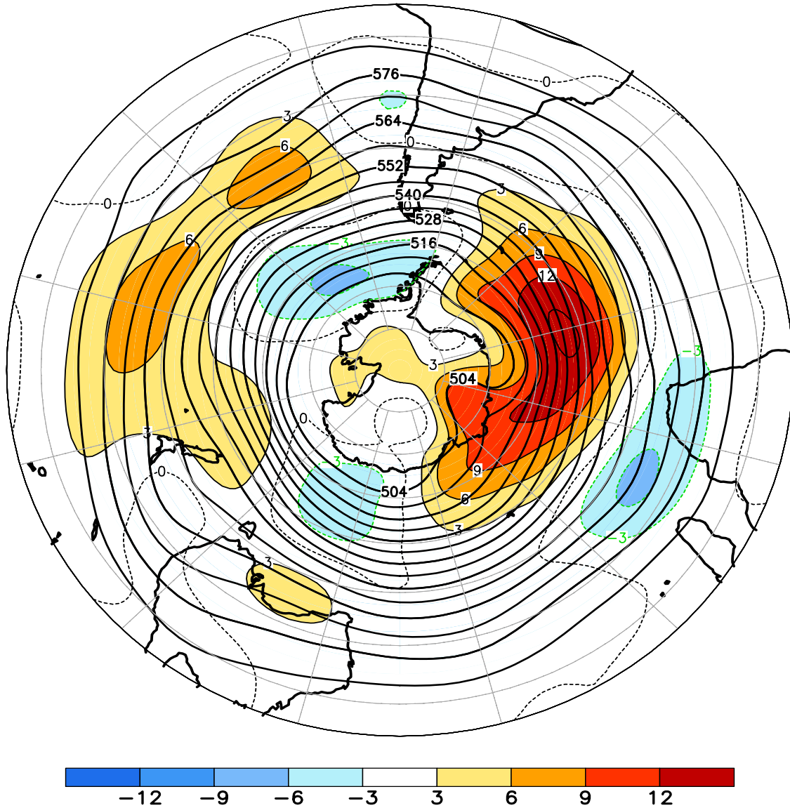
FIGURE E15. Southern Hemisphere mean and anomalous 500-hPa geopotential height (CDAS/Reanalysis) for JUN 2011. Mean heights are denoted by solid contours drawn at an interval of 6 dam. Anomaly contour interval is 3 dam with values less (greater) than -3 dam (3 dam) indicated by dark (light) shading. Anomalies are calculated as departures from the 1981-2010 base period monthly means.
