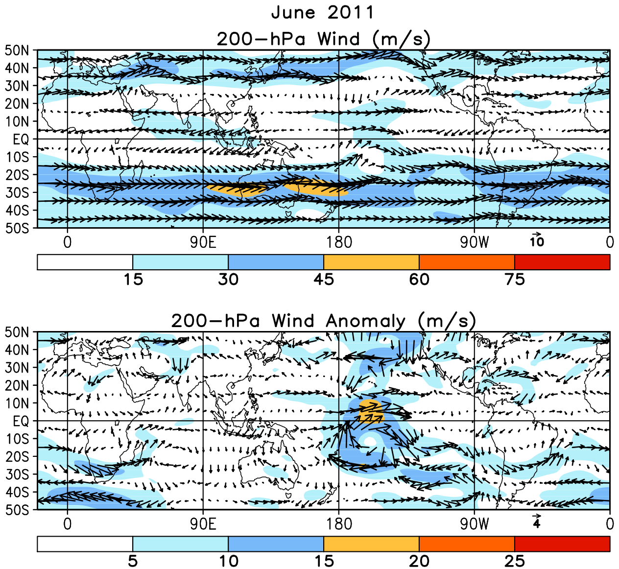
FIGURE T21. Mean (top) and anomalous (bottom) 200-hPa vector wind (CDAS/Reanalysis) for JUN 2011. Contour interval for isotachs is 15 \text{ ms}^{-1} (top) and 5 \text{ ms}^{-1} (bottom). Anomalies are departures from 1981-2010 base period monthly means.
