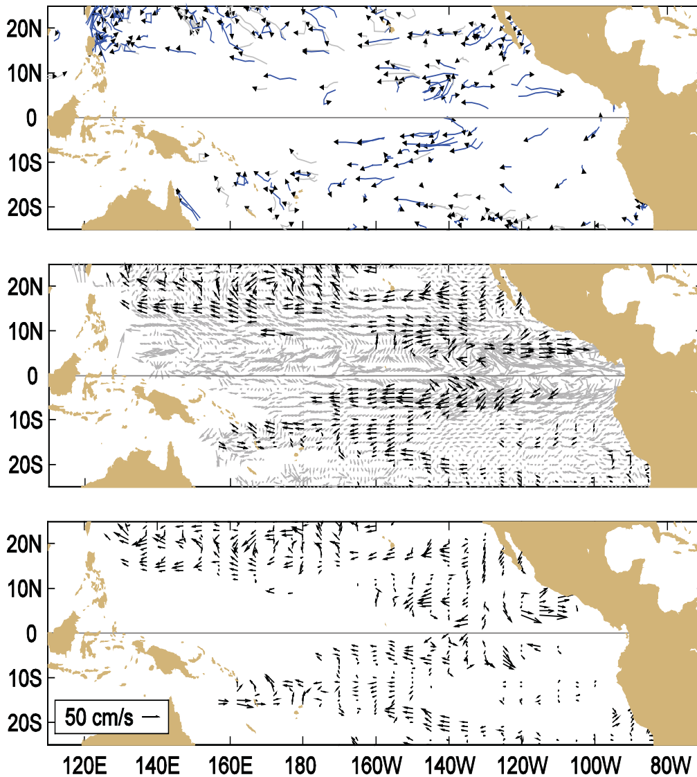
Figure A1.1 Top: Movements of drifting buoys in the tropical Pacific Ocean during June 2011. The linear segments of each trajectory represent a one week displacement. Trajectories of buoys which have lost their subsurface drogues are gray; those with drogues are black.
