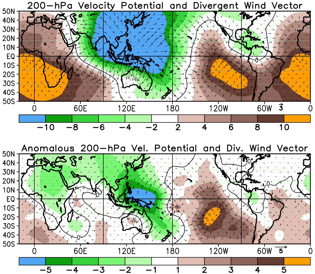
FIGURE T24. Mean (top) and anomalous (bottom) 200-hPa velocity potential ( 10^6\text{m}^2\text{s} ) and divergent wind (CDAS/Reanalysis). Anomalies are departures from the 1981-2010 base period monthly means.
