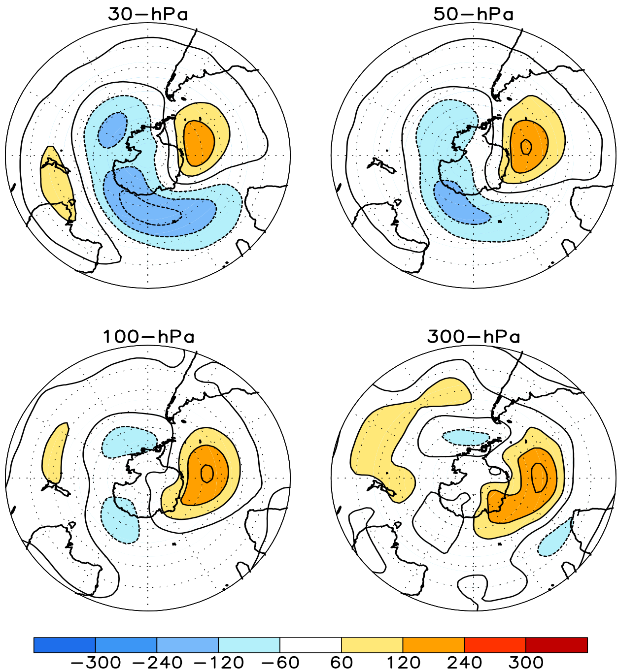
FIGURE S1. Stratospheric height anomalies (m) at selected levels for JUN 2011. Positive values are indicated by solid contours and dark shading. Negative values are indicated by dashed contours and light shading. Contour interval is 60 m. Anomalies are calculated from the 1981-2010 base period means. Winter Hemisphere is shown.
