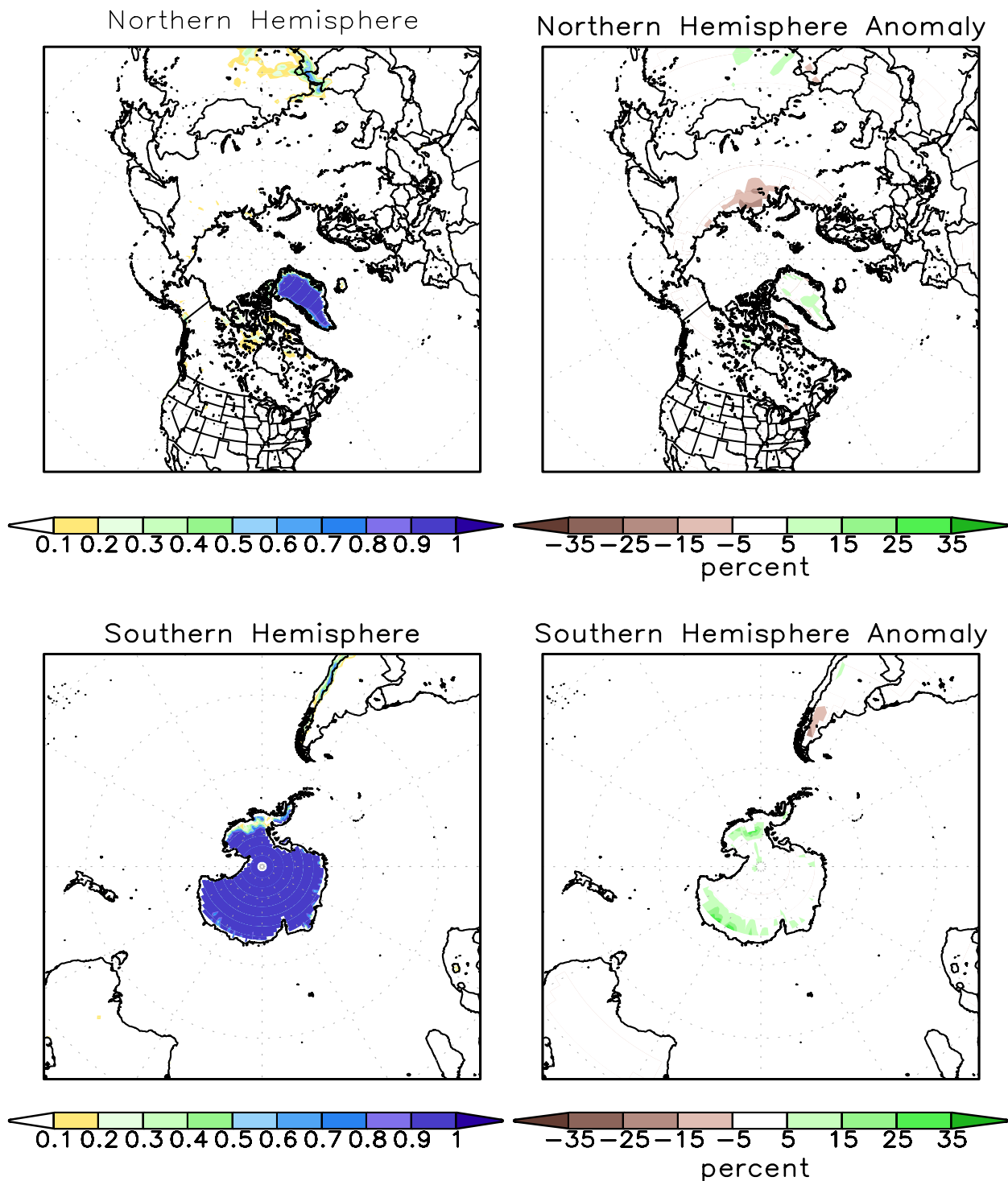
FIGURE A2.2. SSM/I derived snow cover frequency (%) (left) and snow cover anomaly (%) (right) for the month of JUN 2011 based on 1987 - 2010 base period for the Northern Hemisphere (top) and Southern Hemisphere (bottom). It is generated using the algorithm described by Ferraro et. al, 1996, Bull. Amer. Meteor. Soc., vol 77, 891-905.
