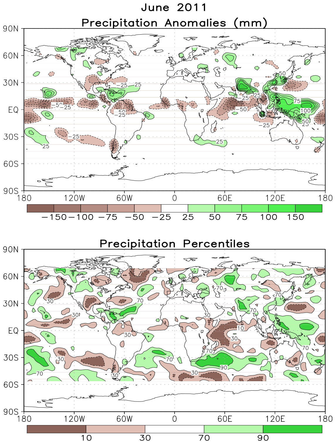
FIGURE E3. Anomalous precipitation (mm, top) and precipitation percentiles based on a Gamma distribution fit to the 1981–2010 base period data (bottom) for JUN 2011. Data are obtained from a merge of raingauge observations and satellite-derived precipitation estimates (Janowiak and Xie 1999, J. Climate , 12 , 3335–3342). Contours are drawn at 200, 100, 50, 25, -25, -50, -100, and -200 mm in top panel. Percentiles are not plotted in regions where mean monthly precipitation is <5mm/month.
