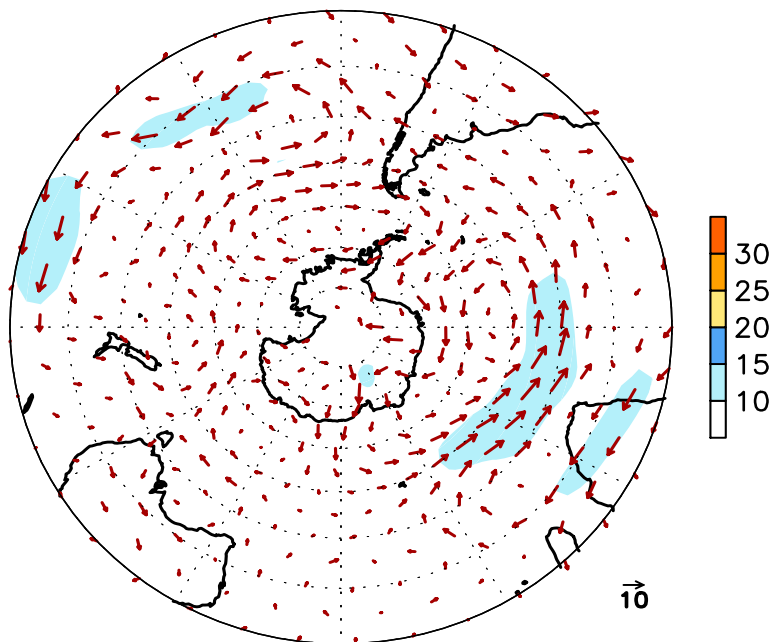
FIGURE E16. Southern Hemisphere mean (left) and anomalous (right) 300-hPa vector wind (CDAS/Reanalysis) for JUN 2011. Mean (anomaly) isotach contour interval is 10 (5) \text{ms}^{-1} . Values greater than 30 \text{ms}^{-1} (left) and 10 \text{ms}^{-1} (rights) are shaded. Anomalies are departures from the 1981-2010 base period monthly means.
