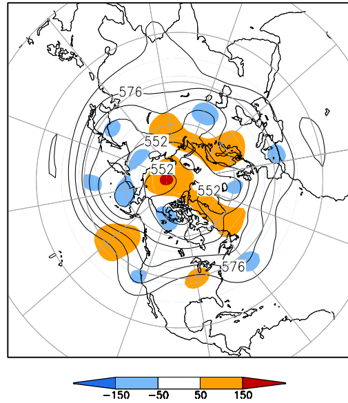
500-hPa Height (dm) & Anomalies (m) (Jun 1–15, 2011)
