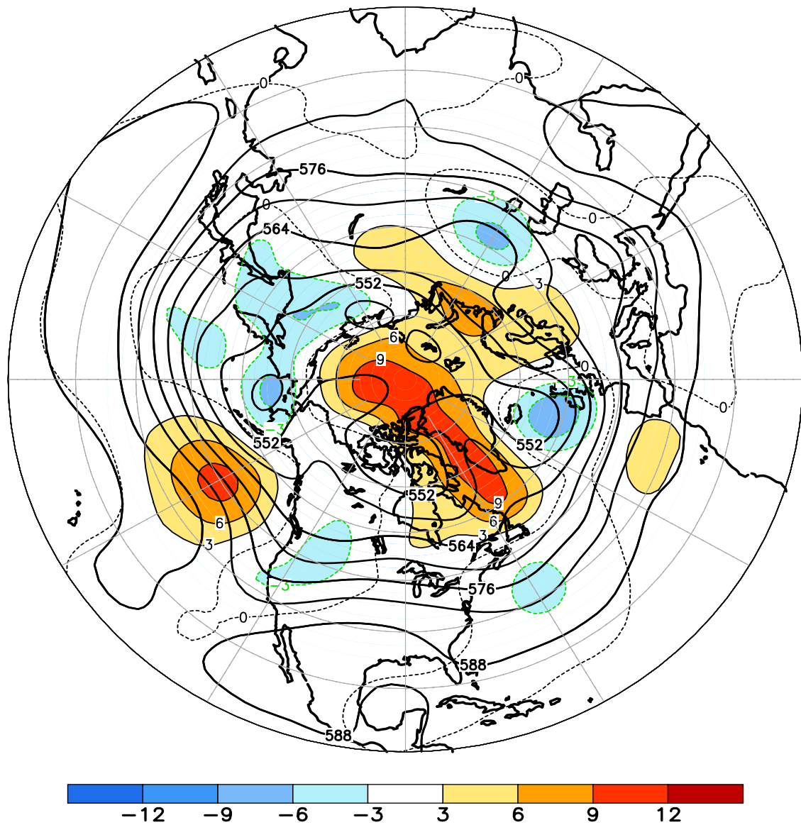
FIGURE E9. Northern Hemisphere mean and anomalous 500-hPa geopotential height (CDAS/Reanalysis) for JUN 2011. Mean heights are denoted by solid contours drawn at an interval of 6 dam. Anomaly contour interval is 3 dam with values less (greater) than -3 dam (3 dam) indicated by dark (light) shading. Anomalies are calculated as departures from the 1981-2010 base period monthly means.
