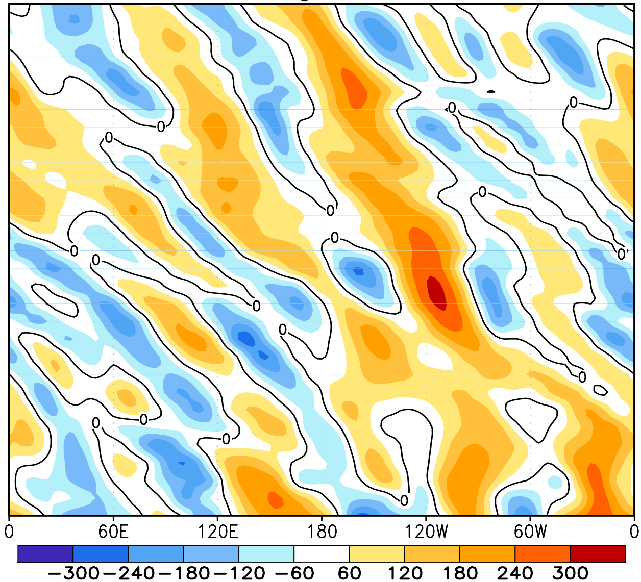
FIGURE E18. Southern Hemisphere: Daily 500-hPa height anomalies for JUN 2011 averaged over the 5° latitude band centered on 40°S. Positive values are indicated by solid contours and dark shading. Negative values are indicated by dashed contours and light shading. Contour interval is 60 m. Anomalies are departures from the 1981-2010 base period daily means.
