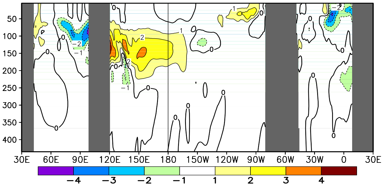
FIGURE T17. Equatorial depth–longitude section of ocean temperature (top) and ocean temperature anomalies (bottom) for JUN 2011. Contour interval is 1°C. Dashed contours in bottom panel indicate negative anomalies. Data are derived from the NCEP’s global ocean data assimilation system version 2 which assimilates oceanic observations into an oceanic GCM (Xue, Y. and Behringer, D.W., 2006: Operational global ocean data assimilation system at NCEP, to be submitted to BAMS). Anomalies are departures from the 1981–2010 base period means.
