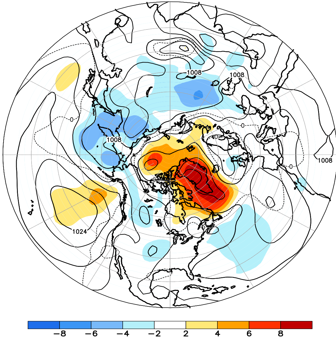
FIGURE E8. Northern Hemisphere mean and anomalous sea level pressure (CDAS/Reanalysis) for JUN 2011. Mean values are denoted by solid contours drawn at an interval of 4 hPa. Anomaly contour interval is 2 hPa with values less (greater) than -2 hPa (2 hPa) indicated by dark (light) shading. Anomalies are calculated as departures from the 1981-2010 base period monthly means.
