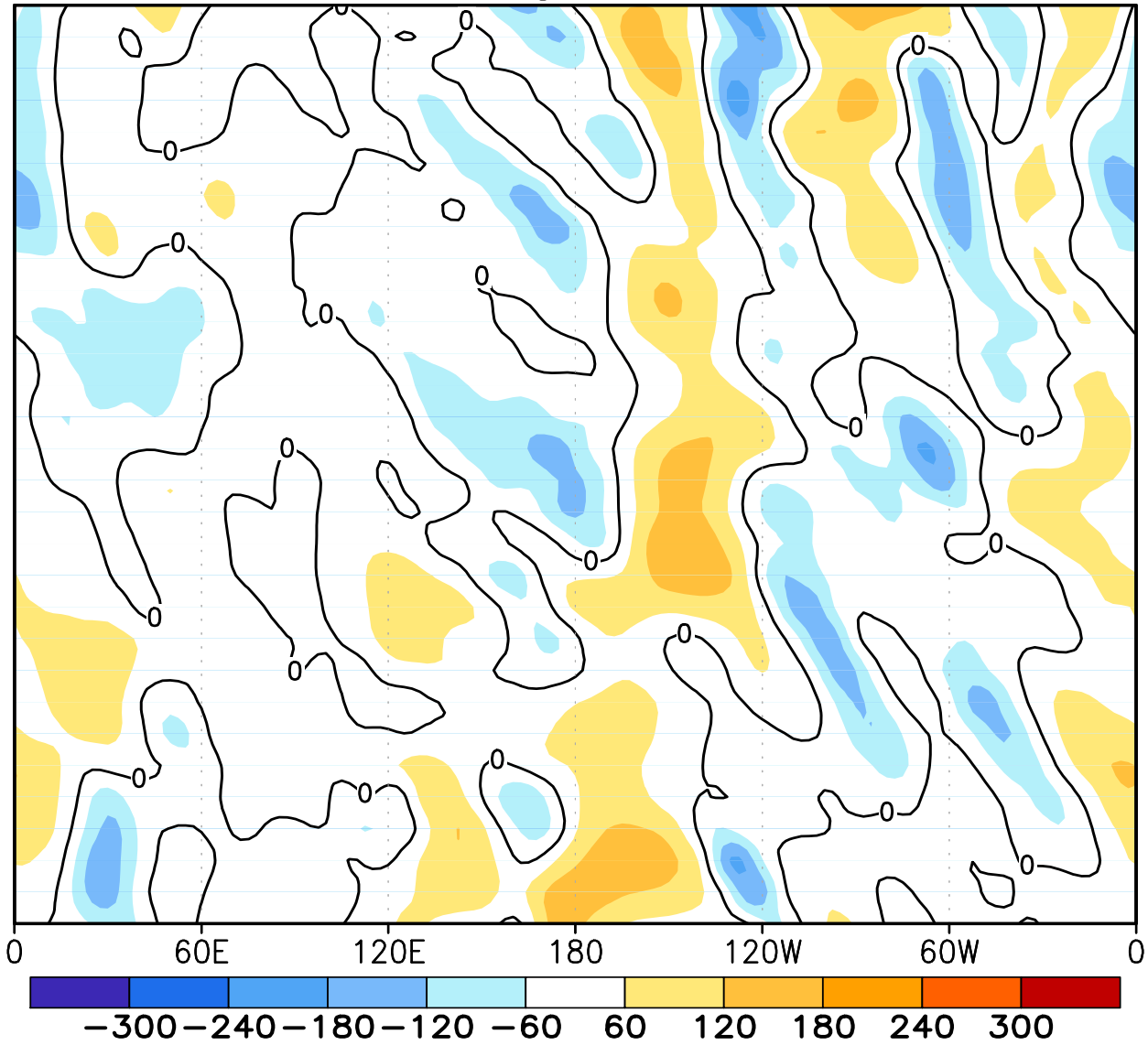
FIGURE E12. Northern Hemisphere: Daily 500-hPa height anomalies for JUN 2011 averaged over the 5° latitude band centered on 40°N. Positive values are indicated by solid contours and dark shading. Negative values are indicated by dashed contours and light shading. Contour interval is 60 m. Anomalies are departures from the 1981-2010 base period daily means.
