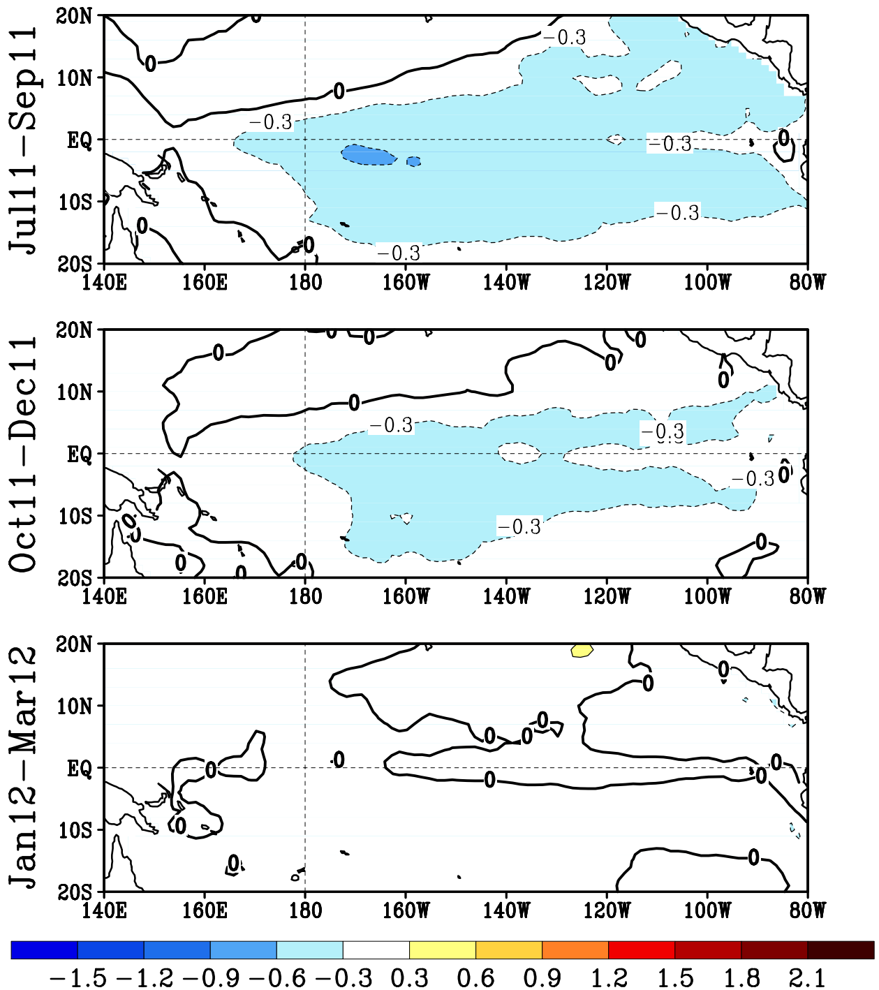
FIGURE F5. Predicted 3-month average sea surface temperature anomalies from the NCEP/CPC Markov model (Xue et al. 2000, J. Climate , 13 , 849-871). The forecast is initiated in JUN 2011 . Contour interval is 0.3C and negative anomalies are indicated by dashed contours. Anomalies are calculated relative to the 1971-2000 climatology.
