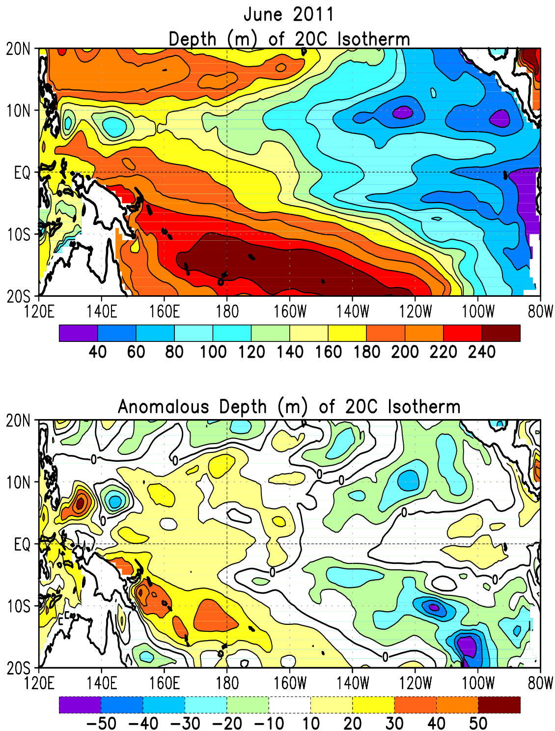
FIGURE T16. Mean (top) and anomalous (bottom) depth of the 20°C isotherm for JUN 2011. Contour interval is 40 m (top) and 10 m (bottom). Dashed contours in bottom panel indicate negative anomalies. Data are derived from the NCEP’s global ocean data assimilation system version 2 which assimilates oceanic observations into an oceanic GCM (Xue, Y. and Behringer, D.W., 2006: Operational global ocean data assimilation system at NCEP, to be submitted to BAMS). Anomalies are departures from the 1981–2010 base period means.
