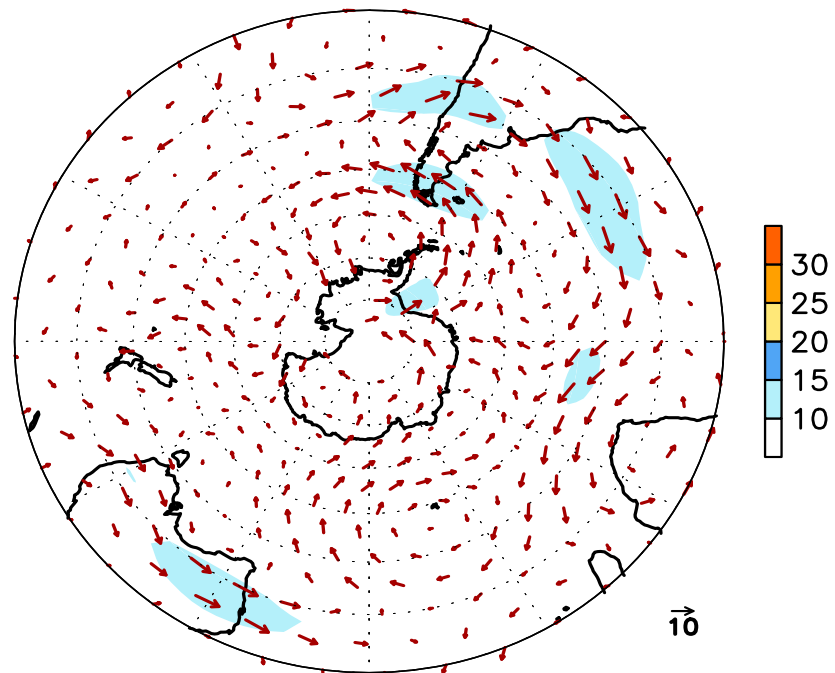
FIGURE E16. Southern Hemisphere mean (left) and anomalous (right) 300-hPa vector wind (CDAS/Reanalysis) for JUL 2020. Mean (anomaly) isotach contour interval is 10 (5) \text{ms}^{-1} . Values greater than 30 \text{ms}^{-1} (left) and 10 \text{ms}^{-1} (rights) are shaded. Anomalies are departures from the 1981-2010 base period monthly means.
