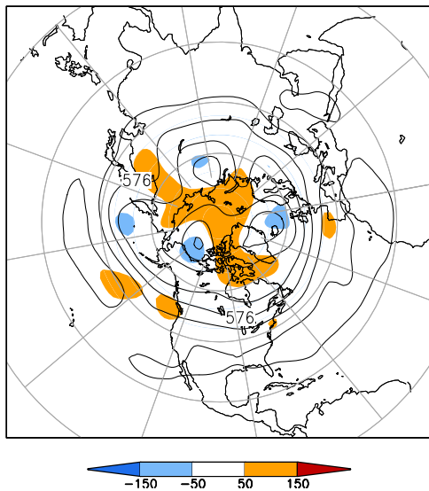
500-hPa Height (dm) & Anomalies (m) (Jul 16-31, 2020)
