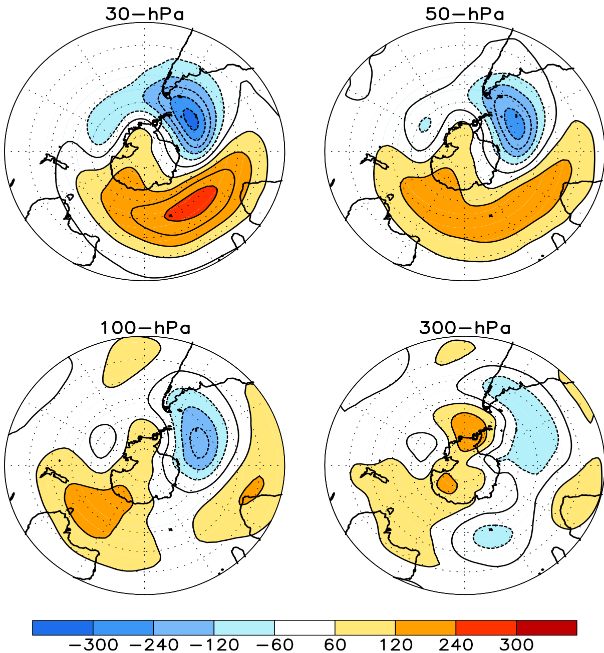
FIGURE S1. Stratospheric height anomalies (m) at selected levels for JUL 2020. Positive values are indicated by solid contours and dark shading. Negative values are indicated by dashed contours and light shading. Contour interval is 60 m. Anomalies are calculated from the 1981-2010 base period means. Winter Hemisphere is shown.
