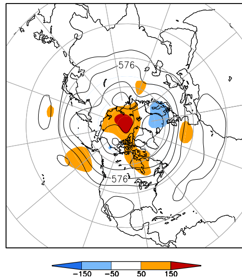
500-hPa Height (dm) & Anomalies (m) (Jul 1-31, 2020)
