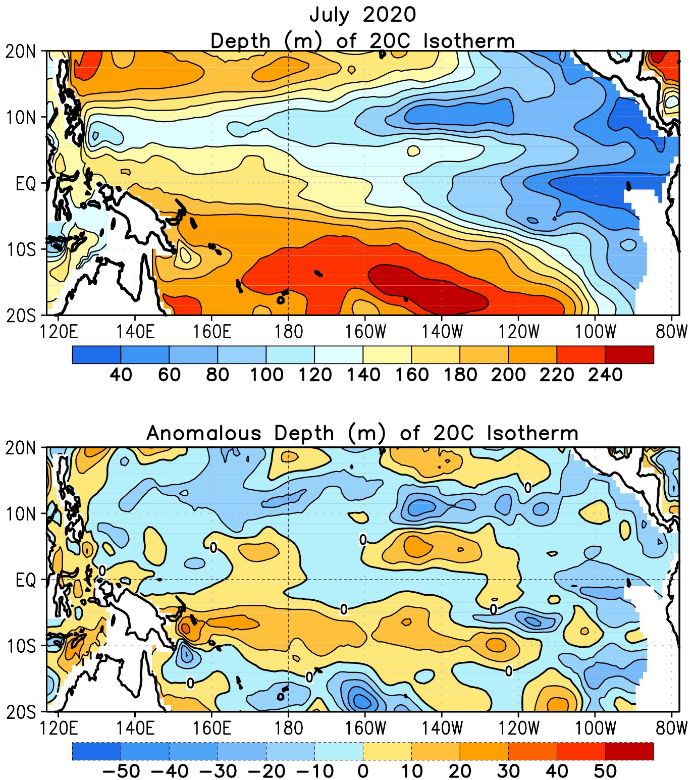
FIGURE T16. Mean (top) and anomalous (bottom) depth of the 20°C isotherm for JUL 2020. Contour interval is 40 m (top) and 10 m (bottom). Dashed contours in bottom panel indicate negative anomalies. Data are derived from the NCEP’s global ocean data assimilation system version 2 which assimilates oceanic observations into an oceanic GCM (Xue, Y. and Behringer, D.W., 2006: Operational global ocean data assimilation system at NCEP, to be submitted to BAMS). Anomalies are departures from the 1981–2010 base period means.
