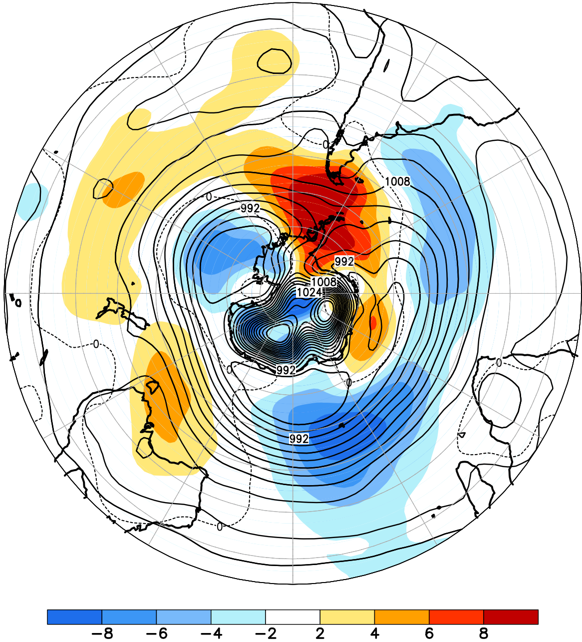
FIGURE E14. Southern Hemisphere mean and anomalous sea level pressure(CDAS/Reanalysis) for JUL 2020. Mean values are denoted by solid contours drawn at an interval of 4 hPa. Anomaly contour interval is 2 hPa with values less (greater) than -2 hPa (2 hPa) indicated by dark (light) shading. Anomalies are calculated as departures from the 1981-2010 base period monthly means.
