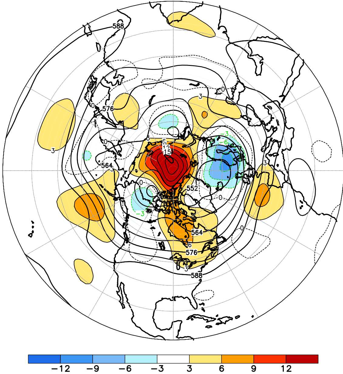
FIGURE E9. Northern Hemisphere mean and anomalous 500-hPa geopotential height (CDAS/Reanalysis) for JUL 2020. Mean heights are denoted by solid contours drawn at an interval of 6 dam. Anomaly contour interval is 3 dam with values less (greater) than -3 dam (3 dam) indicated by dark (light) shading. Anomalies are calculated as departures from the 1981-2010 base period monthly means.
