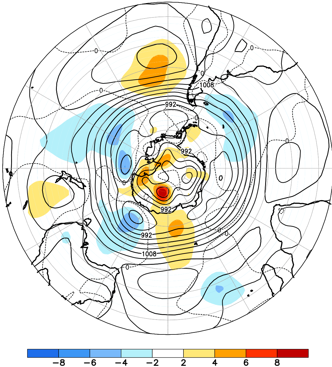
FIGURE E14. Southern Hemisphere mean and anomalous sea level pressure(CDAS/Reanalysis) for JAN 2020. Mean values are denoted by solid contours drawn at an interval of 4 hPa. Anomaly contour interval is 2 hPa with values less (greater) than -2 hPa (2 hPa) indicated by dark (light) shading. Anomalies are calculated as departures from the 1981-2010 base period monthly means.
