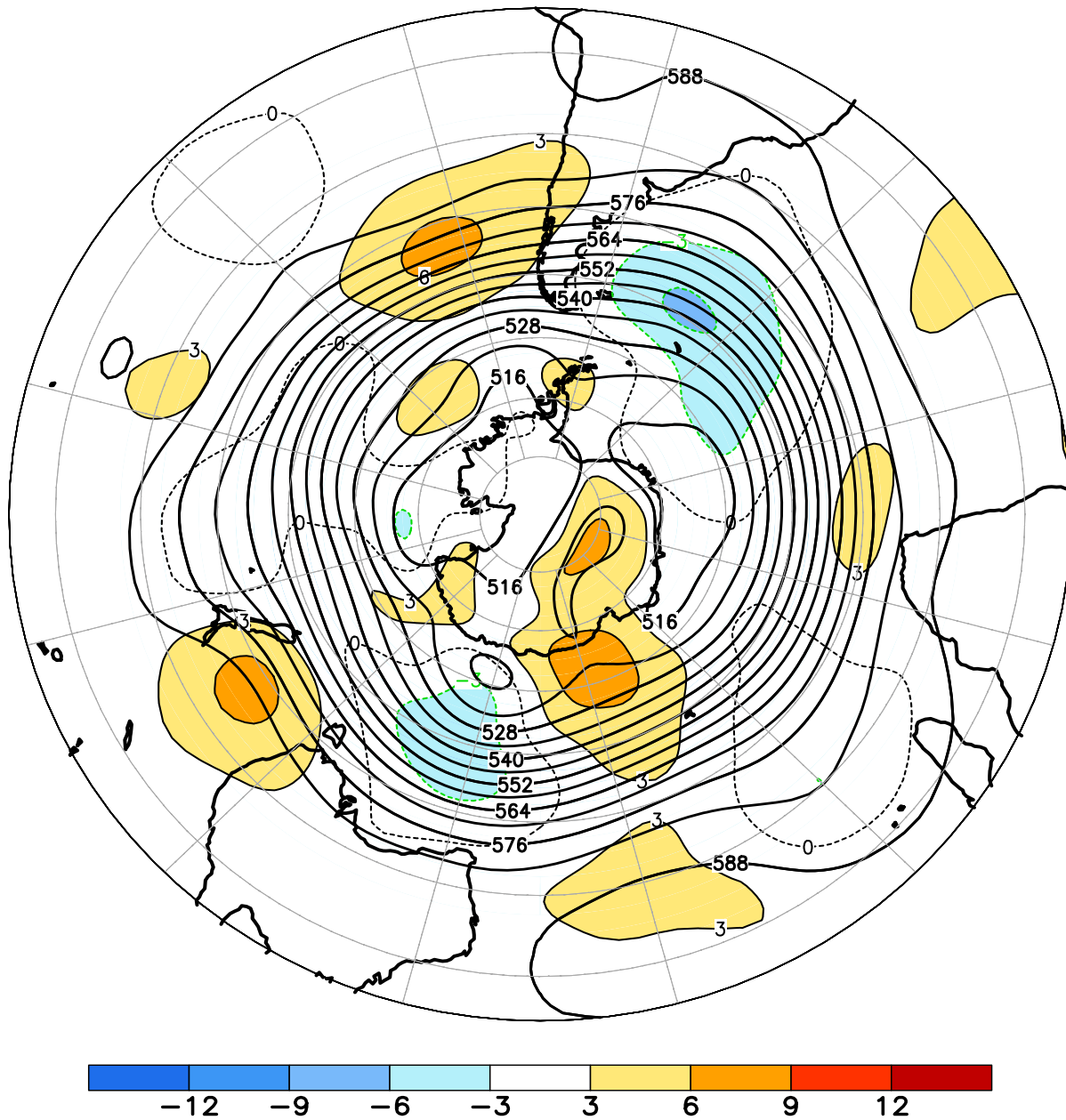
FIGURE E15. Southern Hemisphere mean and anomalous 500-hPa geopotential height (CDAS/Reanalysis) for JAN 2020. Mean heights are denoted by solid contours drawn at an interval of 6 dam. Anomaly contour interval is 3 dam with values less (greater) than -3 dam (3 dam) indicated by dark (light) shading. Anomalies are calculated as departures from the 1981-2010 base period monthly means.
