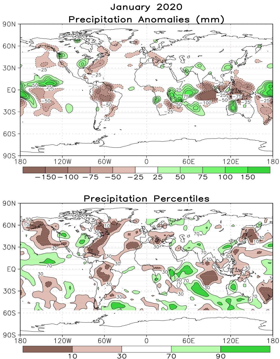
FIGURE E3. Anomalous precipitation (mm, top) and precipitation percentiles based on a Gamma distribution fit to the 1981–2010 base period data (bottom) for JAN 2020. Data are obtained from a merge of raingauge observations and satellite-derived precipitation estimates (Janowiak and Xie 1999, J. Climate , 12 , 3335–3342). Contours are drawn at 200, 100, 50, 25, -25, -50, -100, and -200 mm in top panel. Percentiles are not plotted in regions where mean monthly precipitation is <5mm/month.
