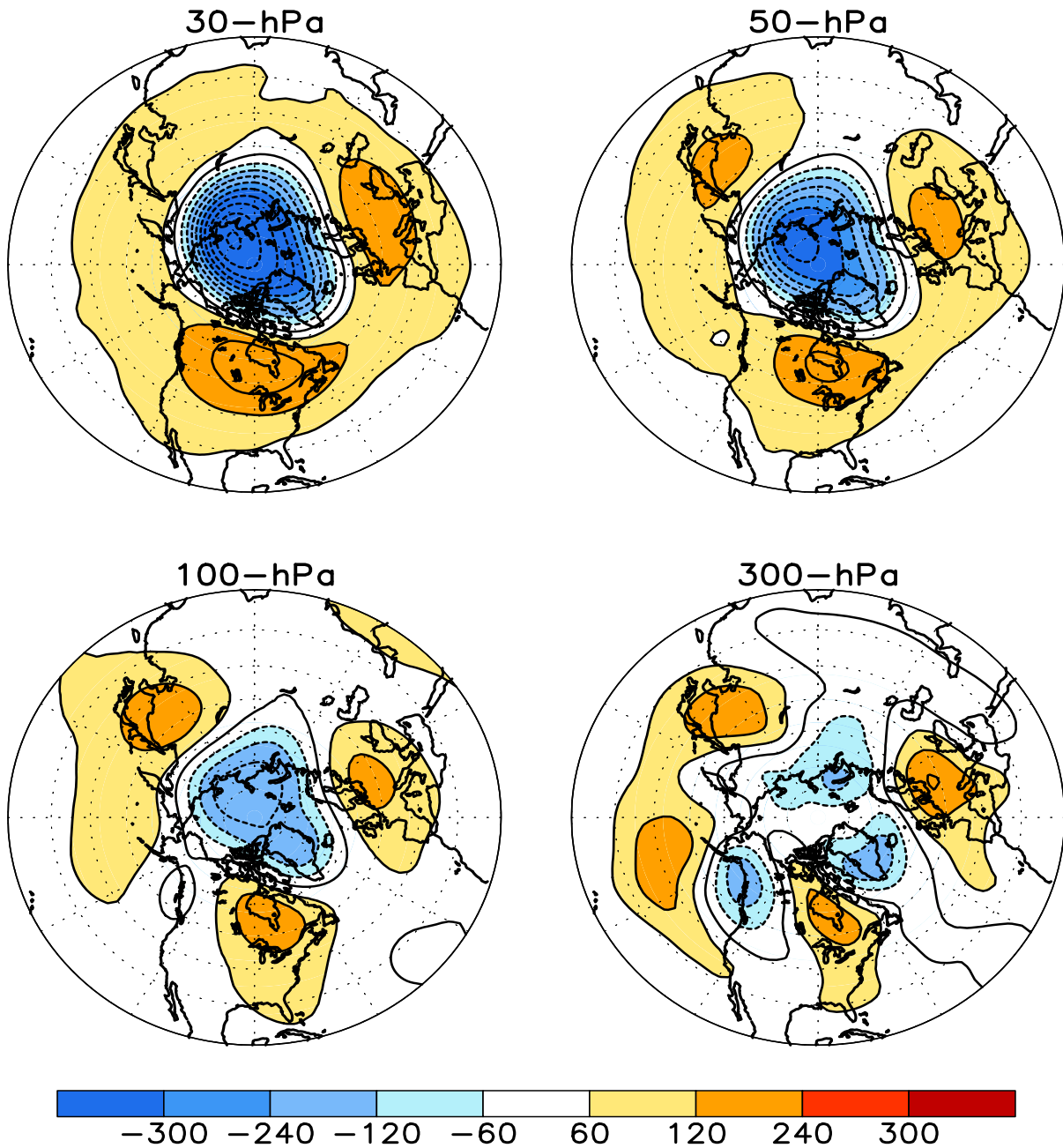
FIGURE S1. Stratospheric height anomalies (m) at selected levels for JAN 2020. Positive values are indicated by solid contours and dark shading. Negative values are indicated by dashed contours and light shading. Contour interval is 60 m. Anomalies are calculated from the 1981-2010 base period means. Winter Hemisphere is shown.
