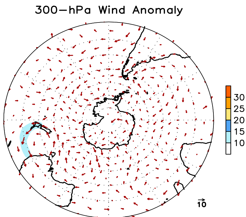
FIGURE E16. Southern Hemisphere mean (left) and anomalous (right) 300-hPa vector wind (CDAS/Reanalysis) for JAN 2020. Mean (anomaly) isotach contour interval is 10 (5) \text{ms}^{-1} . Values greater than 30 \text{ms}^{-1} (left) and 10 \text{ms}^{-1} (rights) are shaded. Anomalies are departures from the 1981-2010 base period monthly means.
