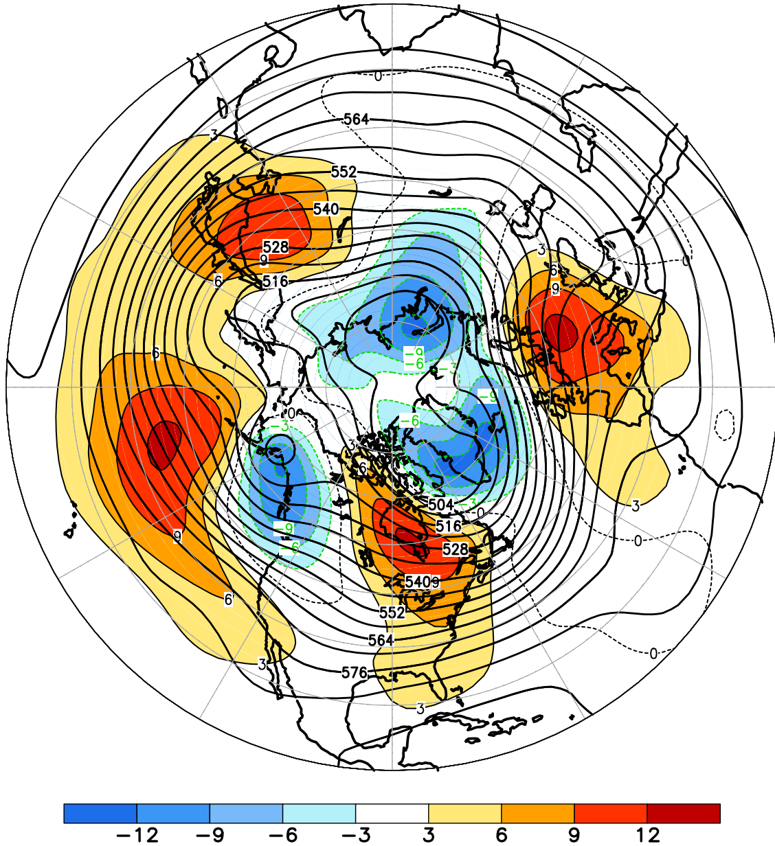
FIGURE E9. Northern Hemisphere mean and anomalous 500-hPa geopotential height (CDAS/Reanalysis) for JAN 2020. Mean heights are denoted by solid contours drawn at an interval of 6 dam. Anomaly contour interval is 3 dam with values less (greater) than -3 dam (3 dam) indicated by dark (light) shading. Anomalies are calculated as departures from the 1981-2010 base period monthly means.
