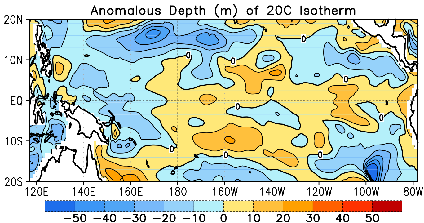
FIGURE T16. Mean (top) and anomalous (bottom) depth of the 20°C isotherm for JAN 2020. Contour interval is 40 m (top) and 10 m (bottom). Dashed contours in bottom panel indicate negative anomalies. Data are derived from the NCEP's global ocean data assimilation system version 2 which assimilates oceanic observations into an oceanic GCM (Xue, Y. and Behringer, D.W., 2006: Operational global ocean data assimilation system at NCEP, to be submitted to BAMS). Anomalies are departures from the 1981–2010 base period means.
