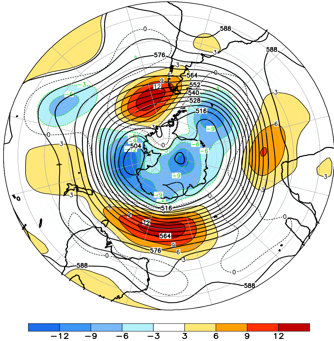
FIGURE E15. Southern Hemisphere mean and anomalous 500-hPa geopotential height (CDAS/Reanalysis) for JAN 2016. Mean heights are denoted by solid contours drawn at an interval of 6 dam. Anomaly contour interval is 3 dam with values less (greater) than -3 dam (3 dam) indicated by dark (light) shading. Anomalies are calculated as departures from the 1981-2010 base period monthly means.
