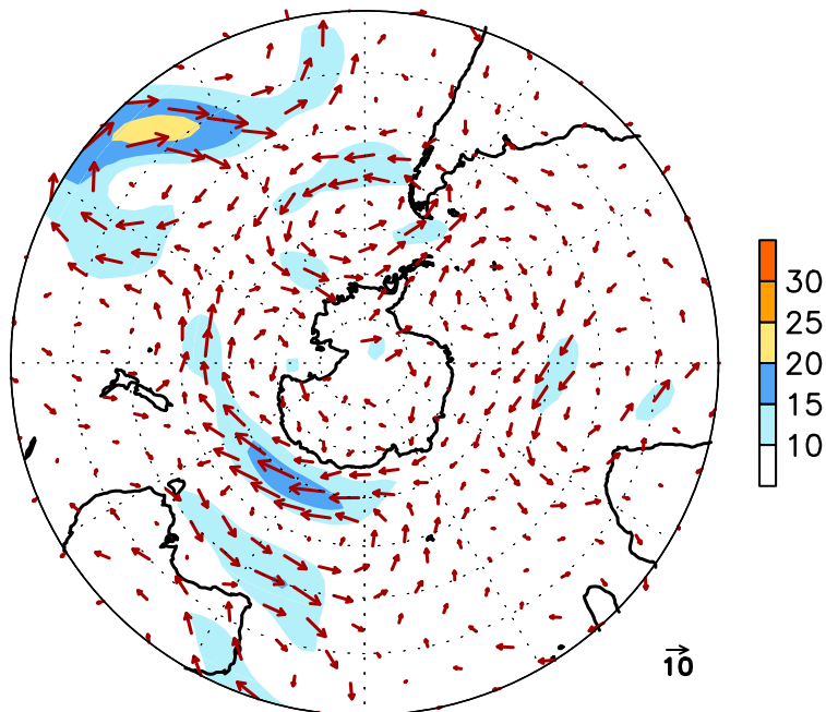
FIGURE E16. Southern Hemisphere mean (left) and anomalous (right) 300-hPa vector wind (CDAS/Reanalysis) for JAN 2016. Mean (anomaly) isotach contour interval is 10 (5) \text{ms}^{-1} . Values greater than 30 \text{ms}^{-1} (left) and 10 \text{ms}^{-1} (rights) are shaded. Anomalies are departures from the 1981-2010 base period monthly means.
