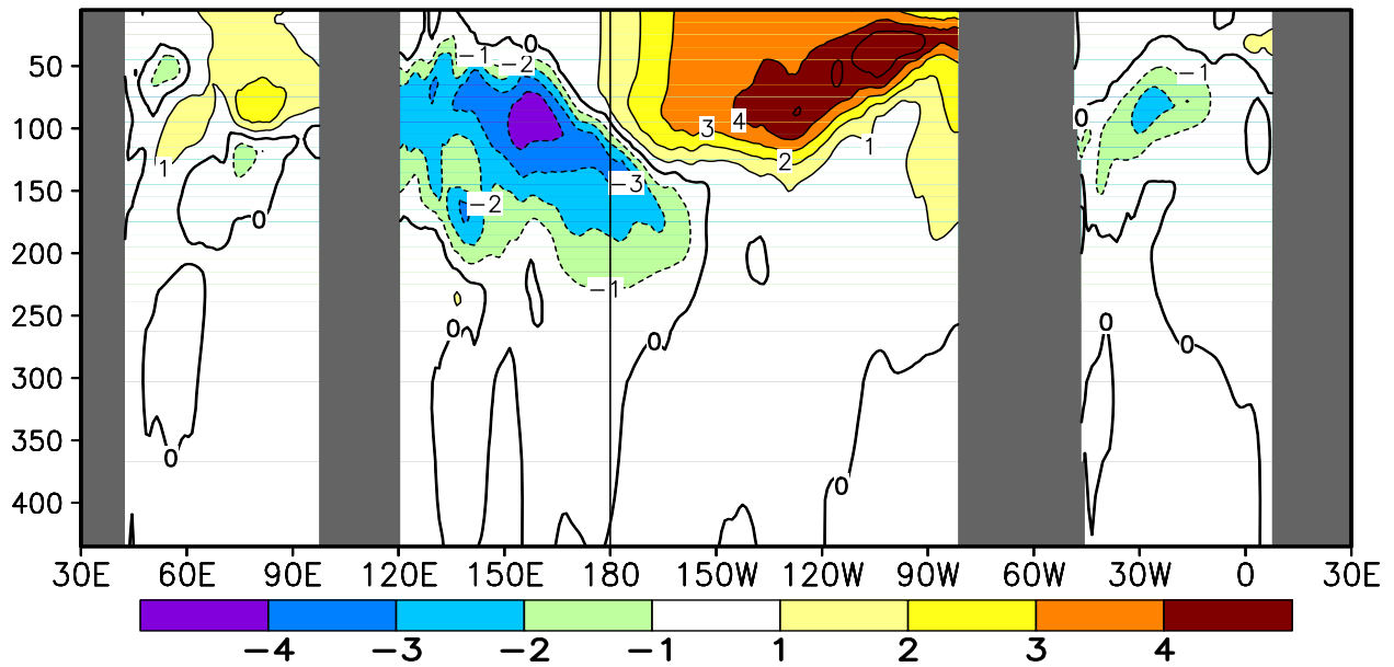
FIGURE T17. Equatorial depth–longitude section of ocean temperature (top) and ocean temperature anomalies (bottom) for JAN 2016. Contour interval is 1°C. Dashed contours in bottom panel indicate negative anomalies. Data are derived from the NCEP’s global ocean data assimilation system version 2 which assimilates oceanic observations into an oceanic GCM (Xue, Y. and Behringer, D.W., 2006: Operational global ocean data assimilation system at NCEP, to be submitted to BAMS). Anomalies are departures from the 1981–2010 base period means.
