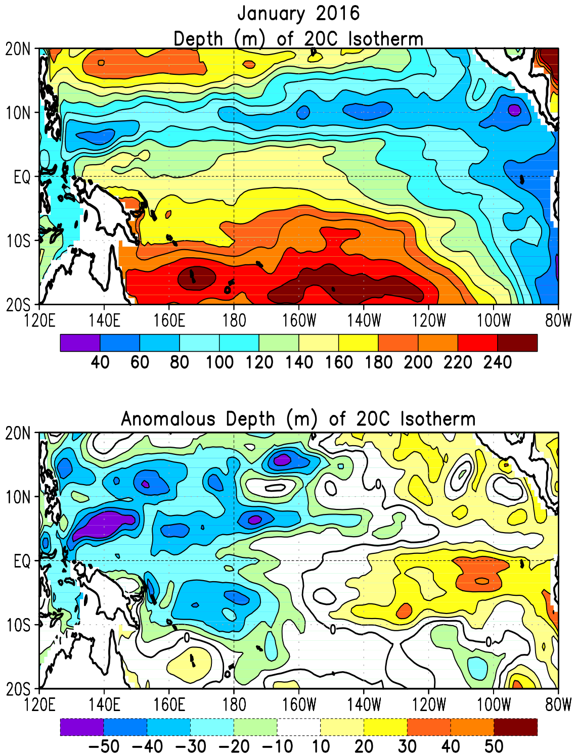
FIGURE T16. Mean (top) and anomalous (bottom) depth of the 20°C isotherm for JAN 2016. Contour interval is 40 m (top) and 10 m (bottom). Dashed contours in bottom panel indicate negative anomalies. Data are derived from the NCEP's global ocean data assimilation system version 2 which assimilates oceanic observations into an oceanic GCM (Xue, Y. and Behringer, D.W., 2006: Operational global ocean data assimilation system at NCEP, to be submitted to BAMS). Anomalies are departures from the 1981–2010 base period means.
