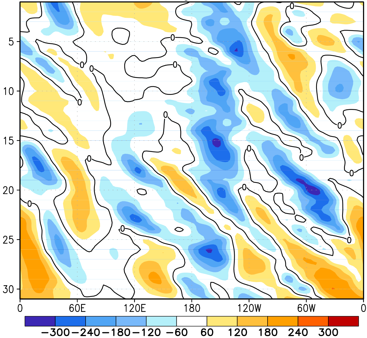
FIGURE E12. Northern Hemisphere: Daily 500-hPa height anomalies for JAN 2016 averaged over the 5° latitude band centered on 40°N. Positive values are indicated by solid contours and dark shading. Negative values are indicated by dashed contours and light shading. Contour interval is 60 m. Anomalies are departures from the 1981-2010 base period daily means.
