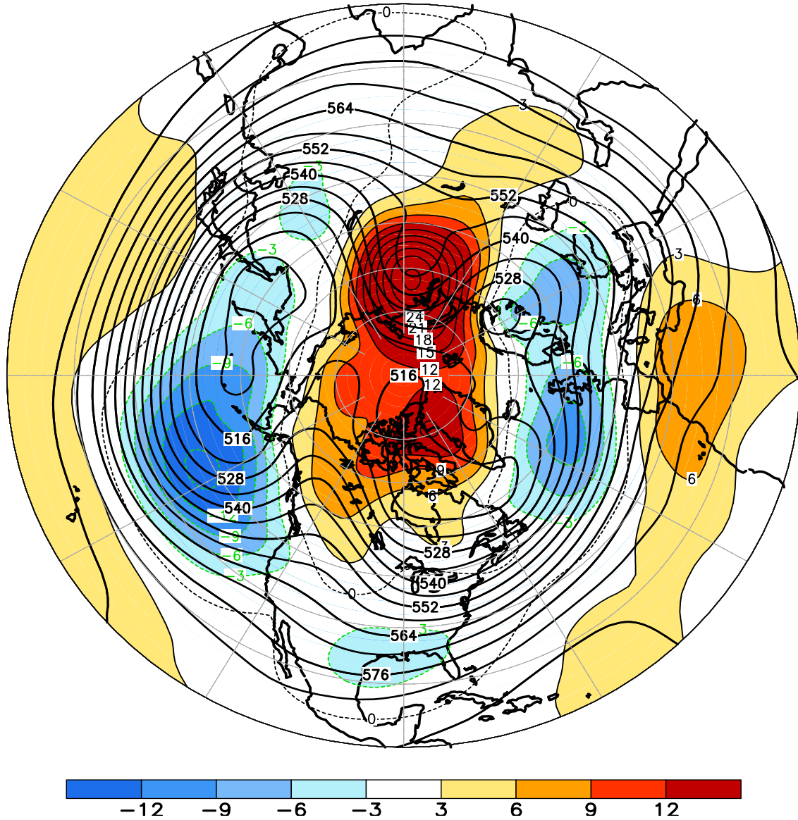
FIGURE E9. Northern Hemisphere mean and anomalous 500-hPa geopotential height (CDAS/Reanalysis) for JAN 2016. Mean heights are denoted by solid contours drawn at an interval of 6 dam. Anomaly contour interval is 3 dam with values less (greater) than -3 dam (3 dam) indicated by dark (light) shading. Anomalies are calculated as departures from the 1981-2010 base period monthly means.
