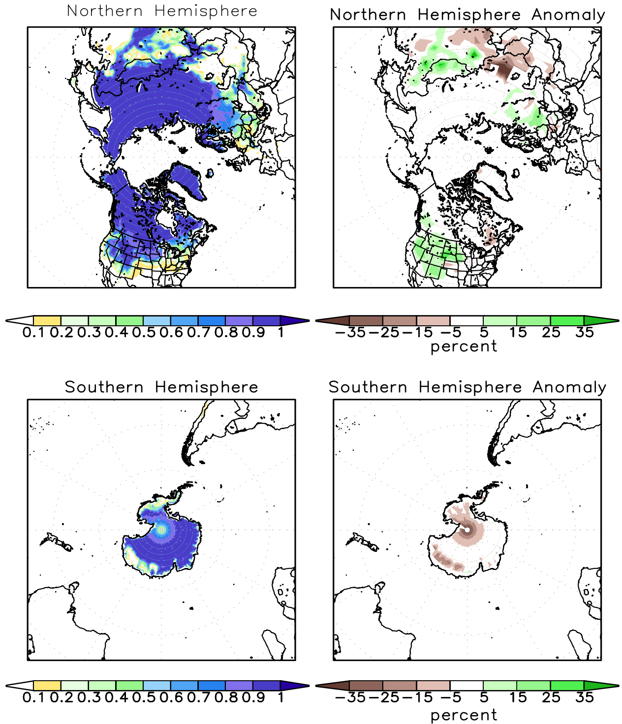
FIGURE A2.2. SSM/I derived snow cover frequency (%) (left) and snow cover anomaly (%) (right) for the month of JAN 2016 based on 1987 - 2010 base period for the Northern Hemisphere (top) and Southern Hemisphere (bottom). It is generated using the algorithm described by Ferraro et. al, 1996, Bull. Amer. Meteor. Soc., vol 77, 891-905.
