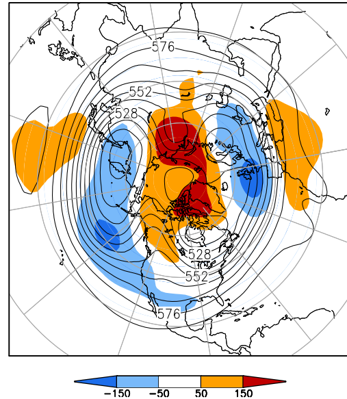
500-hPa Height (dm) & Anomalies (m) (Jan 1–15, 2016)
