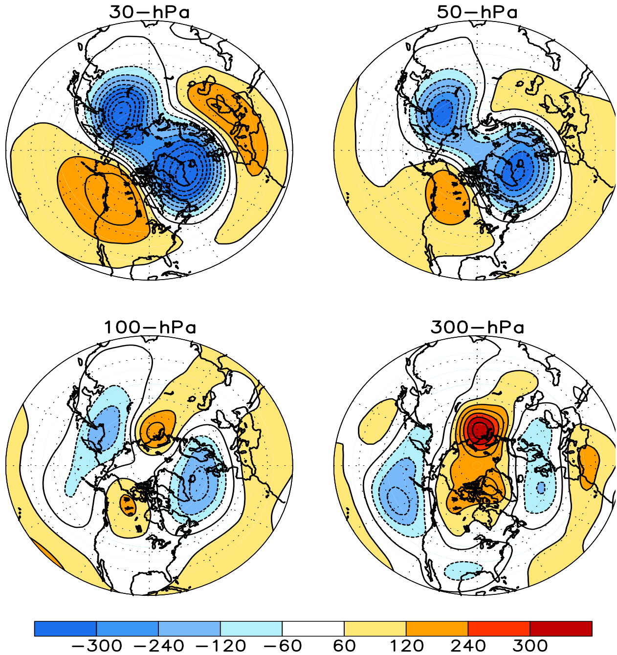
FIGURE S1. Stratospheric height anomalies (m) at selected levels for JAN 2016. Positive values are indicated by solid contours and dark shading. Negative values are indicated by dashed contours and light shading. Contour interval is 60 m. Anomalies are calculated from the 1981-2010 base period means. Winter Hemisphere is shown.
