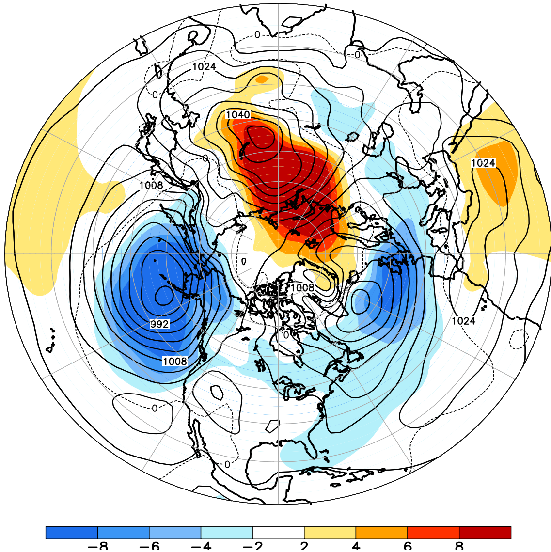
FIGURE E8. Northern Hemisphere mean and anomalous sea level pressure (CDAS/Reanalysis) for JAN 2016. Mean values are denoted by solid contours drawn at an interval of 4 hPa. Anomaly contour interval is 2 hPa with values less (greater) than -2 hPa (2 hPa) indicated by dark (light) shading. Anomalies are calculated as departures from the 1981-2010 base period monthly means.
