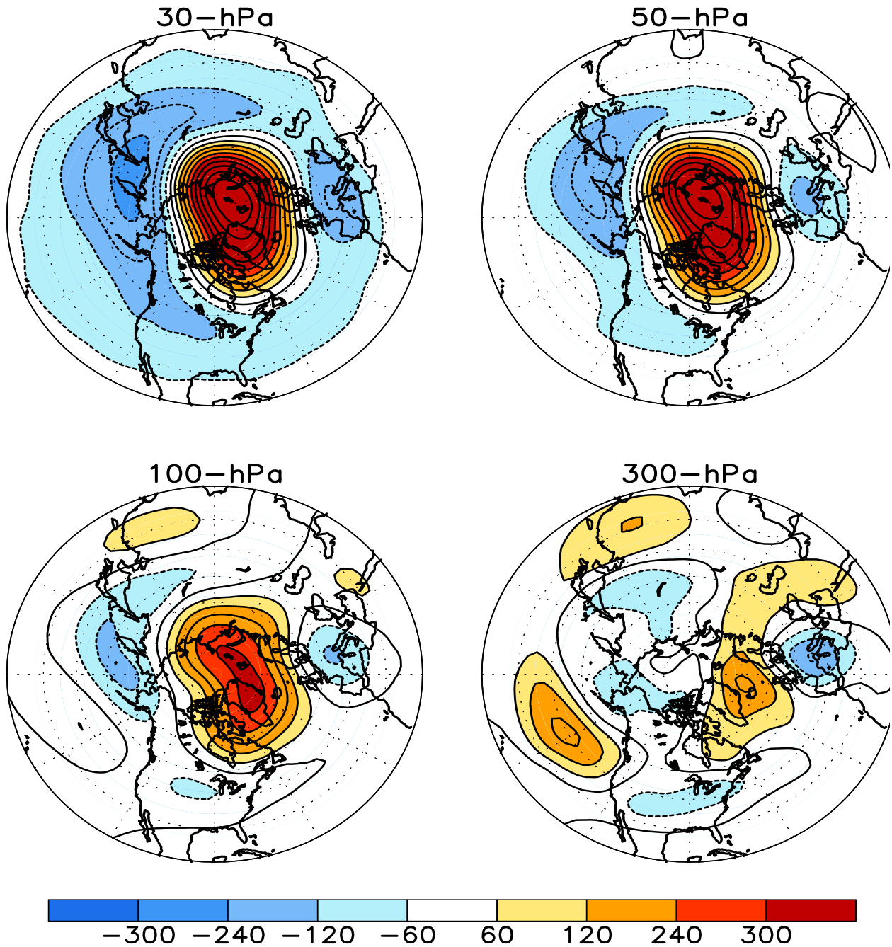
FIGURE S1. Stratospheric height anomalies (m) at selected levels for FEB 2013. Positive values are indicated by solid contours and dark shading. Negative values are indicated by dashed contours and light shading. Contour interval is 60 m. Anomalies are calculated from the 1981-2010 base period means. Winter Hemisphere is shown.
