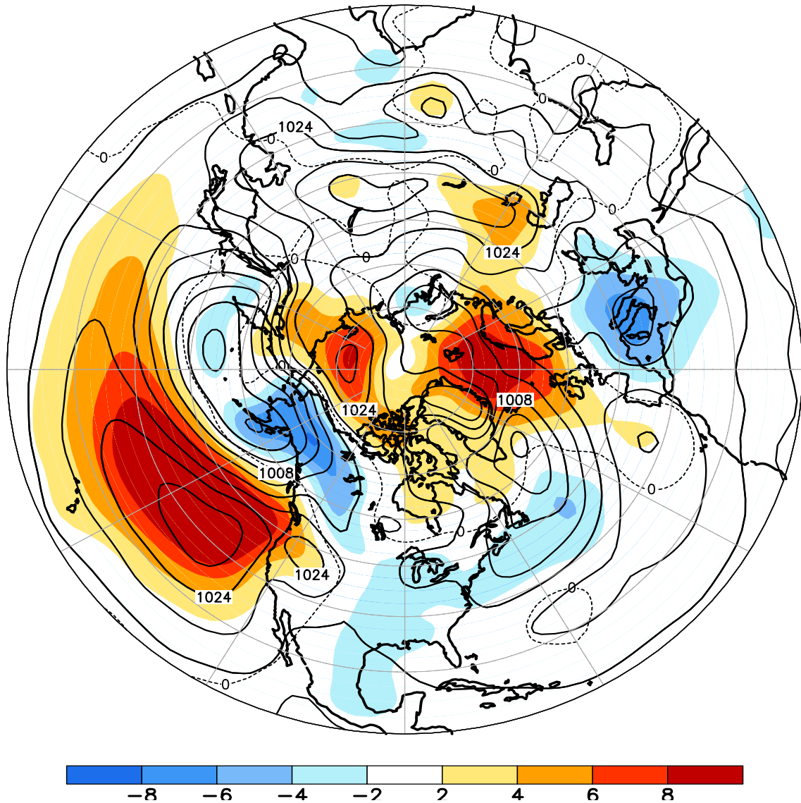
FIGURE E8. Northern Hemisphere mean and anomalous sea level pressure (CDAS/Reanalysis) for FEB 2013. Mean values are denoted by solid contours drawn at an interval of 4 hPa. Anomaly contour interval is 2 hPa with values less (greater) than -2 hPa (2 hPa) indicated by dark (light) shading. Anomalies are calculated as departures from the 1981-2010 base period monthly means.
