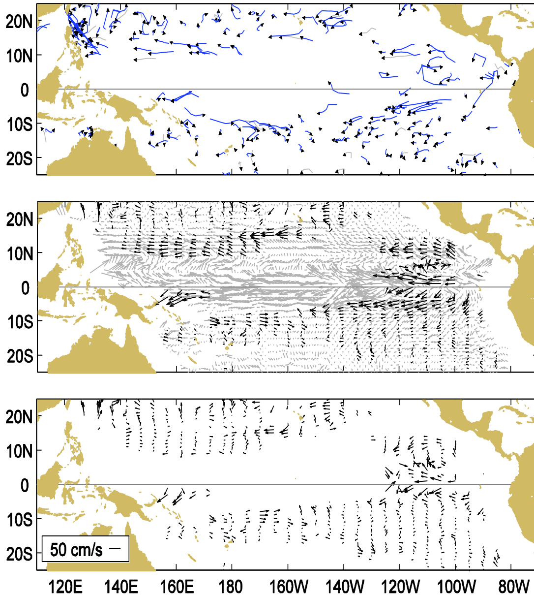
Figure A1.1 Top: Movements of drifting buoys in the tropical Pacific Ocean during February 2013. The linear segments of each trajectory represent a one week displacement. Trajectories of buoys which have lost their subsurface drogues are gray; those with drogues are black.
