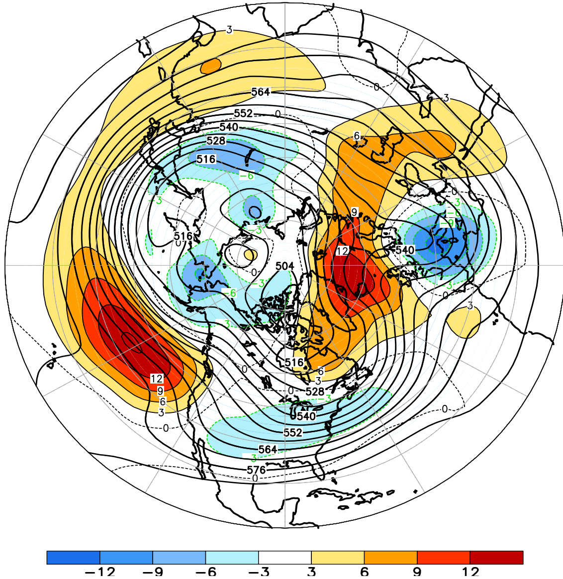
FIGURE E9. Northern Hemisphere mean and anomalous 500-hPa geopotential height (CDAS/Reanalysis) for FEB 2013. Mean heights are denoted by solid contours drawn at an interval of 6 dam. Anomaly contour interval is 3 dam with values less (greater) than -3 dam (3 dam) indicated by dark (light) shading. Anomalies are calculated as departures from the 1981-2010 base period monthly means.
