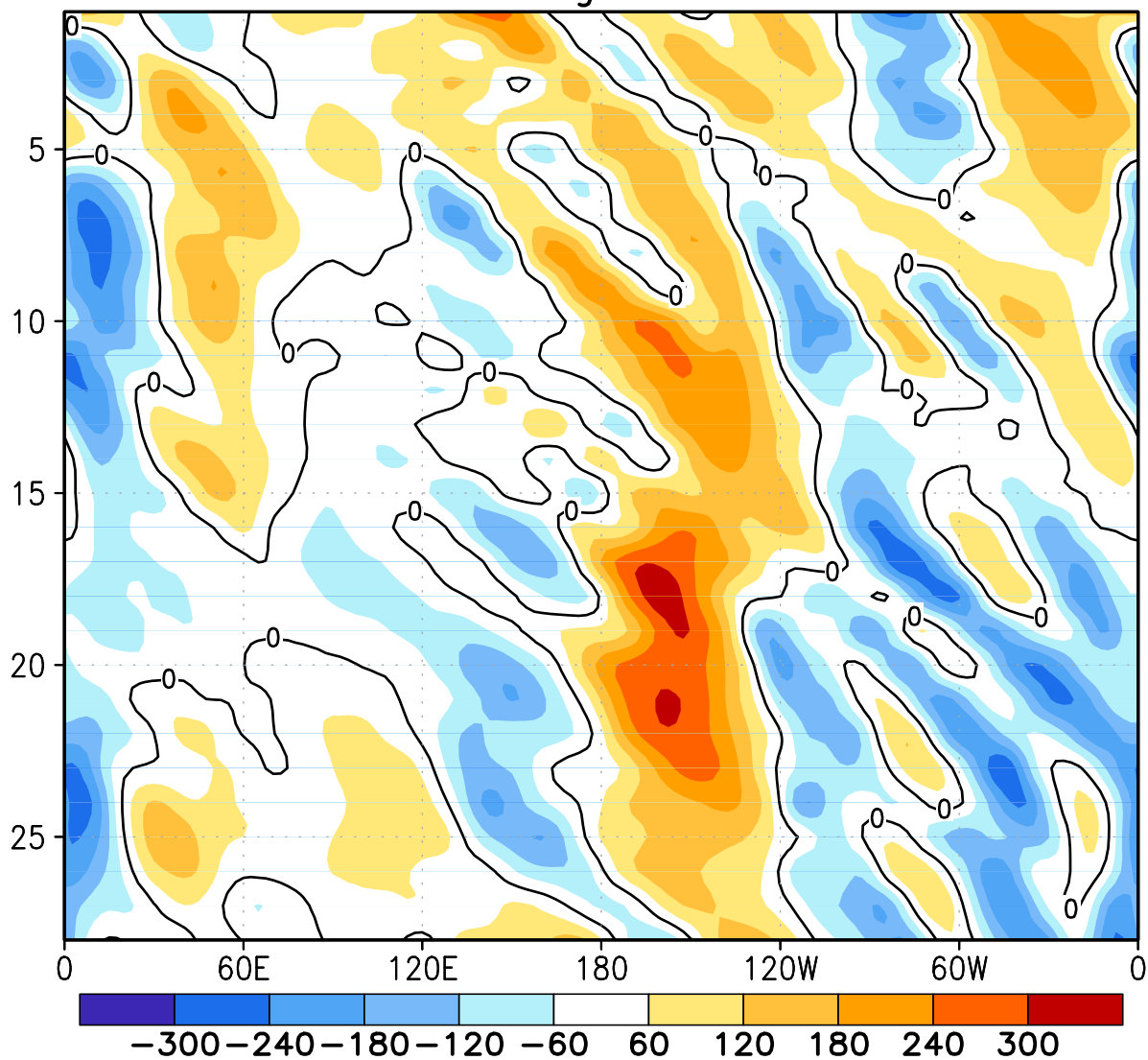
FIGURE E12. Northern Hemisphere: Daily 500-hPa height anomalies for FEB 2013 averaged over the 5° latitude band centered on 40°N. Positive values are indicated by solid contours and dark shading. Negative values are indicated by dashed contours and light shading. Contour interval is 60 m. Anomalies are departures from the 1981-2010 base period daily means.
