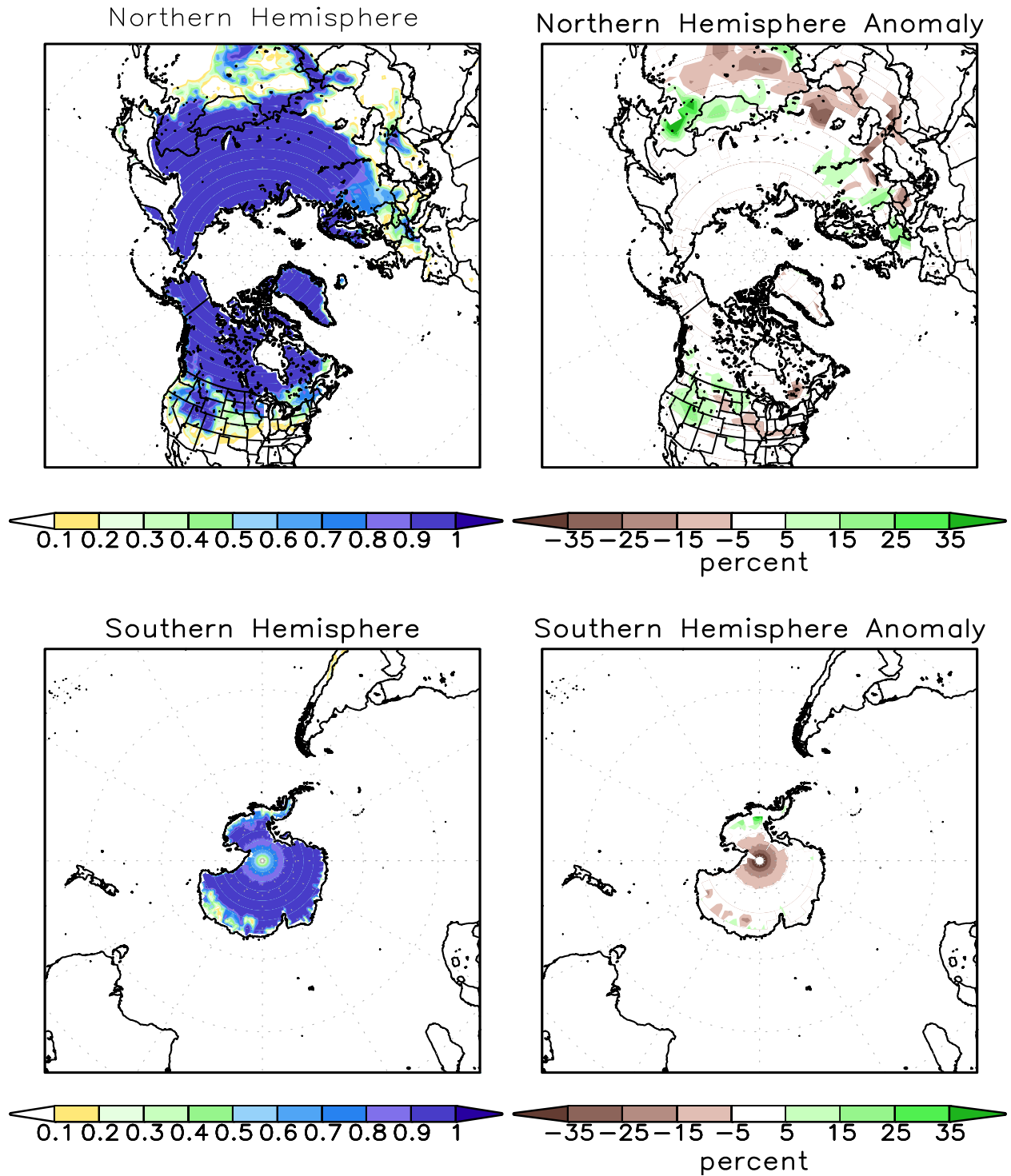
FIGURE A2.2. SSM/I derived snow cover frequency (%) (left) and snow cover anomaly (%) (right) for the month of FEB 2013 based on 1987 - 2010 base period for the Northern Hemisphere (top) and Southern Hemisphere (bottom). It is generated using the algorithm described by Ferraro et. al, 1996, Bull. Amer. Meteor. Soc., vol 77, 891-905.
