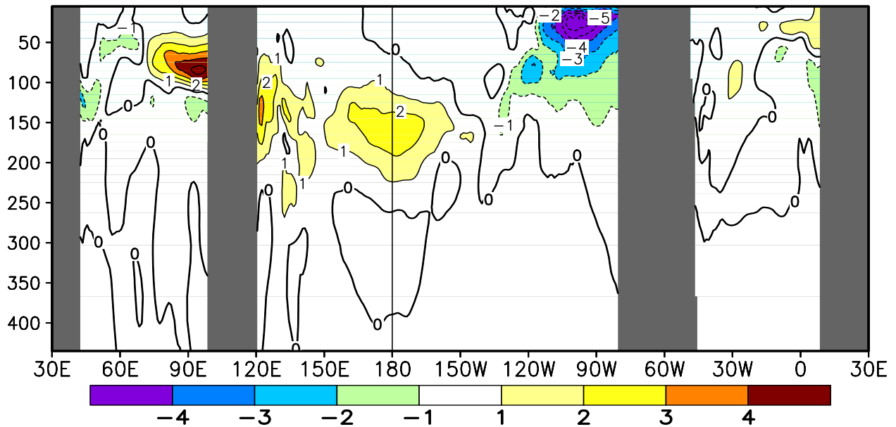
FIGURE T17. Equatorial depth–longitude section of ocean temperature (top) and ocean temperature anomalies (bottom) for FEB 2013. Contour interval is 1°C. Dashed contours in bottom panel indicate negative anomalies. Data are derived from the NCEP’s global ocean data assimilation system version 2 which assimilates oceanic observations into an oceanic GCM (Xue, Y. and Behringer, D.W., 2006: Operational global ocean data assimilation system at NCEP, to be submitted to BAMS). Anomalies are departures from the 1981–2010 base period means.
