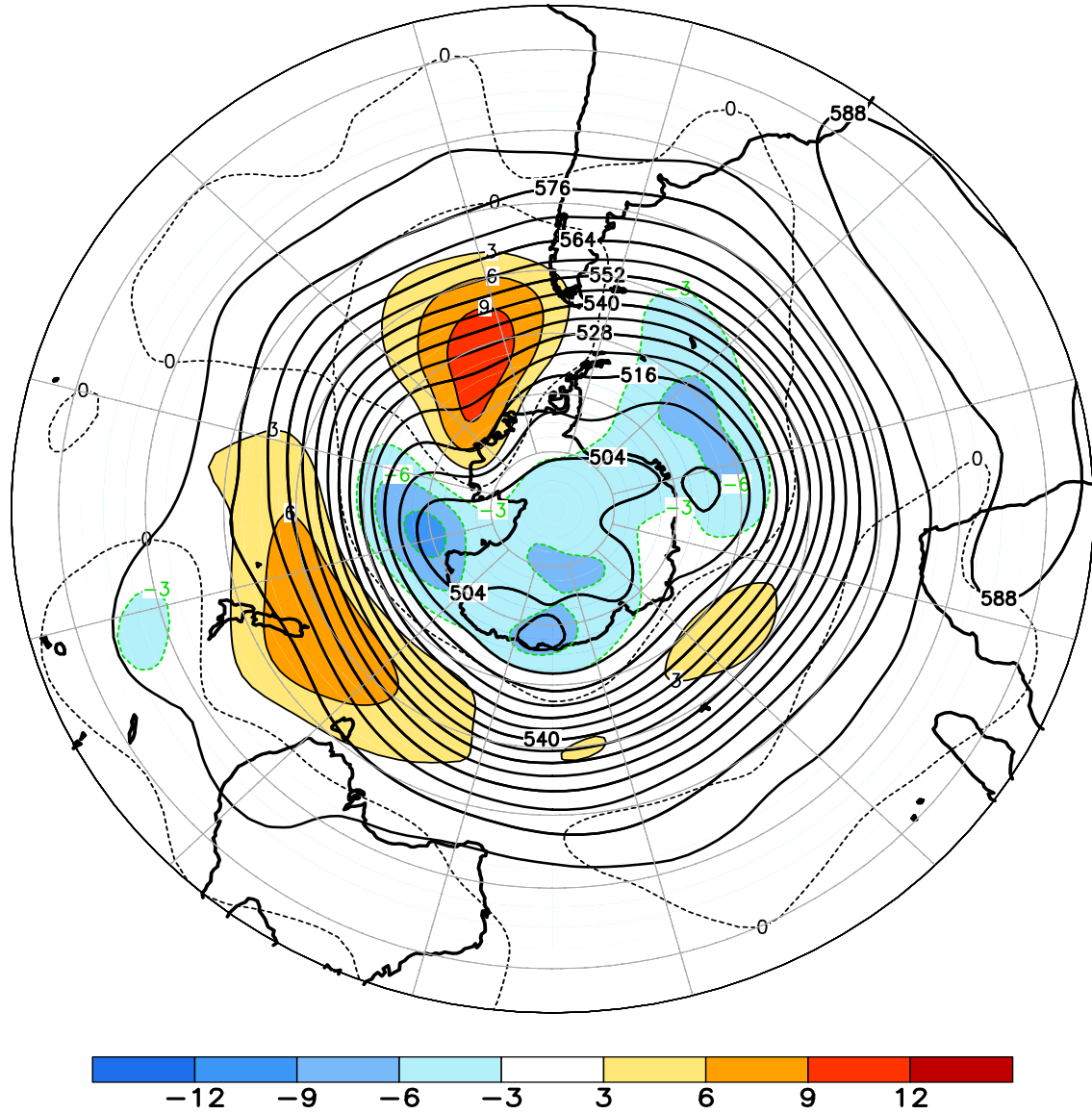
FIGURE E15. Southern Hemisphere mean and anomalous 500-hPa geopotential height (CDAS/Reanalysis) for FEB 2013. Mean heights are denoted by solid contours drawn at an interval of 6 dam. Anomaly contour interval is 3 dam with values less (greater) than -3 dam (3 dam) indicated by dark (light) shading. Anomalies are calculated as departures from the 1981-2010 base period monthly means.
