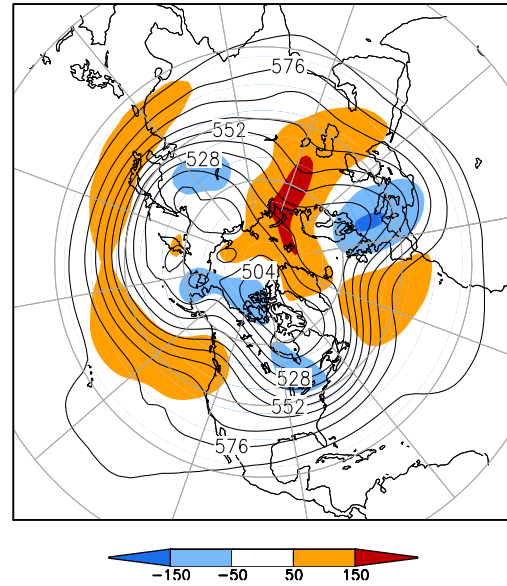
500-hPa Height (dm) & Anomalies (m) (Feb 1–15, 2013)
