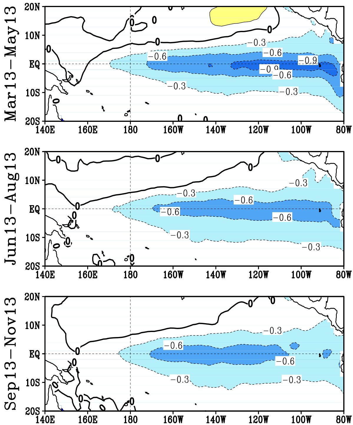
FIGURE F5. Predicted 3-month average sea surface temperature anomalies from the NCEP/CPC Markov model (Xue et al. 2000, J. Climate , 13 , 849-871). The forecast is initiated in FEB 2013 . Contour interval is 0.3C and negative anomalies are indicated by dashed contours. Anomalies are calculated relative to the 1971-2000 climatology.
