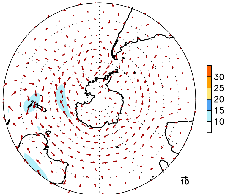
FIGURE E16. Southern Hemisphere mean (left) and anomalous (right) 300-hPa vector wind (CDAS/Reanalysis) for FEB 2013. Mean (anomaly) isotach contour interval is 10 (5) \text{ms}^{-1} . Values greater than 30 \text{ms}^{-1} (left) and 10 \text{ms}^{-1} (rights) are shaded. Anomalies are departures from the 1981-2010 base period monthly means.
