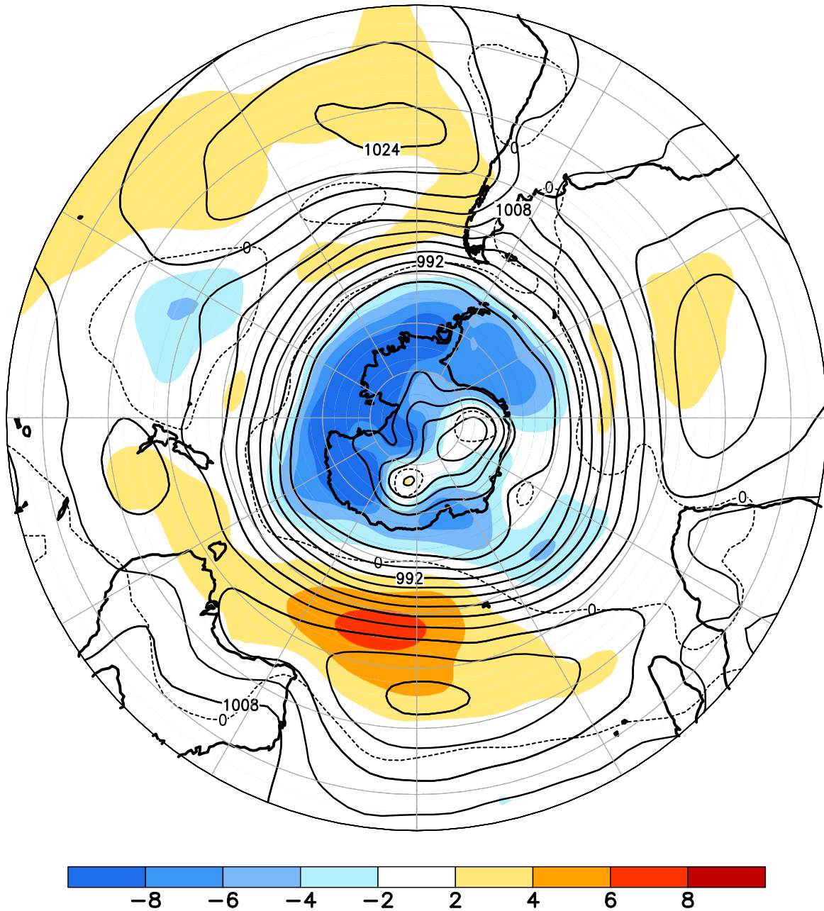
FIGURE E14. Southern Hemisphere mean and anomalous sea level pressure(CDAS/Reanalysis) for DEC 2020. Mean values are denoted by solid contours drawn at an interval of 4 hPa. Anomaly contour interval is 2 hPa with values less (greater) than -2 hPa (2 hPa) indicated by dark (light) shading. Anomalies are calculated as departures from the 1981-2010 base period monthly means.
