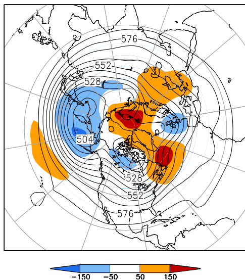
500-hPa Height (dm) & Anomalies (m) (Dec 16–31, 2020)
