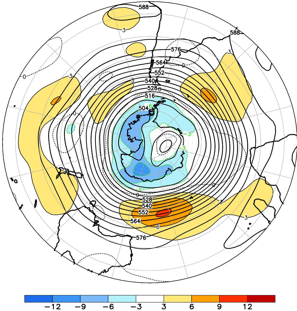
FIGURE E15. Southern Hemisphere mean and anomalous 500-hPa geopotential height (CDAS/Reanalysis) for DEC 2020. Mean heights are denoted by solid contours drawn at an interval of 6 dam. Anomaly contour interval is 3 dam with values less (greater) than -3 dam (3 dam) indicated by dark (light) shading. Anomalies are calculated as departures from the 1981-2010 base period monthly means.
