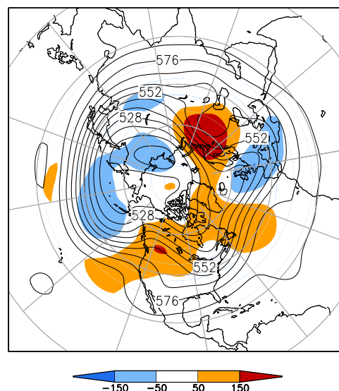
500-hPa Height (dm) & Anomalies (m) (Dec 1–15, 2020)
