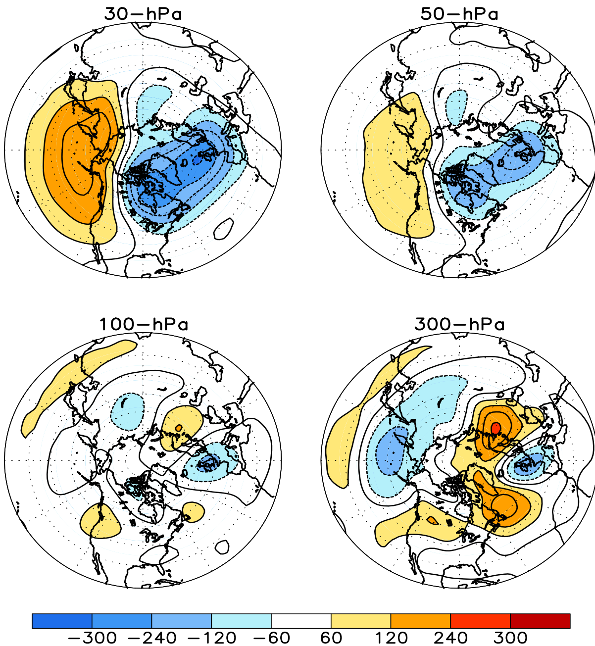
FIGURE S1. Stratospheric height anomalies (m) at selected levels for DEC 2020. Positive values are indicated by solid contours and dark shading. Negative values are indicated by dashed contours and light shading. Contour interval is 60 m. Anomalies are calculated from the 1981-2010 base period means. Winter Hemisphere is shown.
