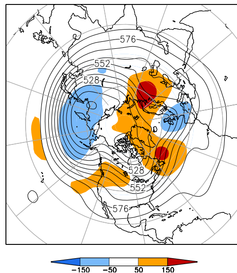
500-hPa Height (dm) & Anomalies (m) (Dec 1–31, 2020)
