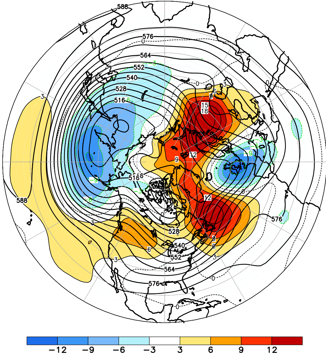
FIGURE E9. Northern Hemisphere mean and anomalous 500-hPa geopotential height (CDAS/Reanalysis) for DEC 2020. Mean heights are denoted by solid contours drawn at an interval of 6 dam. Anomaly contour interval is 3 dam with values less (greater) than -3 dam (3 dam) indicated by dark (light) shading. Anomalies are calculated as departures from the 1981-2010 base period monthly means.
