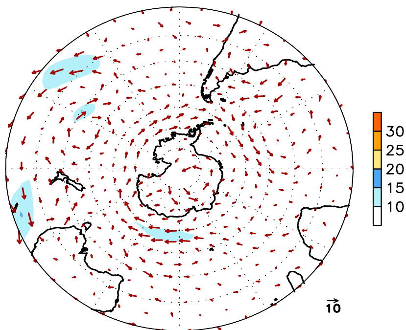
FIGURE E16. Southern Hemisphere mean (left) and anomalous (right) 300-hPa vector wind (CDAS/Reanalysis) for DEC 2020. Mean (anomaly) isotach contour interval is 10 (5) \text{ms}^{-1} . Values greater than 30 \text{ms}^{-1} (left) and 10 \text{ms}^{-1} (rights) are shaded. Anomalies are departures from the 1981-2010 base period monthly means.
