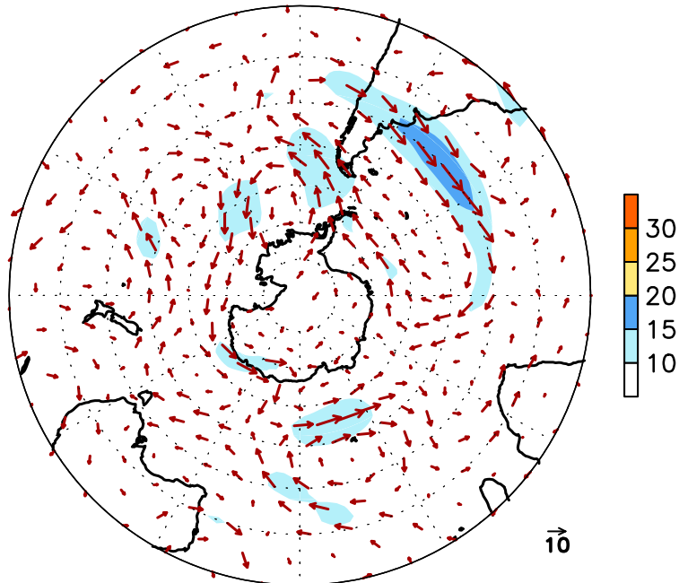
FIGURE E16. Southern Hemisphere mean (left) and anomalous (right) 300-hPa vector wind (CDAS/Reanalysis) for DEC 2012. Mean (anomaly) isotach contour interval is 10 (5) \text{ms}^{-1} . Values greater than 30 \text{ms}^{-1} (left) and 10 \text{ms}^{-1} (rights) are shaded. Anomalies are departures from the 1981-2010 base period monthly means.
