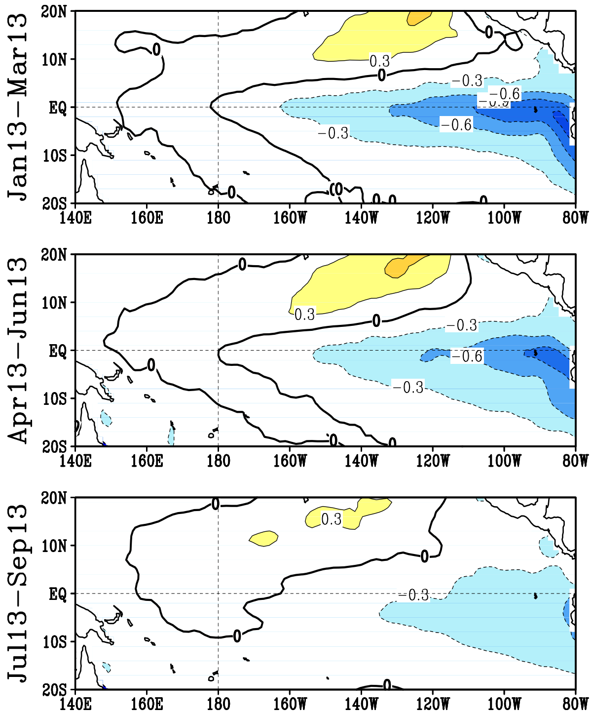
FIGURE F5. Predicted 3-month average sea surface temperature anomalies from the NCEP/CPC Markov model (Xue et al. 2000, J. Climate , 13 , 849-871). The forecast is initiated in DEC 2012 . Contour interval is 0.3C and negative anomalies are indicated by dashed contours. Anomalies are calculated relative to the 1971-2000 climatology.
