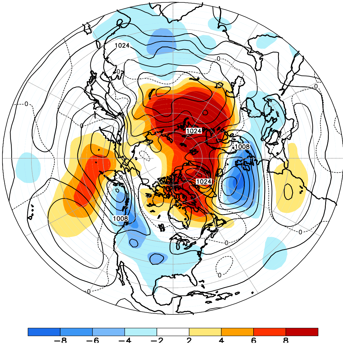
FIGURE E8. Northern Hemisphere mean and anomalous sea level pressure (CDAS/Reanalysis) for DEC 2012. Mean values are denoted by solid contours drawn at an interval of 4 hPa. Anomaly contour interval is 2 hPa with values less (greater) than -2 hPa (2 hPa) indicated by dark (light) shading. Anomalies are calculated as departures from the 1981-2010 base period monthly means.
