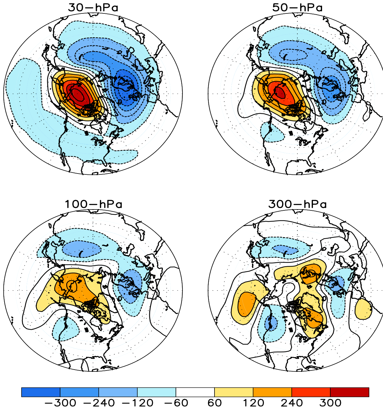
FIGURE S1. Stratospheric height anomalies (m) at selected levels for DEC 2012. Positive values are indicated by solid contours and dark shading. Negative values are indicated by dashed contours and light shading. Contour interval is 60 m. Anomalies are calculated from the 1981-2010 base period means. Winter Hemisphere is shown.
