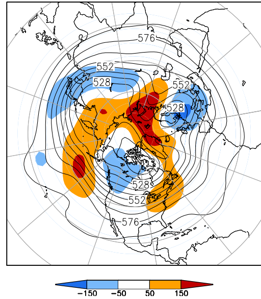
500-hPa Height (dm) & Anomalies (m) (Dec 1–15, 2012)
