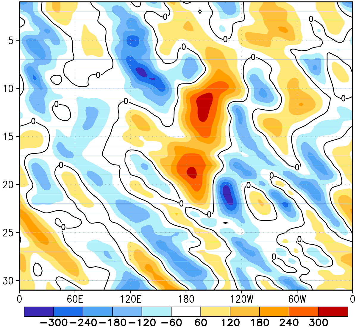
FIGURE E12. Northern Hemisphere: Daily 500-hPa height anomalies for DEC 2012 averaged over the 5° latitude band centered on 40°N. Positive values are indicated by solid contours and dark shading. Negative values are indicated by dashed contours and light shading. Contour interval is 60 m. Anomalies are departures from the 1981-2010 base period daily means.
