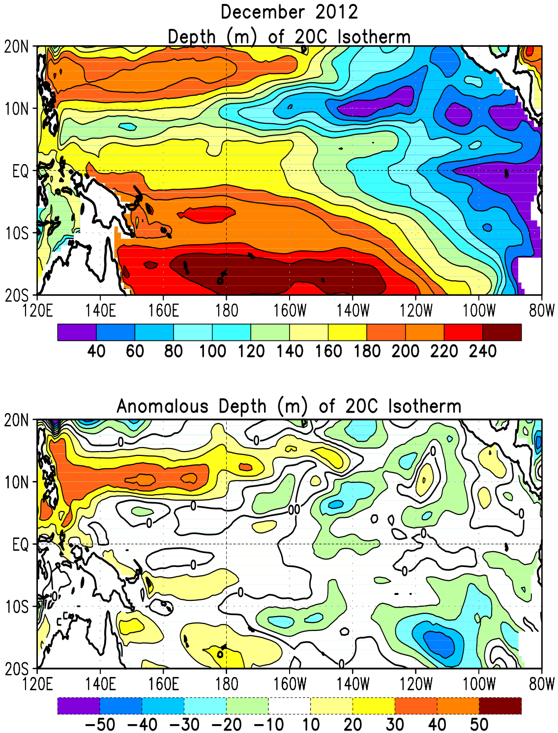
FIGURE T16. Mean (top) and anomalous (bottom) depth of the 20°C isotherm for DEC 2012. Contour interval is 40 m (top) and 10 m (bottom). Dashed contours in bottom panel indicate negative anomalies. Data are derived from the NCEP's global ocean data assimilation system version 2 which assimilates oceanic observations into an oceanic GCM (Xue, Y. and Behringer, D.W., 2006: Operational global ocean data assimilation system at NCEP, to be submitted to BAMS). Anomalies are departures from the 1981–2010 base period means.
