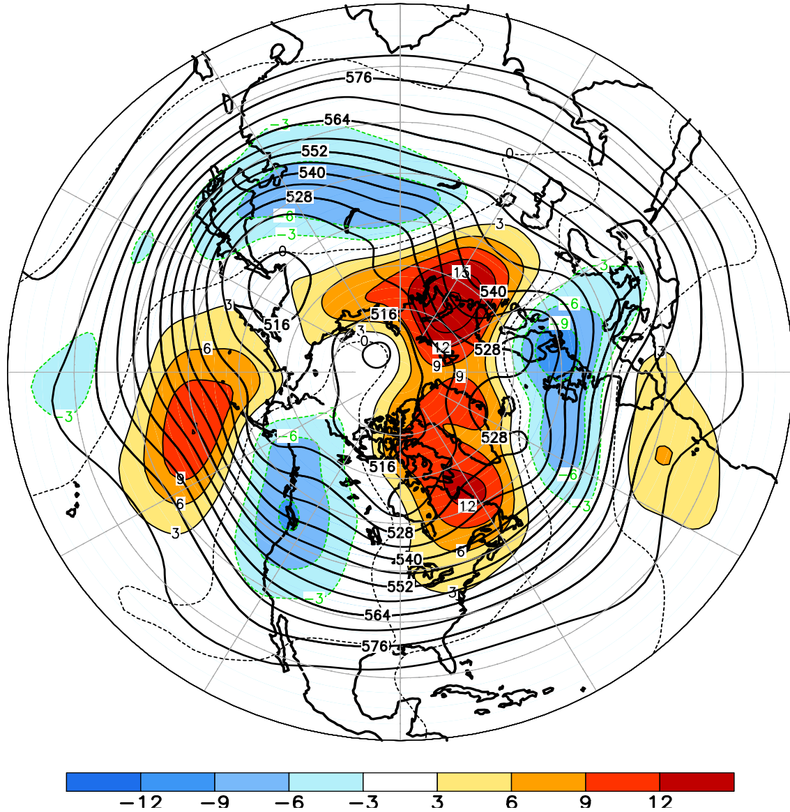
FIGURE E9. Northern Hemisphere mean and anomalous 500-hPa geopotential height (CDAS/Reanalysis) for DEC 2012. Mean heights are denoted by solid contours drawn at an interval of 6 dam. Anomaly contour interval is 3 dam with values less (greater) than -3 dam (3 dam) indicated by dark (light) shading. Anomalies are calculated as departures from the 1981-2010 base period monthly means.
