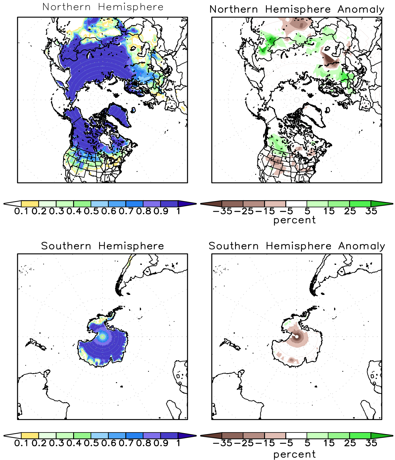
FIGURE A2.2. SSM/I derived snow cover frequency (%) (left) and snow cover anomaly (%) (right) for the month of DEC 2012 based on 1987 - 2010 base period for the Northern Hemisphere (top) and Southern Hemisphere (bottom). It is generated using the algorithm described by Ferraro et. al, 1996, Bull. Amer. Meteor. Soc., vol 77, 891-905.
