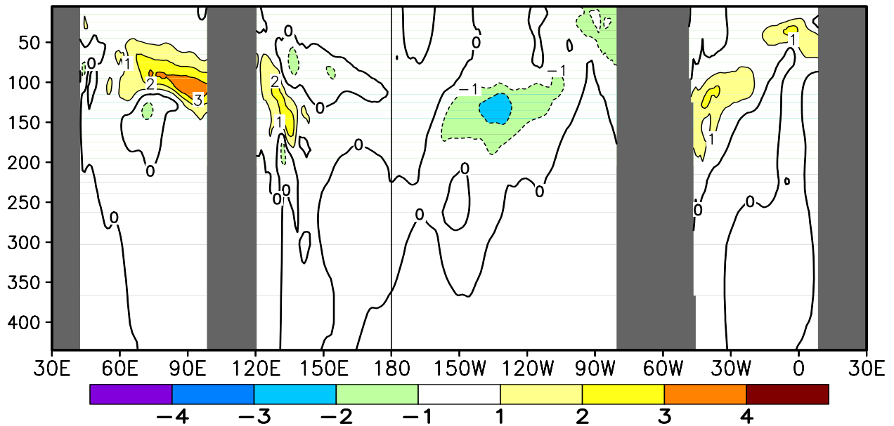
FIGURE T17. Equatorial depth–longitude section of ocean temperature (top) and ocean temperature anomalies (bottom) for DEC 2012. Contour interval is 1°C. Dashed contours in bottom panel indicate negative anomalies. Data are derived from the NCEP’s global ocean data assimilation system version 2 which assimilates oceanic observations into an oceanic GCM (Xue, Y. and Behringer, D.W., 2006: Operational global ocean data assimilation system at NCEP, to be submitted to BAMS). Anomalies are departures from the 1981–2010 base period means.
