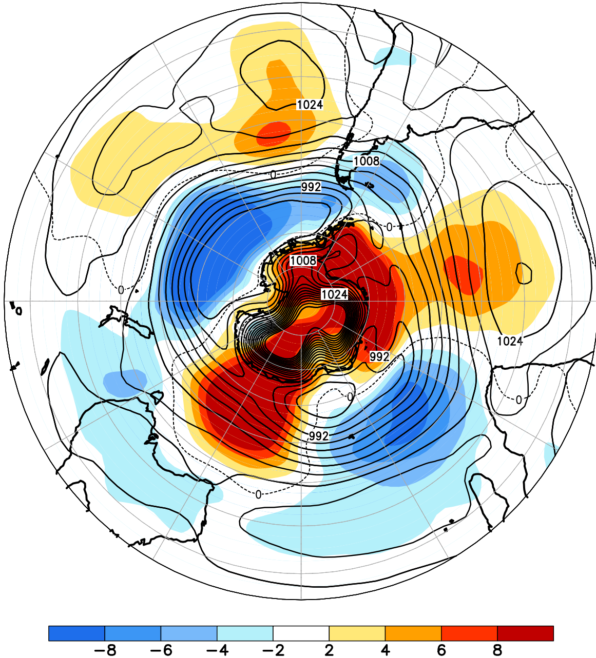
FIGURE E14. Southern Hemisphere mean and anomalous sea level pressure(CDAS/Reanalysis) for AUG 2020. Mean values are denoted by solid contours drawn at an interval of 4 hPa. Anomaly contour interval is 2 hPa with values less (greater) than -2 hPa (2 hPa) indicated by dark (light) shading. Anomalies are calculated as departures from the 1981-2010 base period monthly means.
