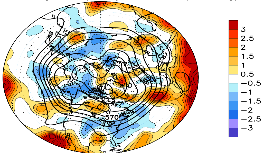
FIGURE E13. Northern Hemisphere 500-hPa heights (thick contours, interval is 6 dam) overlaid with (Top) Standard deviation of 10-day high-pass (HP) filtered height anomalies and (Bottom) Normalized anomalous variance of 10-day HP filtered height anomalies. A Lanczos filter is used to calculate the HP filtered anomalies. Anomalies are departures from the 1981-2010 daily means.
