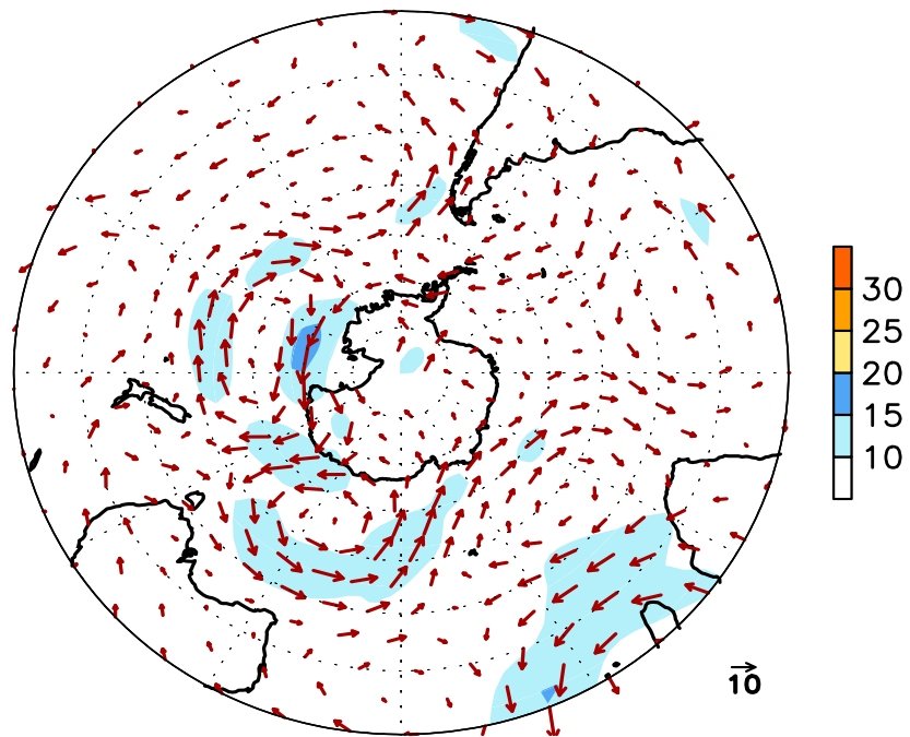
FIGURE E16. Southern Hemisphere mean (left) and anomalous (right) 300-hPa vector wind (CDAS/Reanalysis) for AUG 2020. Mean (anomaly) isotach contour interval is 10 (5) \text{ms}^{-1} . Values greater than 30 \text{ ms}^{-1} (left) and 10 \text{ ms}^{-1} (rights) are shaded. Anomalies are departures from the 1981-2010 base period monthly means.
