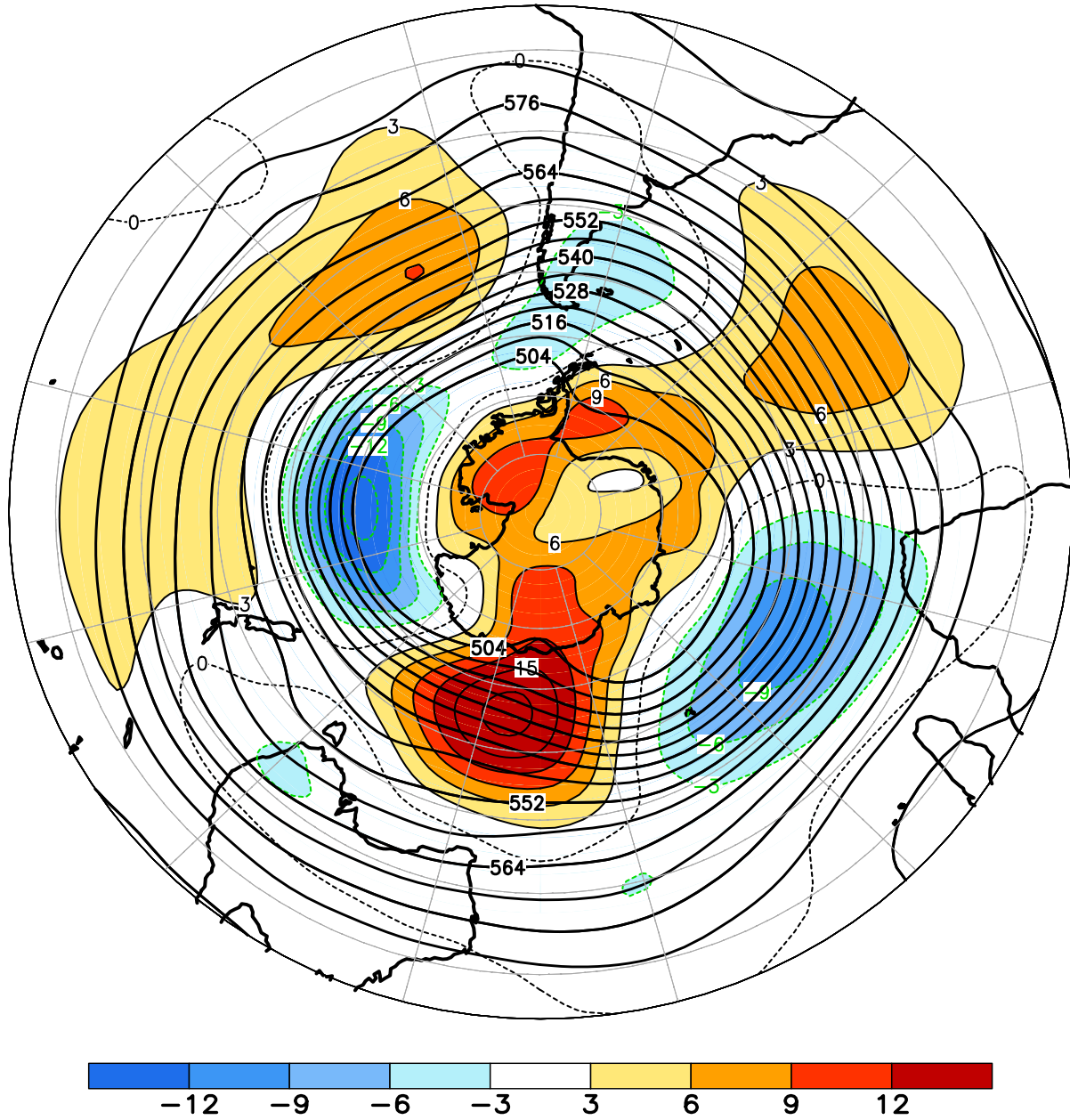
FIGURE E15. Southern Hemisphere mean and anomalous 500-hPa geopotential height (CDAS/Reanalysis) for AUG 2020. Mean heights are denoted by solid contours drawn at an interval of 6 dam. Anomaly contour interval is 3 dam with values less (greater) than -3 dam (3 dam) indicated by dark (light) shading. Anomalies are calculated as departures from the 1981-2010 base period monthly means.
