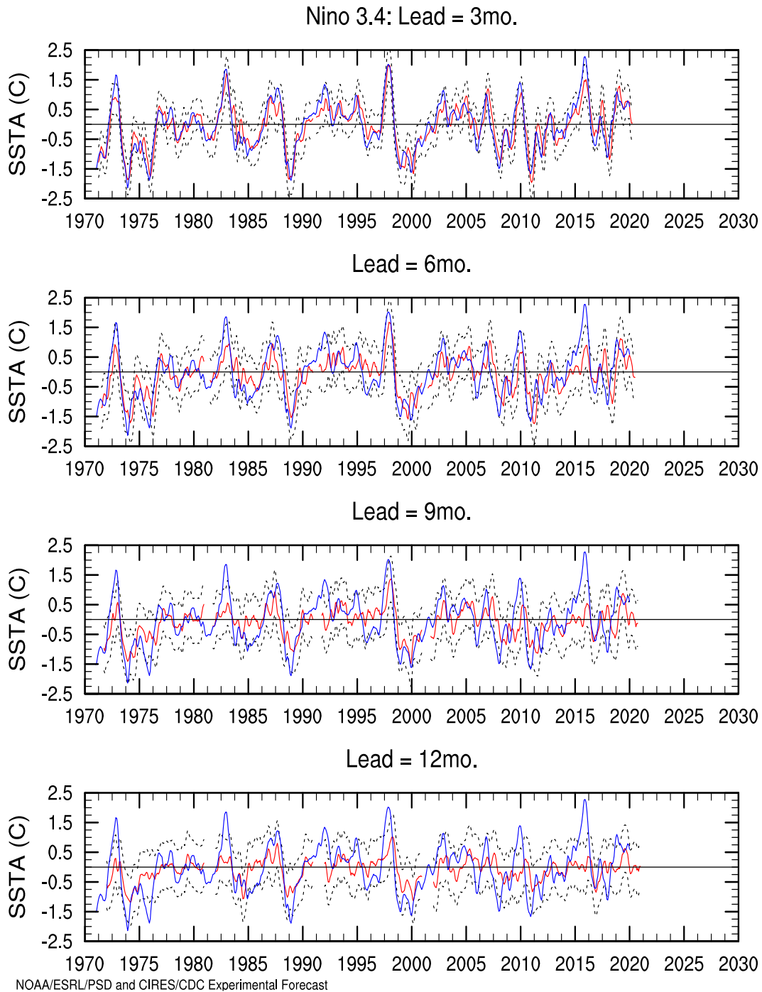
FIGURE F10. Predictions of Niño 3.4 SSTA (blue solid line) and verification (solid red line). The Niño3.4 Index was calculated in the area 6N-6S, 170W-120W. The 1980-2010 climatology was subtracted from ERSST data between 1950 and 2010, after which they were projected onto 20 EOFs containing 90% of the variance. Significant 1950-2010 trends were subtracted from the corresponding PCs, the forecast was made on the detrended anomalies, after which the trend was added to the forecast. The dotted lines indicate the one standard deviation confidence interval for the forecasts based on a perfect adherence to assumption.
