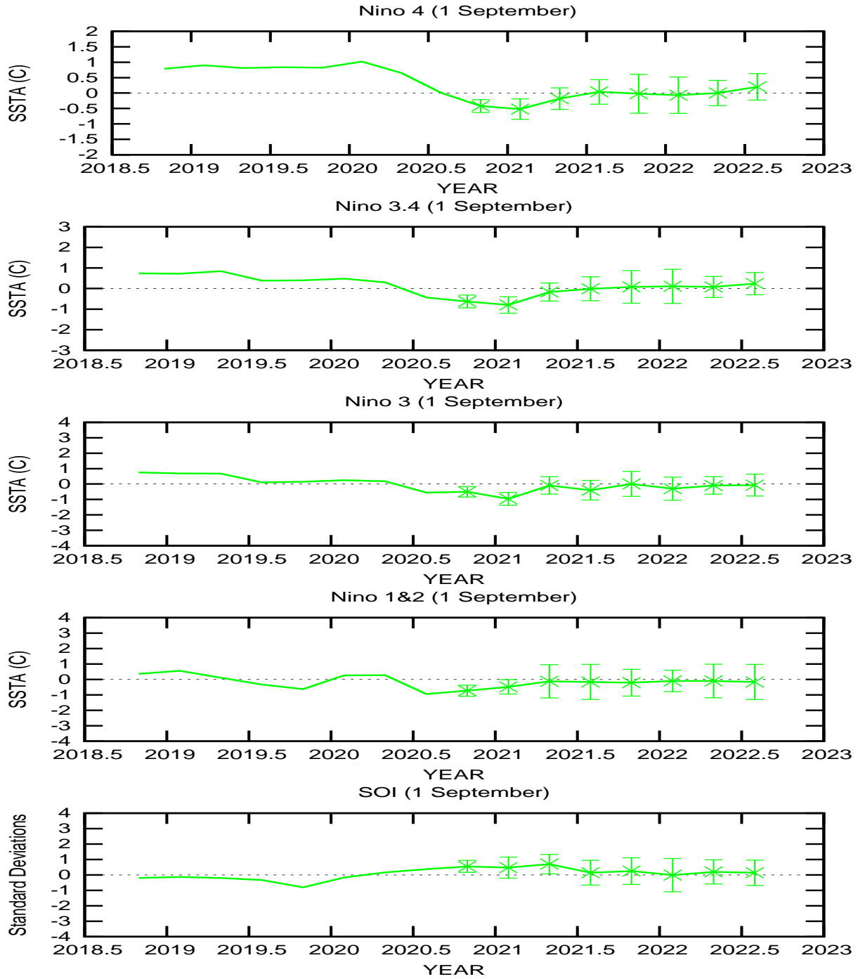
FIGURE F11. ENSO-CLIPER statistical model forecasts of three-month average sea surface temperature anomalies (green lines, deg. C) in (top panel) the Nino 4 region (5N-5S, 160E-150W), (second panel) the Nino 3.4 region (5N-5S, 170W-120W), (third panel) the Nino 3 region (5N-5S, 150W-90W), and (fourth panel) the Nino 1+2 region (0-10S, 90W-80W) (Knaff and Landsea 1997, Wea. Forecasting , 12 , 633-652). Bottom panel shows predictions of the three-month standardized Southern Oscillation Index (SOI, green line). Horizontal bars on green line indicate the adjusted root mean square error (RMSE). The Observed three-month average values are indicated by the thick blue line. SST anomalies are departures from the 1981-2010 base period means, and the SOI is calculated from the 1951-1980 base period means.
