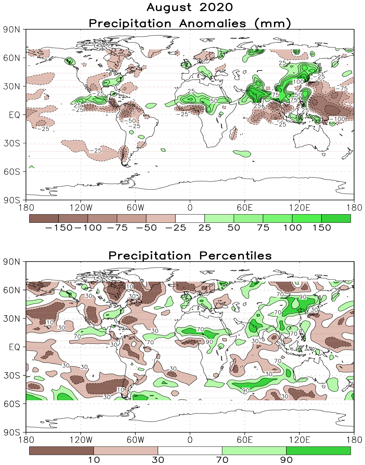
FIGURE E3. Anomalous precipitation (mm, top) and precipitation percentiles based on a Gamma distribution fit to the 1981–2010 base period data (bottom) for AUG 2020. Data are obtained from a merge of raingauge observations and satellite-derived precipitation estimates (Janowiak and Xie 1999, J. Climate , 12 , 3335–3342). Contours are drawn at 200, 100, 50, 25, -25, -50, -100, and -200 mm in top panel. Percentiles are not plotted in regions where mean monthly precipitation is <5mm/month.
