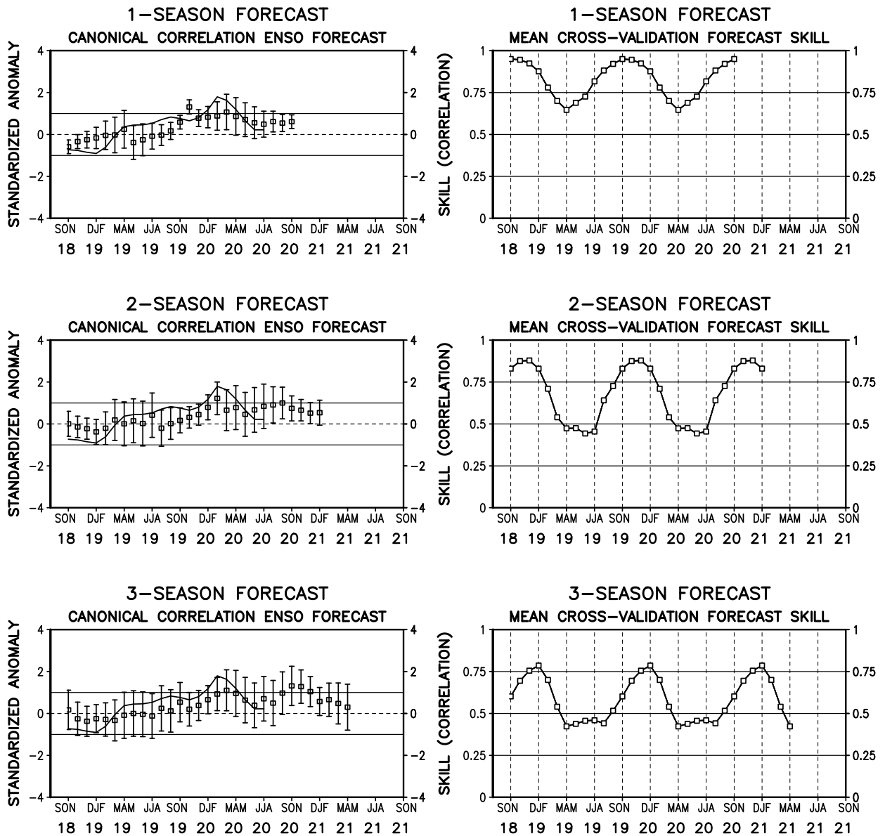
FIGURE F1. Canonical correlation analysis (CCA) sea surface temperature (SST) anomaly prediction for the central Pacific ( 5^{\circ}\text{N} to 5^{\circ}\text{S} , 120^{\circ}\text{W} to 170^{\circ}\text{W} (Barnston and Ropelewski, 1992, J. Climate , 5 , 1316-1345). The three plots on the left hand side are, from top to bottom, the 1-season, 2-season, and 3-season lead forecasts. The solid line in each forecast represents the observed SST standardized anomaly through the latest month. The small squares at the mid-points of the forecast bars represent the real-time CCA predictions based on the anomalies of quasi-global sea level pressure and on the anomalies of tropical Pacific SST, depth of the 20^{\circ}\text{C} isotherm and sea level height over the prior four seasons. The vertical lines represent the one standard deviation error bars for the predictions based on past performance. The three plots on the right side are skills, corresponding to the predicted and observed SST. The skills are derived from cross-correlation tests from 1956 to present. These skills show a clear annual cycle and are inversely proportional to the length of the error bars depicted in the forecast time series.
