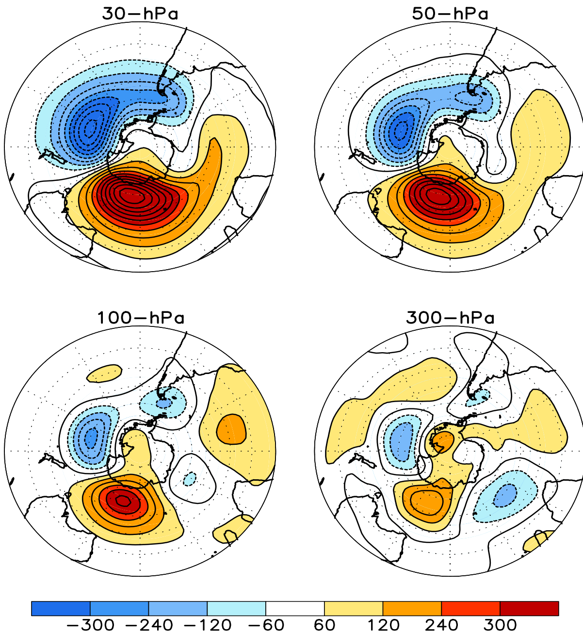
FIGURE S1. Stratospheric height anomalies (m) at selected levels for AUG 2020. Positive values are indicated by solid contours and dark shading. Negative values are indicated by dashed contours and light shading. Contour interval is 60 m. Anomalies are calculated from the 1981-2010 base period means. Winter Hemisphere is shown.
