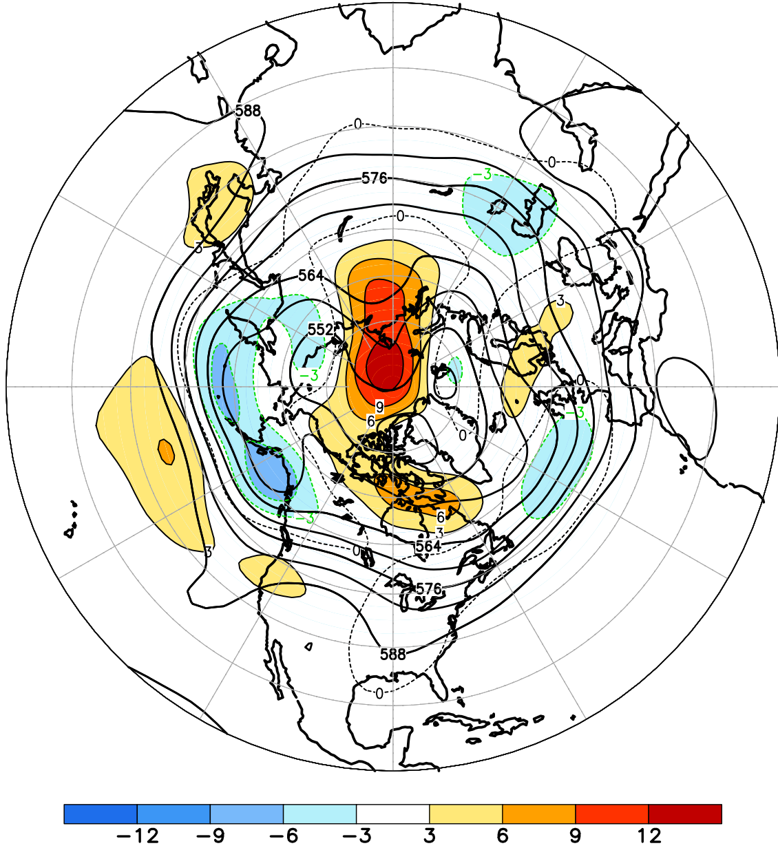
FIGURE E9. Northern Hemisphere mean and anomalous 500-hPa geopotential height (CDAS/Reanalysis) for AUG 2020. Mean heights are denoted by solid contours drawn at an interval of 6 dam. Anomaly contour interval is 3 dam with values less (greater) than -3 dam (3 dam) indicated by dark (light) shading. Anomalies are calculated as departures from the 1981-2010 base period monthly means.
