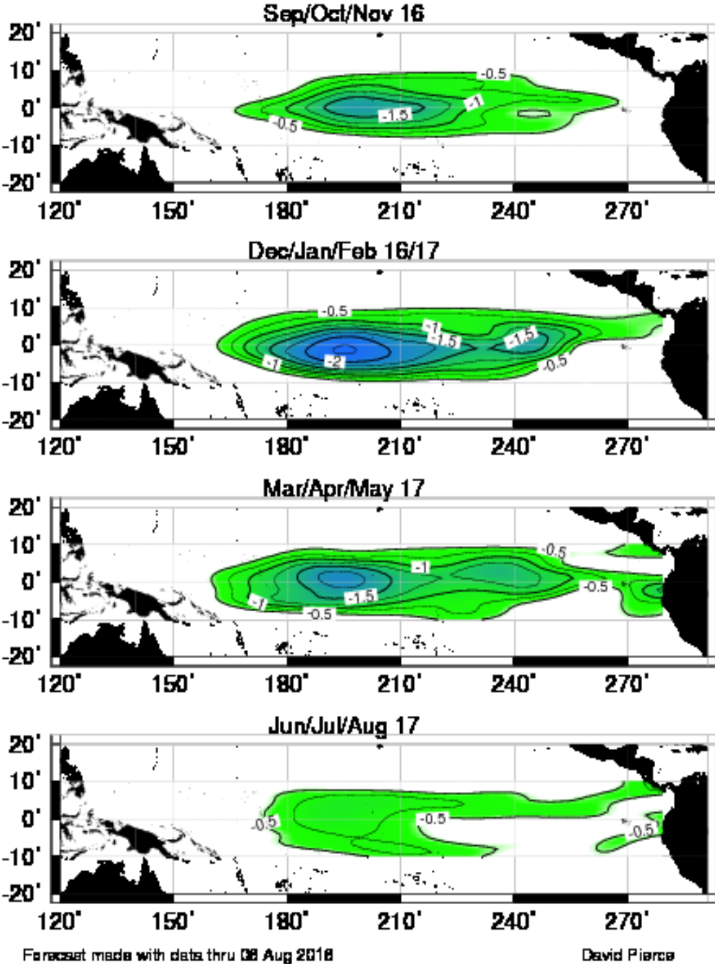
FIGURE F11. SST anomaly forecast for the equatorial Pacific from the Hybrid Coupled Model (HCM) developed by the Scripps Institution of Oceanography and the Max-Plank Institut fuer Meteorologie.
