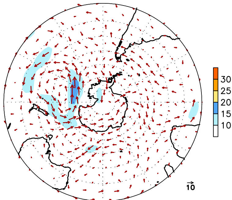
FIGURE E16. Southern Hemisphere mean (left) and anomalous (right) 300-hPa vector wind (CDAS/Reanalysis) for APR 2014. Mean (anomaly) isotach contour interval is 10 (5) \text{ms}^{-1} . Values greater than 30 \text{ms}^{-1} (left) and 10 \text{ms}^{-1} (rights) are shaded. Anomalies are departures from the 1981-2010 base period monthly means.
