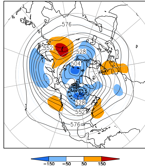
500-hPa Height (dm) & Anomalies (m) (Apr 1–15, 2014)
