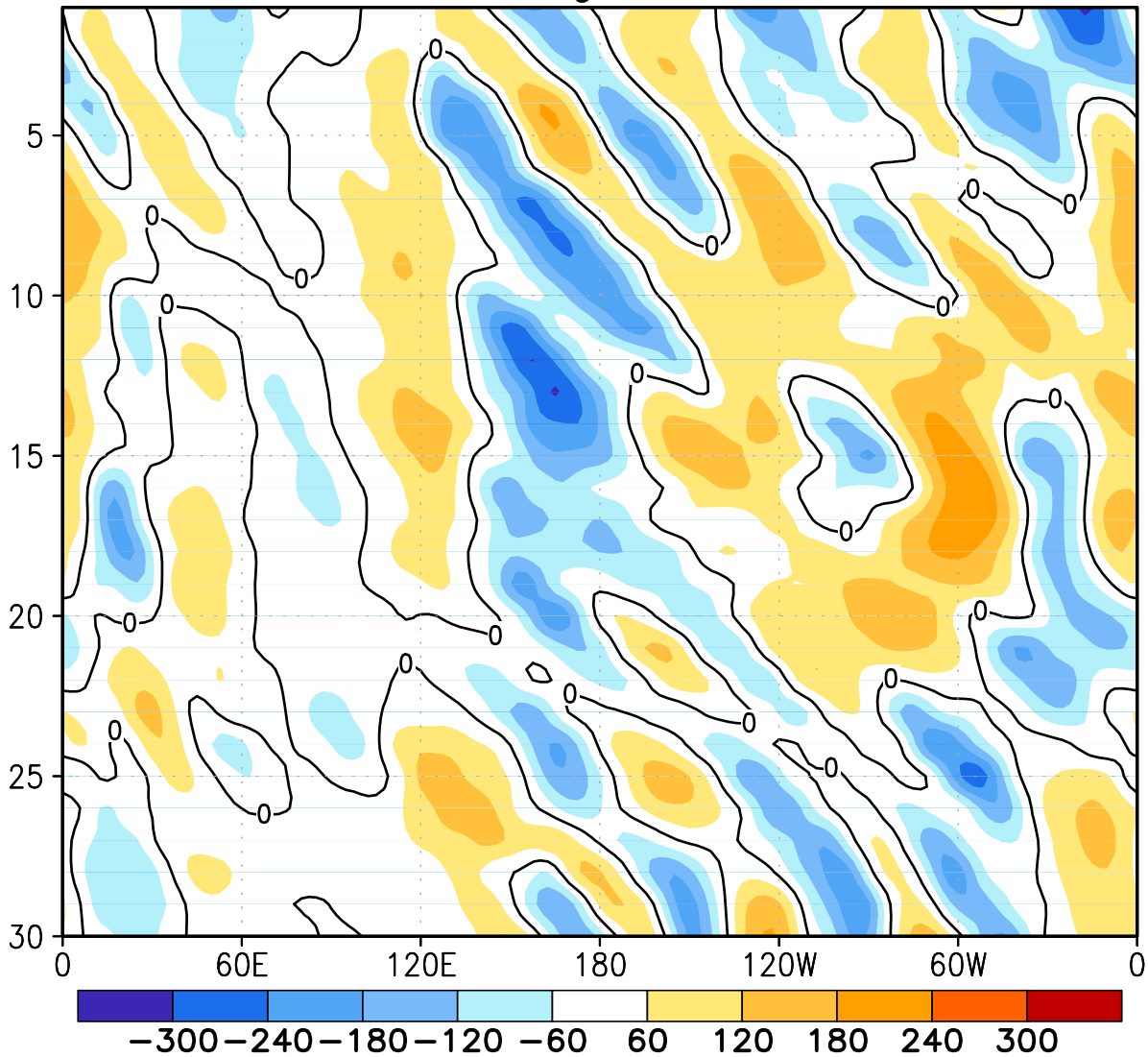
FIGURE E12. Northern Hemisphere: Daily 500-hPa height anomalies for APR 2014 averaged over the 5° latitude band centered on 40°N. Positive values are indicated by solid contours and dark shading. Negative values are indicated by dashed contours and light shading. Contour interval is 60 m. Anomalies are departures from the 1981-2010 base period daily means.
