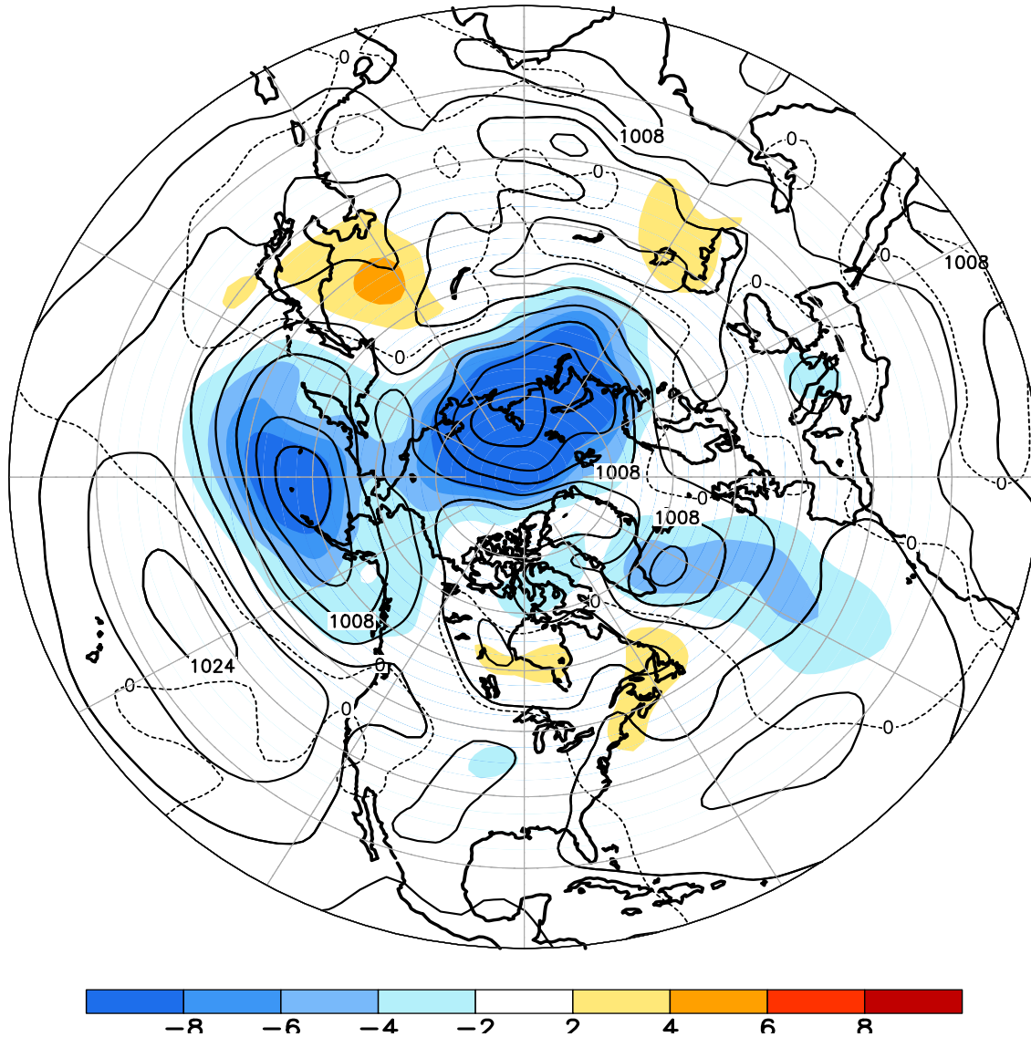
FIGURE E8. Northern Hemisphere mean and anomalous sea level pressure (CDAS/Reanalysis) for APR 2014. Mean values are denoted by solid contours drawn at an interval of 4 hPa. Anomaly contour interval is 2 hPa with values less (greater) than -2 hPa (2 hPa) indicated by dark (light) shading. Anomalies are calculated as departures from the 1981-2010 base period monthly means.
