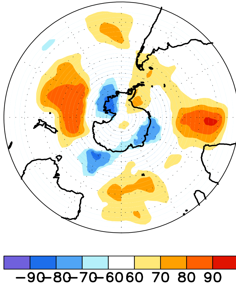
FIGURE E17. Southern Hemisphere percentage of days during APR 2014 in which 500-hPa height anomalies greater than 15 m (red) and less than -15 m (blue) were observed. Values greater than 70% are shaded and contour in-
