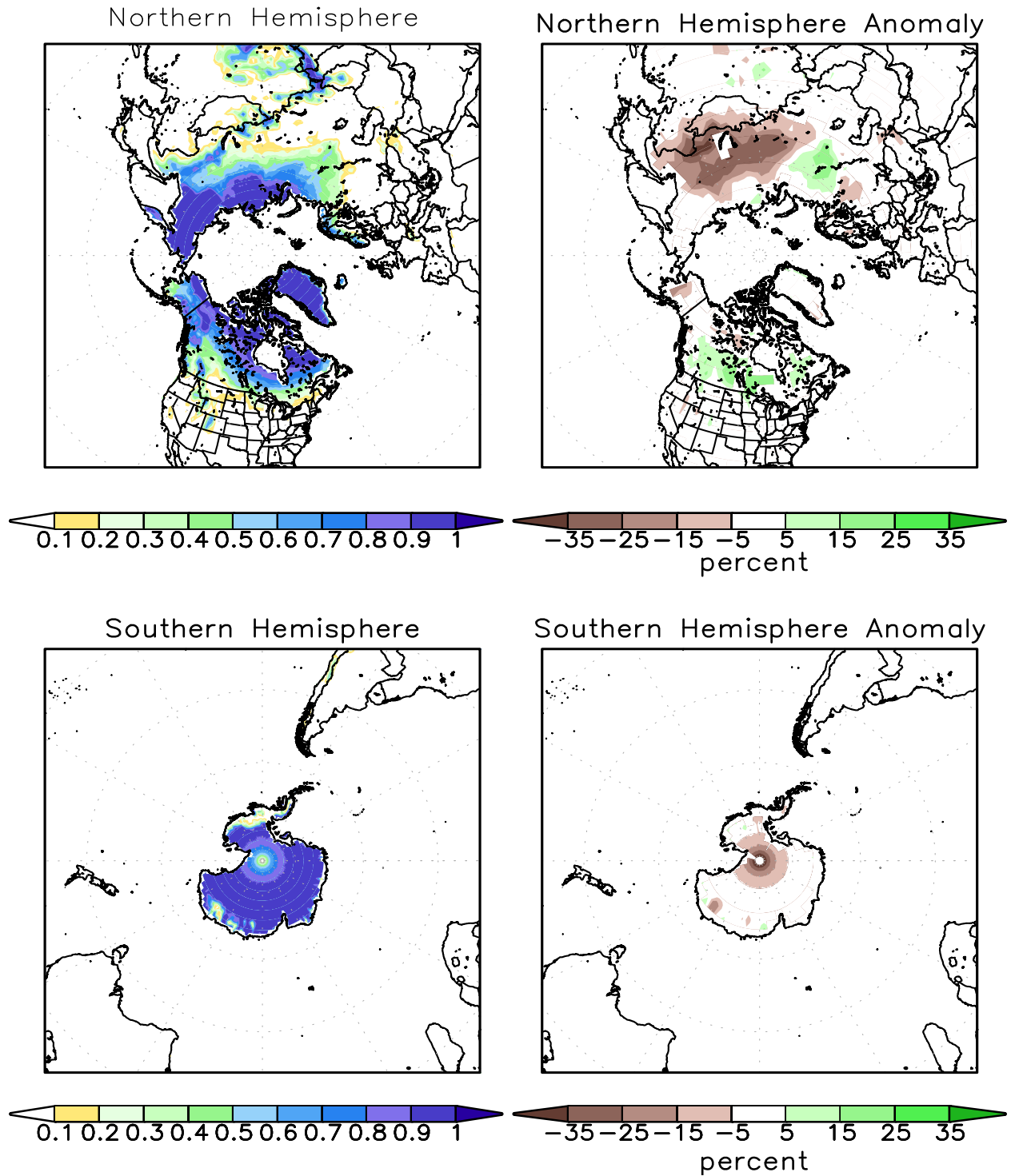
FIGURE A2.2. SSM/I derived snow cover frequency (%) (left) and snow cover anomaly (%) (right) for the month of APR 2014 based on 1987 - 2010 base period for the Northern Hemisphere (top) and Southern Hemisphere (bottom). It is generated using the algorithm described by Ferraro et. al, 1996, Bull. Amer. Meteor. Soc., vol 77, 891-905.
