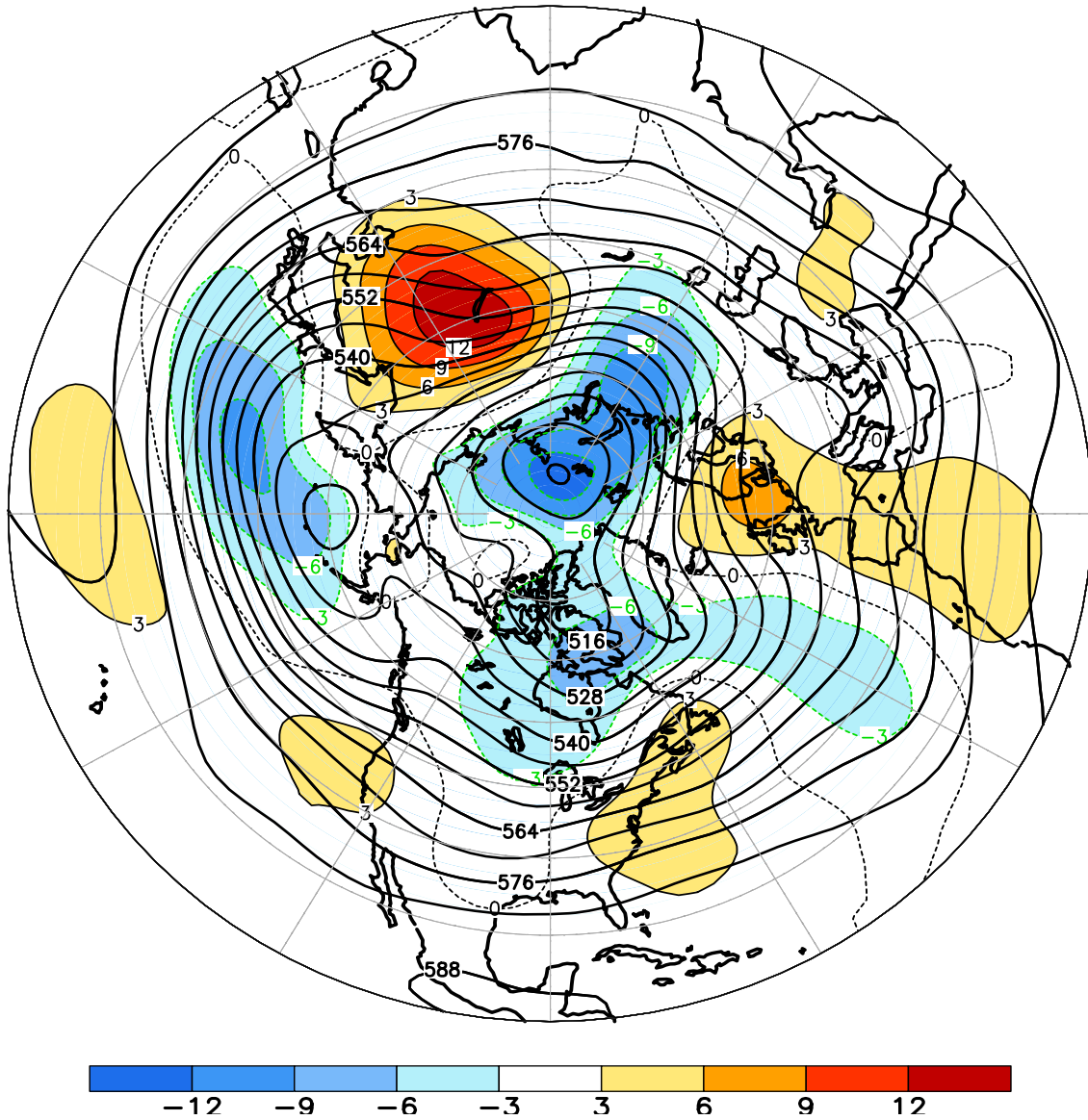
FIGURE E9. Northern Hemisphere mean and anomalous 500-hPa geopotential height (CDAS/Reanalysis) for APR 2014. Mean heights are denoted by solid contours drawn at an interval of 6 dam. Anomaly contour interval is 3 dam with values less (greater) than -3 dam (3 dam) indicated by dark (light) shading. Anomalies are calculated as departures from the 1981-2010 base period monthly means.
