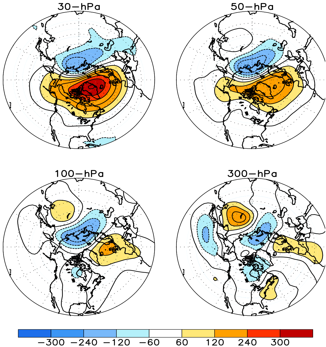
FIGURE S1. Stratospheric height anomalies (m) at selected levels for APR 2014. Positive values are indicated by solid contours and dark shading. Negative values are indicated by dashed contours and light shading. Contour interval is 60 m. Anomalies are calculated from the 1981-2010 base period means. Winter Hemisphere is shown.
