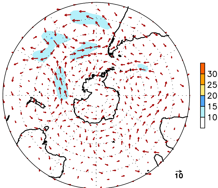
FIGURE E16. Southern Hemisphere mean (left) and anomalous (right) 300-hPa vector wind (CDAS/Reanalysis) for APR 2012. Mean (anomaly) isotach contour interval is 10 (5) \text{ms}^{-1} . Values greater than 30 \text{ ms}^{-1} (left) and 10 \text{ ms}^{-1} (rights) are shaded. Anomalies are departures from the 1981-2010 base period monthly means.
