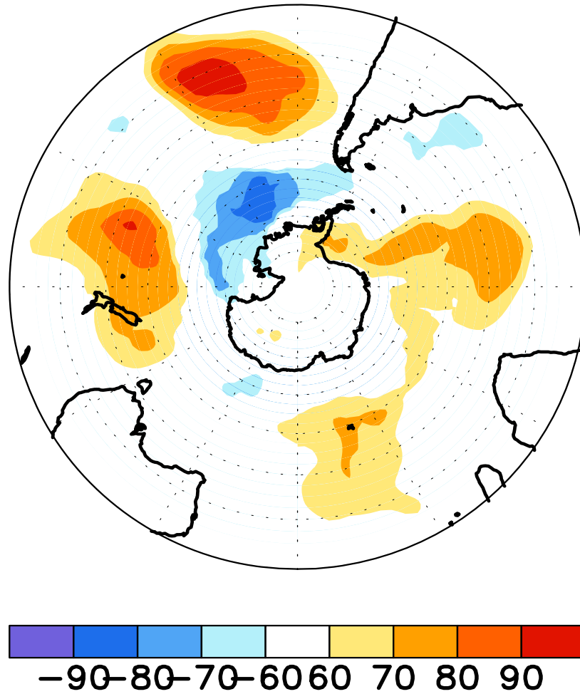
FIGURE E17. Southern Hemisphere percentage of days during APR 2012 in which 500-hPa height anomalies greater than 15 m (red) and less than -15 m (blue) were observed. Values greater than 70% are shaded and contour in-
