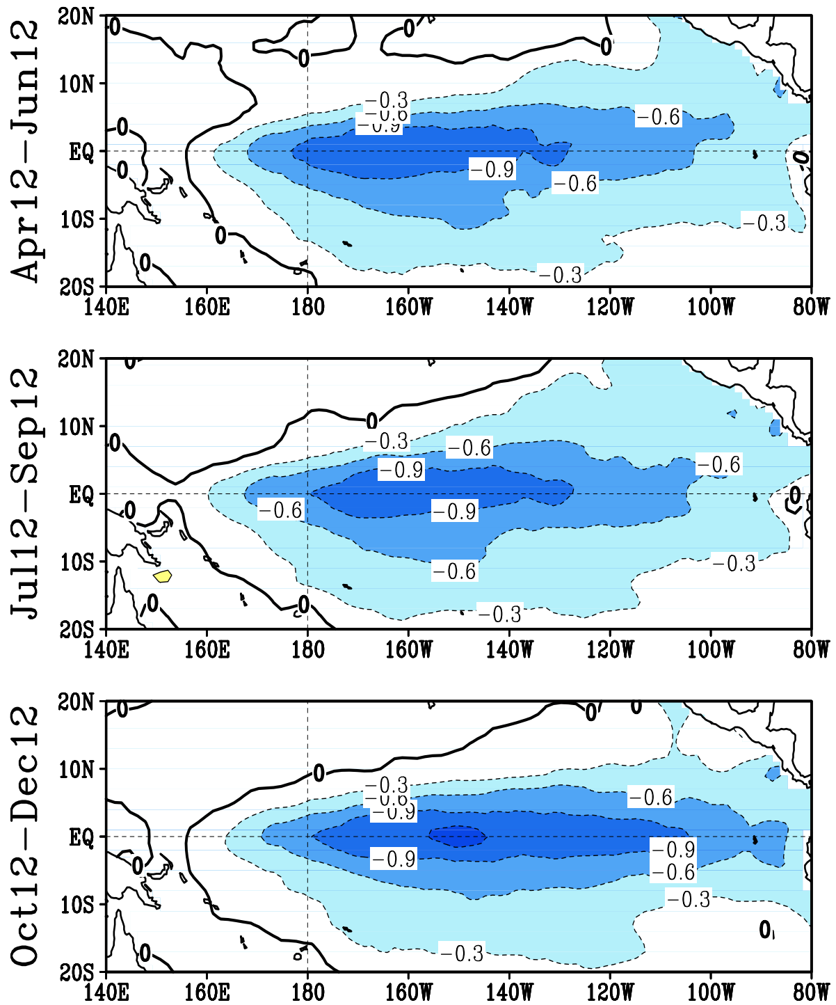
FIGURE F5. Predicted 3-month average sea surface temperature anomalies from the NCEP/CPC Markov model (Xue et al. 2000, J. Climate , 13 , 849-871). The forecast is initiated in APR 2012. Contour interval is 0.3C and negative anomalies are indicated by dashed contours. Anomalies are calculated relative to the 1971-2000 climatology.
