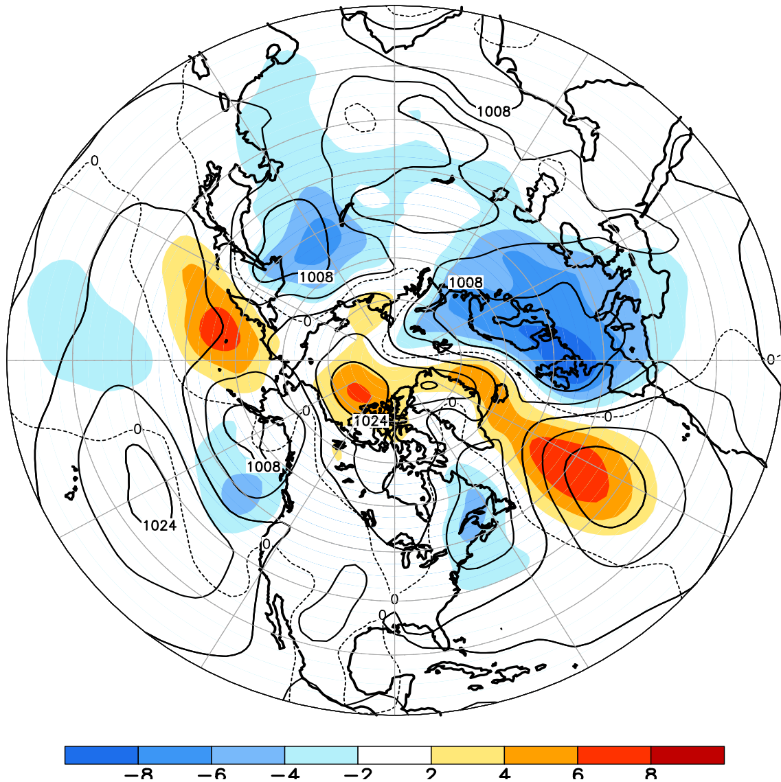
FIGURE E8. Northern Hemisphere mean and anomalous sea level pressure (CDAS/Reanalysis) for APR 2012. Mean values are denoted by solid contours drawn at an interval of 4 hPa. Anomaly contour interval is 2 hPa with values less (greater) than -2 hPa (2 hPa) indicated by dark (light) shading. Anomalies are calculated as departures from the 1981-2010 base period monthly means.
