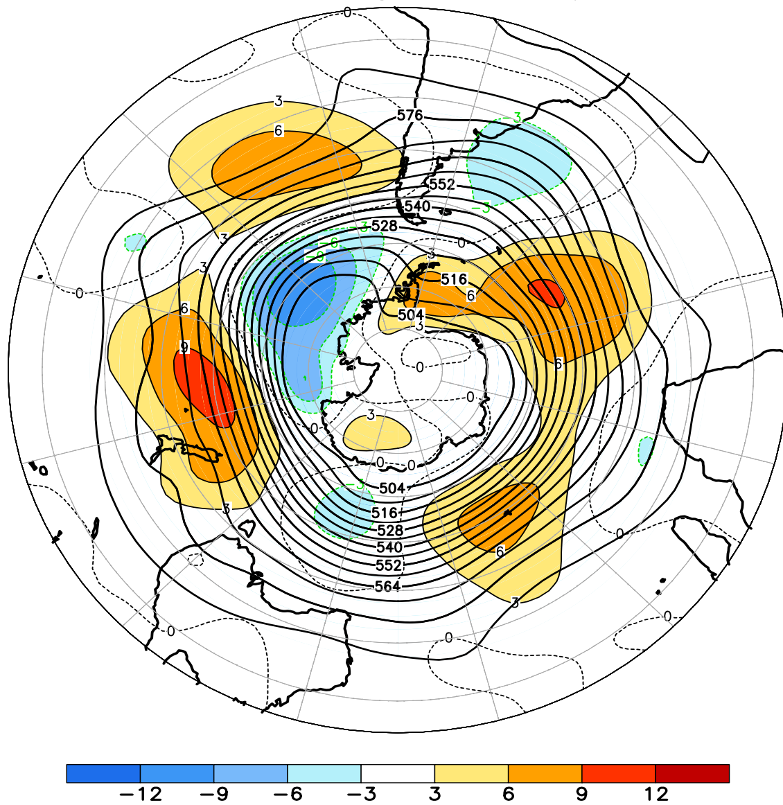
FIGURE E15. Southern Hemisphere mean and anomalous 500-hPa geopotential height (CDAS/Reanalysis) for APR 2012. Mean heights are denoted by solid contours drawn at an interval of 6 dam. Anomaly contour interval is 3 dam with values less (greater) than -3 dam (3 dam) indicated by dark (light) shading. Anomalies are calculated as departures from the 1981-2010 base period monthly means.
