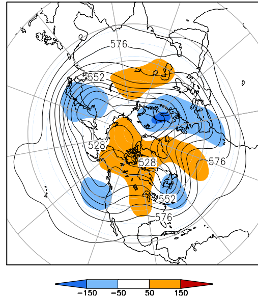
500-hPa Height (dm) & Anomalies (m) (Apr 1–15, 2012)
