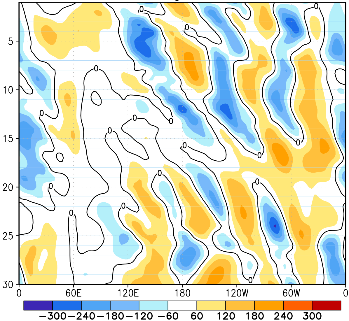
FIGURE E12. Northern Hemisphere: Daily 500-hPa height anomalies for APR 2012 averaged over the 5° latitude band centered on 40°N. Positive values are indicated by solid contours and dark shading. Negative values are indicated by dashed contours and light shading. Contour interval is 60 m. Anomalies are departures from the 1981-2010 base period daily means.
