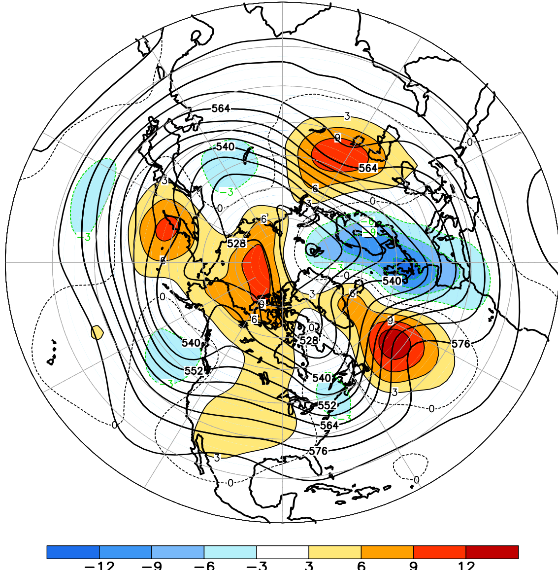
FIGURE E9. Northern Hemisphere mean and anomalous 500-hPa geopotential height (CDAS/Reanalysis) for APR 2012. Mean heights are denoted by solid contours drawn at an interval of 6 dam. Anomaly contour interval is 3 dam with values less (greater) than -3 dam (3 dam) indicated by dark (light) shading. Anomalies are calculated as departures from the 1981-2010 base period monthly means.
