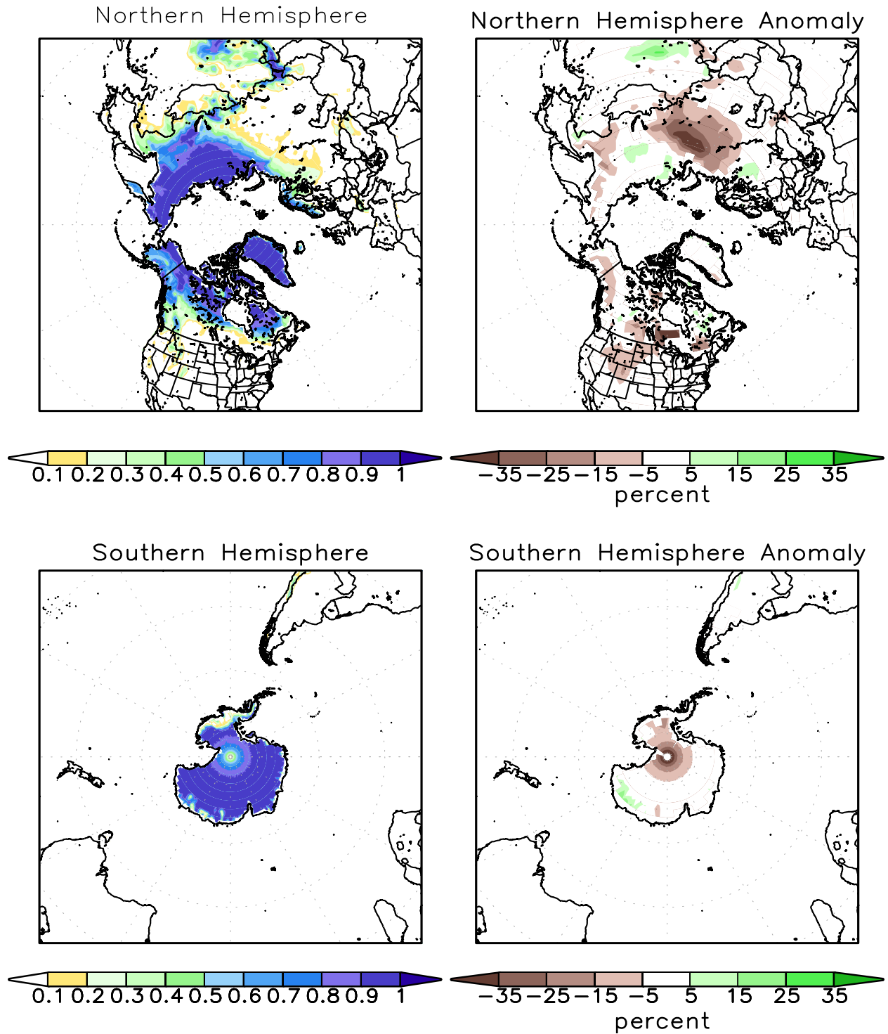
FIGURE A2.2. SSM/I derived snow cover frequency (%) (left) and snow cover anomaly (%) (right) for the month of APR 2012 based on 1987 - 2010 base period for the Northern Hemisphere (top) and Southern Hemisphere (bottom). It is generated using the algorithm described by Ferraro et. al, 1996, Bull. Amer. Meteor. Soc., vol 77, 891-905.
