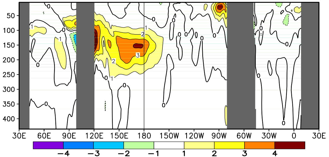
FIGURE T17. Equatorial depth–longitude section of ocean temperature (top) and ocean temperature anomalies (bottom) for APR 2012. Contour interval is 1°C. Dashed contours in bottom panel indicate negative anomalies. Data are derived from the NCEP’s global ocean data assimilation system version 2 which assimilates oceanic observations into an oceanic GCM (Xue, Y. and Behringer, D.W., 2006: Operational global ocean data assimilation system at NCEP, to be submitted to BAMS). Anomalies are departures from the 1981–2010 base period means.
