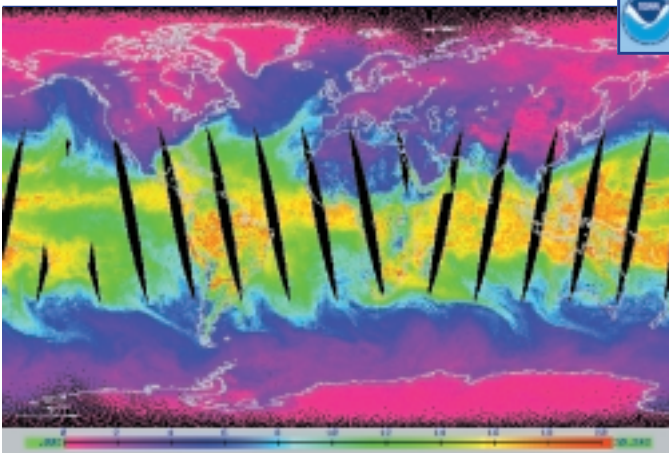
Water vapor mixing ratio products, generated from the first dedicated microwave humidity sounder to fly on POES, are now available at 15 atmospheric levels. This image depicts the 1000 mb water vapor distribution from NOAA-15's AMSU-B on December 21, 1999. Associated atmospheric temperature products are similarly produced for 40 levels, on an orbital basis, from a combination of the HIRS and AMSU-A atmospheric sounding channels (Chs 3-14).
