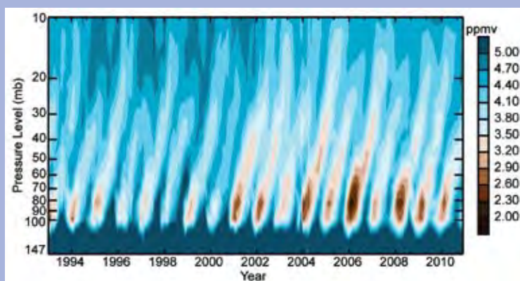
FIG. 2.61. Vertical profiles of tropical (10°N–10°S) stratospheric water vapor mixing ratios from HALOE (1991–2005) and Aura MLS (2004–present). HALOE version 20 mixing ratios were adjusted to better agree with the MLS version 3.3 based on coincident profiles during 2004–05. Adjustments are altitude dependent with a maximum shift of ~0.5 ppmv.
