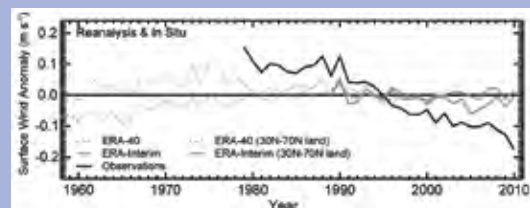
FIG. 2.46. Global average wind speed anomalies over land from reanalysis and observations. The green curves display the wind speed anomalies over land restricted to 30°N–70°N from reanalyses (corresponding to the area covered by the bulk of surface observations). The base period for the anomalies is the 1989–2001 period of overlap from all three datasets.
