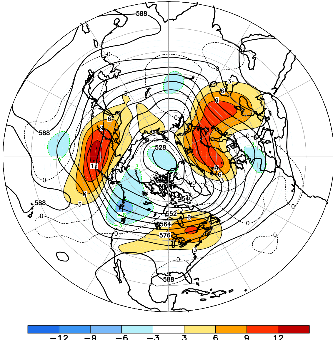
FIGURE E9. Northern Hemisphere mean and anomalous 500-hPa geopotential height (CDAS/Reanalysis) for SEP 2015. Mean heights are denoted by solid contours drawn at an interval of 6 dam. Anomaly contour interval is 3 dam with values less (greater) than -3 dam (3 dam) indicated by dark (light) shading. Anomalies are calculated as departures from the 1981-2010 base period monthly means.
