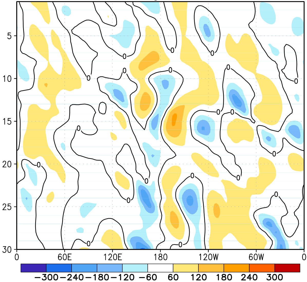
FIGURE E12. Northern Hemisphere: Daily 500-hPa height anomalies for SEP 2015 averaged over the 5° latitude band centered on 40°N. Positive values are indicated by solid contours and dark shading. Negative values are indicated by dashed contours and light shading. Contour interval is 60 m. Anomalies are departures from the 1981-2010 base period daily means.
