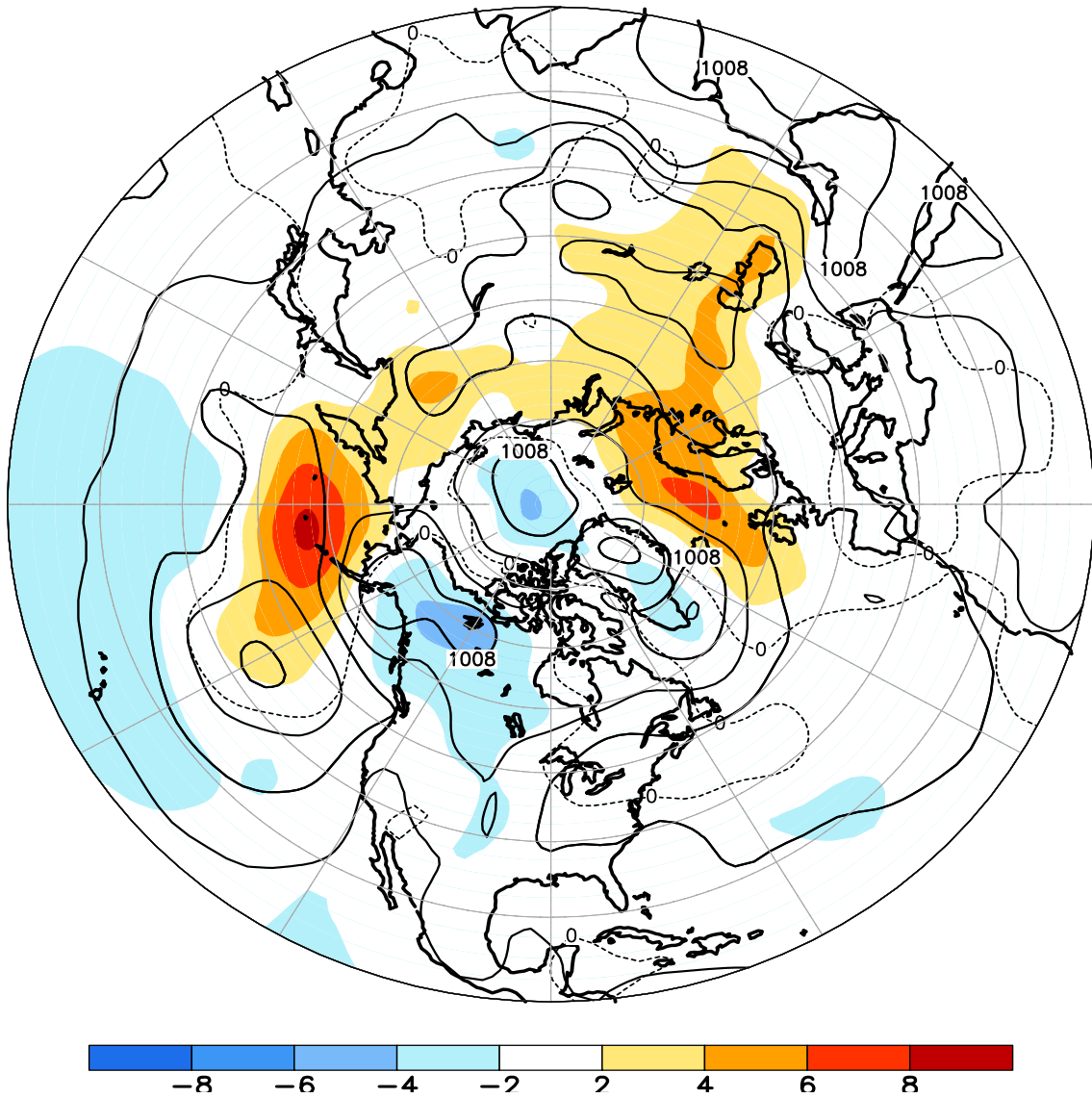
FIGURE E8. Northern Hemisphere mean and anomalous sea level pressure (CDAS/Reanalysis) for SEP 2015. Mean values are denoted by solid contours drawn at an interval of 4 hPa. Anomaly contour interval is 2 hPa with values less (greater) than -2 hPa (2 hPa) indicated by dark (light) shading. Anomalies are calculated as departures from the 1981-2010 base period monthly means.
