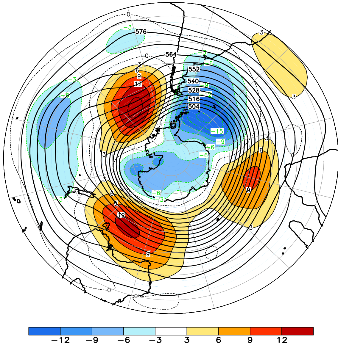
FIGURE E15. Southern Hemisphere mean and anomalous 500-hPa geopotential height (CDAS/Reanalysis) for SEP 2015. Mean heights are denoted by solid contours drawn at an interval of 6 dam. Anomaly contour interval is 3 dam with values less (greater) than -3 dam (3 dam) indicated by dark (light) shading. Anomalies are calculated as departures from the 1981-2010 base period monthly means.
