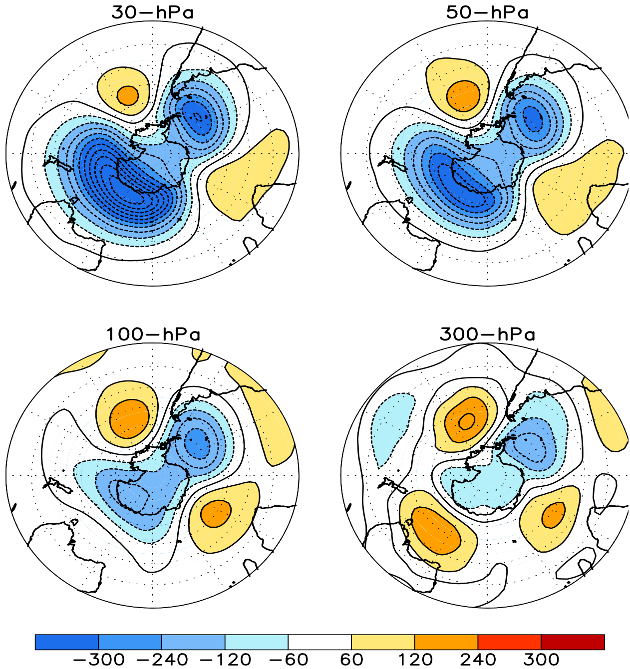
FIGURE S1. Stratospheric height anomalies (m) at selected levels for SEP 2015. Positive values are indicated by solid contours and dark shading. Negative values are indicated by dashed contours and light shading. Contour interval is 60 m. Anomalies are calculated from the 1981-2010 base period means. Winter Hemisphere is shown.
