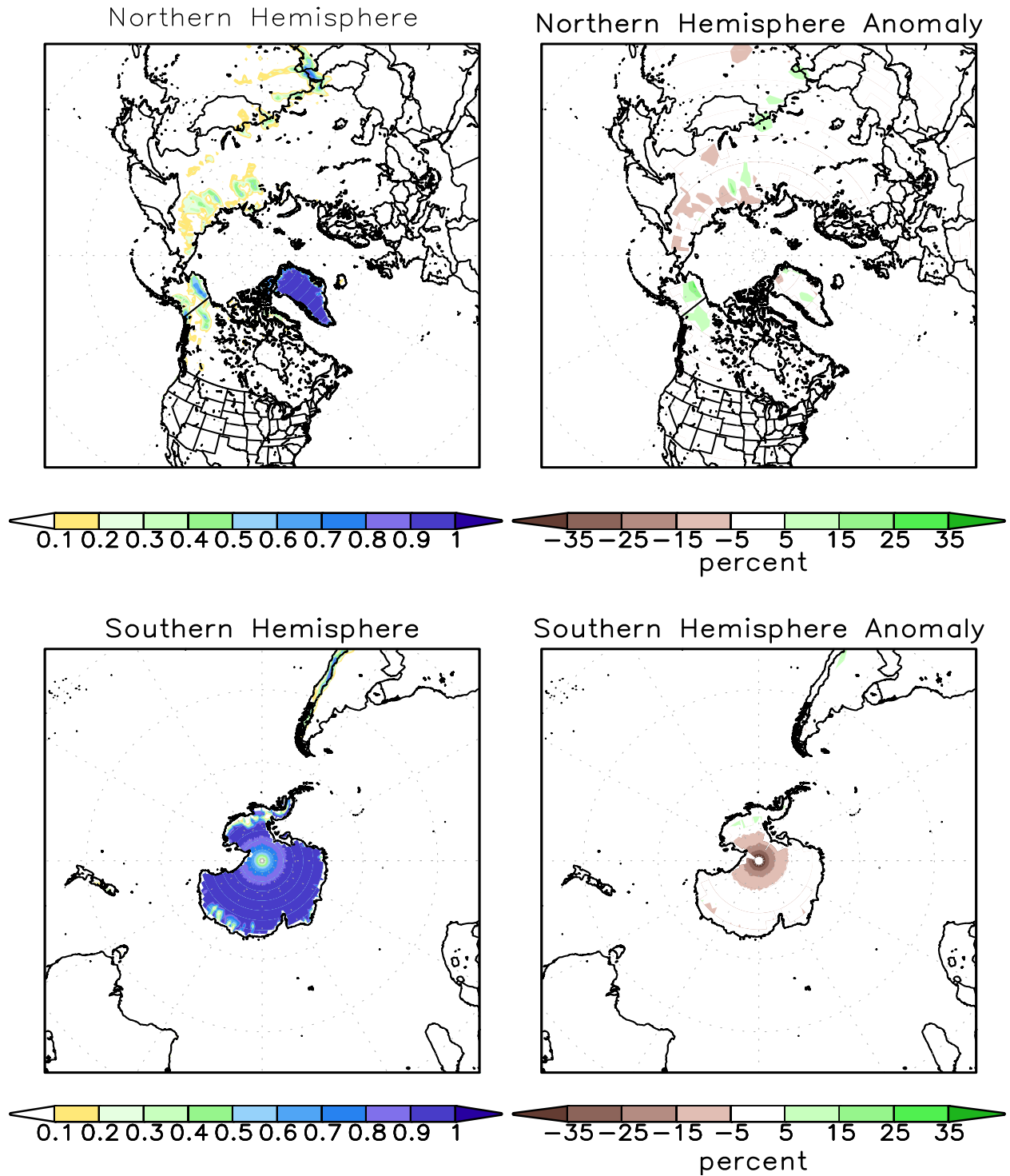
FIGURE A2.2. SSM/I derived snow cover frequency (%) (left) and snow cover anomaly (%) (right) for the month of SEP 2015 based on 1987 - 2010 base period for the Northern Hemisphere (top) and Southern Hemisphere (bottom). It is generated using the algorithm described by Ferraro et. al, 1996, Bull. Amer. Meteor. Soc., vol 77, 891-905.
