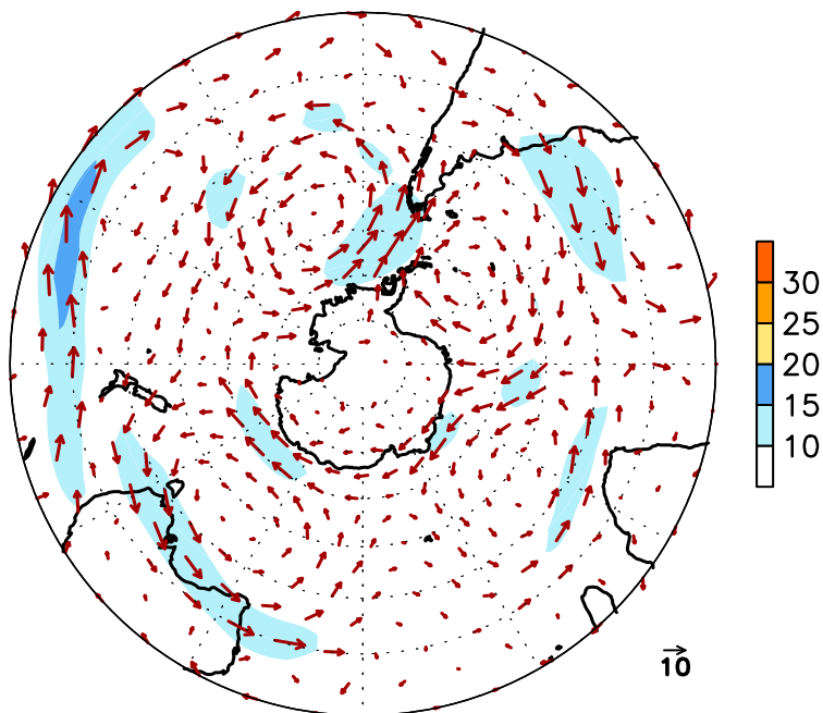
FIGURE E16. Southern Hemisphere mean (left) and anomalous (right) 300-hPa vector wind (CDAS/Reanalysis) for SEP 2015. Mean (anomaly) isotach contour interval is 10 (5) \text{ms}^{-1} . Values greater than 30 \text{ms}^{-1} (left) and 10 \text{ms}^{-1} (rights) are shaded. Anomalies are departures from the 1981-2010 base period monthly means.
