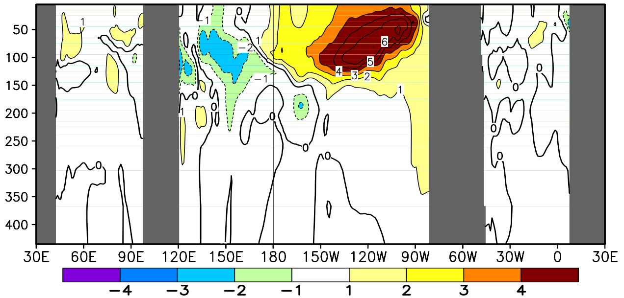
FIGURE T17. Equatorial depth–longitude section of ocean temperature (top) and ocean temperature anomalies (bottom) for SEP 2015. Contour interval is 1°C. Dashed contours in bottom panel indicate negative anomalies. Data are derived from the NCEP’s global ocean data assimilation system version 2 which assimilates oceanic observations into an oceanic GCM (Xue, Y. and Behringer, D.W., 2006: Operational global ocean data assimilation system at NCEP, to be submitted to BAMS). Anomalies are departures from the 1981–2010 base period means.
