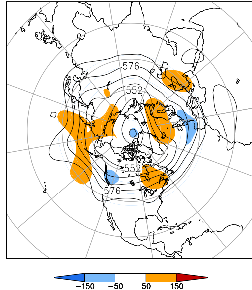
500-hPa Height (dm) & Anomalies (m) (Sep 1–15, 2015)
