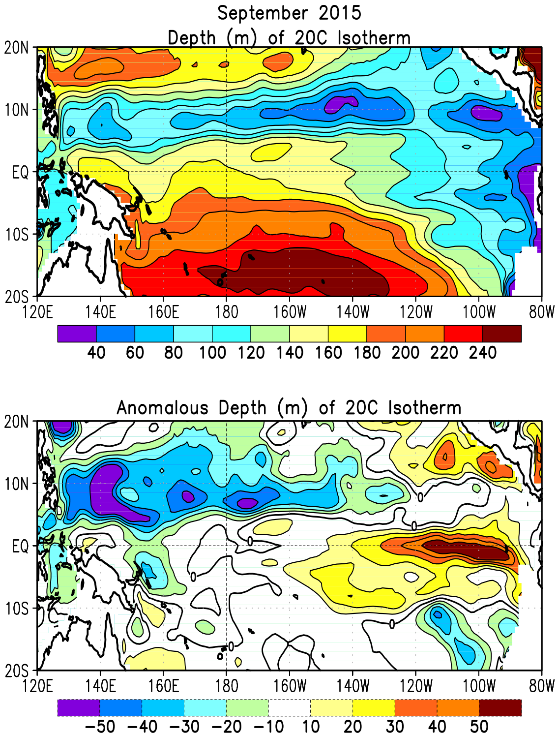
FIGURE T16. Mean (top) and anomalous (bottom) depth of the 20°C isotherm for SEP 2015. Contour interval is 40 m (top) and 10 m (bottom). Dashed contours in bottom panel indicate negative anomalies. Data are derived from the NCEP’s global ocean data assimilation system version 2 which assimilates oceanic observations into an oceanic GCM (Xue, Y. and Behringer, D.W., 2006: Operational global ocean data assimilation system at NCEP, to be submitted to BAMS). Anomalies are departures from the 1981–2010 base period means.
