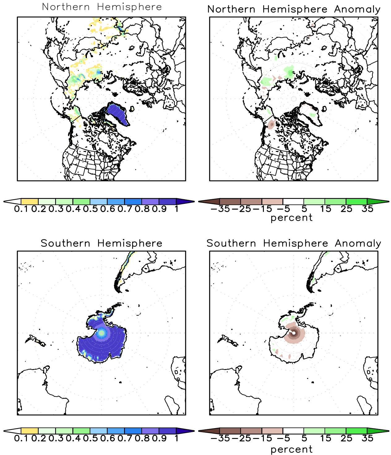
FIGURE A2.2. SSM/I derived snow cover frequency (%) (left) and snow cover anomaly (%) (right) for the month of SEP 2013 based on 1987 - 2010 base period for the Northern Hemisphere (top) and Southern Hemisphere (bottom). It is generated using the algorithm described by Ferraro et. al, 1996, Bull. Amer. Meteor. Soc., vol 77, 891-905.
