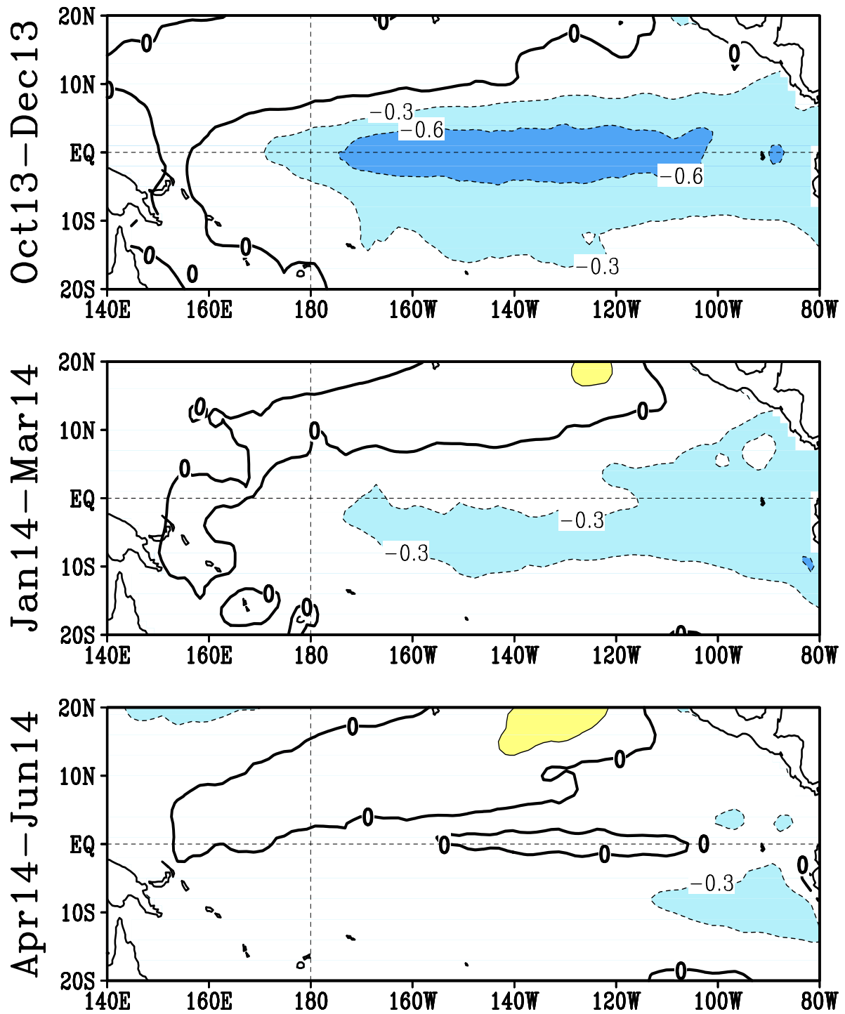
FIGURE F5. Predicted 3-month average sea surface temperature anomalies from the NCEP/CPC Markov model (Xue et al. 2000, J. Climate , 13 , 849-871). The forecast is initiated in SEP 2013 . Contour interval is 0.3C and negative anomalies are indicated by dashed contours. Anomalies are calculated relative to the 1971-2000 climatology.
