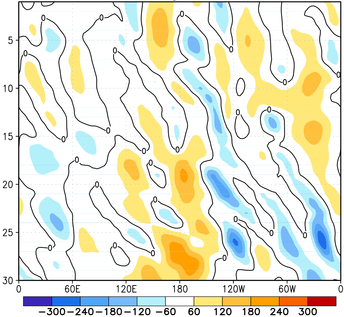
FIGURE E12. Northern Hemisphere: Daily 500-hPa height anomalies for SEP 2013 averaged over the 5° latitude band centered on 40°N. Positive values are indicated by solid contours and dark shading. Negative values are indicated by dashed contours and light shading. Contour interval is 60 m. Anomalies are departures from the 1981-2010 base period daily means.
