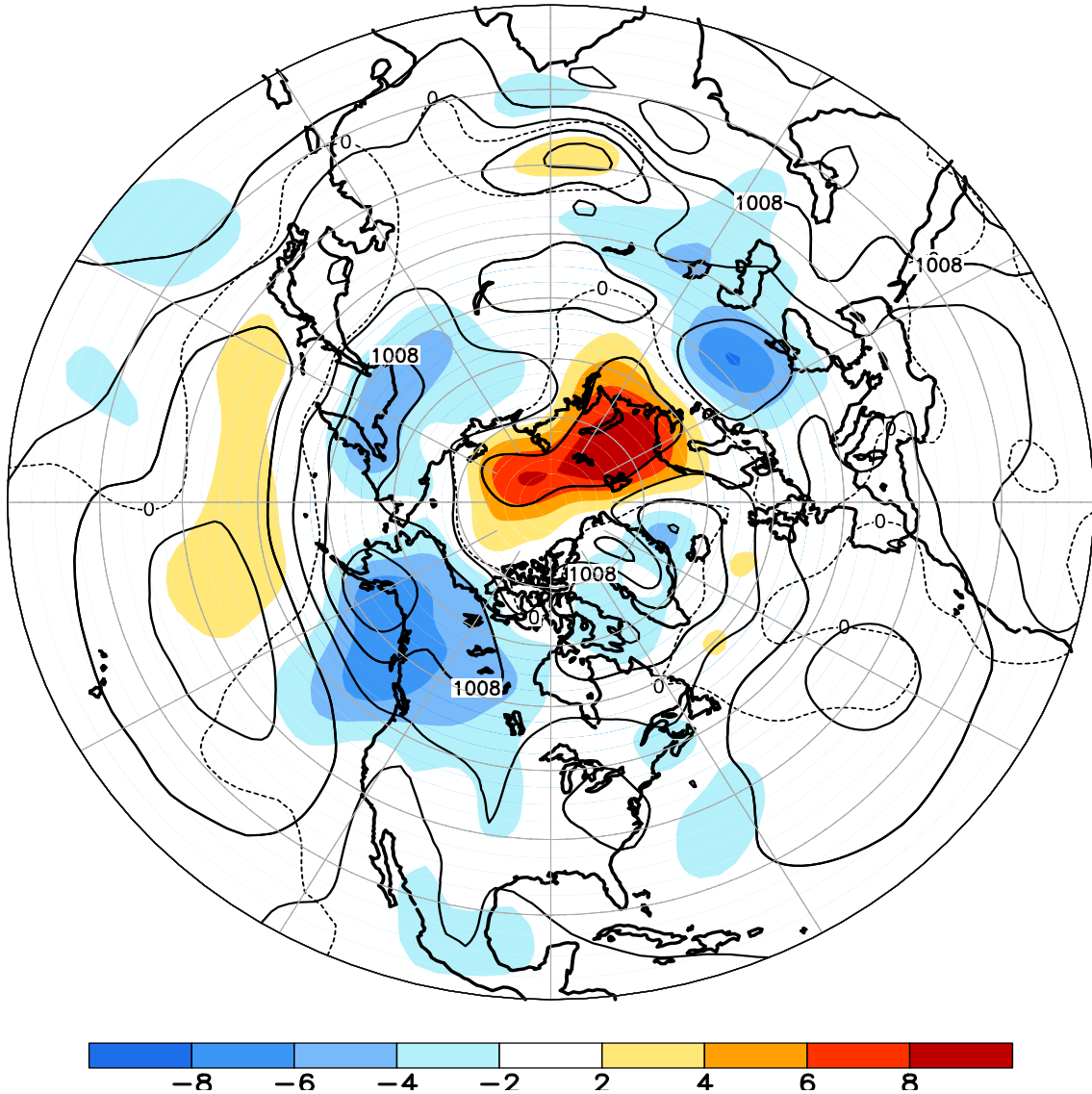
FIGURE E8. Northern Hemisphere mean and anomalous sea level pressure (CDAS/Reanalysis) for SEP 2013. Mean values are denoted by solid contours drawn at an interval of 4 hPa. Anomaly contour interval is 2 hPa with values less (greater) than -2 hPa (2 hPa) indicated by dark (light) shading. Anomalies are calculated as departures from the 1981-2010 base period monthly means.
