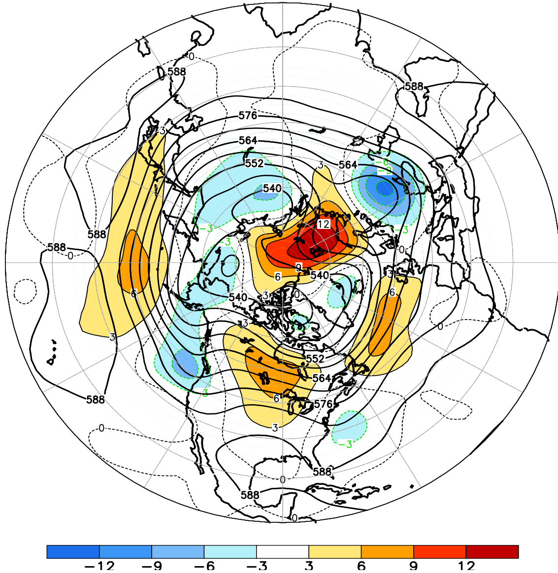
FIGURE E9. Northern Hemisphere mean and anomalous 500-hPa geopotential height (CDAS/Reanalysis) for SEP 2013. Mean heights are denoted by solid contours drawn at an interval of 6 dam. Anomaly contour interval is 3 dam with values less (greater) than -3 dam (3 dam) indicated by dark (light) shading. Anomalies are calculated as departures from the 1981-2010 base period monthly means.
