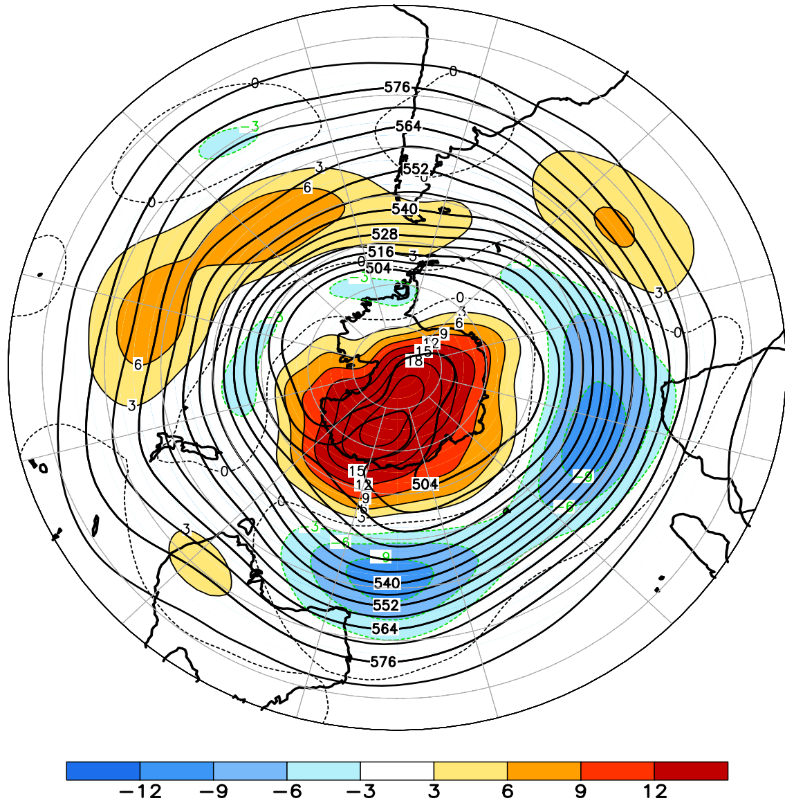
FIGURE E15. Southern Hemisphere mean and anomalous 500-hPa geopotential height (CDAS/Reanalysis) for SEP 2013. Mean heights are denoted by solid contours drawn at an interval of 6 dam. Anomaly contour interval is 3 dam with values less (greater) than -3 dam (3 dam) indicated by dark (light) shading. Anomalies are calculated as departures from the 1981-2010 base period monthly means.
