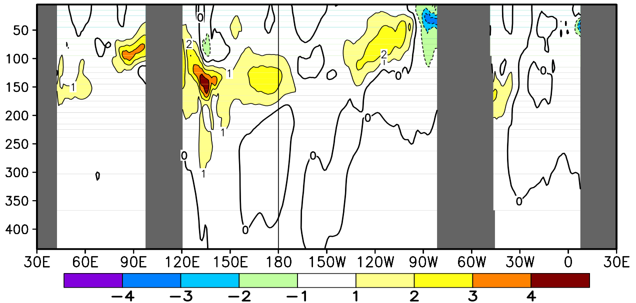
FIGURE T17. Equatorial depth–longitude section of ocean temperature (top) and ocean temperature anomalies (bottom) for SEP 2013. Contour interval is 1°C. Dashed contours in bottom panel indicate negative anomalies. Data are derived from the NCEP’s global ocean data assimilation system version 2 which assimilates oceanic observations into an oceanic GCM (Xue, Y. and Behringer, D.W., 2006: Operational global ocean data assimilation system at NCEP, to be submitted to BAMS). Anomalies are departures from the 1981–2010 base period means.
