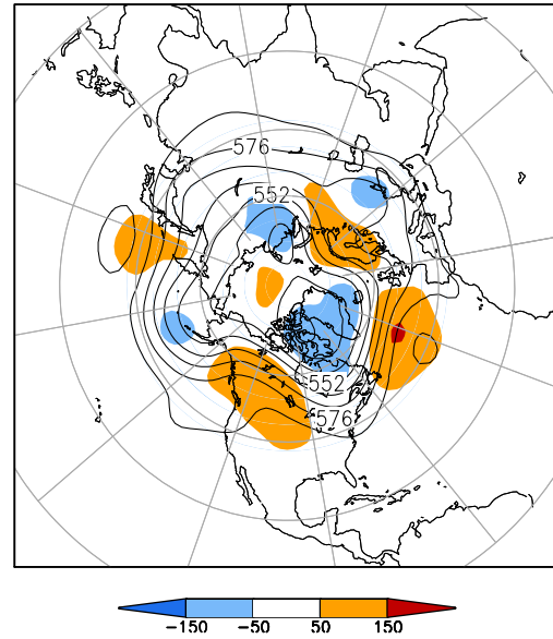
500-hPa Height (dm) & Anomalies (m) (Sep 1–15, 2013)
