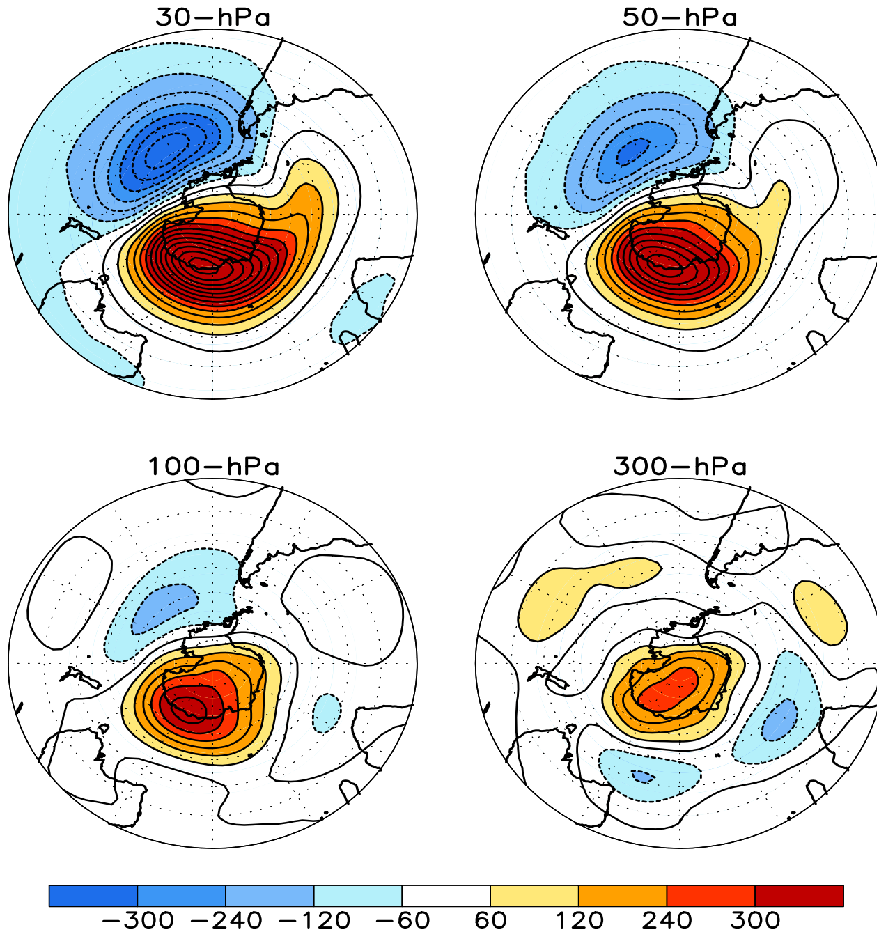
FIGURE S1. Stratospheric height anomalies (m) at selected levels for SEP 2013. Positive values are indicated by solid contours and dark shading. Negative values are indicated by dashed contours and light shading. Contour interval is 60 m. Anomalies are calculated from the 1981-2010 base period means. Winter Hemisphere is shown.
