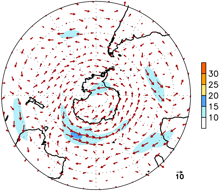
FIGURE E16. Southern Hemisphere mean (left) and anomalous (right) 300-hPa vector wind (CDAS/Reanalysis) for SEP 2013. Mean (anomaly) isotach contour interval is 10 (5) \text{ms}^{-1} . Values greater than 30 \text{ms}^{-1} (left) and 10 \text{ms}^{-1} (rights) are shaded. Anomalies are departures from the 1981-2010 base period monthly means.
