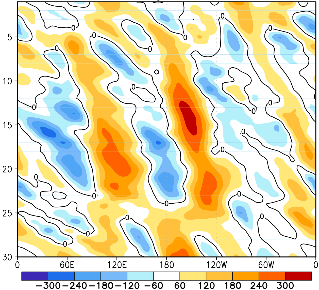
FIGURE E18. Southern Hemisphere: Daily 500-hPa height anomalies for SEP 2010 averaged over the 5° latitude band centered on 40°S. Positive values are indicated by solid contours and dark shading. Negative values are indicated by dashed contours and light shading. Contour interval is 60 m. Anomalies are departures from the 1979-95 base period daily means.
