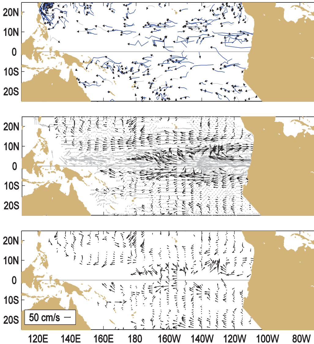
Figure A1.1 Top: Movements of drifting buoys in the tropical Pacific Ocean during September 2010. The linear segments of each trajectory represent a one week displacement. Trajectories of buoys which have lost their subsurface drogues are gray; those with drogues are black.
