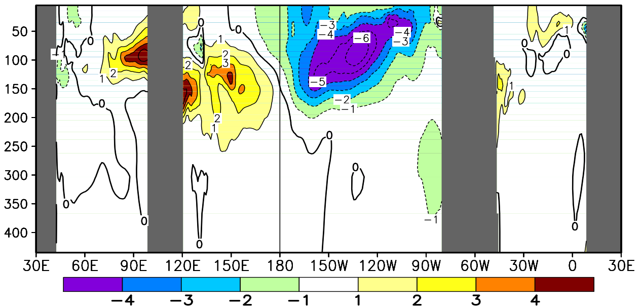
FIGURE T17. Equatorial depth–longitude section of ocean temperature (top) and ocean temperature anomalies (bottom) for SEP 2010. Contour interval is 1°C. Dashed contours in bottom panel indicate negative anomalies. Data are derived from the NCEP’s global ocean data assimilation system version 2 which assimilates oceanic observations into an oceanic GCM (Xue, Y. and Behringer, D.W., 2006: Operational global ocean data assimilation system at NCEP, to be submitted to BAMS). Anomalies are departures from the 1982–2004 base period means.
