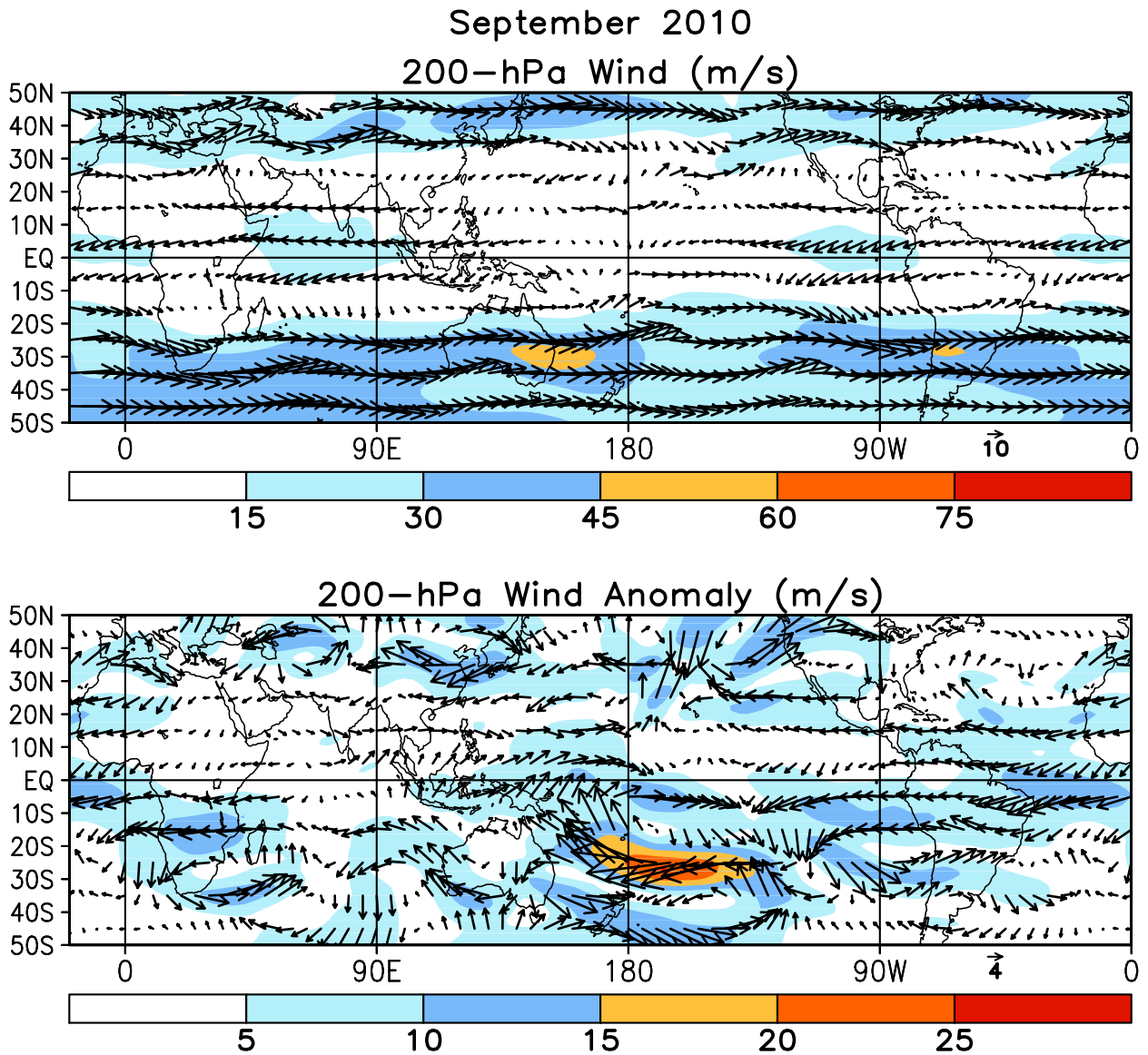
FIGURE T21. Mean (top) and anomalous (bottom) 200-hPa vector wind (CDAS/Reanalysis) for SEP 2010. Contour interval for isotachs is 15 \text{ ms}^{-1} (top) and 5 \text{ ms}^{-1} (bottom). Anomalies are departures from 1979–95 base period monthly means.
