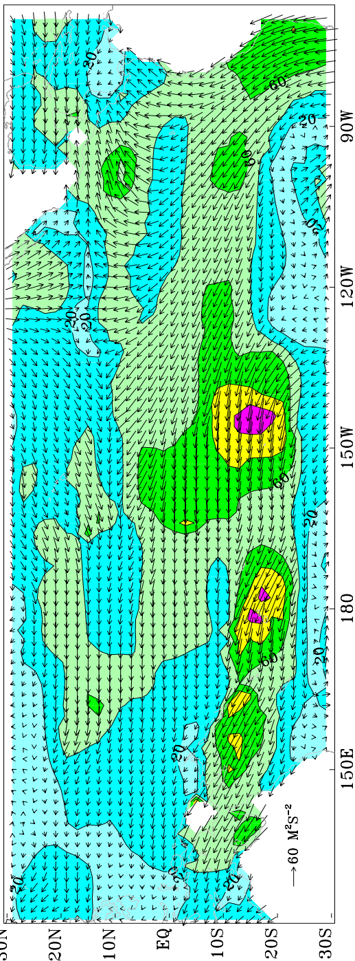
Near-real-time Objective FSU Pseudo-stress Magnitude and Vectors (10m) September 2010
