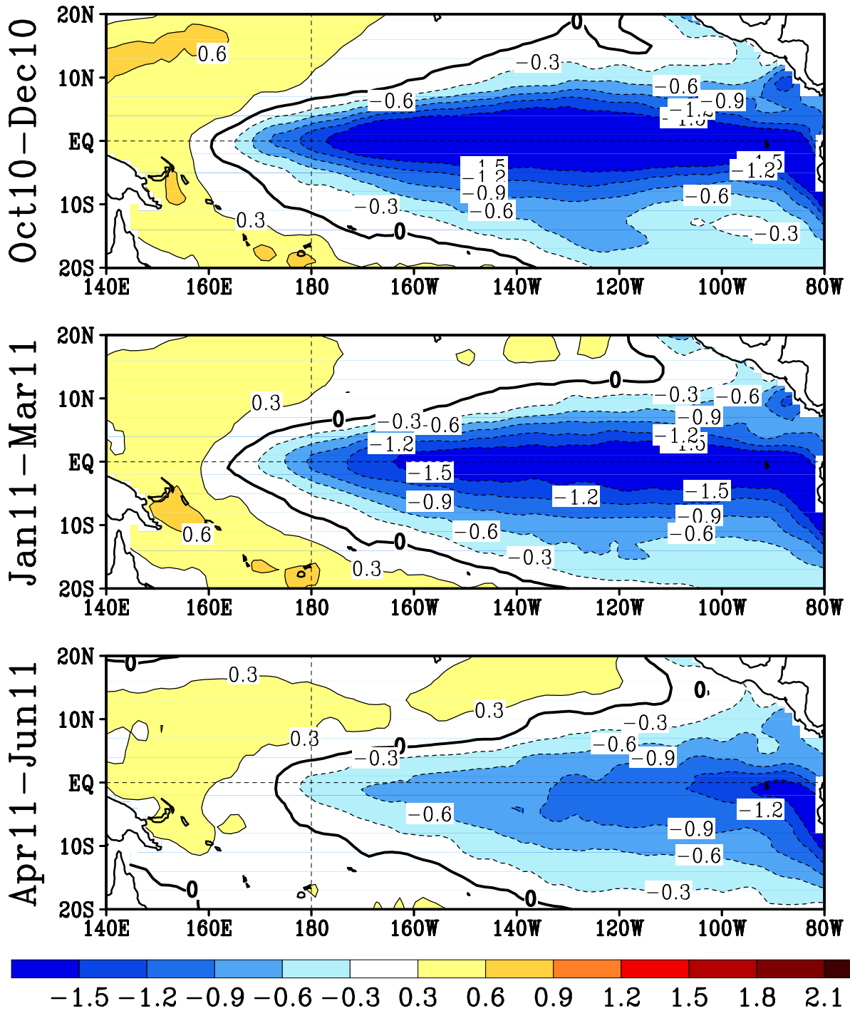
FIGURE F5. Predicted 3-month average sea surface temperature anomalies from the NCEP/CPC Markov model (Xue et al. 2000, J. Climate , 13 , 849-871). The forecast is initiated in SEP 2010. Contour interval is 0.3C and negative anomalies are indicated by dashed contours. Anomalies are calculated relative to the 1971-2000 climatology.
