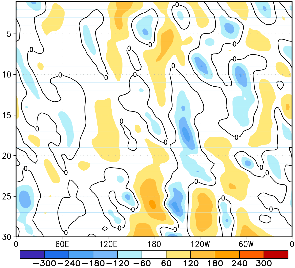
FIGURE E12. Northern Hemisphere: Daily 500-hPa height anomalies for SEP 2010 averaged over the 5° latitude band centered on 40°N. Positive values are indicated by solid contours and dark shading. Negative values are indicated by dashed contours and light shading. Contour interval is 60 m. Anomalies are departures from the 1979-95 base period daily means.
