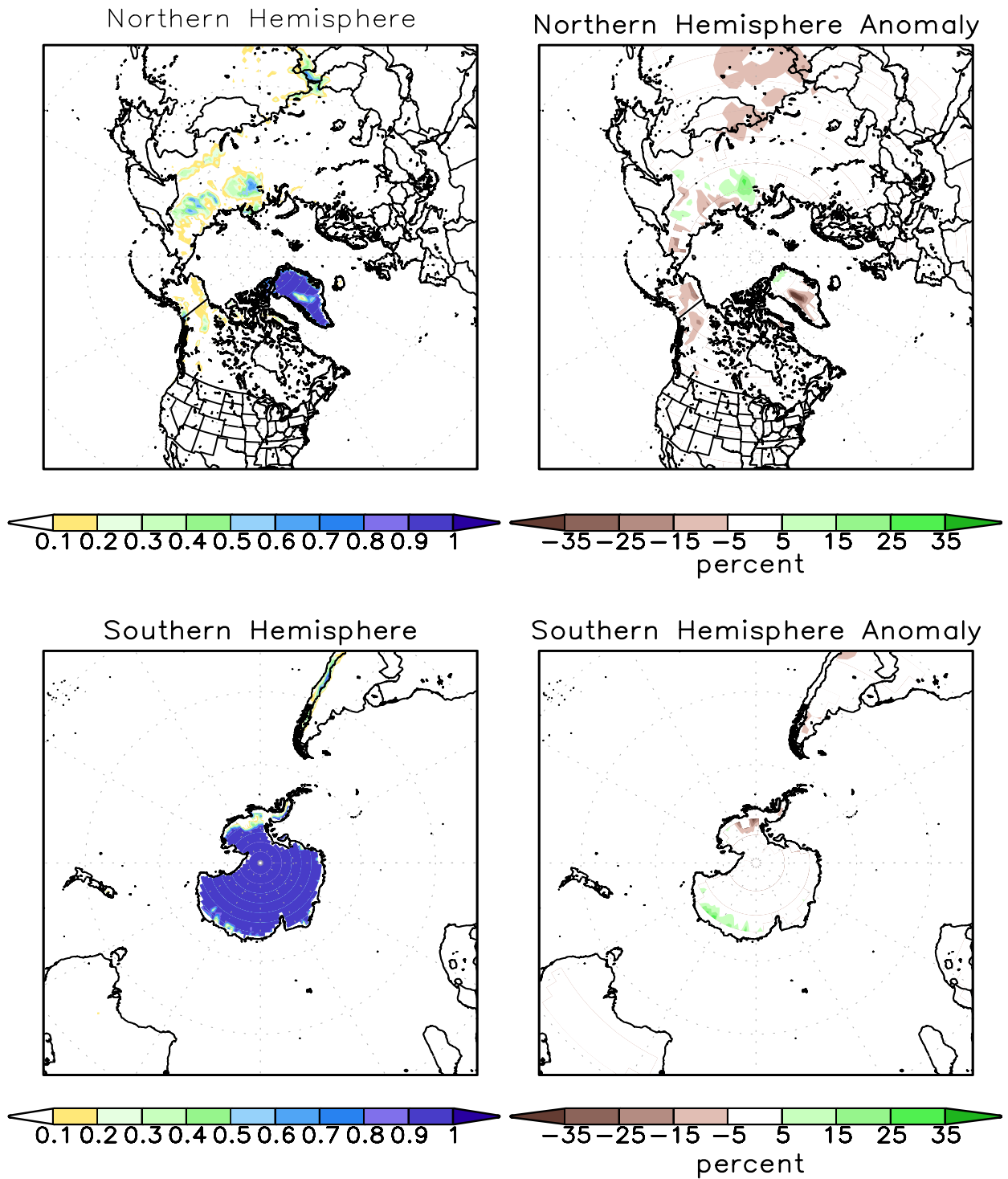
FIGURE A2.2. SSM/I derived snow cover frequency (%) (left) and snow cover anomaly (%) (right) for the month of SEP 2010 based on 1987 - 2006 base period for the Northern Hemisphere (top) and Southern Hemisphere (bottom). It is generated using the algorithm described by Ferraro et. al, 1996, Bull. Amer. Meteor. Soc., vol 77, 891-905.
