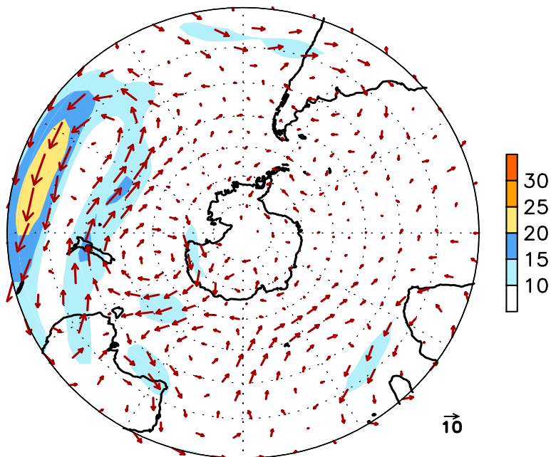
FIGURE E16. Southern Hemisphere mean (left) and anomalous (right) 300-hPa vector wind (CDAS/Reanalysis) for SEP 2010. Mean (anomaly) isotach contour interval is 10 (5) \text{ms}^{-1} . Values greater than 30 \text{ms}^{-1} (left) and 10 \text{ms}^{-1} (rights) are shaded. Anomalies are departures from the 1979-95 base period monthly means.
