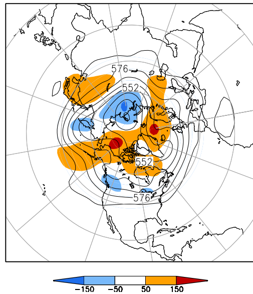
500-hPa Height (dm) & Anomalies (m) (Sep 1–15, 2010)
