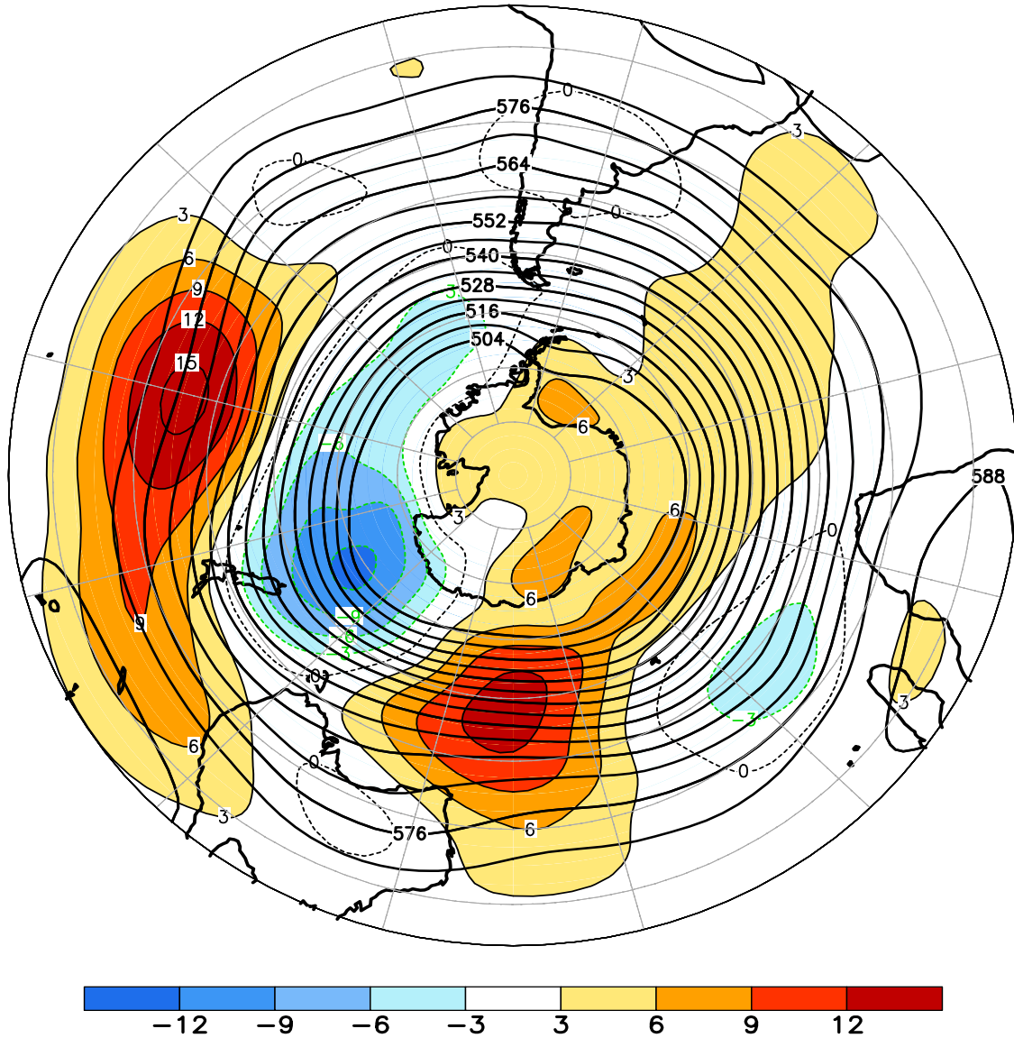
FIGURE E15. Southern Hemisphere mean and anomalous 500-hPa geopotential height (CDAS/Reanalysis) for SEP 2010. Mean heights are denoted by solid contours drawn at an interval of 6 dam. Anomaly contour interval is 3 dam with values less (greater) than -3 dam (3 dam) indicated by dark (light) shading. Anomalies are calculated as departures from the 1979-95 base period monthly means.
