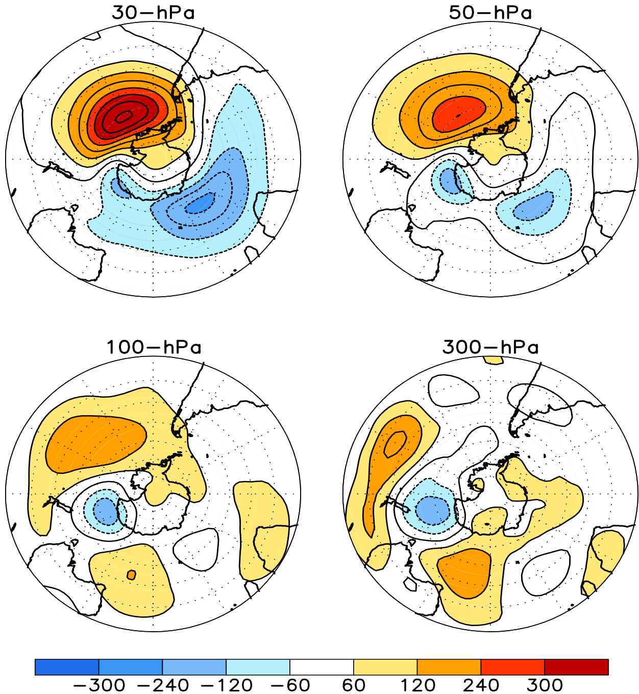
FIGURE S1. Stratospheric height anomalies (m) at selected levels for SEP 2010. Positive values are indicated by solid contours and dark shading. Negative values are indicated by dashed contours and light shading. Contour interval is 60 m. Anomalies are calculated from the 1979–95 base period means. Winter Hemisphere is shown.
