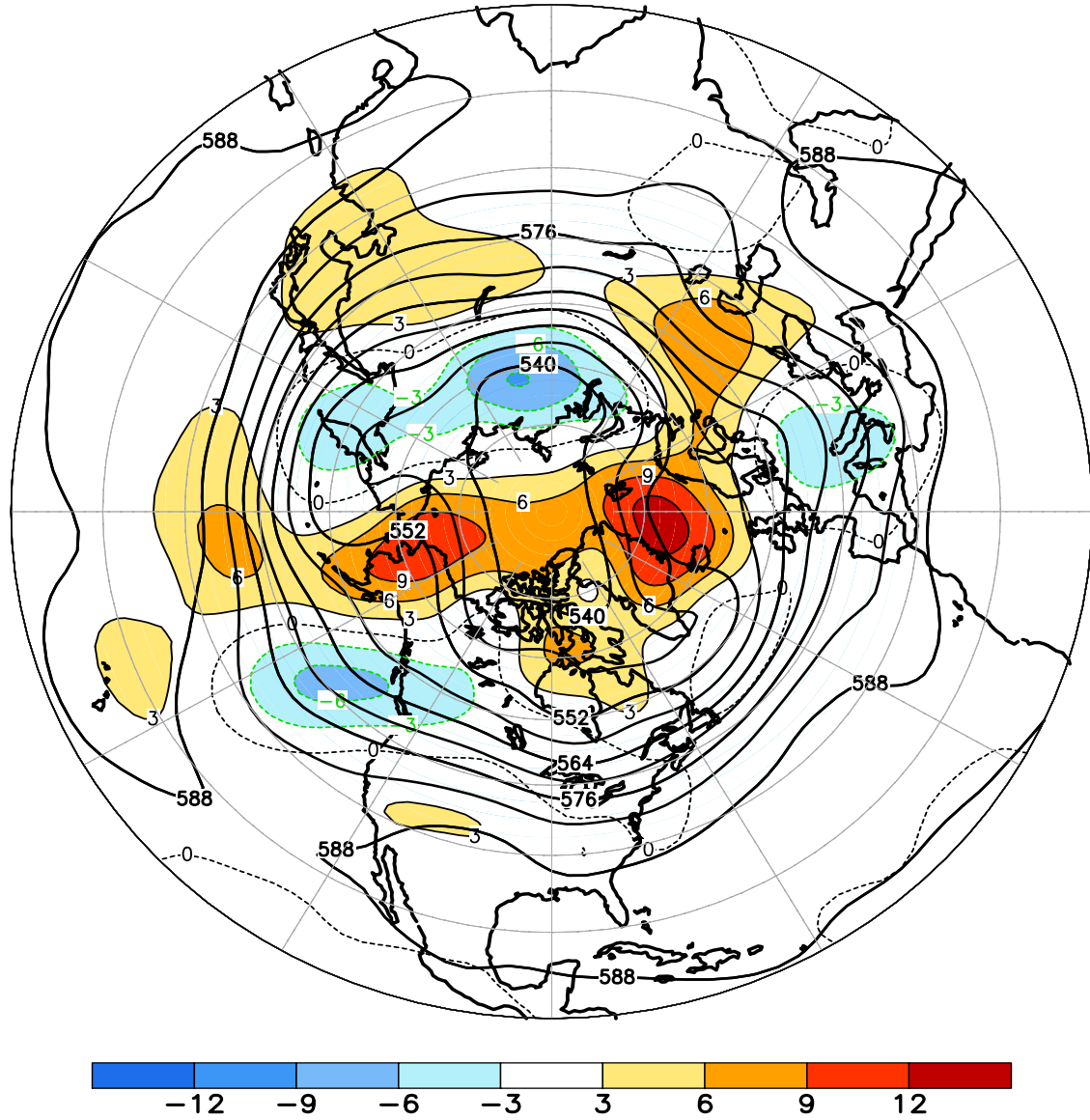
FIGURE E9. Northern Hemisphere mean and anomalous 500-hPa geopotential height (CDAS/Reanalysis) for SEP 2010. Mean heights are denoted by solid contours drawn at an interval of 6 dam. Anomaly contour interval is 3 dam with values less (greater) than -3 dam (3 dam) indicated by dark (light) shading. Anomalies are calculated as departures from the 1979-95 base period monthly means.
