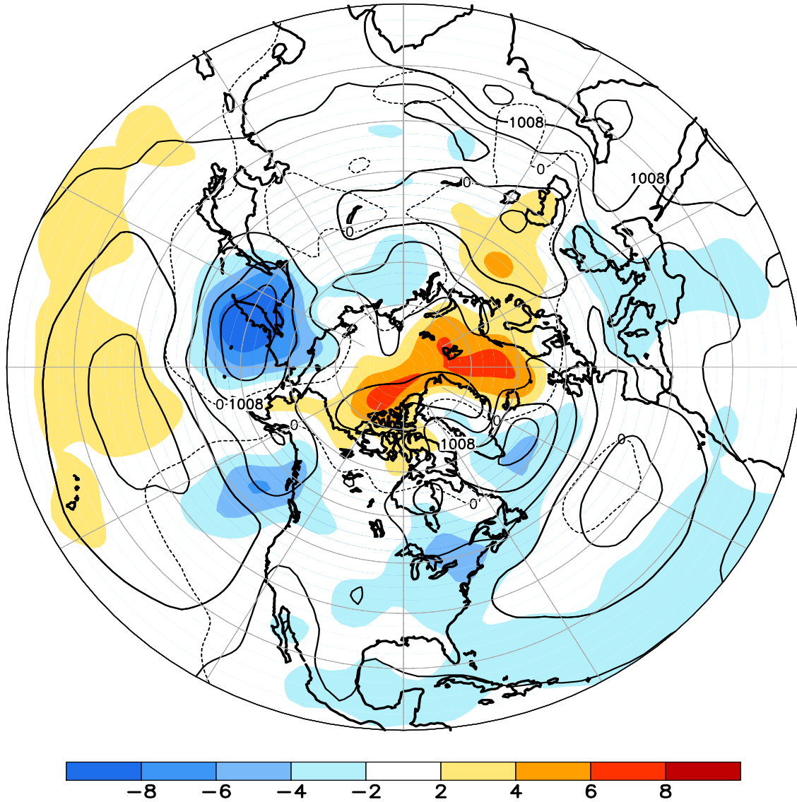
FIGURE E8. Northern Hemisphere mean and anomalous sea level pressure (CDAS/Reanalysis) for SEP 2010. Mean values are denoted by solid contours drawn at an interval of 4 hPa. Anomaly contour interval is 2 hPa with values less (greater) than -2 hPa (2 hPa) indicated by dark (light) shading. Anomalies are calculated as departures from the 1979-95 base period monthly means.
