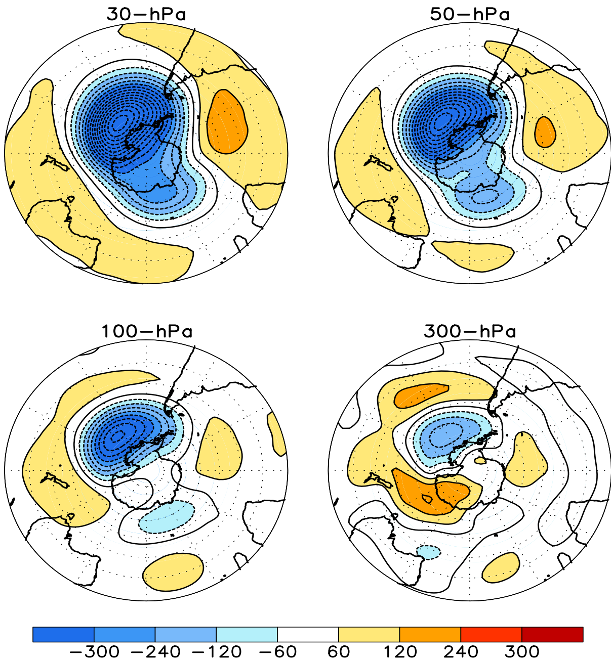
FIGURE S1. Stratospheric height anomalies (m) at selected levels for OCT 2021. Positive values are indicated by solid contours and dark shading. Negative values are indicated by dashed contours and light shading. Contour interval is 60 m. Anomalies are calculated from the 1991-2020 base period means. Winter Hemisphere is shown.
