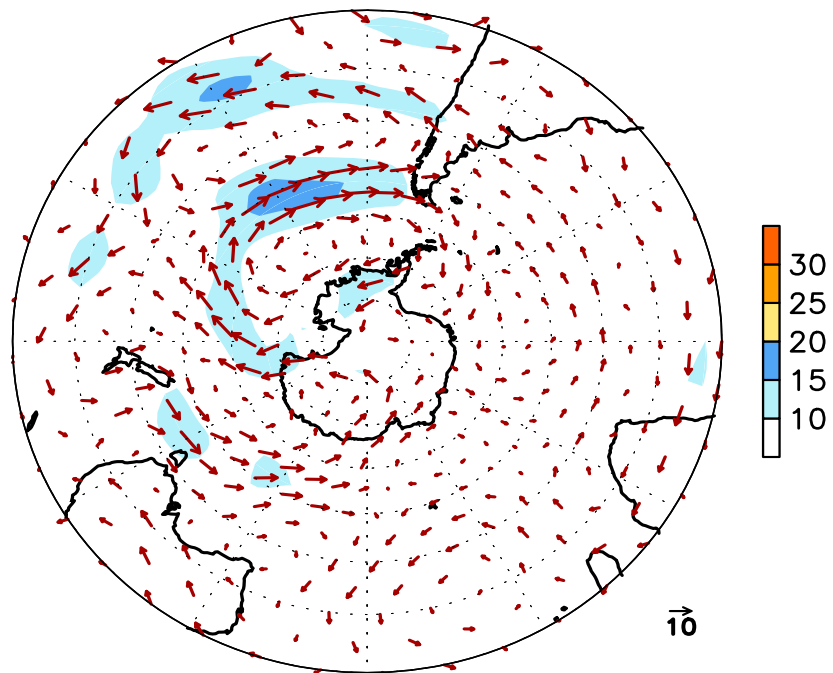
FIGURE E16. Southern Hemisphere mean (left) and anomalous (right) 300-hPa vector wind (CDAS/Reanalysis) for OCT 2021. Mean (anomaly) isotach contour interval is 10 (5) ms -1 . Values greater than 30 ms -1 (left) and 10 ms -1 (rights) are shaded. Anomalies are departures from the 1991-2020 base period monthly means.
