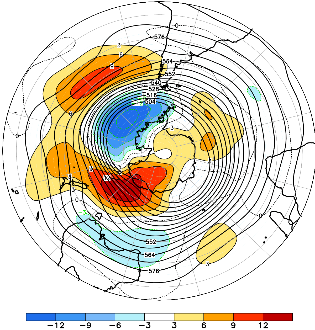
FIGURE E15. Southern Hemisphere mean and anomalous 500-hPa geopotential height (CDAS/Reanalysis) for OCT 2021. Mean heights are denoted by solid contours drawn at an interval of 6 dam. Anomaly contour interval is 3 dam with values less (greater) than -3 dam (3 dam) indicated by dark (light) shading. Anomalies are calculated as departures from the 1991-2020 base period monthly means.
