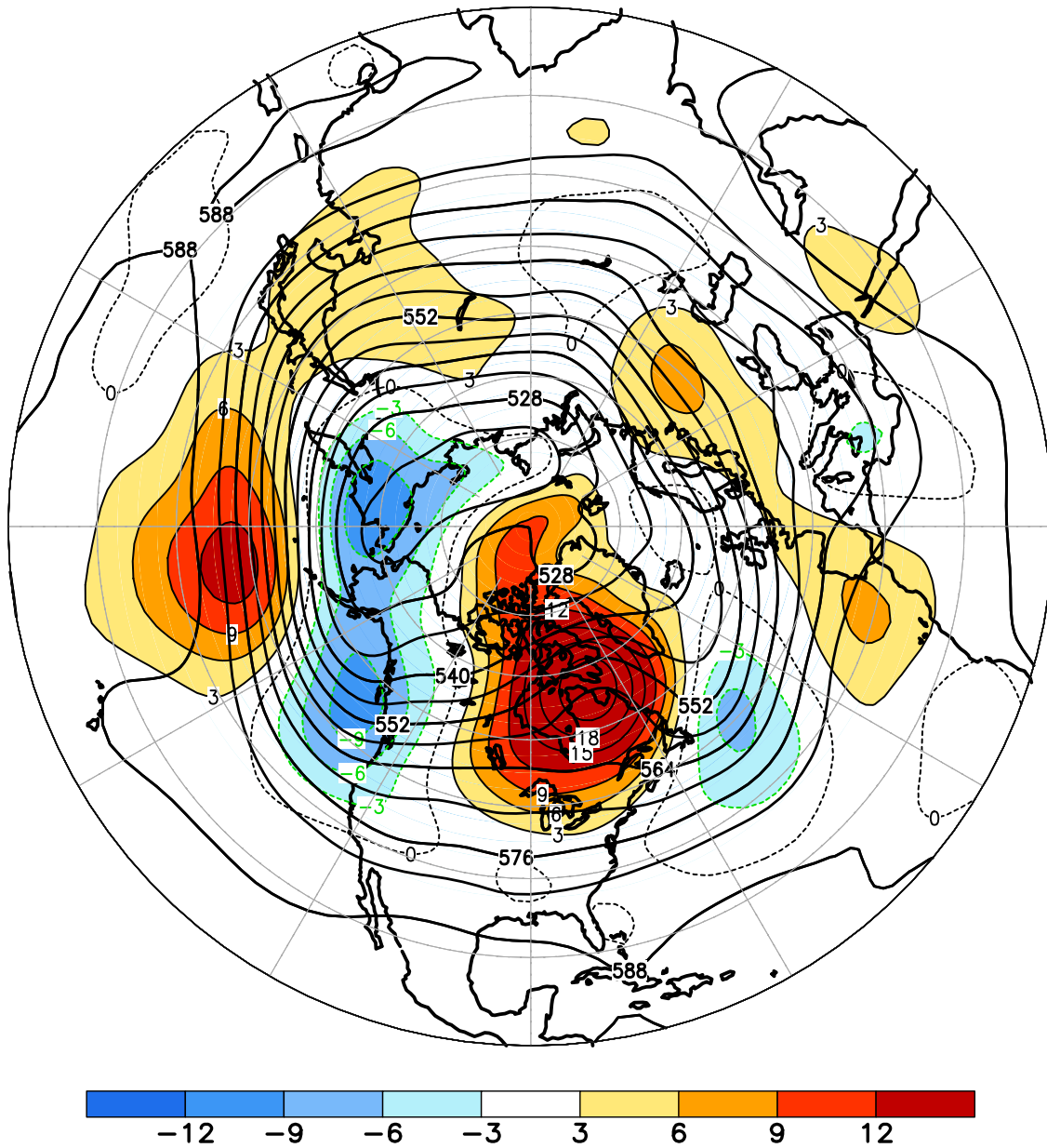
FIGURE E9. Northern Hemisphere mean and anomalous 500-hPa geopotential height (CDAS/Reanalysis) for OCT 2021. Mean heights are denoted by solid contours drawn at an interval of 6 dam. Anomaly contour interval is 3 dam with values less (greater) than -3 dam (3 dam) indicated by dark (light) shading. Anomalies are calculated as departures from the 1991-2020 base period monthly means.
