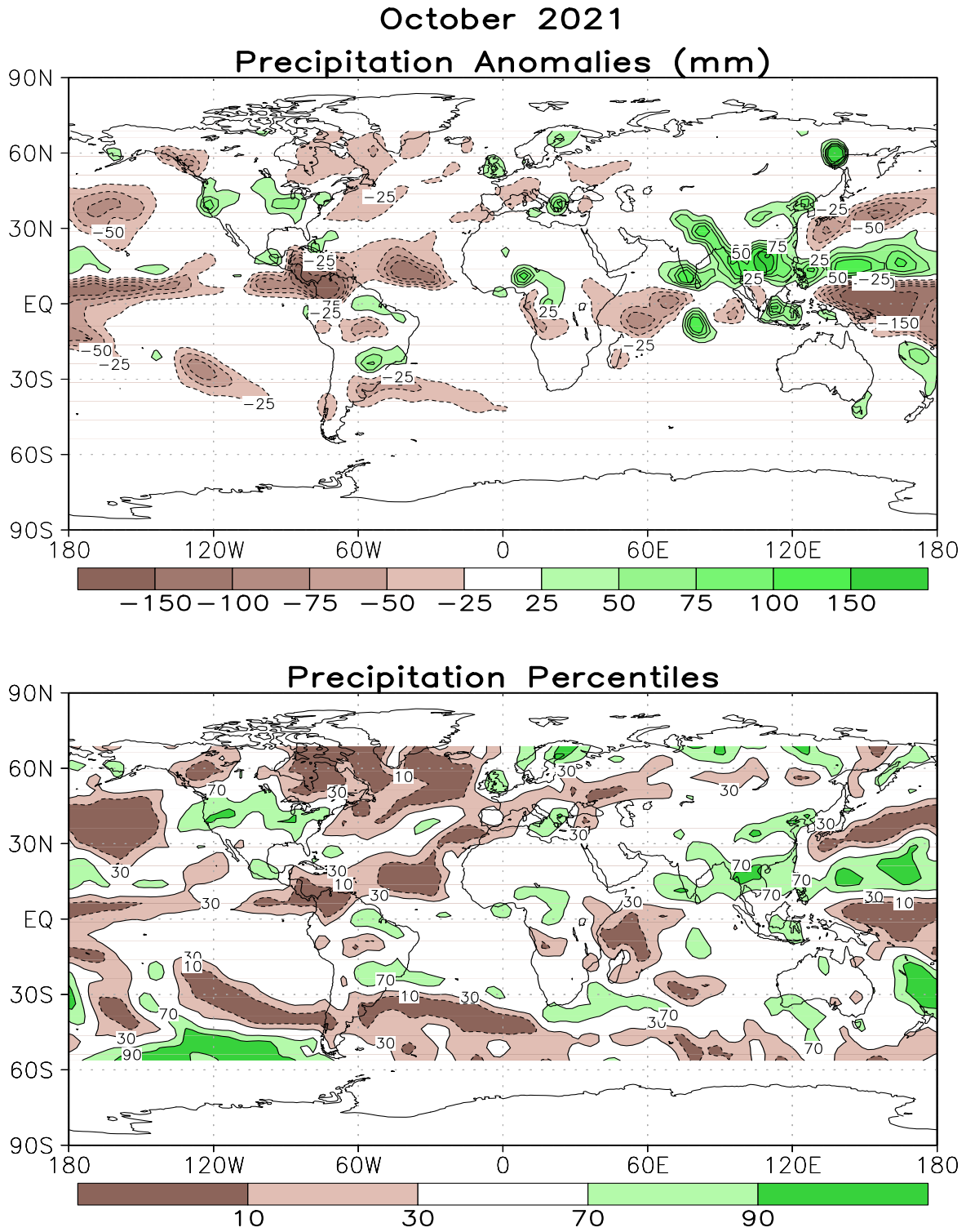
FIGURE E3. Anomalous precipitation (mm, top) and precipitation percentiles based on a Gamma distribution fit to the 1981-2010 base period data (bottom) for OCT 2021. Data are obtained from a merge of raingauge observations and satellite-derived precipitation estimates (Janowiak and Xie 1999, J. Climate , 12, 3335–3342). Contours are drawn at 200, 100, 50, 25, -25, -50, -100, and -200 mm in top panel. Percentiles are not plotted in regions where mean monthly precipitation is <5mm/month.
