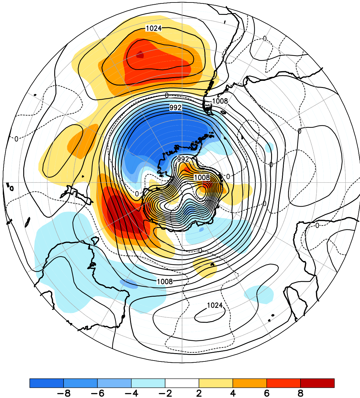
FIGURE E14. Southern Hemisphere mean and anomalous sea level pressure(CDAS/Reanalysis) for OCT 2021. Mean values are denoted by solid contours drawn at an interval of 4 hPa. Anomaly contour interval is 2 hPa with values less (greater) than -2 hPa (2 hPa) indicated by dark (light) shading. Anomalies are calculated as departures from the 1991-2020 base period monthly means.
