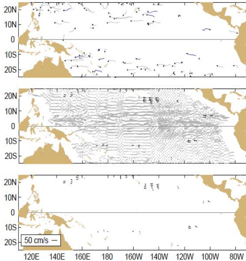
Figure A1.1 Top: Movements of drifting buoys in the tropical Pacific Ocean during October 2017. The linear segments of each trajectory represent a one week displacement. Trajectories of buoys which have lost their subsurface drogues are gray; those with drogues are black.
