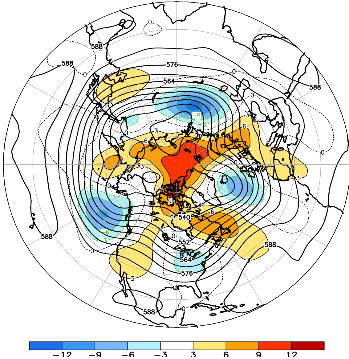
FIGURE E9. Northern Hemisphere mean and anomalous 500-hPa geopotential height (CDAS/Reanalysis) for OCT 2014. Mean heights are denoted by solid contours drawn at an interval of 6 dam. Anomaly contour interval is 3 dam with values less (greater) than -3 dam (3 dam) indicated by dark (light) shading. Anomalies are calculated as departures from the 1981-2010 base period monthly means.
