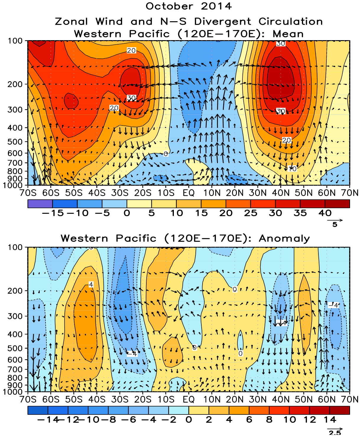
FIGURE T31. Pressure-latitude section of the mean (top) and anomalous (bottom) zonal wind ( m s^{-1} ) and divergent circulation averaged over the west Pacific sector (120E–170E). The divergent circulation is represented by vectors of combined pressure vertical velocity and the divergent component of the meridional wind. Red shading and solid contours denote a westerly (top) or anomalous westerly (bottom) zonal wind. Blue shading and dashed contours denote an easterly (top) or anomalous easterly (bottom) zonal wind. Anomalies are departures from the 1981–2010 base period monthly means.
