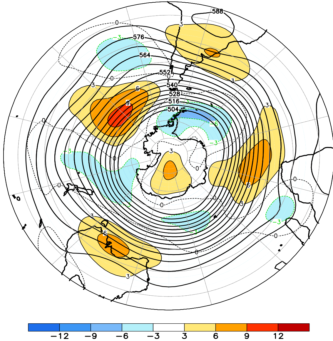
FIGURE E15. Southern Hemisphere mean and anomalous 500-hPa geopotential height (CDAS/Reanalysis) for OCT 2014. Mean heights are denoted by solid contours drawn at an interval of 6 dam. Anomaly contour interval is 3 dam with values less (greater) than -3 dam (3 dam) indicated by dark (light) shading. Anomalies are calculated as departures from the 1981-2010 base period monthly means.
