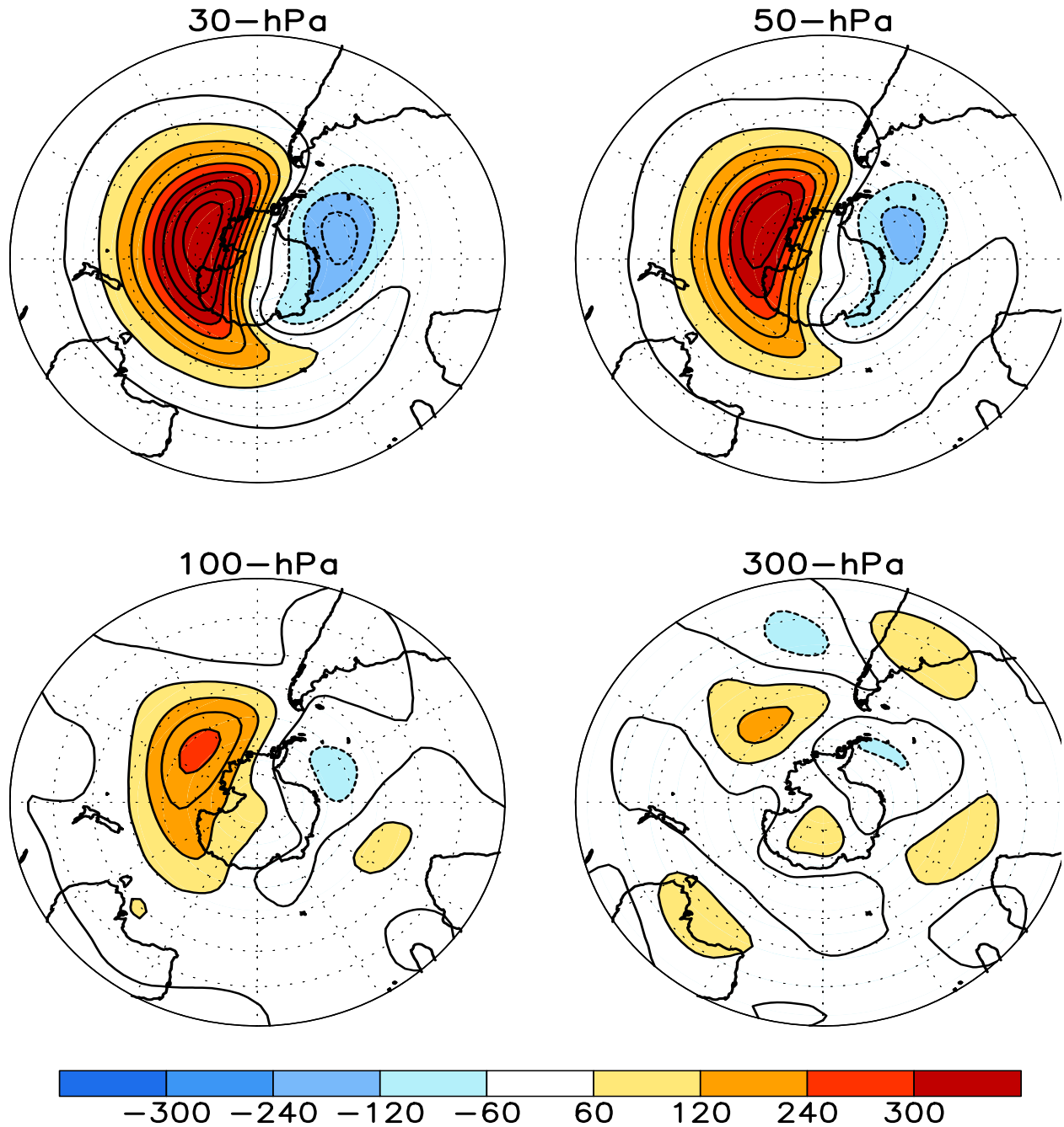
FIGURE S1. Stratospheric height anomalies (m) at selected levels for OCT 2014. Positive values are indicated by solid contours and dark shading. Negative values are indicated by dashed contours and light shading. Contour interval is 60 m. Anomalies are calculated from the 1981-2010 base period means. Winter Hemisphere is shown.
