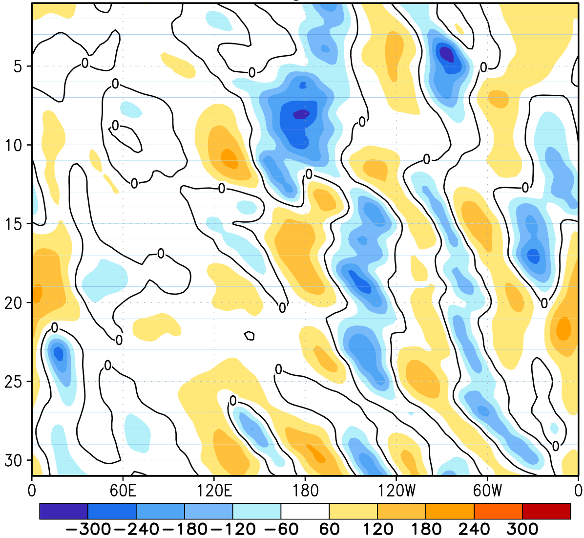
FIGURE E12. Northern Hemisphere: Daily 500-hPa height anomalies for OCT 2014 averaged over the 5° latitude band centered on 40°N. Positive values are indicated by solid contours and dark shading. Negative values are indicated by dashed contours and light shading. Contour interval is 60 m. Anomalies are departures from the 1981-2010 base period daily means.
