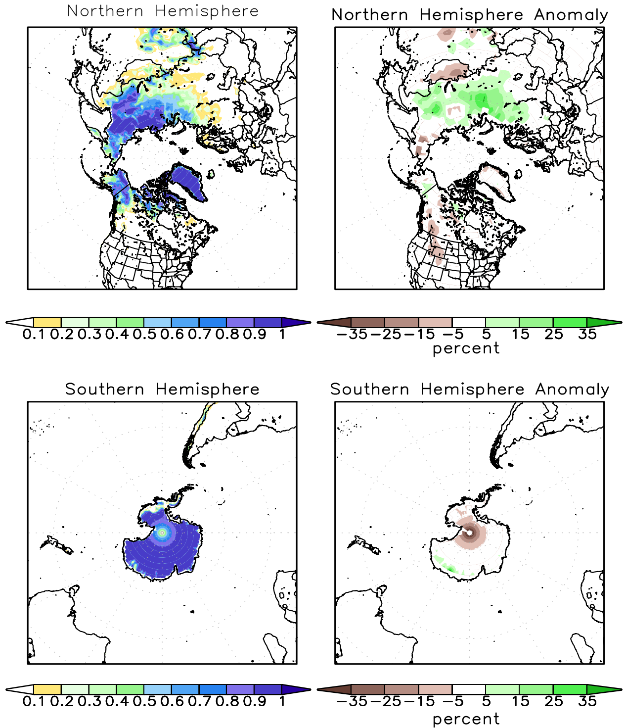
FIGURE A2.2. SSM/I derived snow cover frequency (%) (left) and snow cover anomaly (%) (right) for the month of OCT 2014 based on 1987 - 2010 base period for the Northern Hemisphere (top) and Southern Hemisphere (bottom). It is generated using the algorithm described by Ferraro et. al, 1996, Bull. Amer. Meteor. Soc., vol 77, 891-905.
