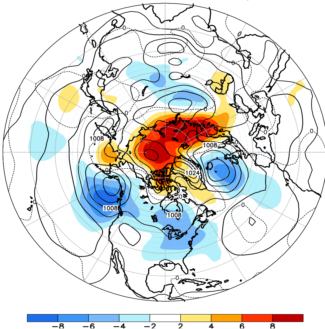
FIGURE E8. Northern Hemisphere mean and anomalous sea level pressure (CDAS/Reanalysis) for OCT 2014. Mean values are denoted by solid contours drawn at an interval of 4 hPa. Anomaly contour interval is 2 hPa with values less (greater) than -2 hPa (2 hPa) indicated by dark (light) shading. Anomalies are calculated as departures from the 1981-2010 base period monthly means.
