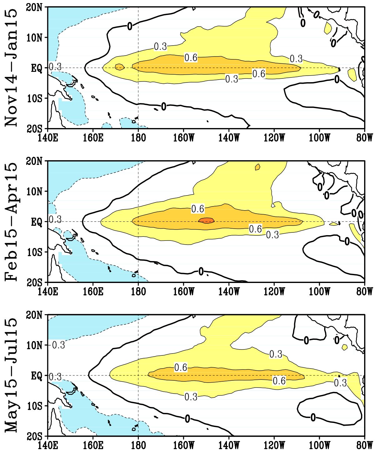
FIGURE F5. Predicted 3-month average sea surface temperature anomalies from the NCEP/CPC Markov model (Xue et al. 2000, J. Climate , 13 , 849-871). The forecast is initiated in OCT 2014 . Contour interval is 0.3C and negative anomalies are indicated by dashed contours. Anomalies are calculated relative to the 1971-2000 climatology.
