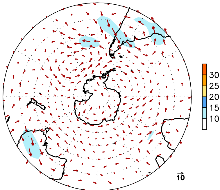
FIGURE E16. Southern Hemisphere mean (left) and anomalous (right) 300-hPa vector wind (CDAS/Reanalysis) for OCT 2014. Mean (anomaly) isotach contour interval is 10 (5) \text{ms}^{-1} . Values greater than 30 \text{ms}^{-1} (left) and 10 \text{ms}^{-1} (rights) are shaded. Anomalies are departures from the 1981-2010 base period monthly means.
