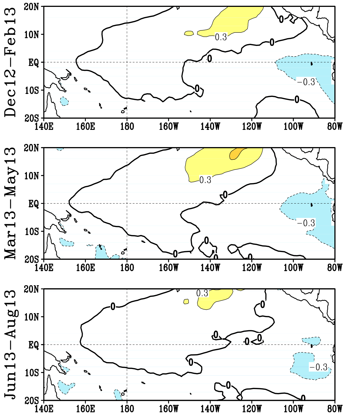
FIGURE F5. Predicted 3-month average sea surface temperature anomalies from the NCEP/CPC Markov model (Xue et al. 2000, J. Climate , 13 , 849-871). The forecast is initiated in NOV 2012. Contour interval is 0.3C and negative anomalies are indicated by dashed contours. Anomalies are calculated relative to the 1971-2000 climatology.
