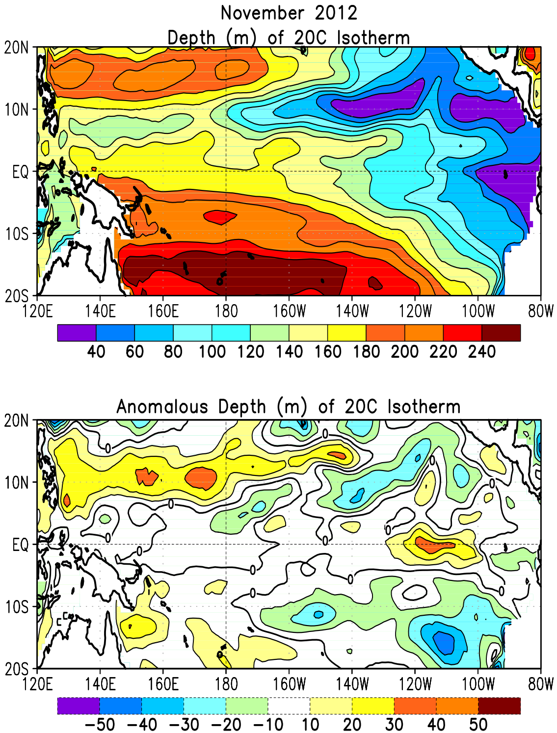
FIGURE T16. Mean (top) and anomalous (bottom) depth of the 20°C isotherm for NOV 2012. Contour interval is 40 m (top) and 10 m (bottom). Dashed contours in bottom panel indicate negative anomalies. Data are derived from the NCEP’s global ocean data assimilation system version 2 which assimilates oceanic observations into an oceanic GCM (Xue, Y. and Behringer, D.W., 2006: Operational global ocean data assimilation system at NCEP, to be submitted to BAMS). Anomalies are departures from the 1981–2010 base period means.
