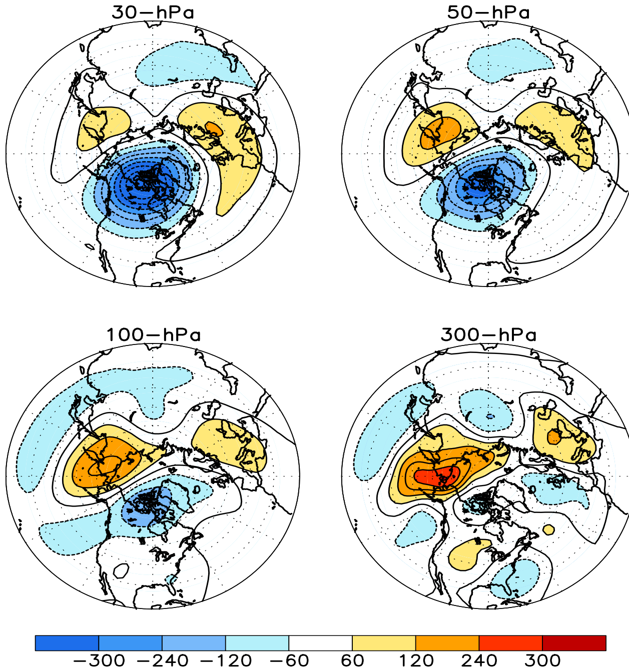
FIGURE S1. Stratospheric height anomalies (m) at selected levels for NOV 2012. Positive values are indicated by solid contours and dark shading. Negative values are indicated by dashed contours and light shading. Contour interval is 60 m. Anomalies are calculated from the 1981-2010 base period means. Winter Hemisphere is shown.
