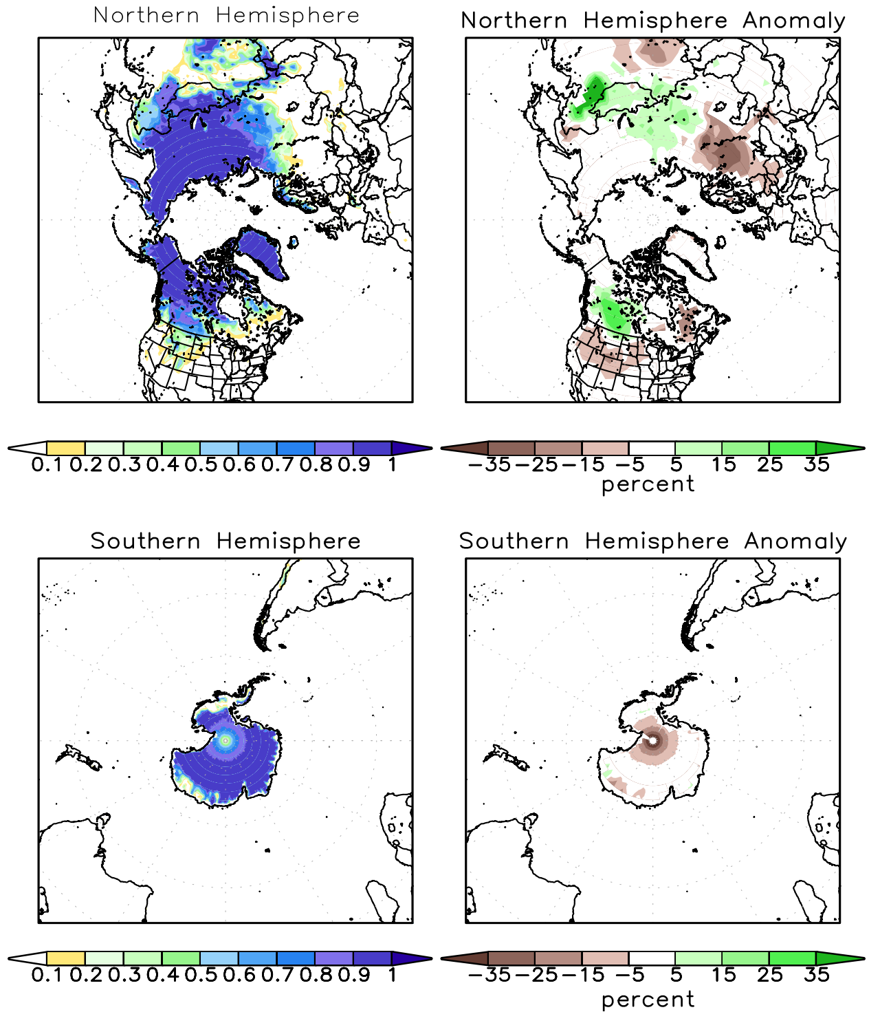
FIGURE A2.2. SSM/I derived snow cover frequency (%) (left) and snow cover anomaly (%) (right) for the month of NOV 2012 based on 1987 - 2010 base period for the Northern Hemisphere (top) and Southern Hemisphere (bottom). It is generated using the algorithm described by Ferraro et. al, 1996, Bull. Amer. Meteor. Soc., vol 77, 891-905.
