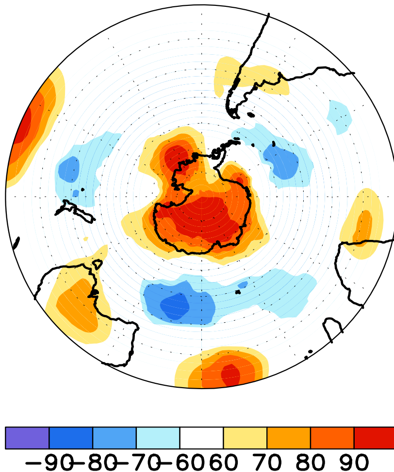
FIGURE E17. Southern Hemisphere percentage of days during NOV 2012 in which 500-hPa height anomalies greater than 15 m (red) and less than -15 m (blue) were observed. Values greater than 70% are shaded and contour in-
