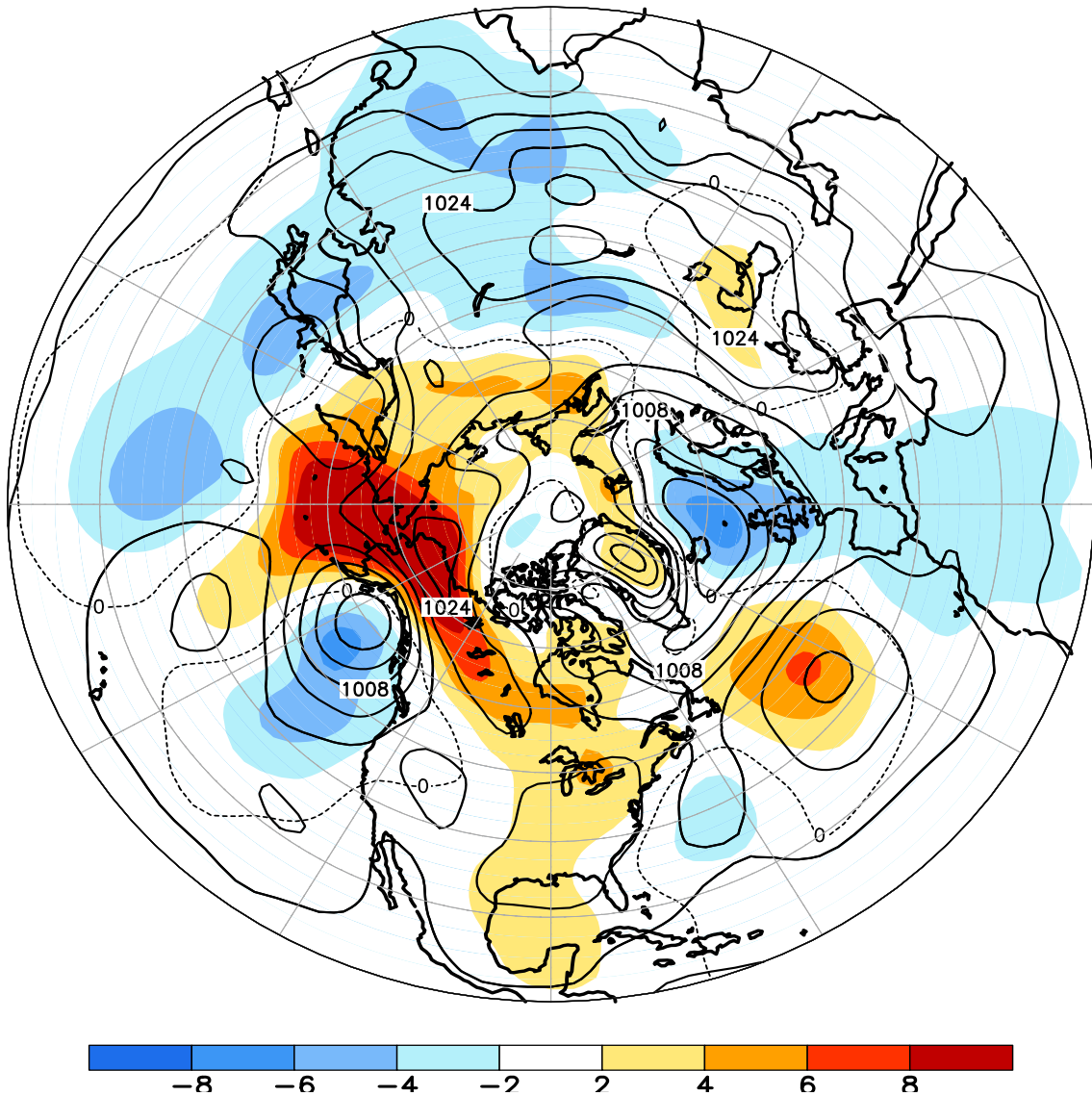
FIGURE E8. Northern Hemisphere mean and anomalous sea level pressure (CDAS/Reanalysis) for NOV 2012. Mean values are denoted by solid contours drawn at an interval of 4 hPa. Anomaly contour interval is 2 hPa with values less (greater) than -2 hPa (2 hPa) indicated by dark (light) shading. Anomalies are calculated as departures from the 1981-2010 base period monthly means.
