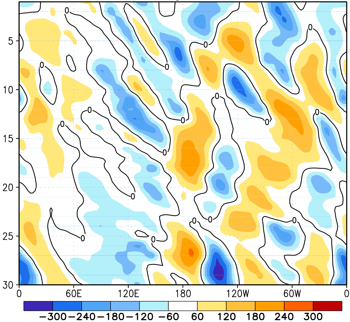
FIGURE E12. Northern Hemisphere: Daily 500-hPa height anomalies for NOV 2012 averaged over the 5° latitude band centered on 40°N. Positive values are indicated by solid contours and dark shading. Negative values are indicated by dashed contours and light shading. Contour interval is 60 m. Anomalies are departures from the 1981-2010 base period daily means.
