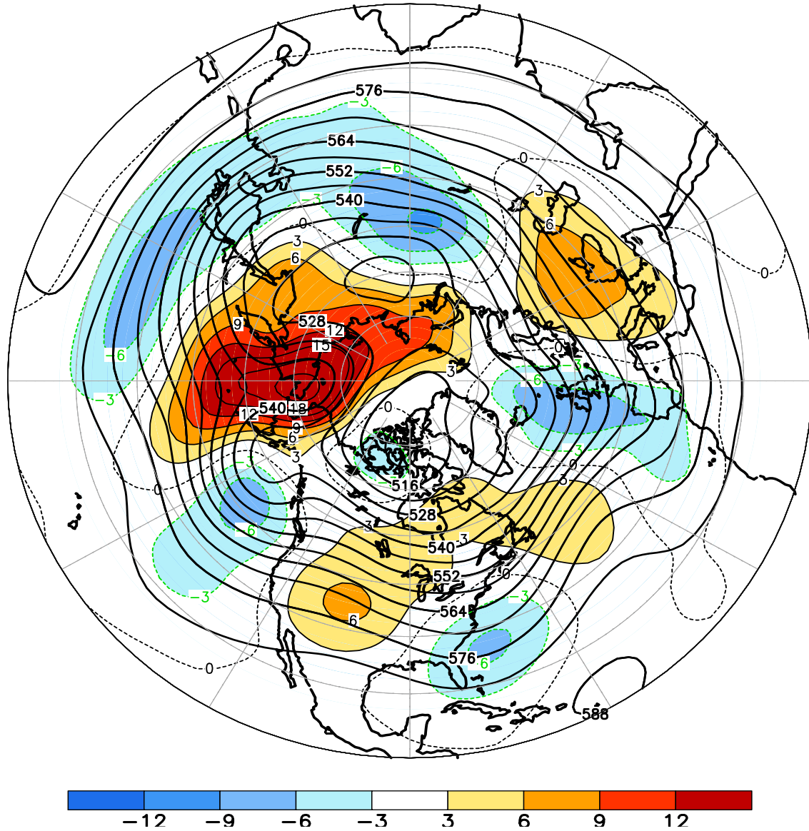
FIGURE E9. Northern Hemisphere mean and anomalous 500-hPa geopotential height (CDAS/Reanalysis) for NOV 2012. Mean heights are denoted by solid contours drawn at an interval of 6 dam. Anomaly contour interval is 3 dam with values less (greater) than -3 dam (3 dam) indicated by dark (light) shading. Anomalies are calculated as departures from the 1981-2010 base period monthly means.
