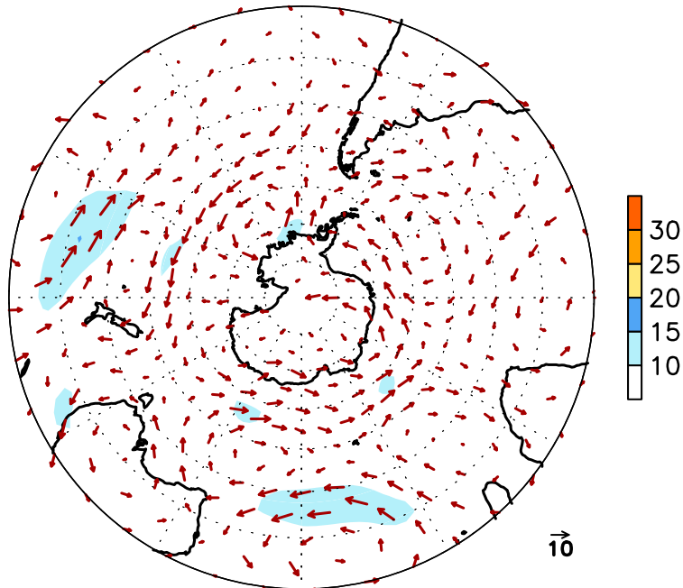
FIGURE E16. Southern Hemisphere mean (left) and anomalous (right) 300-hPa vector wind (CDAS/Reanalysis) for NOV 2012. Mean (anomaly) isotach contour interval is 10 (5) ms -1 . Values greater than 30 ms -1 (left) and 10 ms -1 (rights) are shaded. Anomalies are departures from the 1981-2010 base period monthly means.
