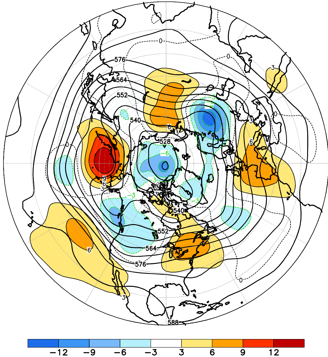
FIGURE E9. Northern Hemisphere mean and anomalous 500-hPa geopotential height (CDAS/Reanalysis) for MAY 2022. Mean heights are denoted by solid contours drawn at an interval of 6 dam. Anomaly contour interval is 3 dam with values less (greater) than -3 dam (3 dam) indicated by dark (light) shading. Anomalies are calculated as departures from the 1991-2020 base period monthly means.
