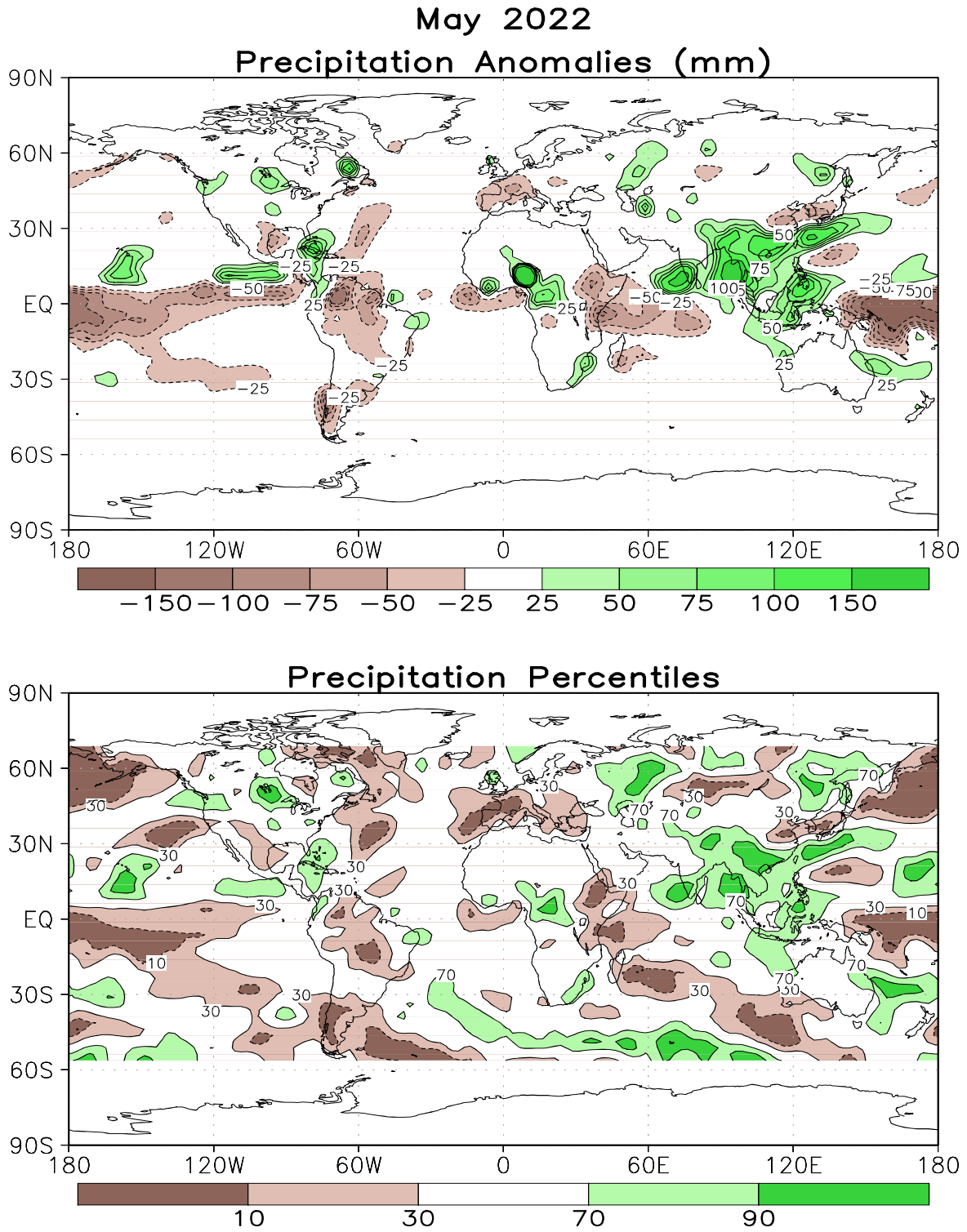
FIGURE E3. Anomalous precipitation (mm, top) and precipitation percentiles based on a Gamma distribution fit to the 1981-2010 base period data (bottom) for MAY 2022. Data are obtained from a merge of raingauge observations and satellite-derived precipitation estimates (Janowiak and Xie 1999, J. Climate , 12 , 3335–3342). Contours are drawn at 200, 100, 50, 25, -25, -50, -100, and -200 mm in top panel. Percentiles are not plotted in regions where mean monthly precipitation is <5mm/month.
