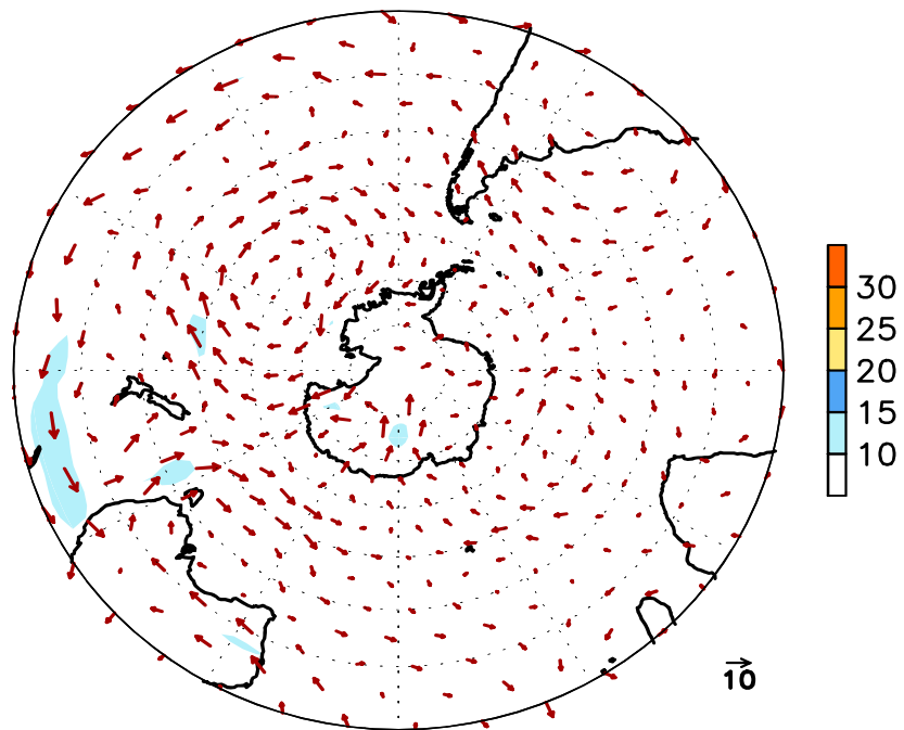
FIGURE E16. Southern Hemisphere mean (left) and anomalous (right) 300-hPa vector wind (CDAS/Reanalysis) for MAY 2022. Mean (anomaly) isotach contour interval is 10 (5) \text{ms}^{-1} . Values greater than 30 \text{ms}^{-1} (left) and 10 \text{ms}^{-1} (rights) are shaded. Anomalies are departures from the 1991-2020 base period monthly means.
