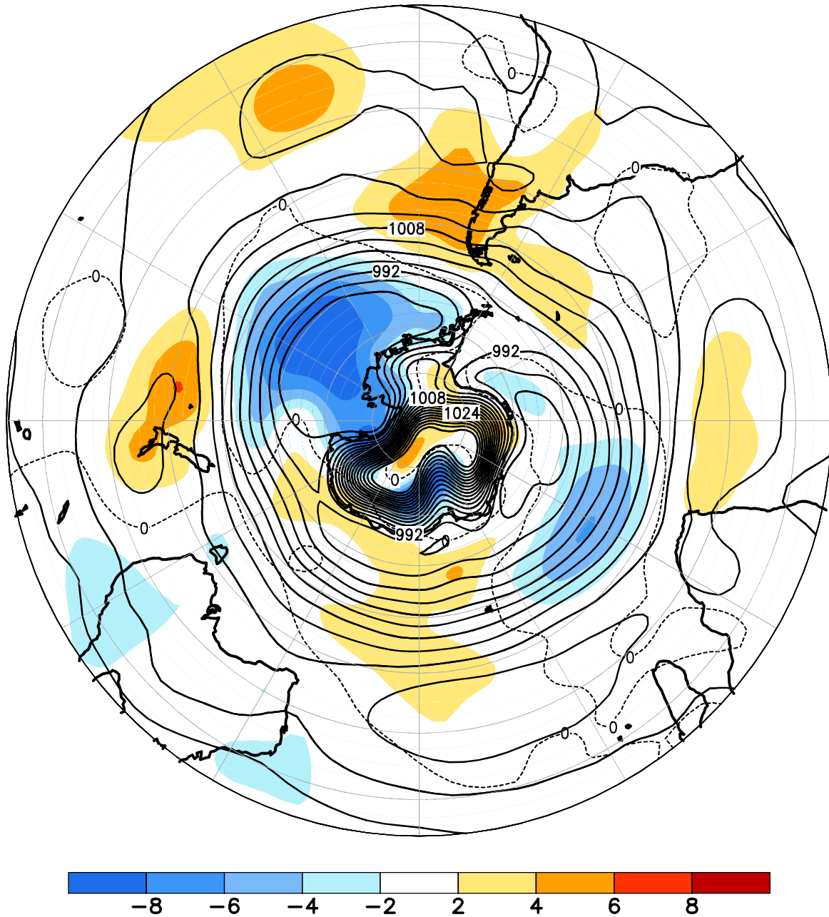
FIGURE E14. Southern Hemisphere mean and anomalous sea level pressure(CDAS/Reanalysis) for MAY 2022. Mean values are denoted by solid contours drawn at an interval of 4 hPa. Anomaly contour interval is 2 hPa with values less (greater) than -2 hPa (2 hPa) indicated by dark (light) shading. Anomalies are calculated as departures from the 1991-2020 base period monthly means.
