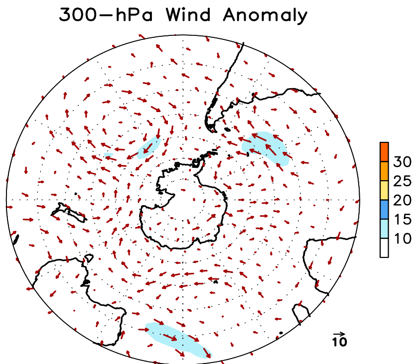
FIGURE E16. Southern Hemisphere mean (left) and anomalous (right) 300-hPa vector wind (CDAS/Reanalysis) for MAY 2021. Mean (anomaly) isotach contour interval is 10 (5) \text{ms}^{-1} . Values greater than 30 \text{ms}^{-1} (left) and 10 \text{ms}^{-1} (rights) are shaded. Anomalies are departures from the 1981-2010 base period monthly means.
