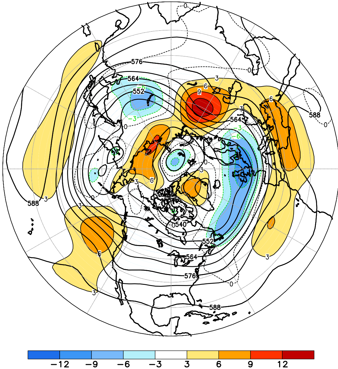
FIGURE E9. Northern Hemisphere mean and anomalous 500-hPa geopotential height (CDAS/Reanalysis) for MAY 2021. Mean heights are denoted by solid contours drawn at an interval of 6 dam. Anomaly contour interval is 3 dam with values less (greater) than -3 dam (3 dam) indicated by dark (light) shading. Anomalies are calculated as departures from the 1981-2010 base period monthly means.
