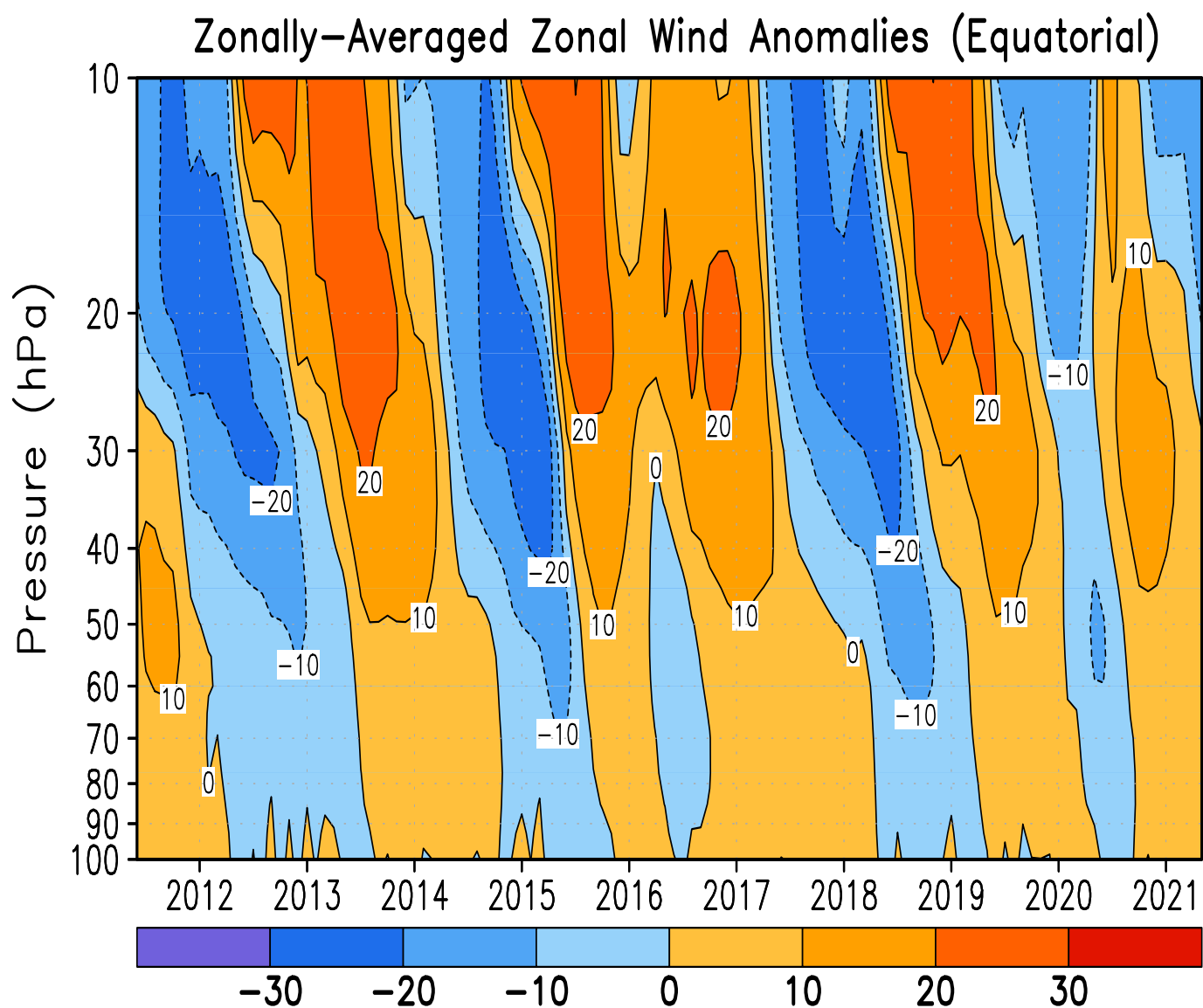
FIGURE T14. Equatorial time-height section of anomalous zonally-averaged zonal wind ( \text{m s}^{-1} ) (CDAS/Reanalysis). Contour interval is 10 \text{m s}^{-1} . Anomalies are departures from the 1981-2010 base period monthly means.
