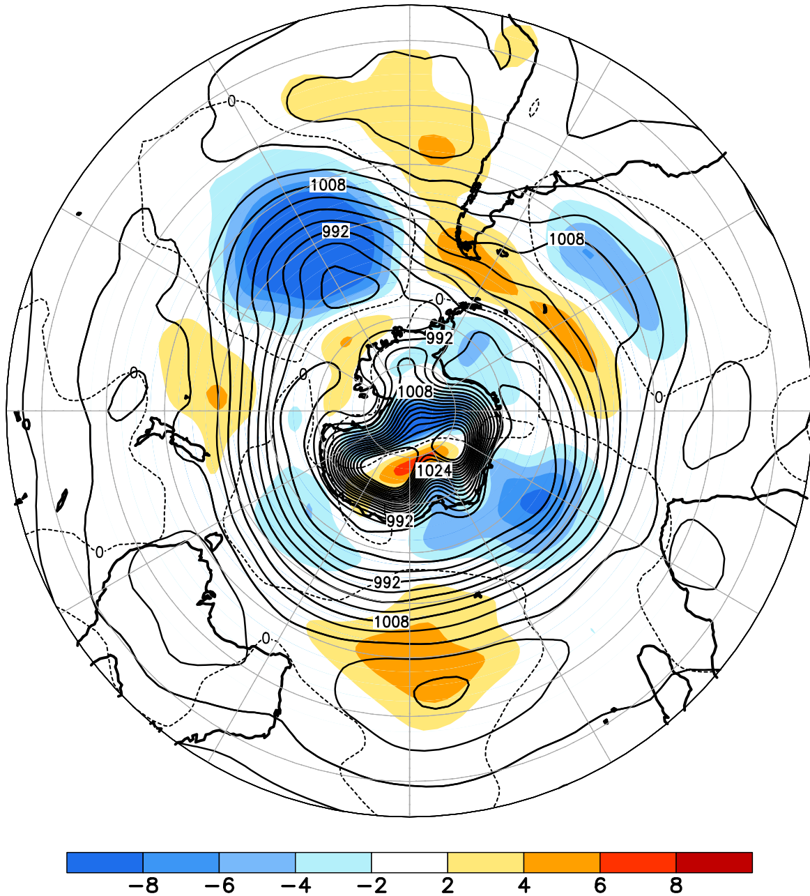
FIGURE E14. Southern Hemisphere mean and anomalous sea level pressure(CDAS/Reanalysis) for MAY 2021. Mean values are denoted by solid contours drawn at an interval of 4 hPa. Anomaly contour interval is 2 hPa with values less (greater) than -2 hPa (2 hPa) indicated by dark (light) shading. Anomalies are calculated as departures from the 1981-2010 base period monthly means.
