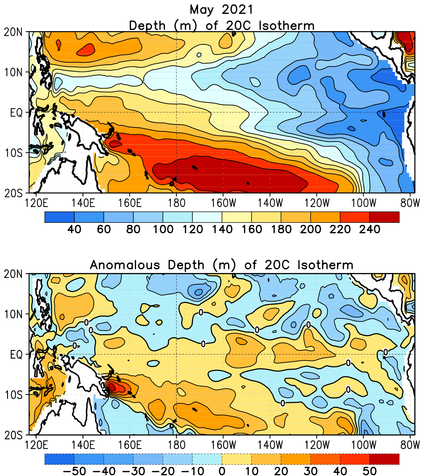
FIGURE T16. Mean (top) and anomalous (bottom) depth of the 20°C isotherm for MAY 2021. Contour interval is 40 m (top) and 10 m (bottom). Dashed contours in bottom panel indicate negative anomalies. Data are derived from the NCEP's global ocean data assimilation system version 2 which assimilates oceanic observations into an oceanic GCM (Xue, Y. and Behringer, D.W., 2006: Operational global ocean data assimilation system at NCEP, to be submitted to BAMS). Anomalies are departures from the 1981–2010 base period means.
