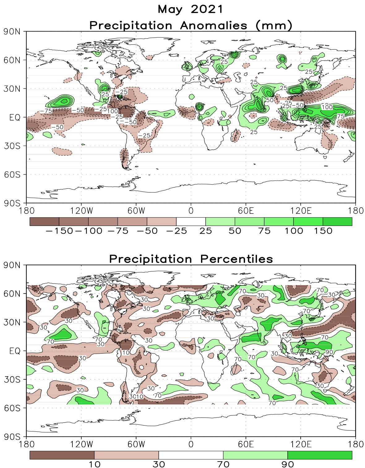
FIGURE E3. Anomalous precipitation (mm, top) and precipitation percentiles based on a Gamma distribution fit to the 1981–2010 base period data (bottom) for MAY 2021. Data are obtained from a merge of raingauge observations and satellite-derived precipitation estimates (Janowiak and Xie 1999, J. Climate , 12 , 3335–3342). Contours are drawn at 200, 100, 50, 25, -25, -50, -100, and -200 mm in top panel. Percentiles are not plotted in regions where mean monthly precipitation is <5mm/month.
