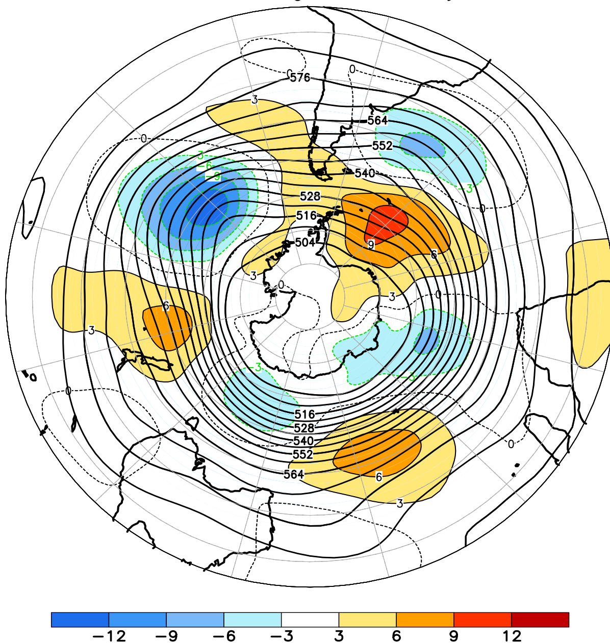
FIGURE E15. Southern Hemisphere mean and anomalous 500-hPa geopotential height (CDAS/Reanalysis) for MAY 2021. Mean heights are denoted by solid contours drawn at an interval of 6 dam. Anomaly contour interval is 3 dam with values less (greater) than -3 dam (3 dam) indicated by dark (light) shading. Anomalies are calculated as departures from the 1981-2010 base period monthly means.
