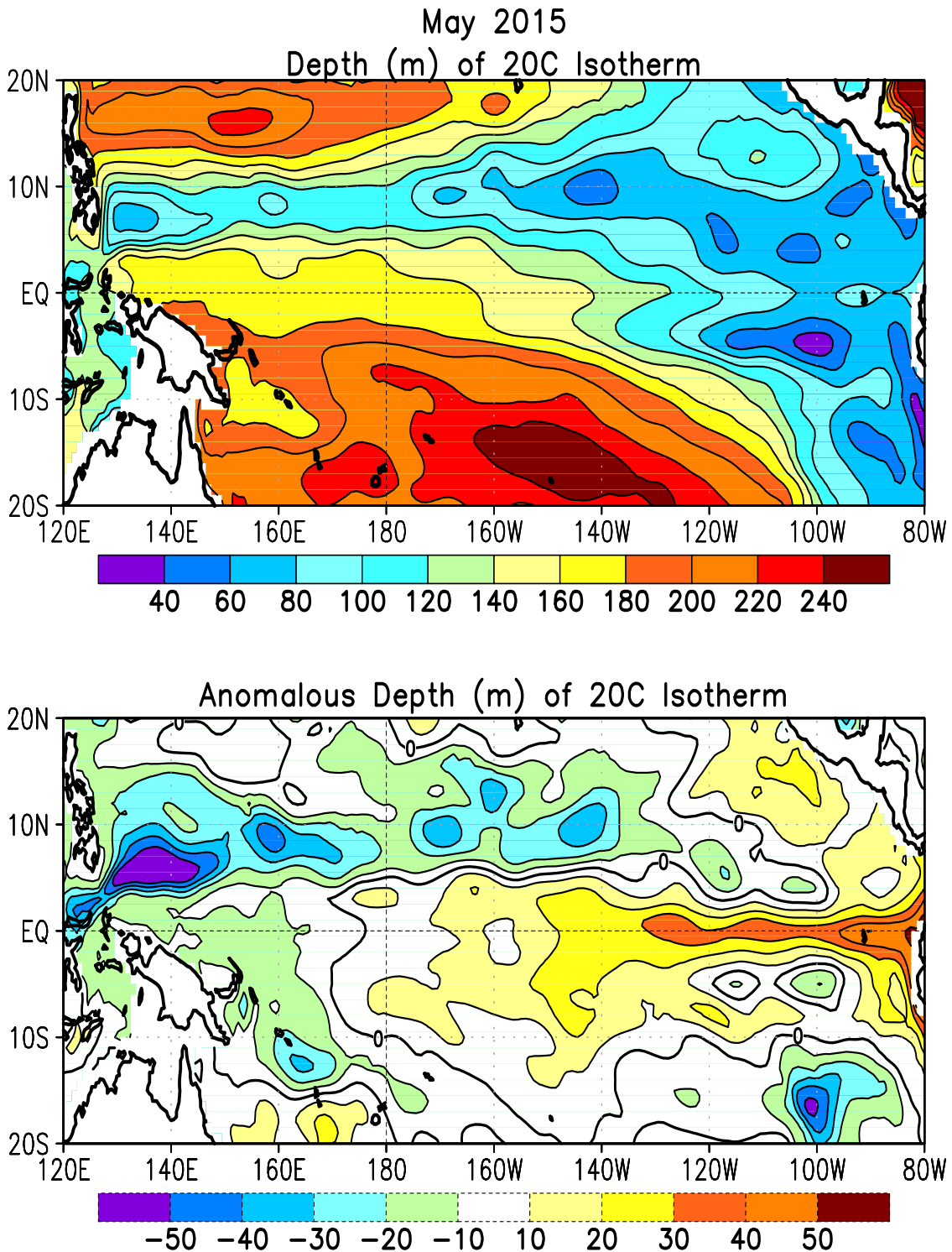
FIGURE T16. Mean (top) and anomalous (bottom) depth of the 20°C isotherm for MAY 2015. Contour interval is 40 m (top) and 10 m (bottom). Dashed contours in bottom panel indicate negative anomalies. Data are derived from the NCEP’s global ocean data assimilation system version 2 which assimilates oceanic observations into an oceanic GCM (Xue, Y. and Behringer, D.W., 2006: Operational global ocean data assimilation system at NCEP, to be submitted to BAMS). Anomalies are departures from the 1981–2010 base period means.
