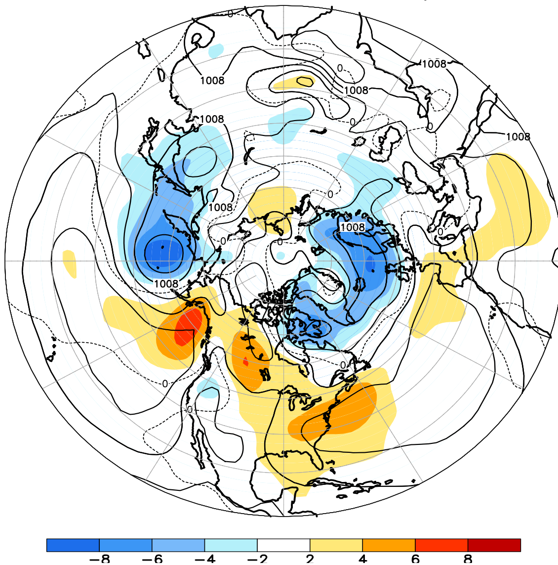
FIGURE E8. Northern Hemisphere mean and anomalous sea level pressure (CDAS/Reanalysis) for MAY 2015. Mean values are denoted by solid contours drawn at an interval of 4 hPa. Anomaly contour interval is 2 hPa with values less (greater) than -2 hPa (2 hPa) indicated by dark (light) shading. Anomalies are calculated as departures from the 1981-2010 base period monthly means.
