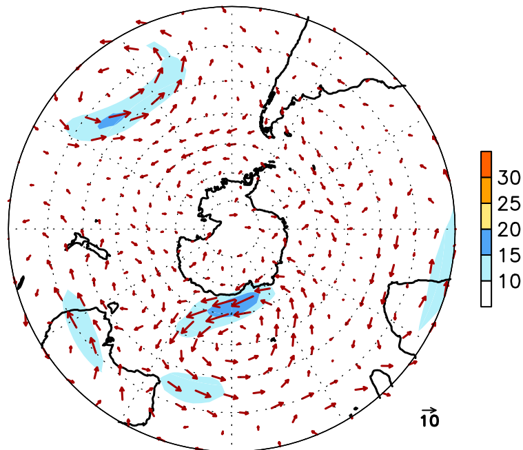
FIGURE E16. Southern Hemisphere mean (left) and anomalous (right) 300-hPa vector wind (CDAS/Reanalysis) for MAY 2015. Mean (anomaly) isotach contour interval is 10 (5) \text{ms}^{-1} . Values greater than 30 \text{ms}^{-1} (left) and 10 \text{ms}^{-1} (rights) are shaded. Anomalies are departures from the 1981-2010 base period monthly means.
