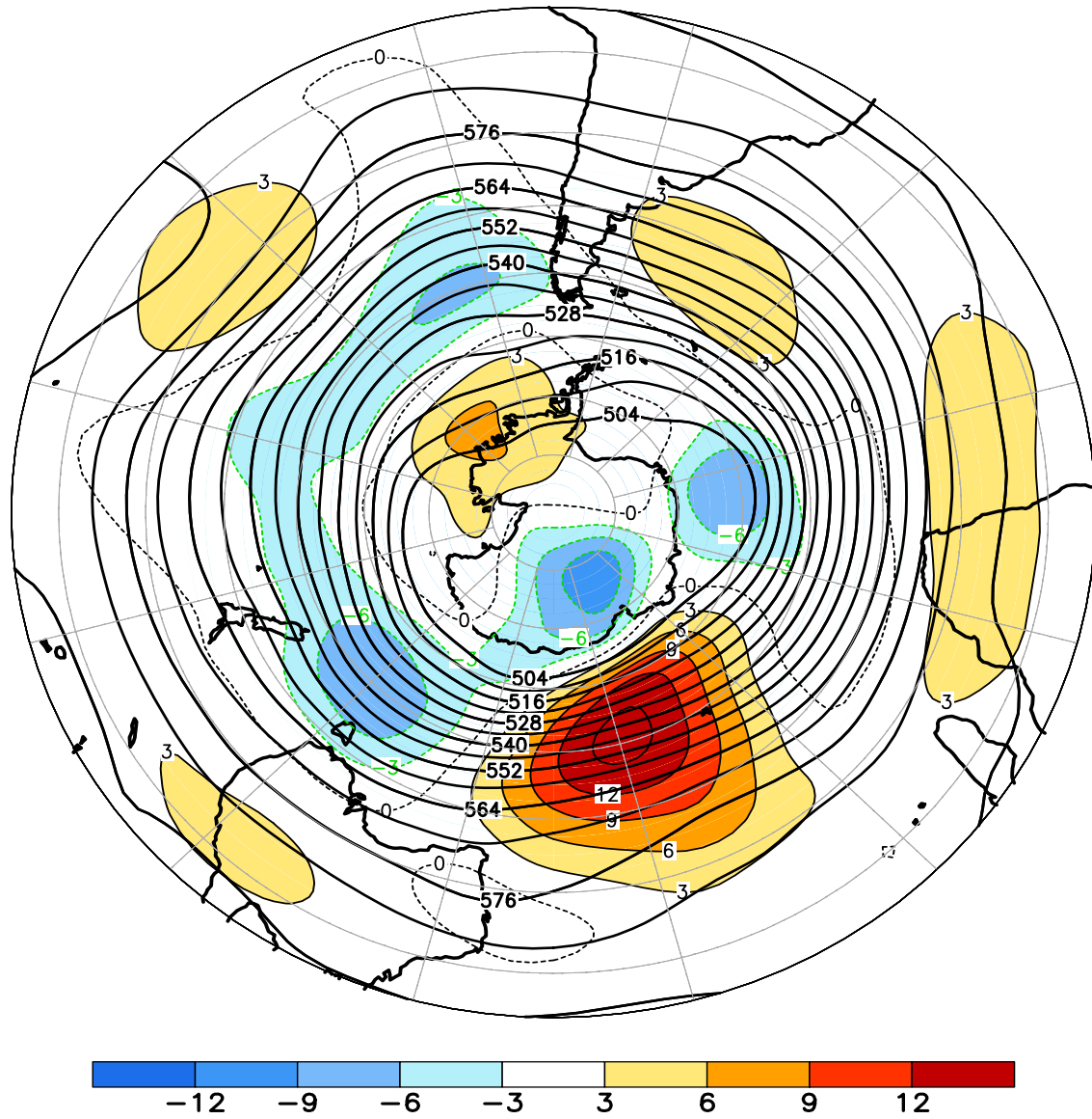
FIGURE E15. Southern Hemisphere mean and anomalous 500-hPa geopotential height (CDAS/Reanalysis) for MAY 2015. Mean heights are denoted by solid contours drawn at an interval of 6 dam. Anomaly contour interval is 3 dam with values less (greater) than -3 dam (3 dam) indicated by dark (light) shading. Anomalies are calculated as departures from the 1981-2010 base period monthly means.
