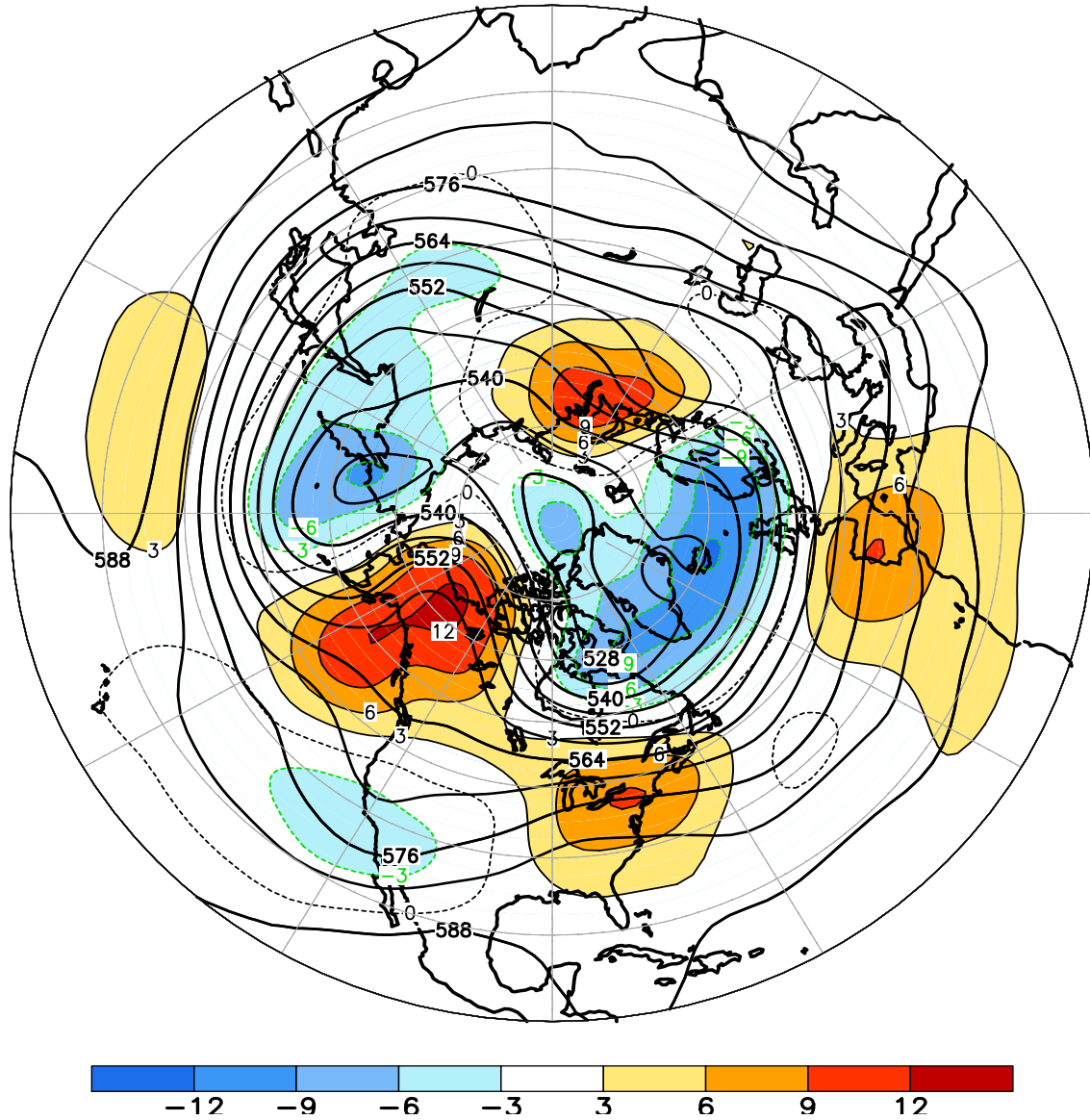
FIGURE E9. Northern Hemisphere mean and anomalous 500-hPa geopotential height (CDAS/Reanalysis) for MAY 2015. Mean heights are denoted by solid contours drawn at an interval of 6 dam. Anomaly contour interval is 3 dam with values less (greater) than -3 dam (3 dam) indicated by dark (light) shading. Anomalies are calculated as departures from the 1981-2010 base period monthly means.
