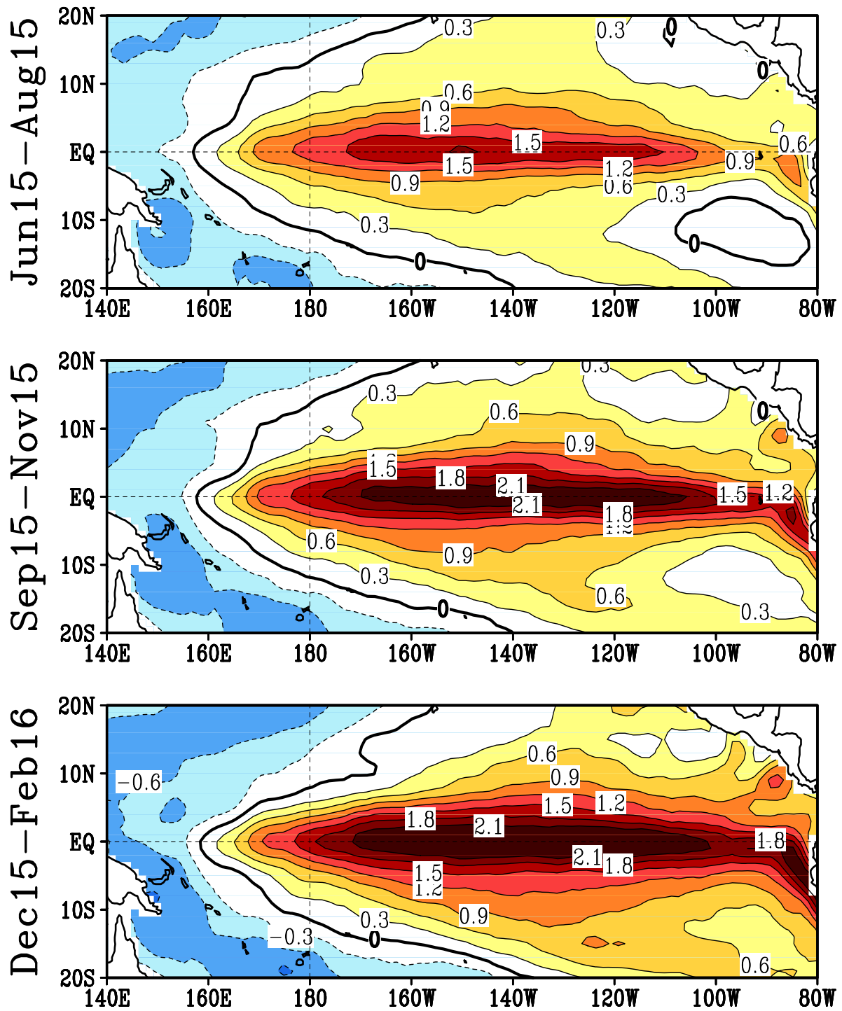
FIGURE F5. Predicted 3-month average sea surface temperature anomalies from the NCEP/CPC Markov model (Xue et al. 2000, J. Climate , 13 , 849-871). The forecast is initiated in MAY 2015 . Contour interval is 0.3C and negative anomalies are indicated by dashed contours. Anomalies are calculated relative to the 1971-2000 climatology.
