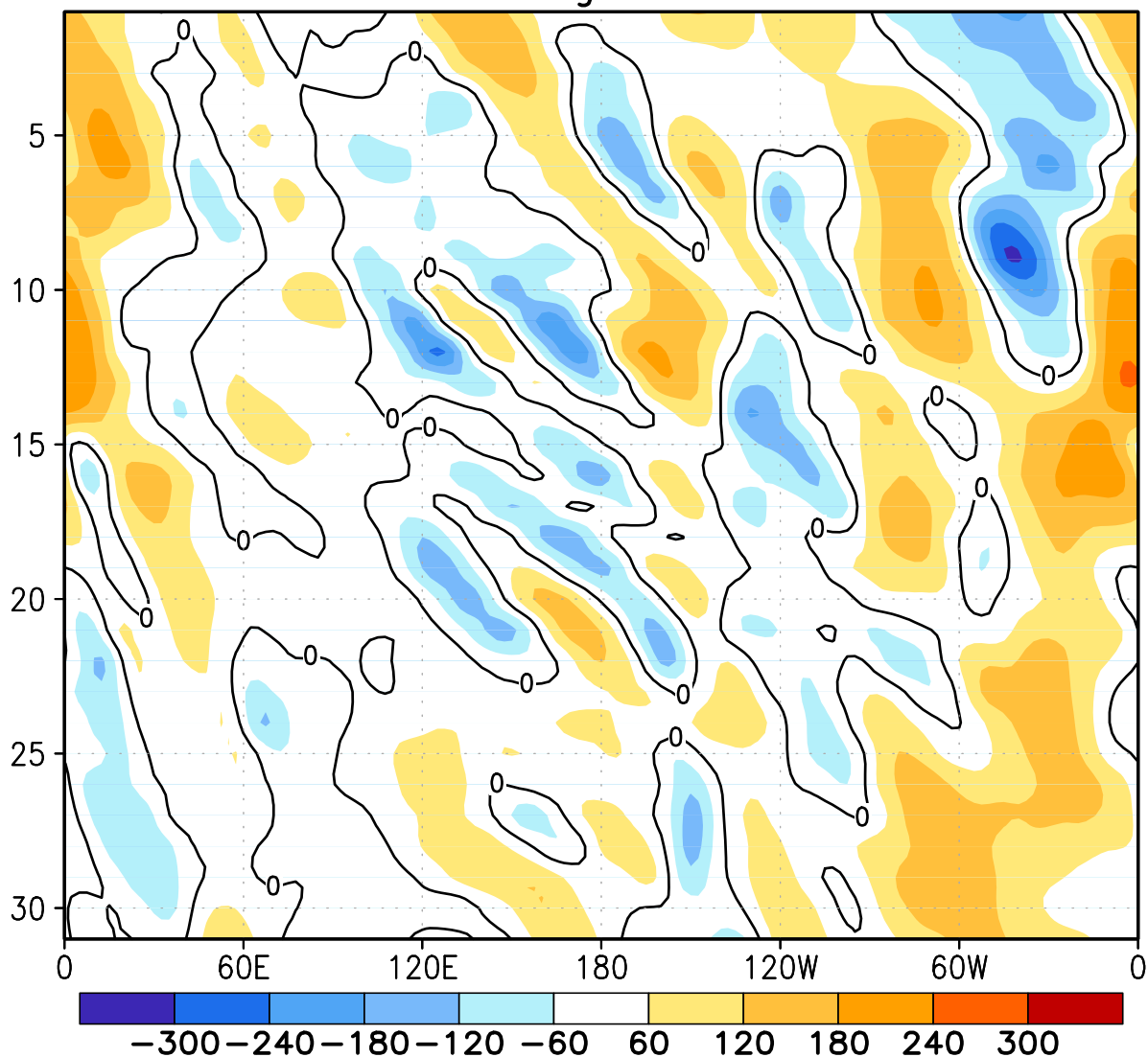
FIGURE E12. Northern Hemisphere: Daily 500-hPa height anomalies for MAY 2015 averaged over the 5° latitude band centered on 40°N. Positive values are indicated by solid contours and dark shading. Negative values are indicated by dashed contours and light shading. Contour interval is 60 m. Anomalies are departures from the 1981-2010 base period daily means.
