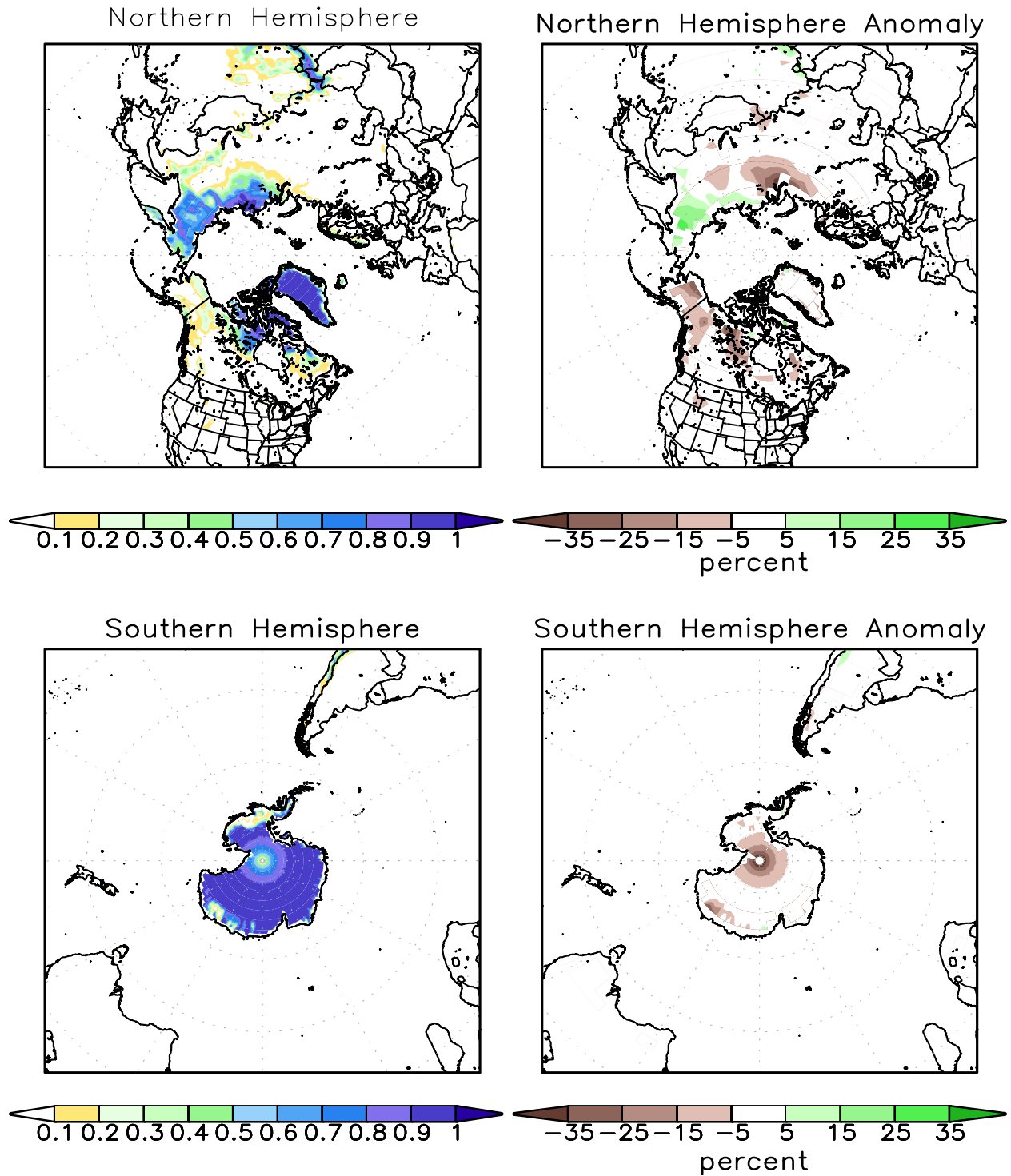
FIGURE A2.2. SSM/I derived snow cover frequency (%) (left) and snow cover anomaly (%) (right) for the month of MAY 2015 based on 1987 - 2010 base period for the Northern Hemisphere (top) and Southern Hemisphere (bottom). It is generated using the algorithm described by Ferraro et. al, 1996, Bull. Amer. Meteor. Soc., vol 77, 891-905.
