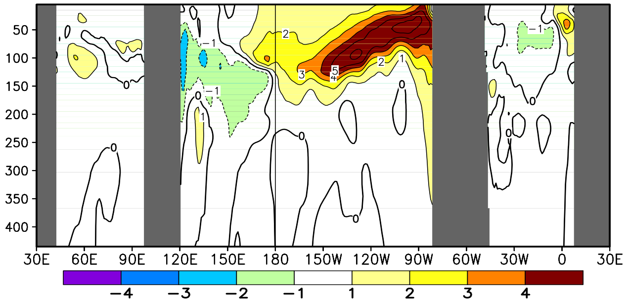
FIGURE T17. Equatorial depth–longitude section of ocean temperature (top) and ocean temperature anomalies (bottom) for MAY 2015. Contour interval is 1°C. Dashed contours in bottom panel indicate negative anomalies. Data are derived from the NCEP’s global ocean data assimilation system version 2 which assimilates oceanic observations into an oceanic GCM (Xue, Y. and Behringer, D.W., 2006: Operational global ocean data assimilation system at NCEP, to be submitted to BAMS). Anomalies are departures from the 1981–2010 base period means.
