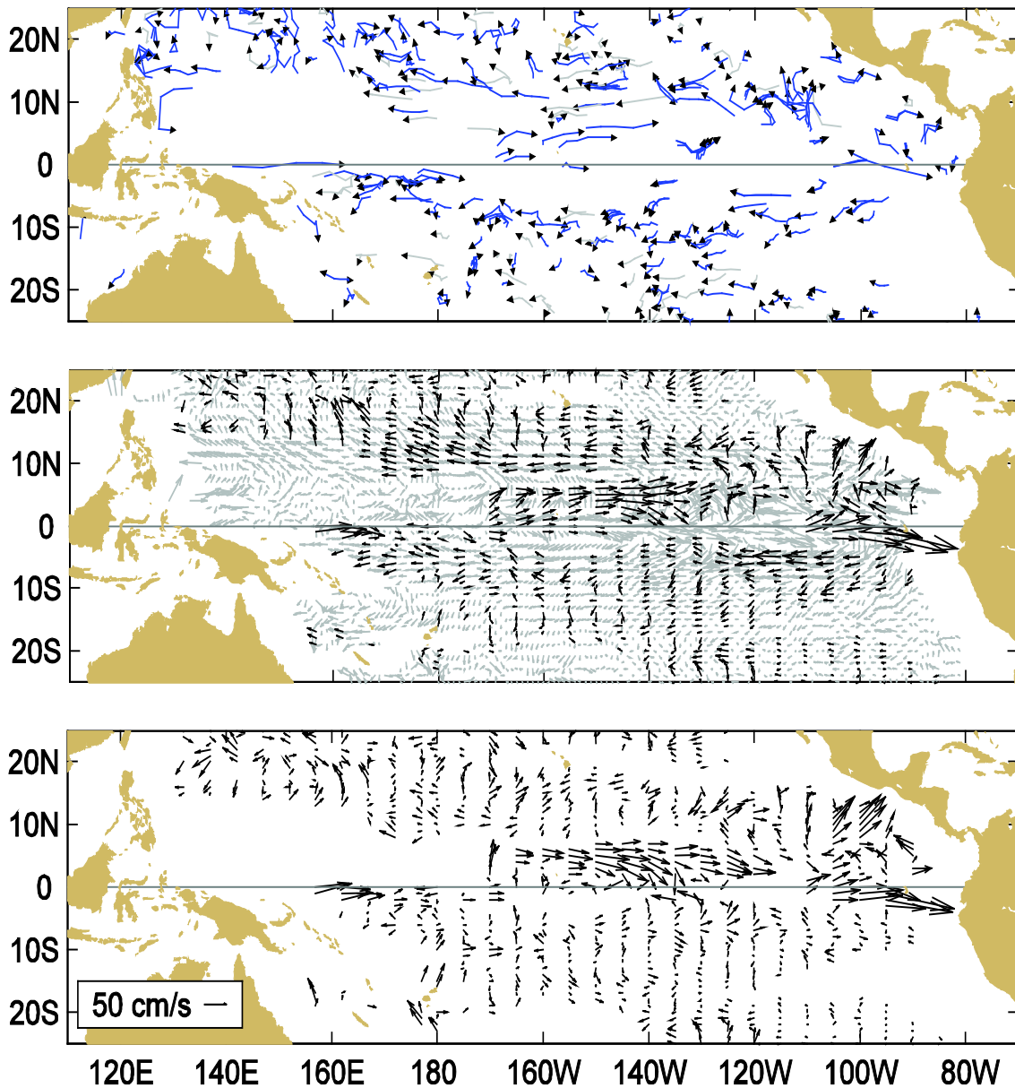
Figure A1.1 Top: Movements of drifting buoys in the tropical Pacific Ocean during May 2015. The linear segments of each trajectory represent a one week displacement. Trajectories of buoys which have lost their subsurface drogues are gray; those with drogues are black.
