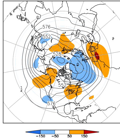
500-hPa Height (dm) & Anomalies (m) (May 1–15, 2015)
