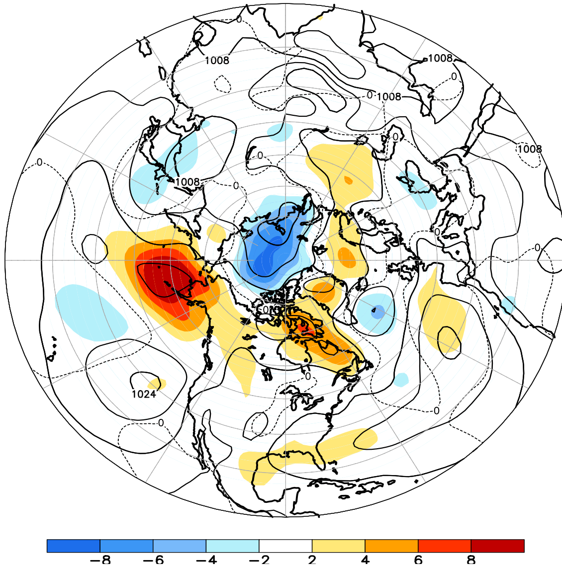
FIGURE E8. Northern Hemisphere mean and anomalous sea level pressure (CDAS/Reanalysis) for MAY 2014. Mean values are denoted by solid contours drawn at an interval of 4 hPa. Anomaly contour interval is 2 hPa with values less (greater) than -2 hPa (2 hPa) indicated by dark (light) shading. Anomalies are calculated as departures from the 1981-2010 base period monthly means.
