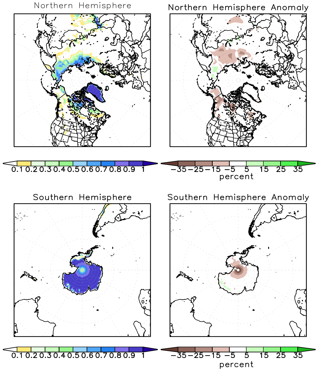
FIGURE A2.2. SSM/I derived snow cover frequency (%) (left) and snow cover anomaly (%) (right) for the month of MAY 2014 based on 1987 - 2010 base period for the Northern Hemisphere (top) and Southern Hemisphere (bottom). It is generated using the algorithm described by Ferraro et. al, 1996, Bull. Amer. Meteor. Soc., vol 77, 891-905.
