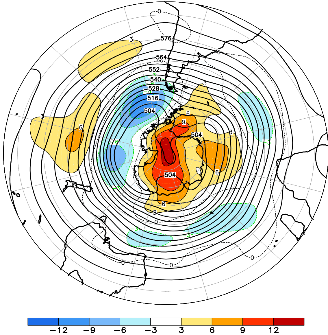
FIGURE E15. Southern Hemisphere mean and anomalous 500-hPa geopotential height (CDAS/Reanalysis) for MAY 2014. Mean heights are denoted by solid contours drawn at an interval of 6 dam. Anomaly contour interval is 3 dam with values less (greater) than -3 dam (3 dam) indicated by dark (light) shading. Anomalies are calculated as departures from the 1981-2010 base period monthly means.
