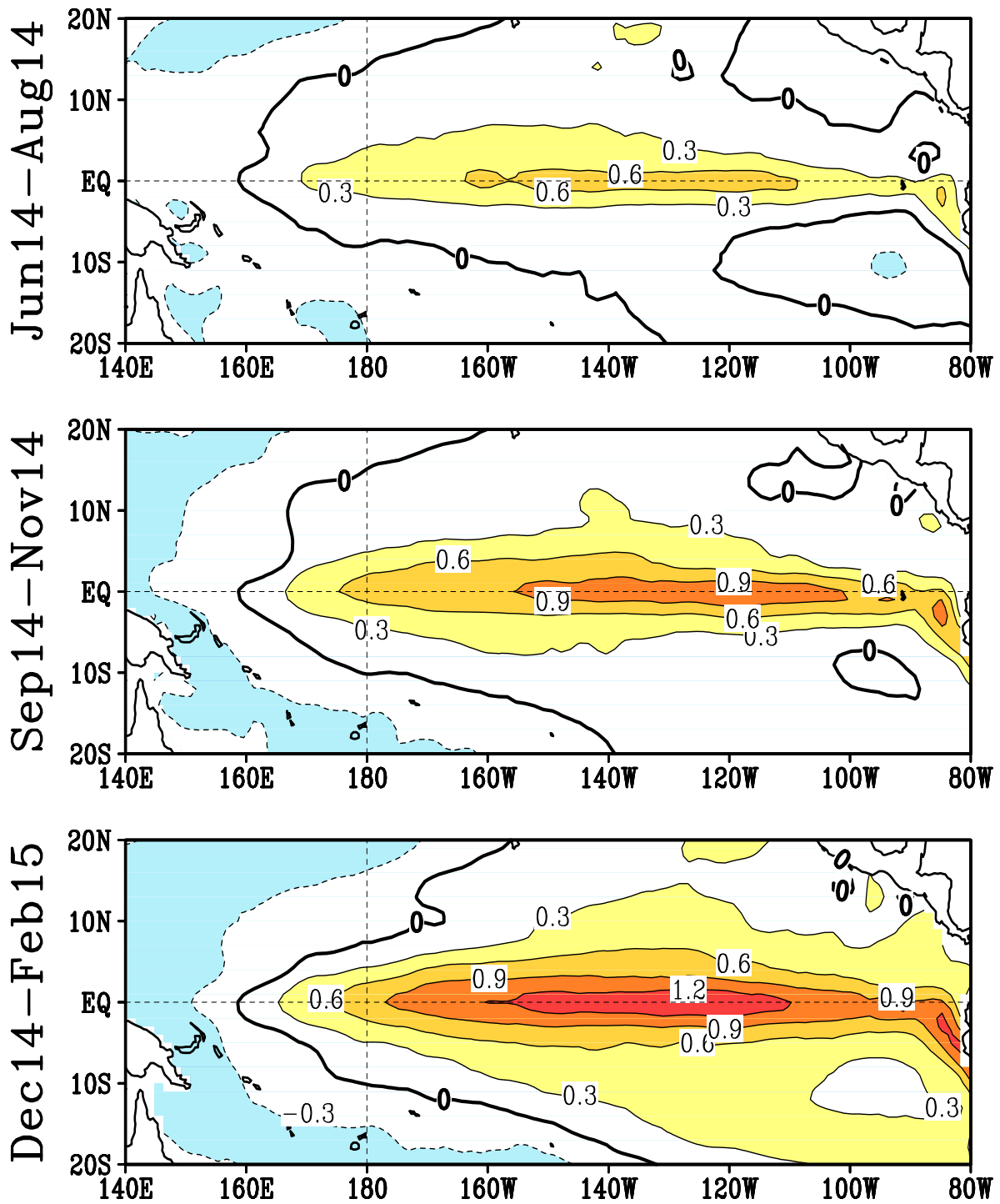
FIGURE F5. Predicted 3-month average sea surface temperature anomalies from the NCEP/CPC Markov model (Xue et al. 2000, J. Climate , 13 , 849-871). The forecast is initiated in MAY 2014 . Contour interval is 0.3C and negative anomalies are indicated by dashed contours. Anomalies are calculated relative to the 1971-2000 climatology.
