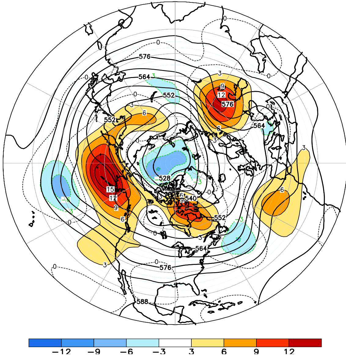
FIGURE E9. Northern Hemisphere mean and anomalous 500-hPa geopotential height (CDAS/Reanalysis) for MAY 2014. Mean heights are denoted by solid contours drawn at an interval of 6 dam. Anomaly contour interval is 3 dam with values less (greater) than -3 dam (3 dam) indicated by dark (light) shading. Anomalies are calculated as departures from the 1981-2010 base period monthly means.
