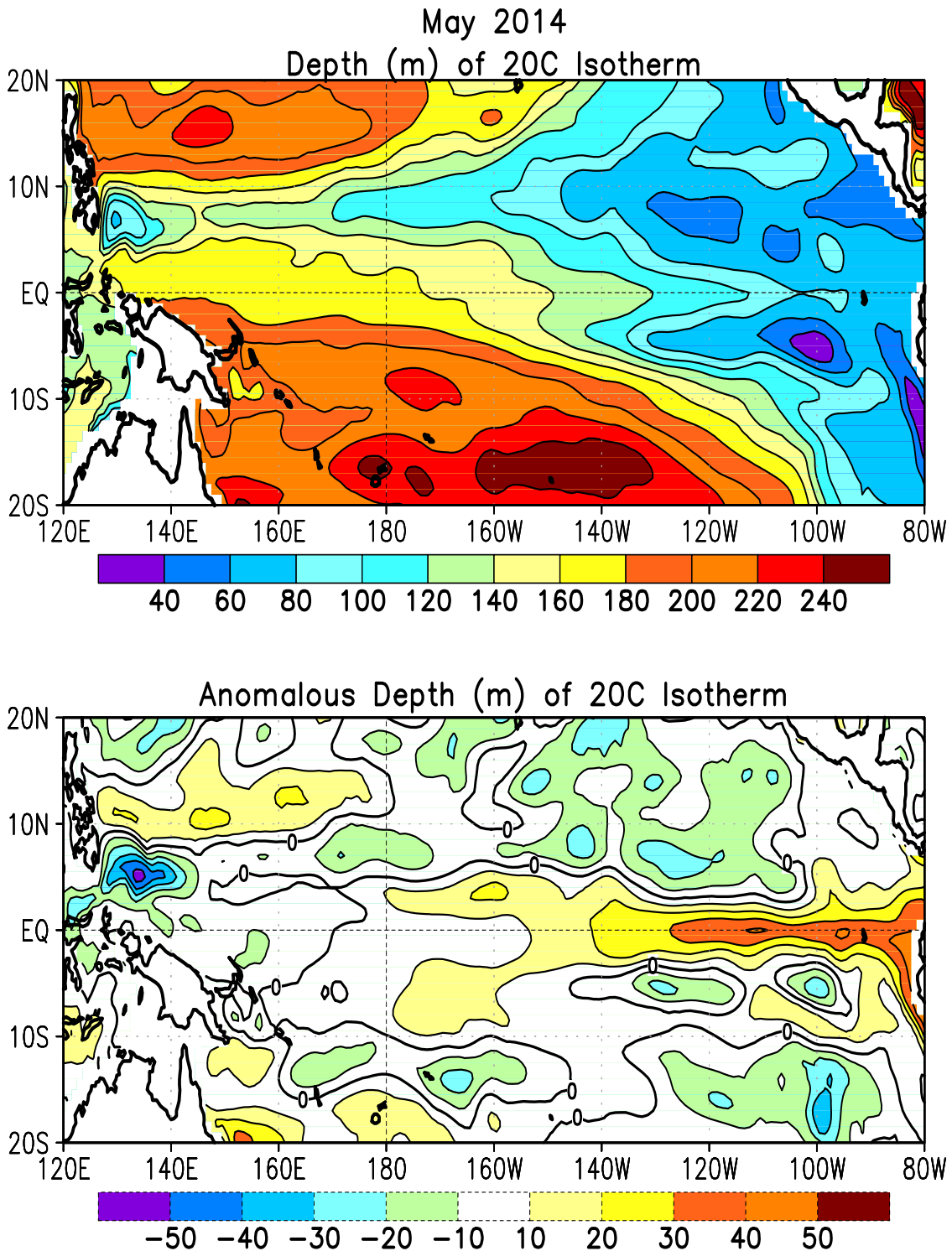
FIGURE T16. Mean (top) and anomalous (bottom) depth of the 20°C isotherm for MAY 2014. Contour interval is 40 m (top) and 10 m (bottom). Dashed contours in bottom panel indicate negative anomalies. Data are derived from the NCEP’s global ocean data assimilation system version 2 which assimilates oceanic observations into an oceanic GCM (Xue, Y. and Behringer, D.W., 2006: Operational global ocean data assimilation system at NCEP, to be submitted to BAMS). Anomalies are departures from the 1981–2010 base period means.
