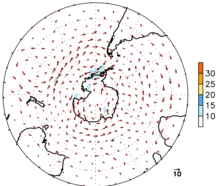
FIGURE E16. Southern Hemisphere mean (left) and anomalous (right) 300-hPa vector wind (CDAS/Reanalysis) for MAY 2014. Mean (anomaly) isotach contour interval is 10 (5) \text{ms}^{-1} . Values greater than 30 \text{ms}^{-1} (left) and 10 \text{ms}^{-1} (rights) are shaded. Anomalies are departures from the 1981-2010 base period monthly means.
