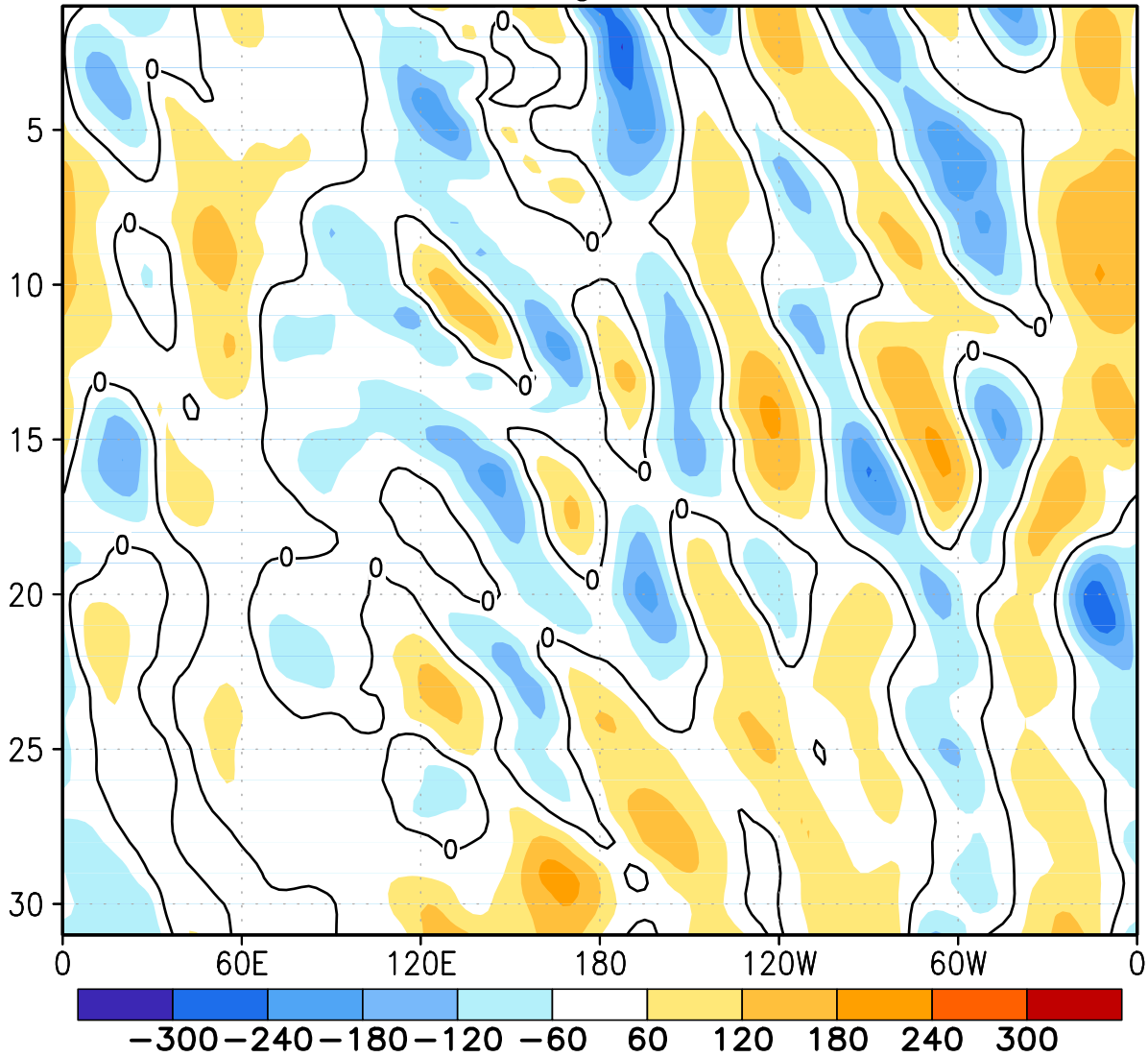
FIGURE E12. Northern Hemisphere: Daily 500-hPa height anomalies for MAY 2014 averaged over the 5° latitude band centered on 40°N. Positive values are indicated by solid contours and dark shading. Negative values are indicated by dashed contours and light shading. Contour interval is 60 m. Anomalies are departures from the 1981-2010 base period daily means.
