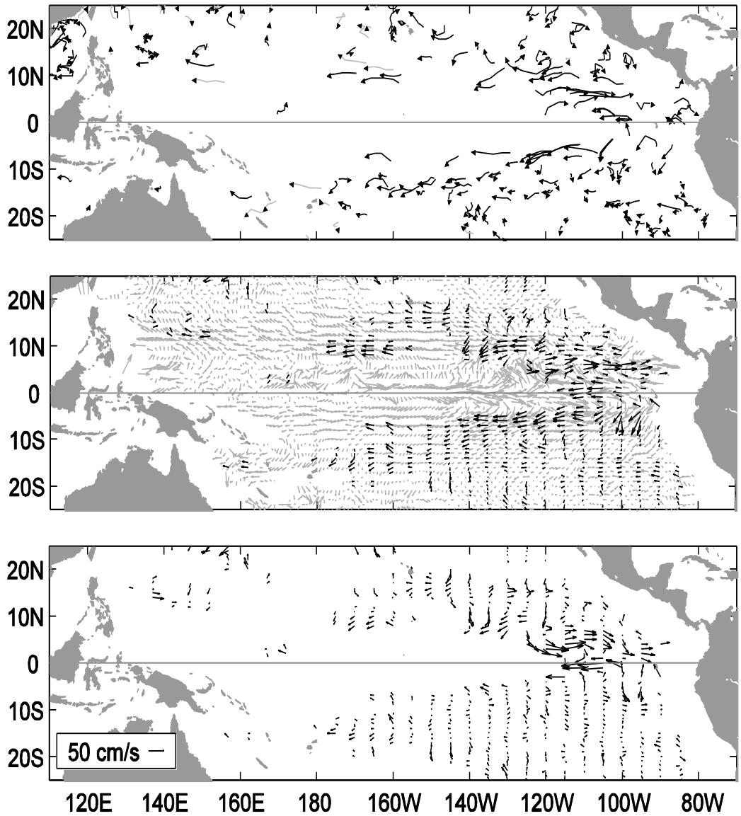
Figure A1.1 Top: Movements of drifting buoys in the tropical Pacific Ocean during May 2014. The linear segments of each trajectory represent a one week displacement. Trajectories of buoys which have lost their subsurface drogues are gray; those with drogues are black. Middle: Monthly mean currents calculated from all buoys 1993-2002 (gray), and currents measured by the drogued buoys this month (black) smoothed by an optimal filter.
