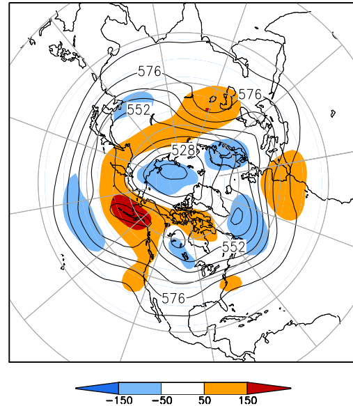
500-hPa Height (dm) & Anomalies (m) (May 1–15, 2014)
