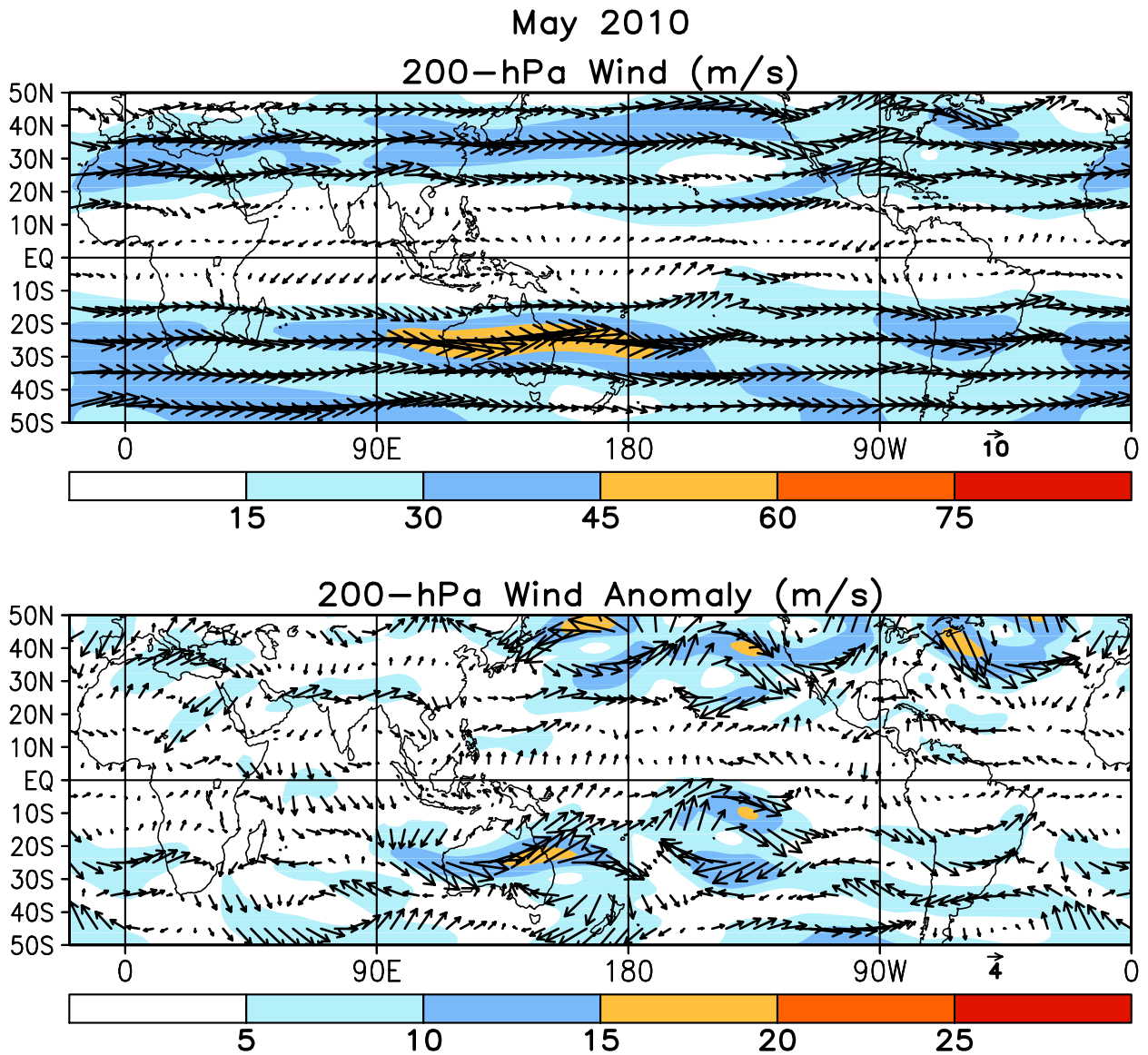
FIGURE T21. Mean (top) and anomalous (bottom) 200-hPa vector wind (CDAS/Reanalysis) for MAY 2010. Contour interval for isotachs is 15 \text{ ms}^{-1} (top) and 5 \text{ ms}^{-1} (bottom). Anomalies are departures from 1979–95 base period monthly means.
