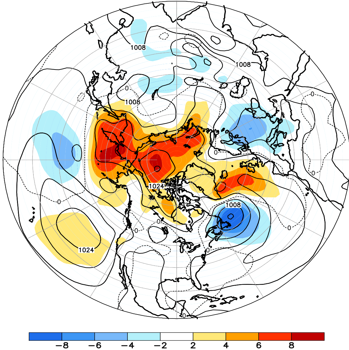
FIGURE E8. Northern Hemisphere mean and anomalous sea level pressure (CDAS/Reanalysis) for MAY 2010. Mean values are denoted by solid contours drawn at an interval of 4 hPa. Anomaly contour interval is 2 hPa with values less (greater) than -2 hPa (2 hPa) indicated by dark (light) shading. Anomalies are calculated as departures from the 1979-95 base period monthly means.
