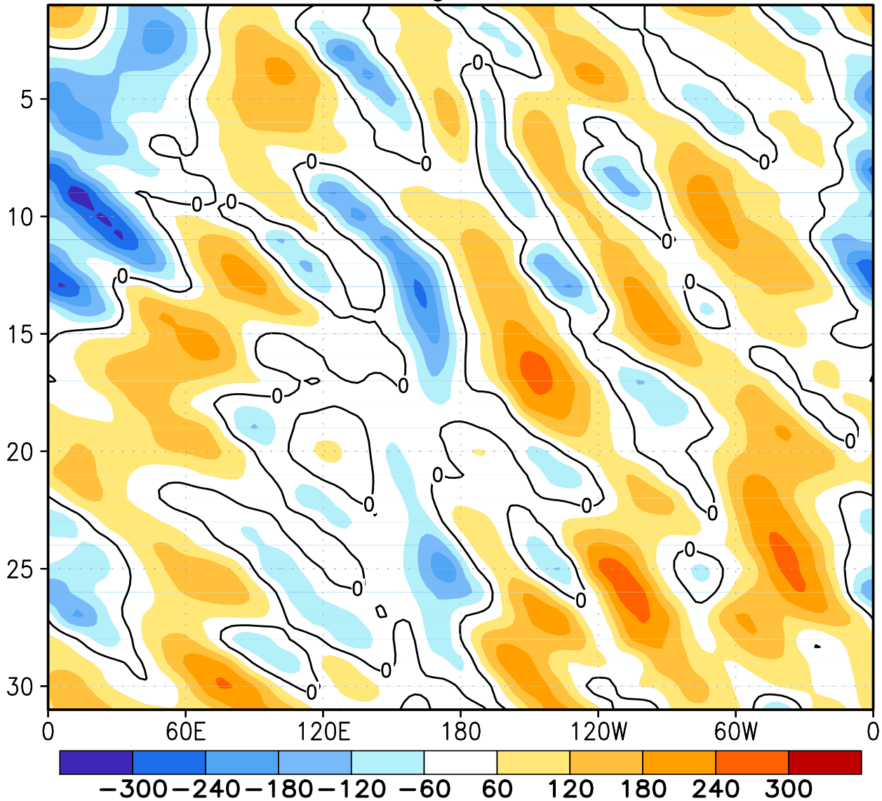
FIGURE E18. Southern Hemisphere: Daily 500-hPa height anomalies for MAY 2010 averaged over the 5° latitude band centered on 40°S. Positive values are indicated by solid contours and dark shading. Negative values are indicated by dashed contours and light shading. Contour interval is 60 m. Anomalies are departures from the 1979-95 base period daily means.
