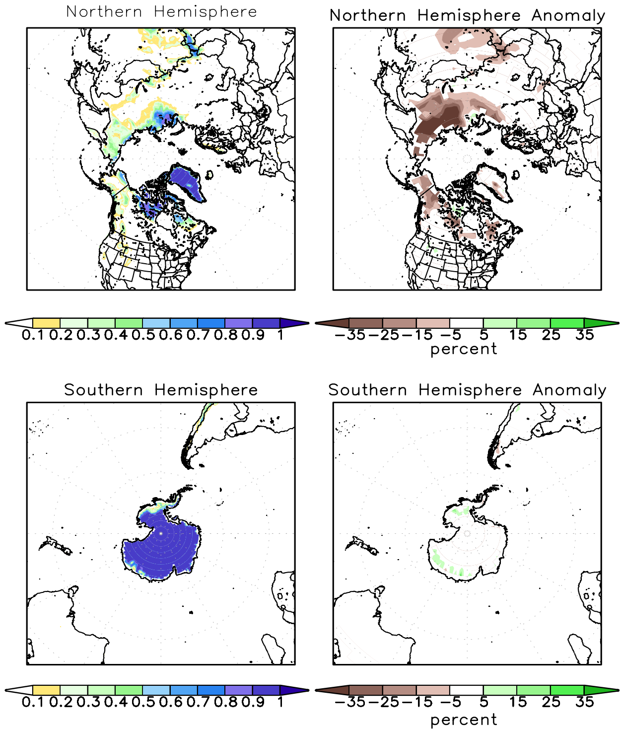
FIGURE A2.2. SSM/I derived snow cover frequency (%) (left) and snow cover anomaly (%) (right) for the month of MAY 2010 based on 1987 - 2006 base period for the Northern Hemisphere (top) and Southern Hemisphere (bottom). It is generated using the algorithm described by Ferraro et. al, 1996, Bull. Amer. Meteor. Soc., vol 77, 891-905.
