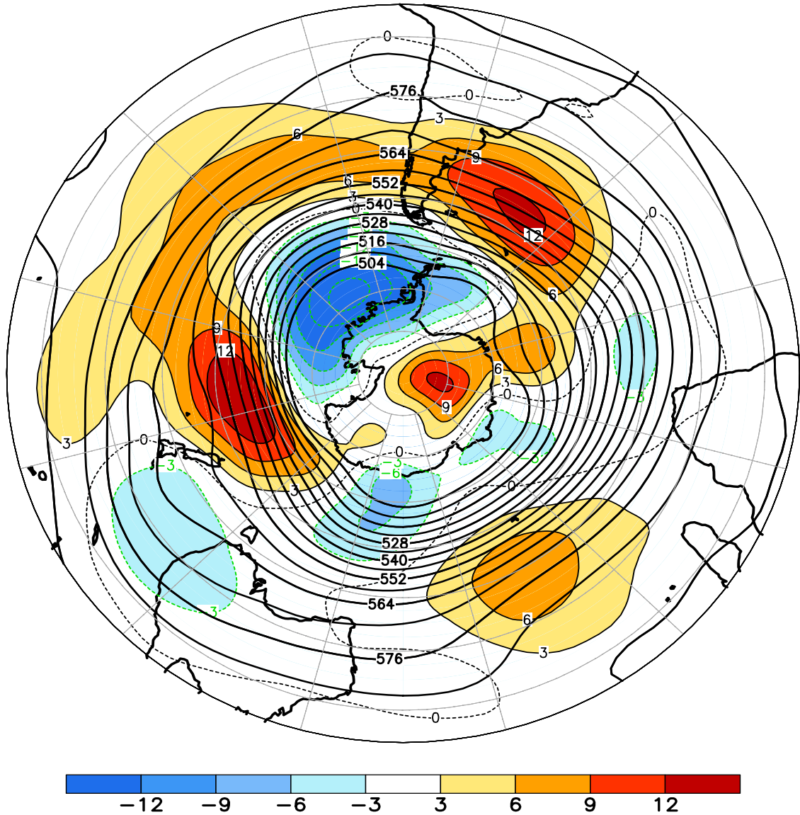
FIGURE E15. Southern Hemisphere mean and anomalous 500-hPa geopotential height (CDAS/Reanalysis) for MAY 2010. Mean heights are denoted by solid contours drawn at an interval of 6 dam. Anomaly contour interval is 3 dam with values less (greater) than -3 dam (3 dam) indicated by dark (light) shading. Anomalies are calculated as departures from the 1979-95 base period monthly means.
