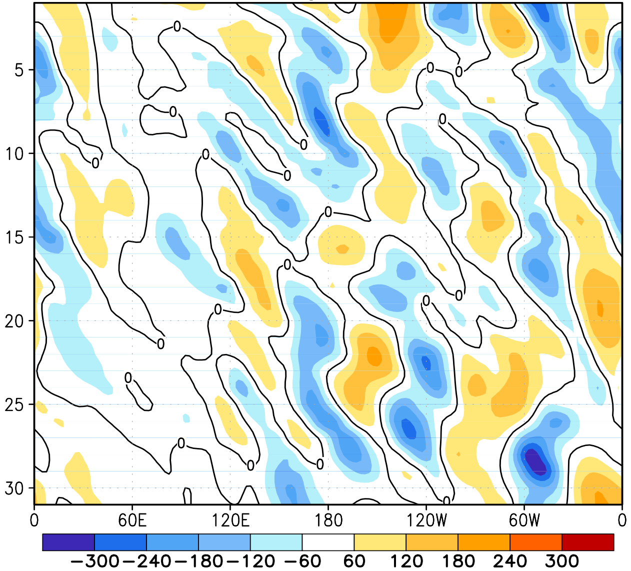
FIGURE E12. Northern Hemisphere: Daily 500-hPa height anomalies for MAY 2010 averaged over the 5° latitude band centered on 40°N. Positive values are indicated by solid contours and dark shading. Negative values are indicated by dashed contours and light shading. Contour interval is 60 m. Anomalies are departures from the 1979-95 base period daily means.
