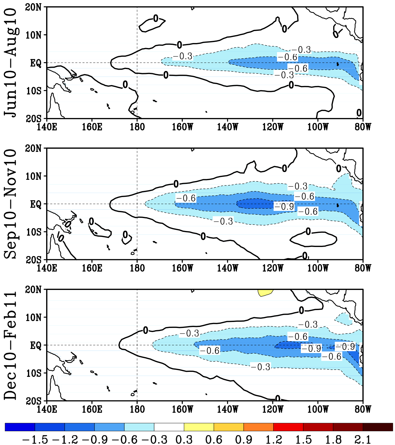
FIGURE F5. Predicted 3-month average sea surface temperature anomalies from the NCEP/CPC Markov model (Xue et al. 2000, J. Climate , 13 , 849-871). The forecast is initiated in MAY 2010. Contour interval is 0.3C and negative anomalies are indicated by dashed contours. Anomalies are calculated relative to the 1971-2000 climatology.
