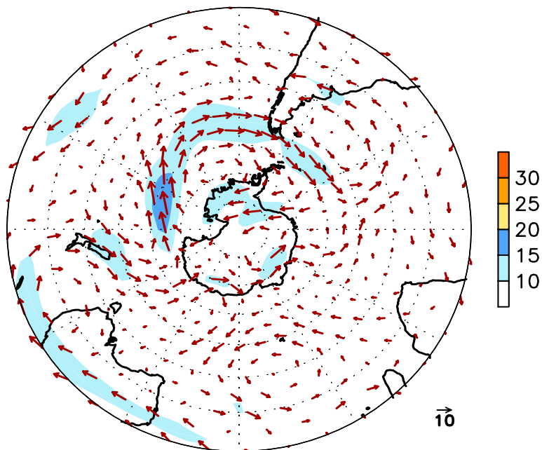
FIGURE E16. Southern Hemisphere mean (left) and anomalous (right) 300-hPa vector wind (CDAS/Reanalysis) for MAY 2010. Mean (anomaly) isotach contour interval is 10 (5) \text{ms}^{-1} . Values greater than 30 \text{ms}^{-1} (left) and 10 \text{ms}^{-1} (rights) are shaded. Anomalies are departures from the 1979-95 base period monthly means.
