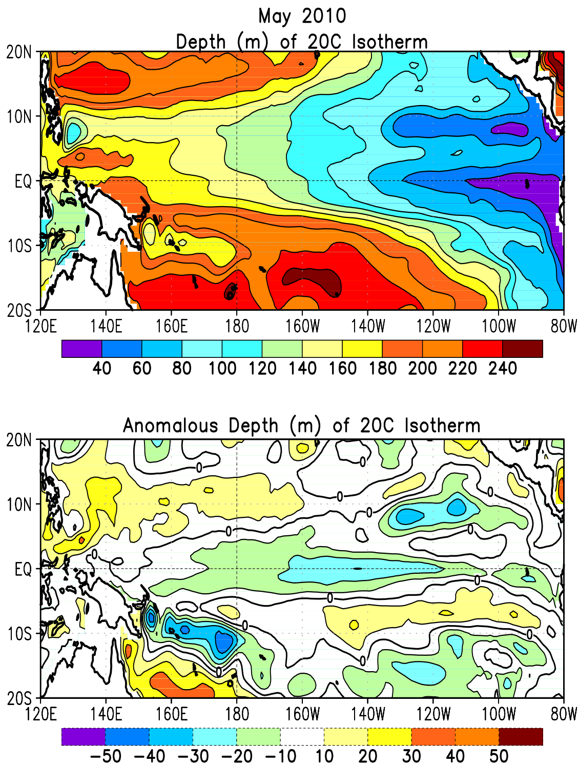
FIGURE T16. Mean (top) and anomalous (bottom) depth of the 20°C isotherm for MAY 2010. Contour interval is 40 m (top) and 10 m (bottom). Dashed contours in bottom panel indicate negative anomalies. Data are derived from the NCEP’s global ocean data assimilation system version 2 which assimilates oceanic observations into an oceanic GCM (Xue, Y. and Behringer, D.W., 2006: Operational global ocean data assimilation system at NCEP, to be submitted to BAMS). Anomalies are departures from the 1982–2004 base period means.
