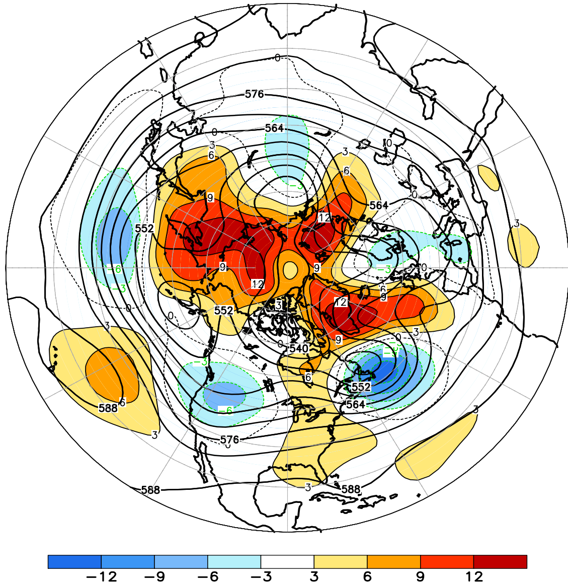
FIGURE E9. Northern Hemisphere mean and anomalous 500-hPa geopotential height (CDAS/Reanalysis) for MAY 2010. Mean heights are denoted by solid contours drawn at an interval of 6 dam. Anomaly contour interval is 3 dam with values less (greater) than -3 dam (3 dam) indicated by dark (light) shading. Anomalies are calculated as departures from the 1979-95 base period monthly means.
