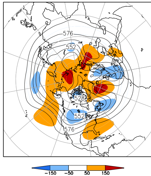
500-hPa Height (dm) & Anomalies (m) (May 1–15, 2010)
