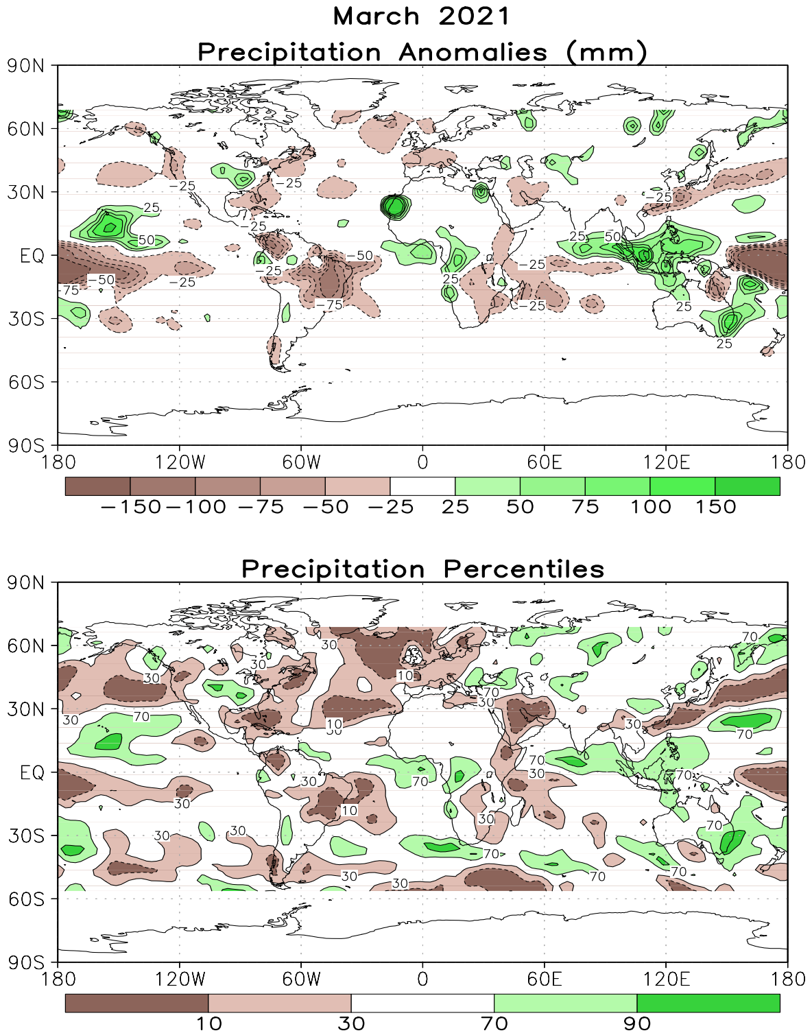
FIGURE E3. Anomalous precipitation (mm, top) and precipitation percentiles based on a Gamma distribution fit to the 1981–2010 base period data (bottom) for MAR 2021. Data are obtained from a merge of raingauge observations and satellite-derived precipitation estimates (Janowiak and Xie 1999, J. Climate , 12 , 3335–3342). Contours are drawn at 200, 100, 50, 25, -25, -50, -100, and -200 mm in top panel. Percentiles are not plotted in regions where mean monthly precipitation is <5mm/month.
