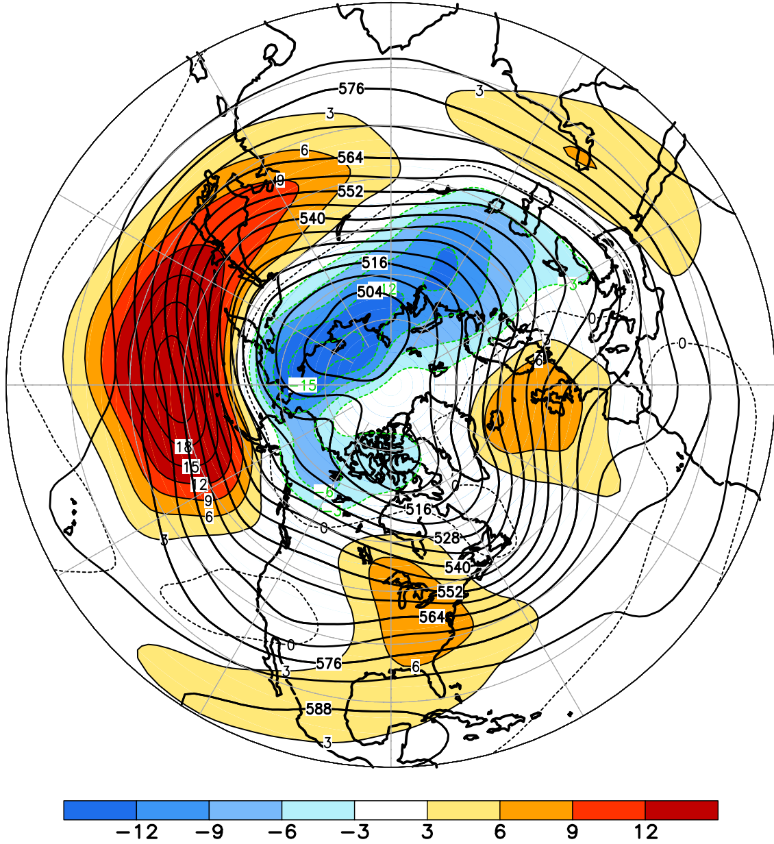
FIGURE E9. Northern Hemisphere mean and anomalous 500-hPa geopotential height (CDAS/Reanalysis) for MAR 2021. Mean heights are denoted by solid contours drawn at an interval of 6 dam. Anomaly contour interval is 3 dam with values less (greater) than -3 dam (3 dam) indicated by dark (light) shading. Anomalies are calculated as departures from the 1981-2010 base period monthly means.
