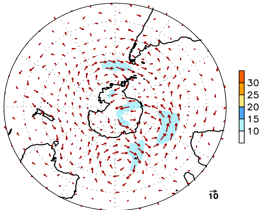
FIGURE E16. Southern Hemisphere mean (left) and anomalous (right) 300-hPa vector wind (CDAS/Reanalysis) for MAR 2021. Mean (anomaly) isotach contour interval is 10 (5) \text{ms}^{-1} . Values greater than 30 \text{ms}^{-1} (left) and 10 \text{ms}^{-1} (rights) are shaded. Anomalies are departures from the 1981-2010 base period monthly means.
