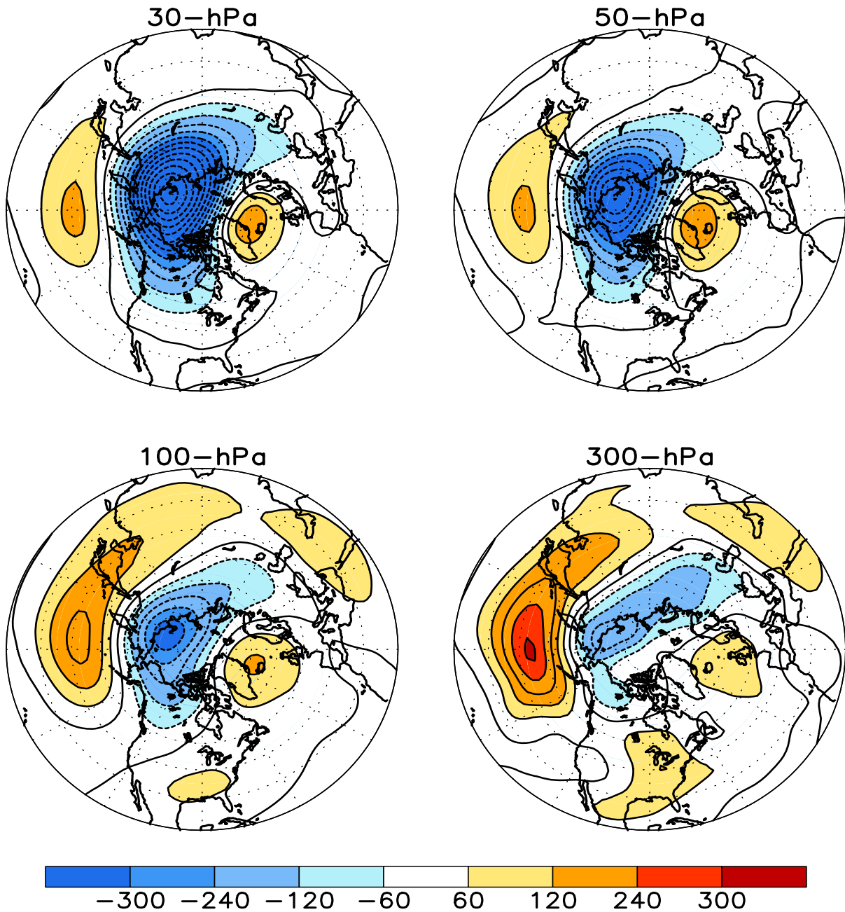
FIGURE S1. Stratospheric height anomalies (m) at selected levels for MAR 2021. Positive values are indicated by solid contours and dark shading. Negative values are indicated by dashed contours and light shading. Contour interval is 60 m. Anomalies are calculated from the 1981-2010 base period means. Winter Hemisphere is shown.
