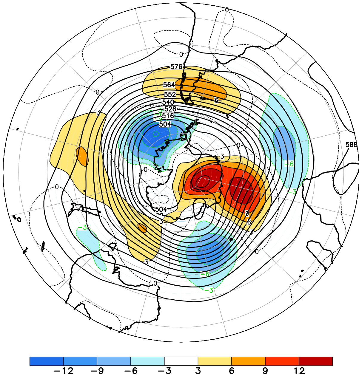
FIGURE E15. Southern Hemisphere mean and anomalous 500-hPa geopotential height (CDAS/Reanalysis) for MAR 2021. Mean heights are denoted by solid contours drawn at an interval of 6 dam. Anomaly contour interval is 3 dam with values less (greater) than -3 dam (3 dam) indicated by dark (light) shading. Anomalies are calculated as departures from the 1981-2010 base period monthly means.
