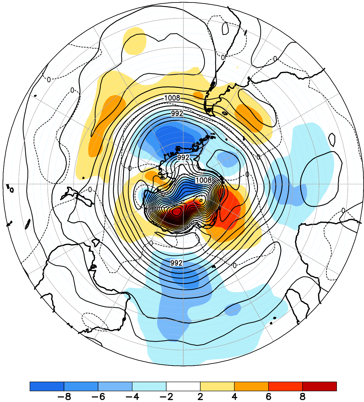
FIGURE E14. Southern Hemisphere mean and anomalous sea level pressure(CDAS/Reanalysis) for MAR 2021. Mean values are denoted by solid contours drawn at an interval of 4 hPa. Anomaly contour interval is 2 hPa with values less (greater) than -2 hPa (2 hPa) indicated by dark (light) shading. Anomalies are calculated as departures from the 1981-2010 base period monthly means.
