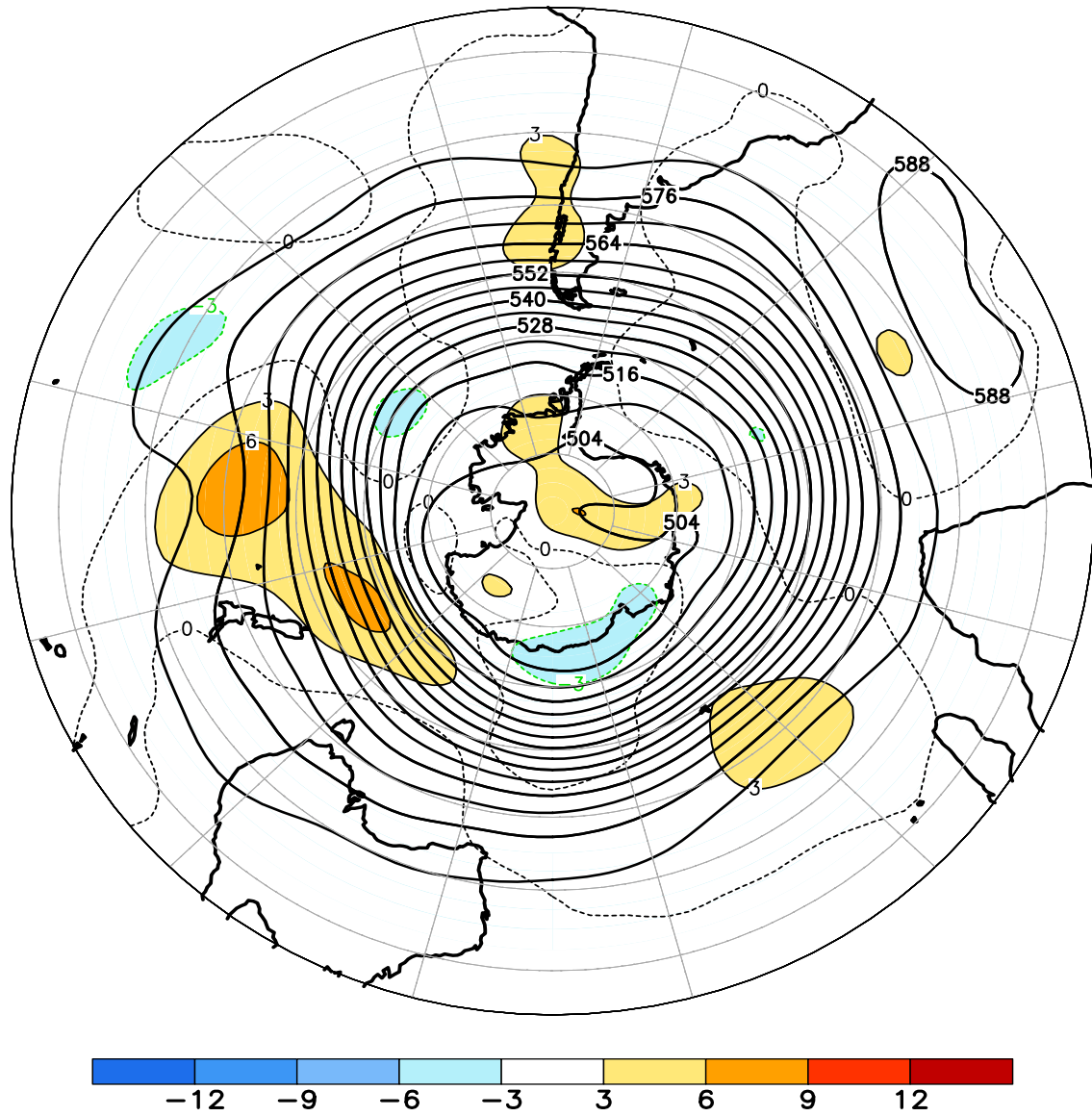
FIGURE E15. Southern Hemisphere mean and anomalous 500-hPa geopotential height (CDAS/Reanalysis) for MAR 2012. Mean heights are denoted by solid contours drawn at an interval of 6 dam. Anomaly contour interval is 3 dam with values less (greater) than -3 dam (3 dam) indicated by dark (light) shading. Anomalies are calculated as departures from the 1981-2010 base period monthly means.
