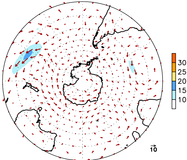
FIGURE E16. Southern Hemisphere mean (left) and anomalous (right) 300-hPa vector wind (CDAS/Reanalysis) for MAR 2012. Mean (anomaly) isotach contour interval is 10 (5) \text{ms}^{-1} . Values greater than 30 \text{ms}^{-1} (left) and 10 \text{ms}^{-1} (rights) are shaded. Anomalies are departures from the 1981-2010 base period monthly means.
