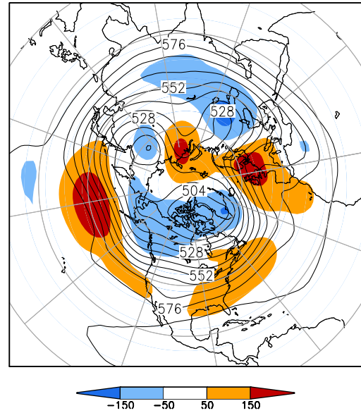
500-hPa Height (dm) & Anomalies (m) (Mar 1–15, 2012)
