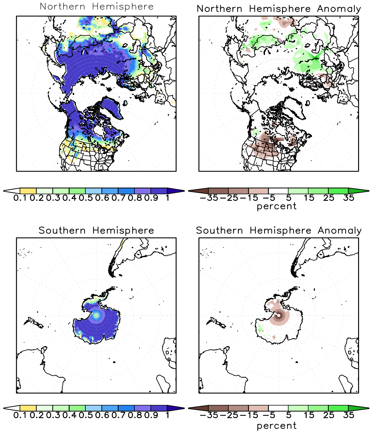
FIGURE A2.2. SSM/I derived snow cover frequency (%) (left) and snow cover anomaly (%) (right) for the month of MAR 2012 based on 1987 - 2010 base period for the Northern Hemisphere (top) and Southern Hemisphere (bottom). It is generated using the algorithm described by Ferraro et. al, 1996, Bull. Amer. Meteor. Soc., vol 77, 891-905.
