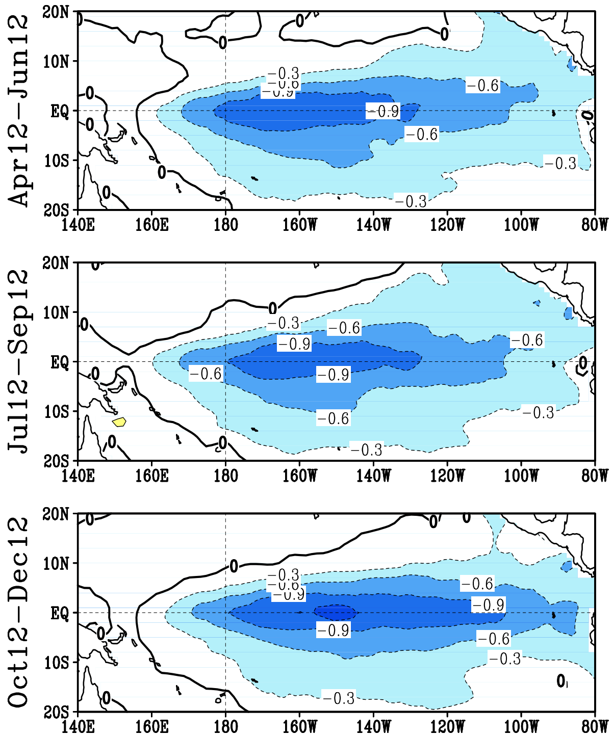
FIGURE F5. Predicted 3-month average sea surface temperature anomalies from the NCEP/CPC Markov model (Xue et al. 2000, J. Climate , 13 , 849-871). The forecast is initiated in MAR 2012. Contour interval is 0.3C and negative anomalies are indicated by dashed contours. Anomalies are calculated relative to the 1971-2000 climatology.
