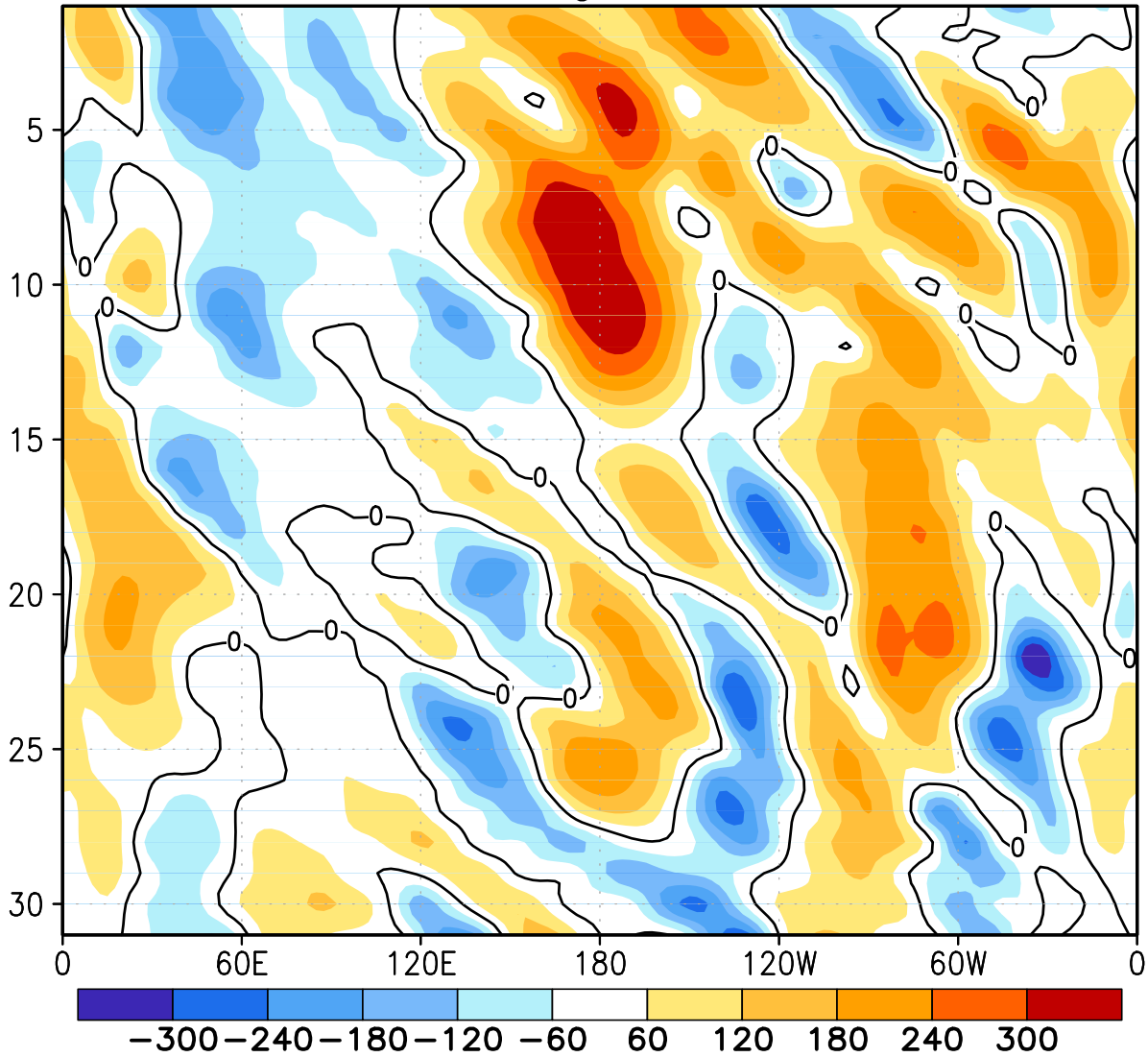
FIGURE E12. Northern Hemisphere: Daily 500-hPa height anomalies for MAR 2012 averaged over the 5° latitude band centered on 40°N. Positive values are indicated by solid contours and dark shading. Negative values are indicated by dashed contours and light shading. Contour interval is 60 m. Anomalies are departures from the 1981-2010 base period daily means.
