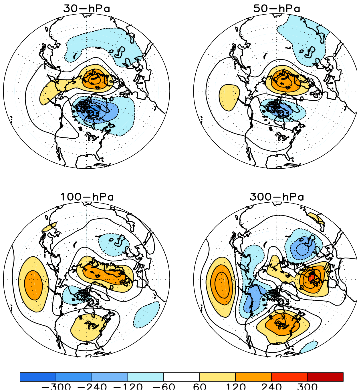
FIGURE S1. Stratospheric height anomalies (m) at selected levels for MAR 2012. Positive values are indicated by solid contours and dark shading. Negative values are indicated by dashed contours and light shading. Contour interval is 60 m. Anomalies are calculated from the 1981-2010 base period means. Winter Hemisphere is shown.
