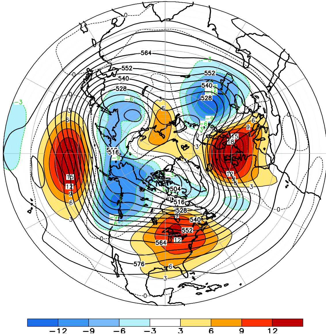
FIGURE E9. Northern Hemisphere mean and anomalous 500-hPa geopotential height (CDAS/Reanalysis) for MAR 2012. Mean heights are denoted by solid contours drawn at an interval of 6 dam. Anomaly contour interval is 3 dam with values less (greater) than -3 dam (3 dam) indicated by dark (light) shading. Anomalies are calculated as departures from the 1981-2010 base period monthly means.
