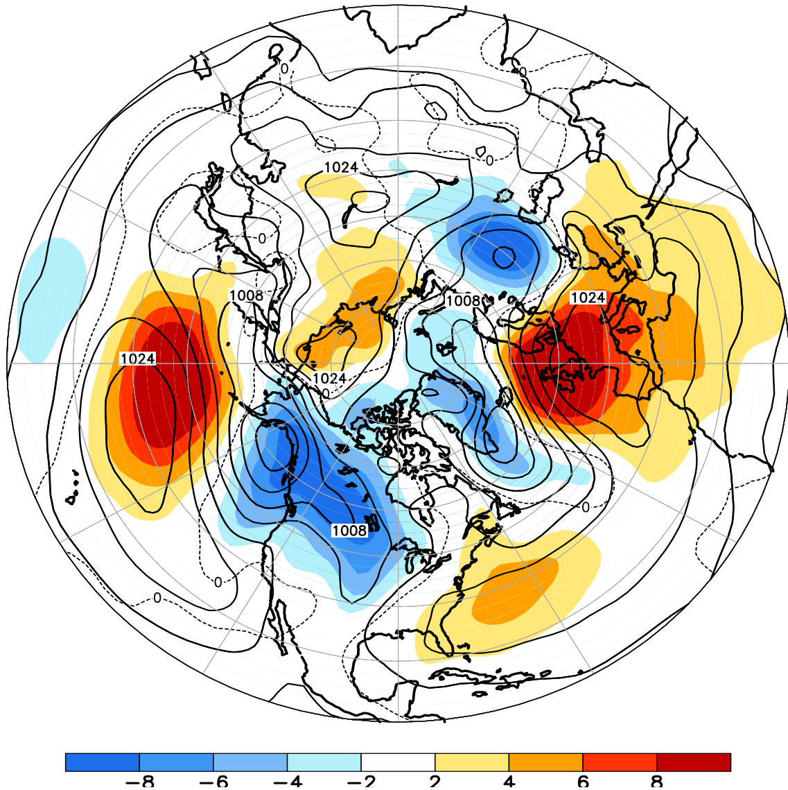
FIGURE E8. Northern Hemisphere mean and anomalous sea level pressure (CDAS/Reanalysis) for MAR 2012. Mean values are denoted by solid contours drawn at an interval of 4 hPa. Anomaly contour interval is 2 hPa with values less (greater) than -2 hPa (2 hPa) indicated by dark (light) shading. Anomalies are calculated as departures from the 1981-2010 base period monthly means.
