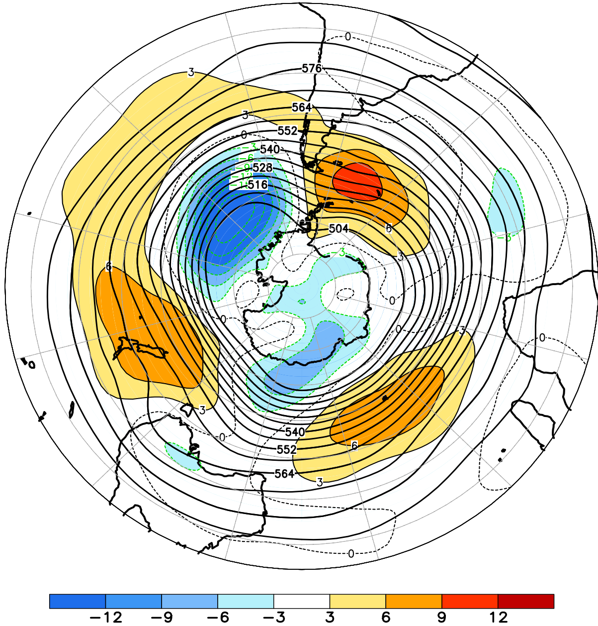
FIGURE E15. Southern Hemisphere mean and anomalous 500-hPa geopotential height (CDAS/Reanalysis) for JUN 2021. Mean heights are denoted by solid contours drawn at an interval of 6 dam. Anomaly contour interval is 3 dam with values less (greater) than -3 dam (3 dam) indicated by dark (light) shading. Anomalies are calculated as departures from the 1991-2020 base period monthly means.
