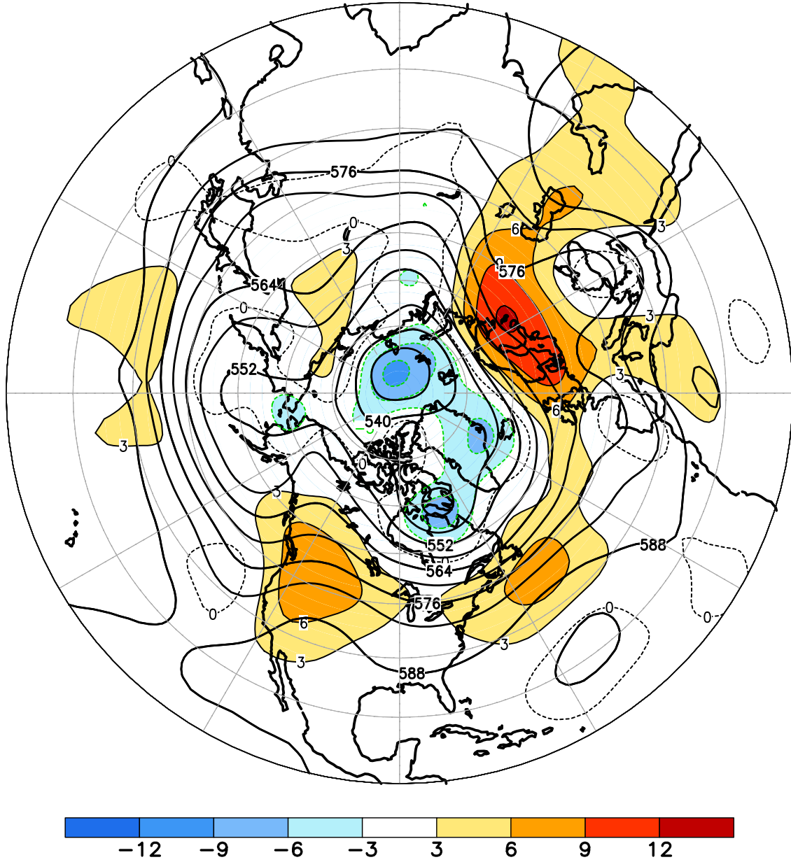
FIGURE E9. Northern Hemisphere mean and anomalous 500-hPa geopotential height (CDAS/Reanalysis) for JUN 2021. Mean heights are denoted by solid contours drawn at an interval of 6 dam. Anomaly contour interval is 3 dam with values less (greater) than -3 dam (3 dam) indicated by dark (light) shading. Anomalies are calculated as departures from the 1991-2020 base period monthly means.
