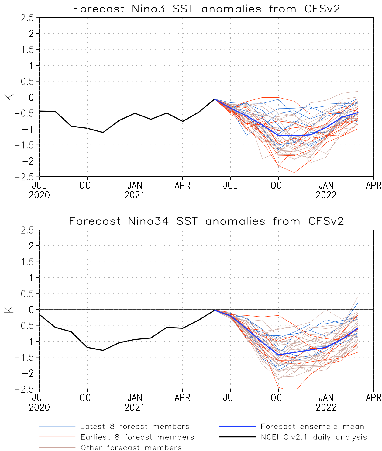
FIGURE F4. Predicted and observed sea surface temperature (SST) anomalies for the Nino 3 (top) and Nino 3.4 (bottom) regions from the NCEP Coupled Forecast System Model (CFSv2). The forecasts consist of 40 forecast members. The ensemble mean of all 40 forecast members is shown by the blue line, individual members are shown by thin lines, and the observation is indicated by the black line. The Nino-3 region spans the eastern equatorial Pacific between 5N-5S, 150W-90W. The Nino 3.4 region spans the east-central equatorial Pacific between 5N-5S, 170W-120W.
