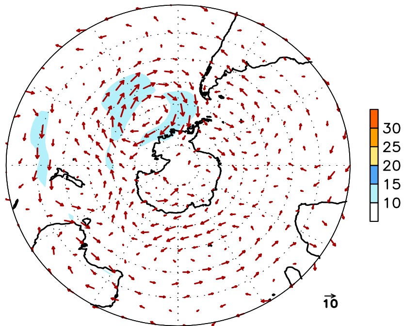
FIGURE E16. Southern Hemisphere mean (left) and anomalous (right) 300-hPa vector wind (CDAS/Reanalysis) for JUN 2021. Mean (anomaly) isotach contour interval is 10 (5) ms -1 . Values greater than 30 ms -1 (left) and 10 ms -1 (rights) are shaded. Anomalies are departures from the 1991-2020 base period monthly means.
