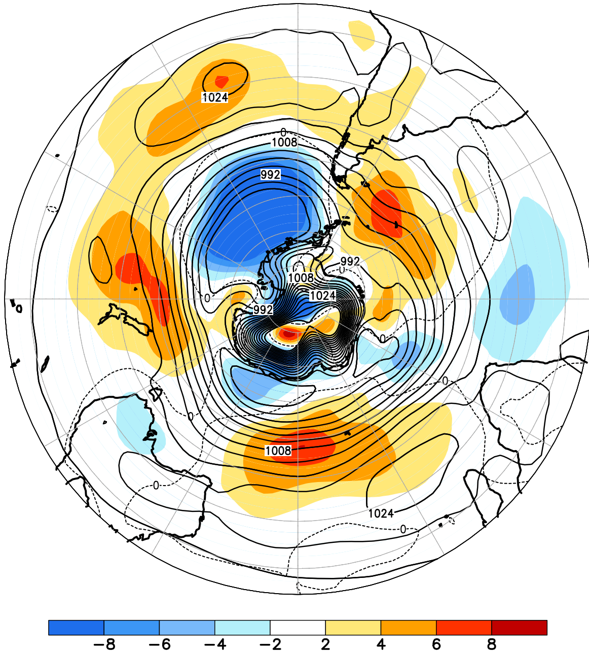
FIGURE E14. Southern Hemisphere mean and anomalous sea level pressure(CDAS/Reanalysis) for JUN 2021. Mean values are denoted by solid contours drawn at an interval of 4 hPa. Anomaly contour interval is 2 hPa with values less (greater) than -2 hPa (2 hPa) indicated by dark (light) shading. Anomalies are calculated as departures from the 1991-2020 base period monthly means.
