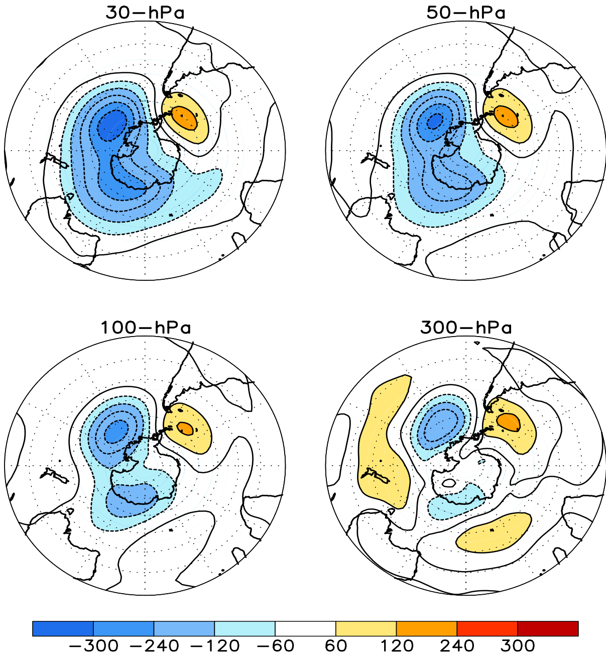
FIGURE S1. Stratospheric height anomalies (m) at selected levels for JUN 2021. Positive values are indicated by solid contours and dark shading. Negative values are indicated by dashed contours and light shading. Contour interval is 60 m. Anomalies are calculated from the 1991-2020 base period means. Winter Hemisphere is shown.
