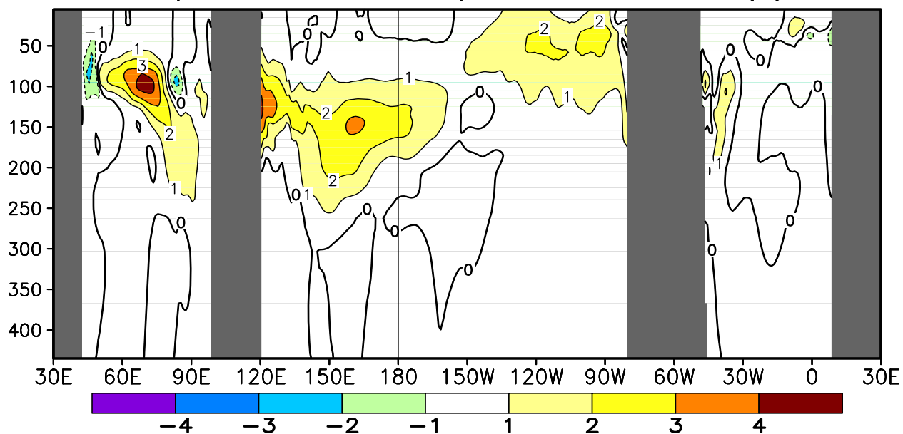
FIGURE T17. Equatorial depth–longitude section of ocean temperature (top) and ocean temperature anomalies (bottom) for JUN 2012. Contour interval is 1°C. Dashed contours in bottom panel indicate negative anomalies. Data are derived from the NCEP’s global ocean data assimilation system version 2 which assimilates oceanic observations into an oceanic GCM (Xue, Y. and Behringer, D.W., 2006: Operational global ocean data assimilation system at NCEP, to be submitted to BAMS). Anomalies are departures from the 1981–2010 base period means.
