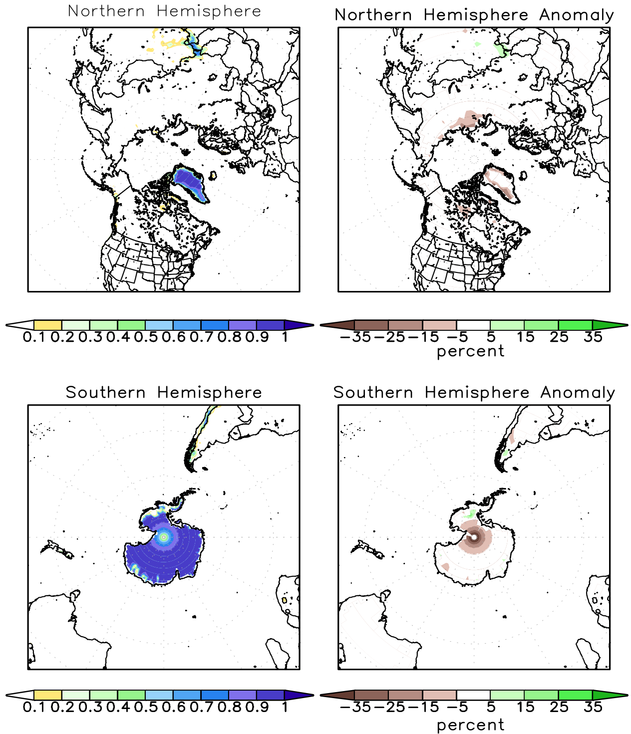
FIGURE A2.2. SSM/I derived snow cover frequency (%) (left) and snow cover anomaly (%) (right) for the month of JUN 2012 based on 1987 - 2010 base period for the Northern Hemisphere (top) and Southern Hemisphere (bottom). It is generated using the algorithm described by Ferraro et. al, 1996, Bull. Amer. Meteor. Soc., vol 77, 891-905.
