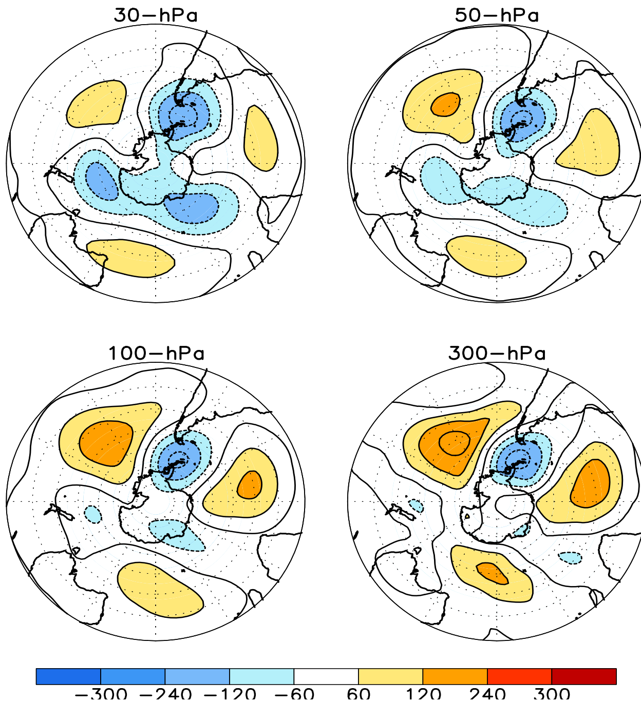
FIGURE S1. Stratospheric height anomalies (m) at selected levels for JUN 2012. Positive values are indicated by solid contours and dark shading. Negative values are indicated by dashed contours and light shading. Contour interval is 60 m. Anomalies are calculated from the 1981-2010 base period means. Winter Hemisphere is shown.
