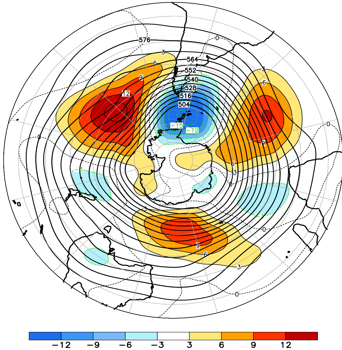
FIGURE E15. Southern Hemisphere mean and anomalous 500-hPa geopotential height (CDAS/Reanalysis) for JUN 2012. Mean heights are denoted by solid contours drawn at an interval of 6 dam. Anomaly contour interval is 3 dam with values less (greater) than -3 dam (3 dam) indicated by dark (light) shading. Anomalies are calculated as departures from the 1981-2010 base period monthly means.
