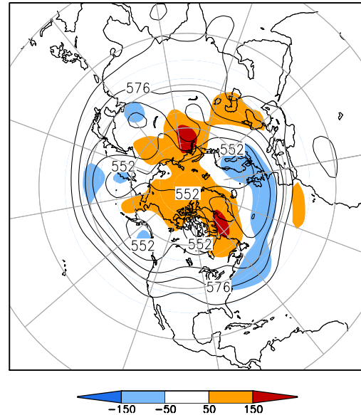
500-hPa Height (dm) & Anomalies (m) (Jun 1–15, 2012)
