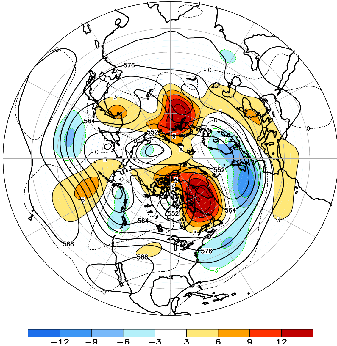
FIGURE E9. Northern Hemisphere mean and anomalous 500-hPa geopotential height (CDAS/Reanalysis) for JUN 2012. Mean heights are denoted by solid contours drawn at an interval of 6 dam. Anomaly contour interval is 3 dam with values less (greater) than -3 dam (3 dam) indicated by dark (light) shading. Anomalies are calculated as departures from the 1981-2010 base period monthly means.
