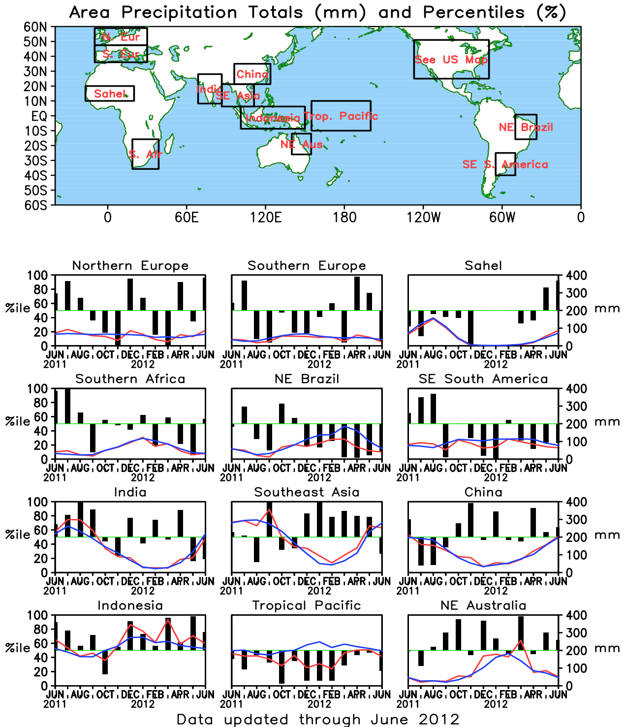
FIGURE E4. Areal estimates of monthly mean precipitation amounts (mm, solid lines) and precipitation percentiles (% , bars) for the most recent 13 months obtained from a merge of rain gauge observations and satellite-derived precipitation estimates (Janowiak and Xie 1999, J. Climate , 12, 3335–3342). The monthly precipitation climatology (mm, dashed lines) is from the 1981–2010 base period monthly means. Monthly percentiles are not shown if the monthly mean is less than 5 mm.
