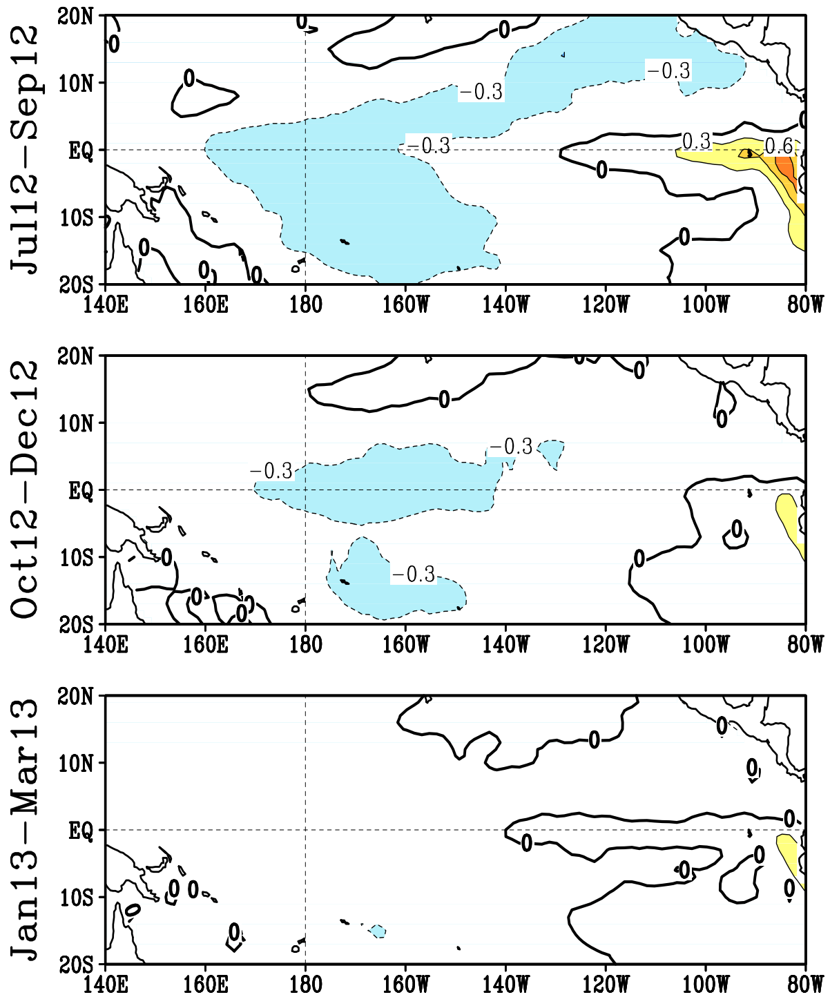
FIGURE F5. Predicted 3-month average sea surface temperature anomalies from the NCEP/CPC Markov model (Xue et al. 2000, J. Climate , 13 , 849-871). The forecast is initiated in JUN 2012 . Contour interval is 0.3C and negative anomalies are indicated by dashed contours. Anomalies are calculated relative to the 1971-2000 climatology.
