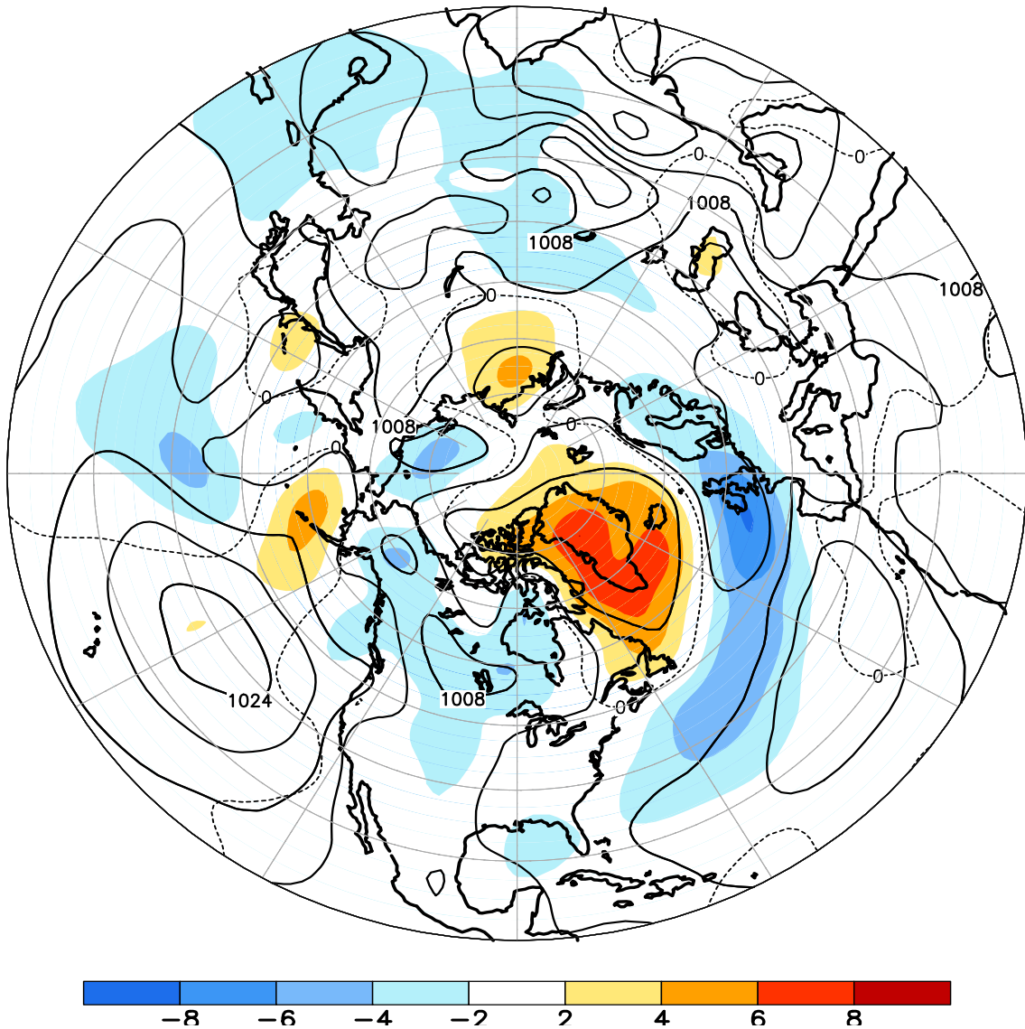
FIGURE E8. Northern Hemisphere mean and anomalous sea level pressure (CDAS/Reanalysis) for JUN 2012. Mean values are denoted by solid contours drawn at an interval of 4 hPa. Anomaly contour interval is 2 hPa with values less (greater) than -2 hPa (2 hPa) indicated by dark (light) shading. Anomalies are calculated as departures from the 1981-2010 base period monthly means.
