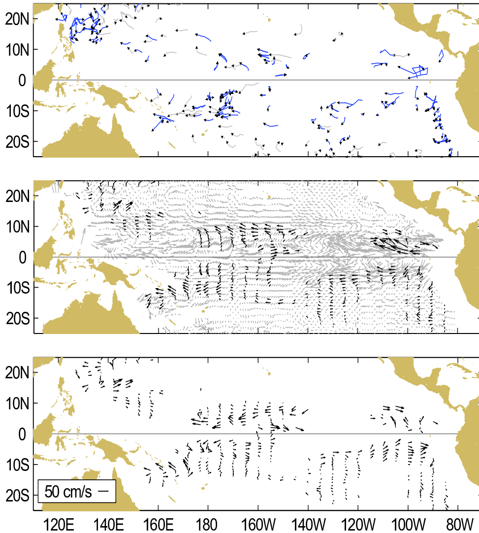
Figure A1.1 Top: Movements of drifting buoys in the tropical Pacific Ocean during June 2012. The linear segments of each trajectory represent a one week displacement. Trajectories of buoys which have lost their subsurface drogues are gray; those with drogues are black. Middle: Monthly mean currents calculated from all buoys 1993-2002 (gray), and currents measured by the drogued buoys this month (black) smoothed by an optimal filter. Bottom: Anomalies from the climatological monthly mean currents for this month.
