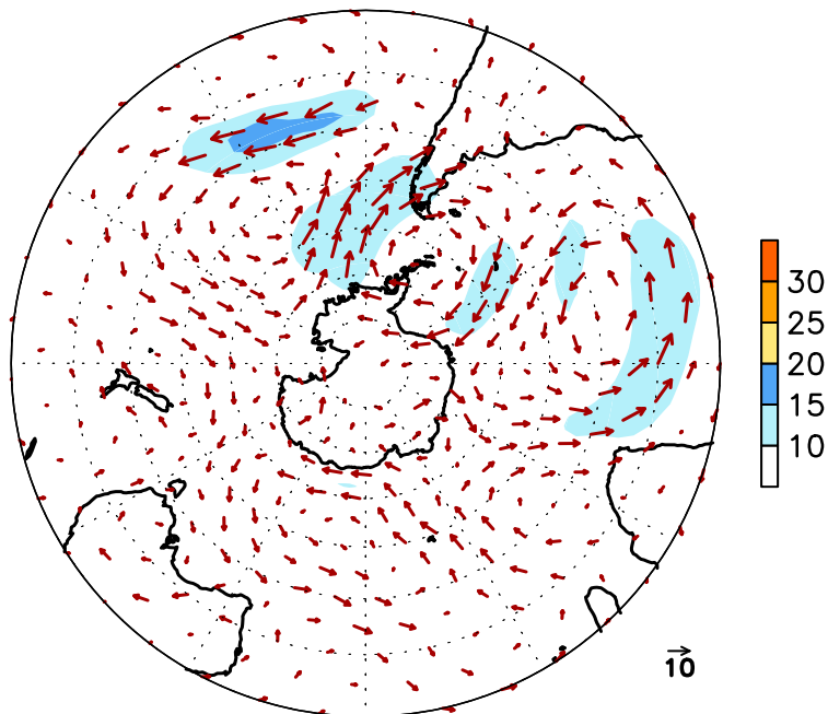
FIGURE E16. Southern Hemisphere mean (left) and anomalous (right) 300-hPa vector wind (CDAS/Reanalysis) for JUN 2012. Mean (anomaly) isotach contour interval is 10 (5) ms -1 . Values greater than 30 ms -1 (left) and 10 ms -1 (rights) are shaded. Anomalies are departures from the 1981-2010 base period monthly means.
