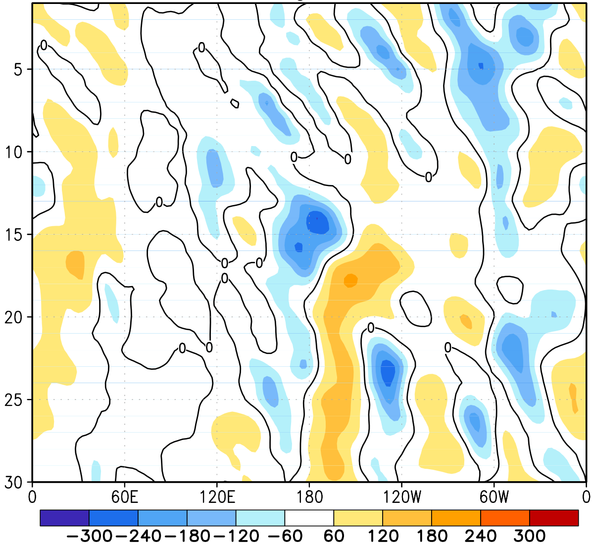
FIGURE E12. Northern Hemisphere: Daily 500-hPa height anomalies for JUN 2012 averaged over the 5° latitude band centered on 40°N. Positive values are indicated by solid contours and dark shading. Negative values are indicated by dashed contours and light shading. Contour interval is 60 m. Anomalies are departures from the 1981-2010 base period daily means.
