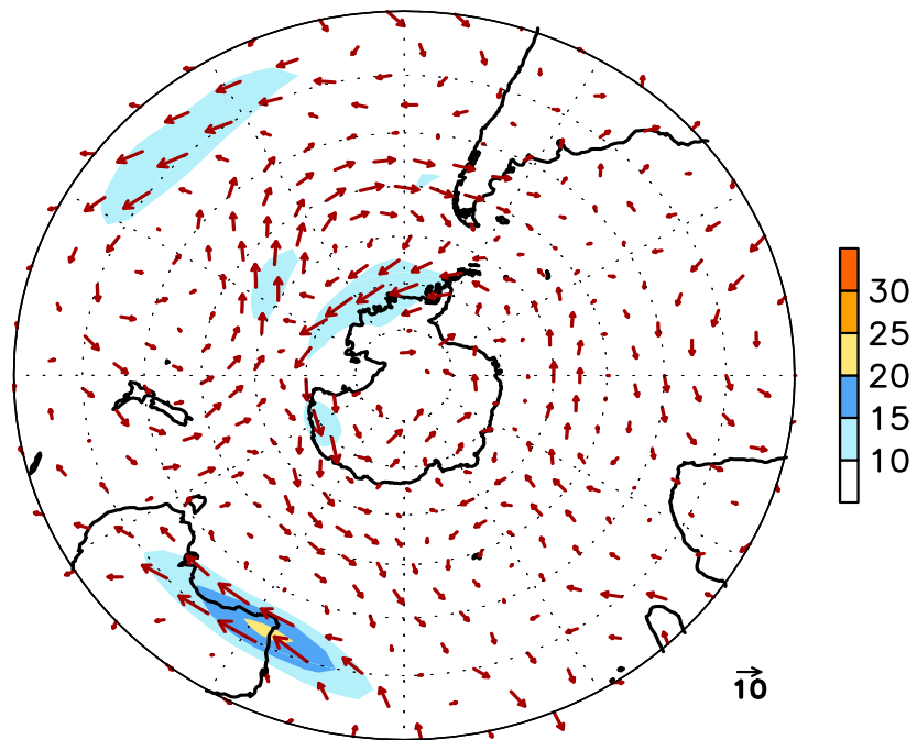
FIGURE E16. Southern Hemisphere mean (left) and anomalous (right) 300-hPa vector wind (CDAS/Reanalysis) for JUL 2021. Mean (anomaly) isotach contour interval is 10 (5) ms -1 . Values greater than 30 ms -1 (left) and 10 ms -1 (rights) are shaded. Anomalies are departures from the 1991-2020 base period monthly means.
