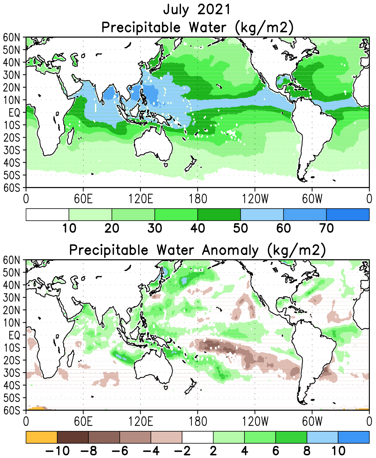
FIGURE T28. Mean (top) and anomalous (bottom) vertically integrated water vapor or precipitable water (kg m -2 ) based on the Special Sensor Microwave/Imager (SSM/I) (Ferraro et. al, 1996: Bull. Amer. Meteor. Soc. , 77, 891-905). Anomalies are calculated from the 1987-2010 base period means.
