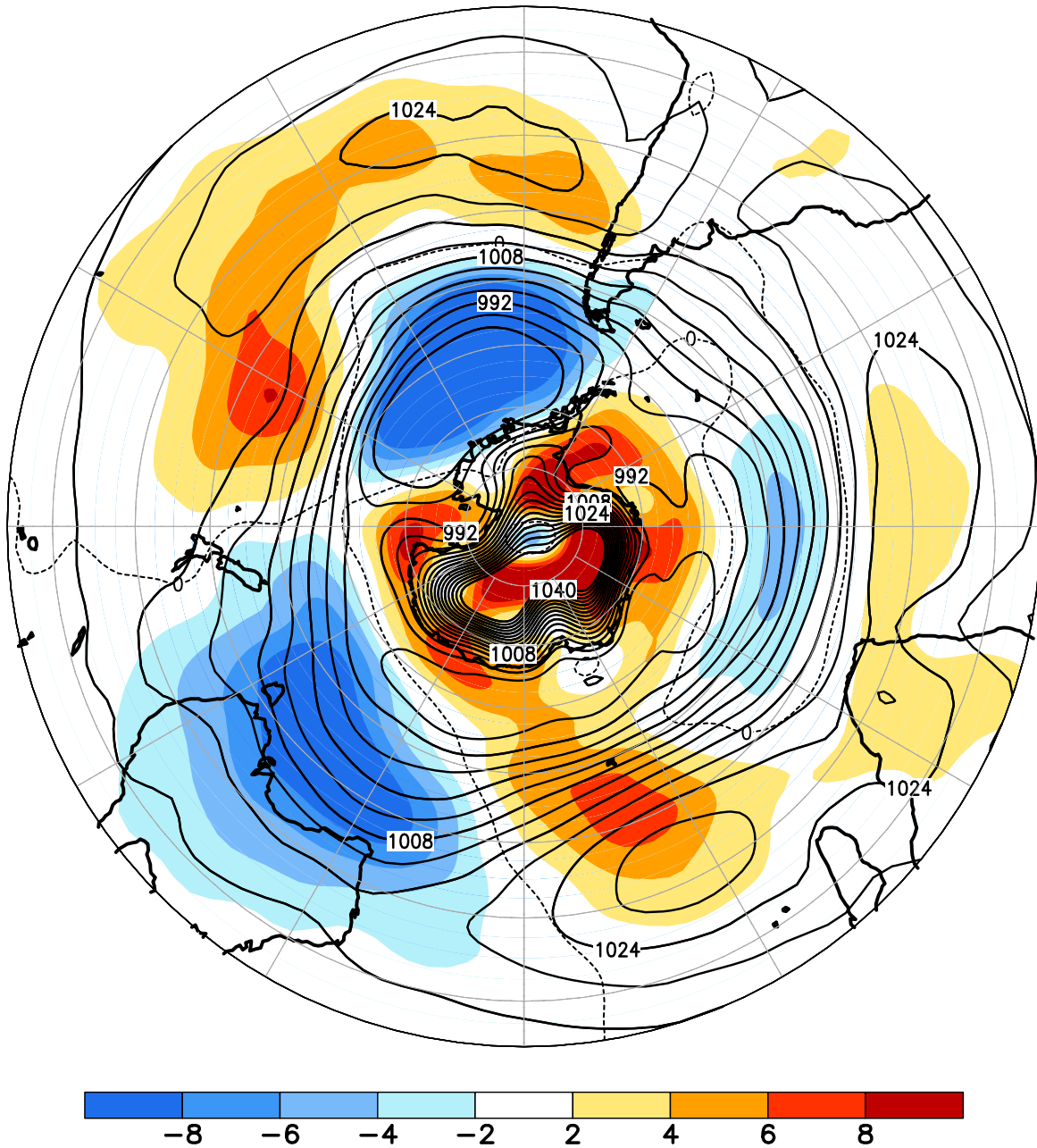
FIGURE E14. Southern Hemisphere mean and anomalous sea level pressure(CDAS/Reanalysis) for JUL 2021. Mean values are denoted by solid contours drawn at an interval of 4 hPa. Anomaly contour interval is 2 hPa with values less (greater) than -2 hPa (2 hPa) indicated by dark (light) shading. Anomalies are calculated as departures from the 1991-2020 base period monthly means.
