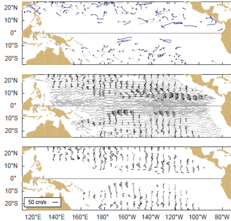
Figure A1.1 Top: Movements of drifting buoys in the tropical Pacific Ocean during July 2021. The linear segments of each trajectory represent a one week displacement. Trajectories of buoys which have lost their subsurface drogues are gray; those with drogues are black.
