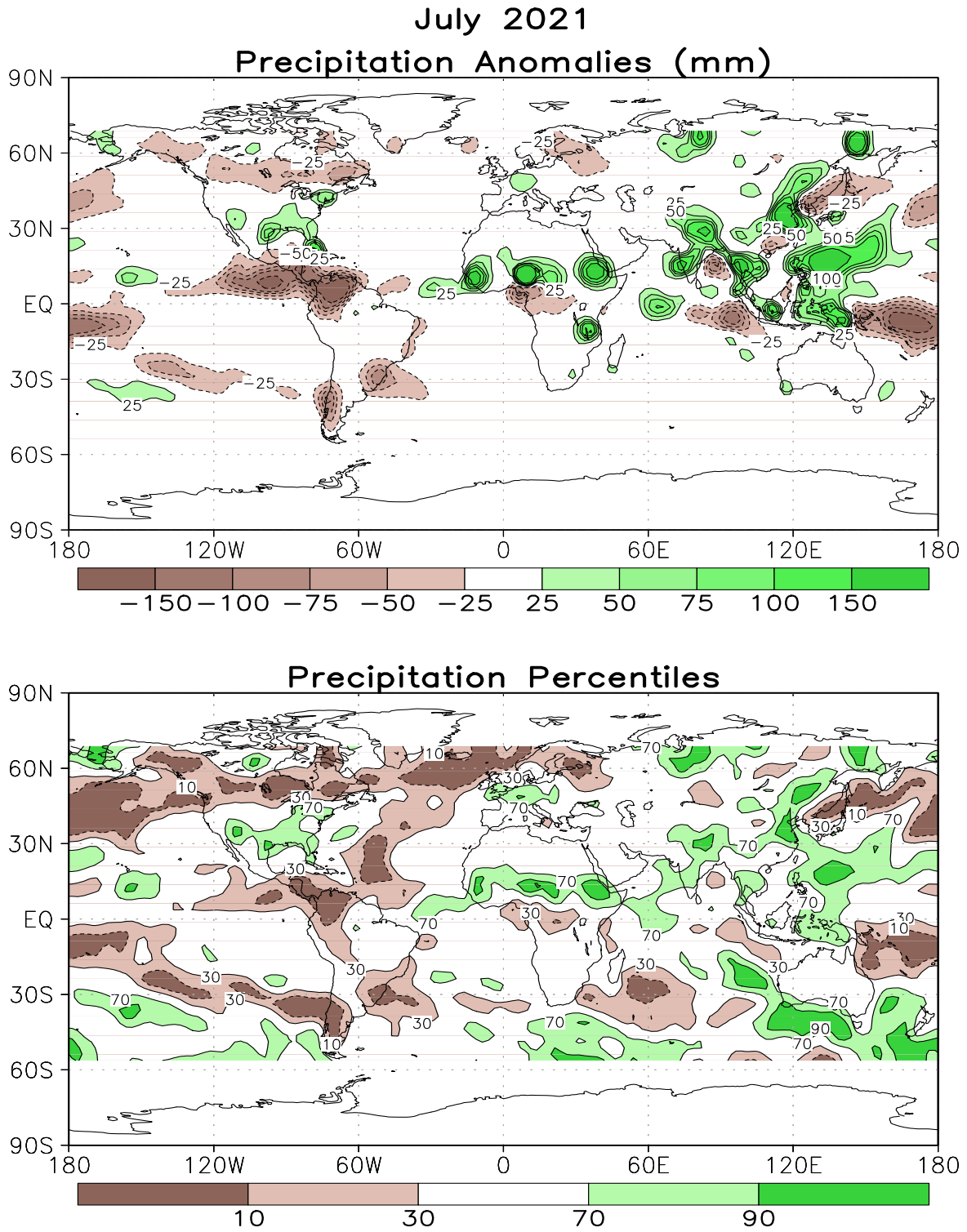
FIGURE E3. Anomalous precipitation (mm, top) and precipitation percentiles based on a Gamma distribution fit to the 1981-2010 base period data (bottom) for JUL 2021. Data are obtained from a merge of raingauge observations and satellite-derived precipitation estimates (Janowiak and Xie 1999, J. Climate , 12 , 3335–3342). Contours are drawn at 200, 100, 50, 25, -25, -50, -100, and -200 mm in top panel. Percentiles are not plotted in regions where mean monthly precipitation is <5mm/month.
