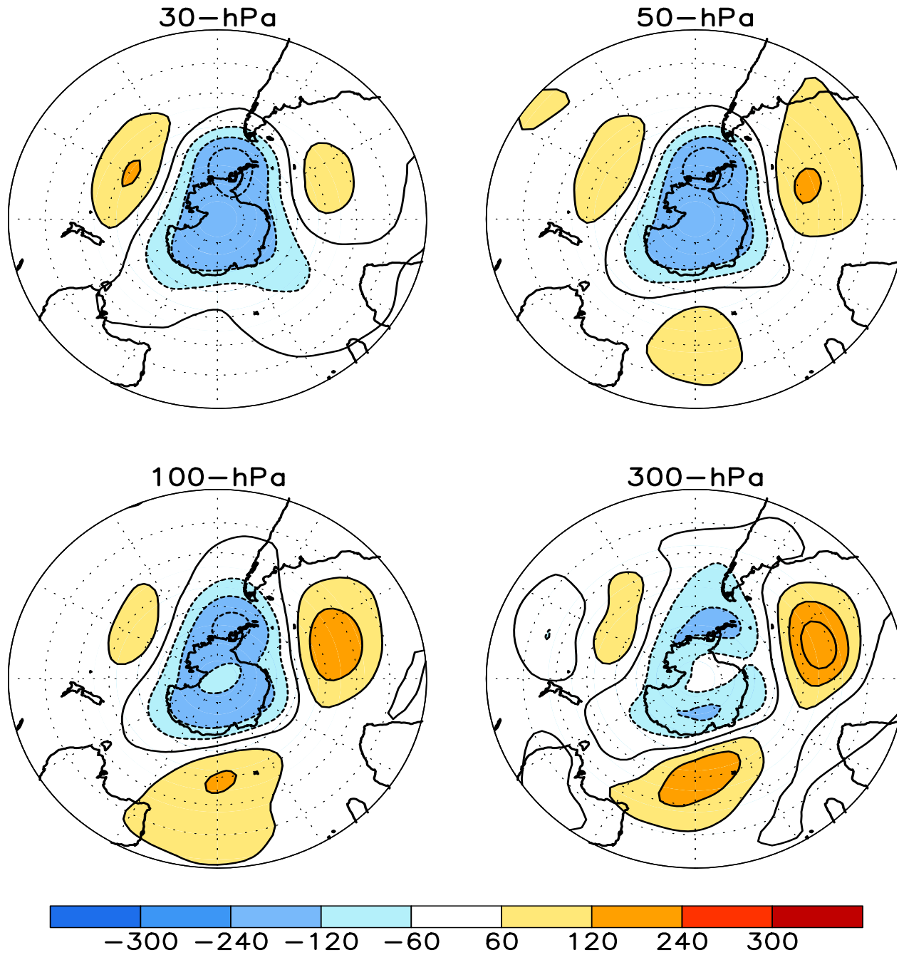
FIGURE S1. Stratospheric height anomalies (m) at selected levels for JUL 2015. Positive values are indicated by solid contours and dark shading. Negative values are indicated by dashed contours and light shading. Contour interval is 60 m. Anomalies are calculated from the 1981-2010 base period means. Winter Hemisphere is shown.
