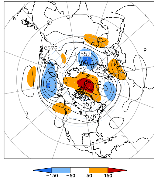
500-hPa Height (dm) & Anomalies (m) (Jul 1–15, 2015)
