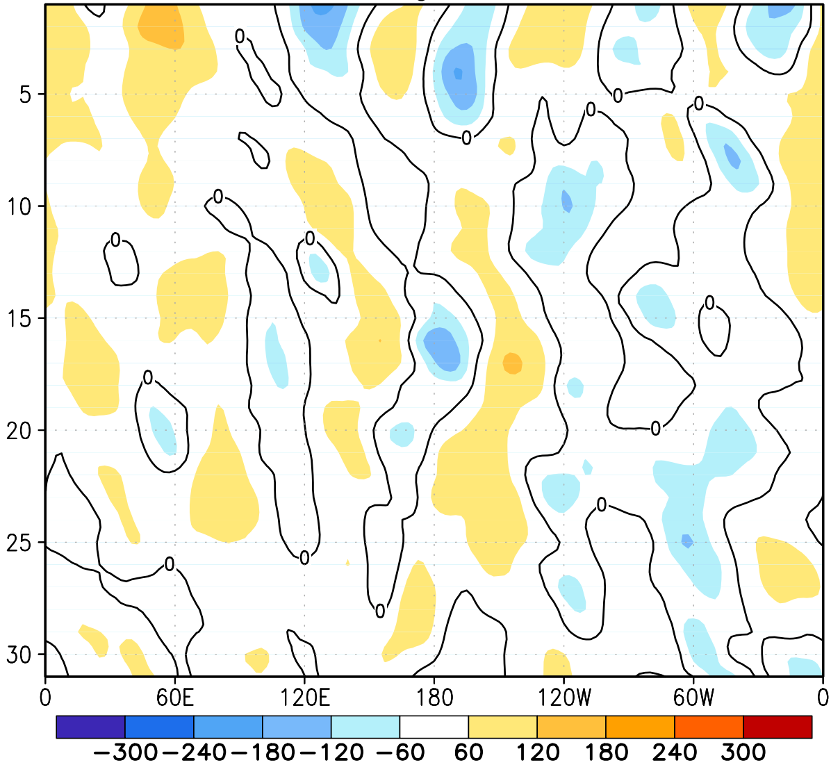
FIGURE E12. Northern Hemisphere: Daily 500-hPa height anomalies for JUL 2015 averaged over the 5° latitude band centered on 40°N. Positive values are indicated by solid contours and dark shading. Negative values are indicated by dashed contours and light shading. Contour interval is 60 m. Anomalies are departures from the 1981-2010 base period daily means.
