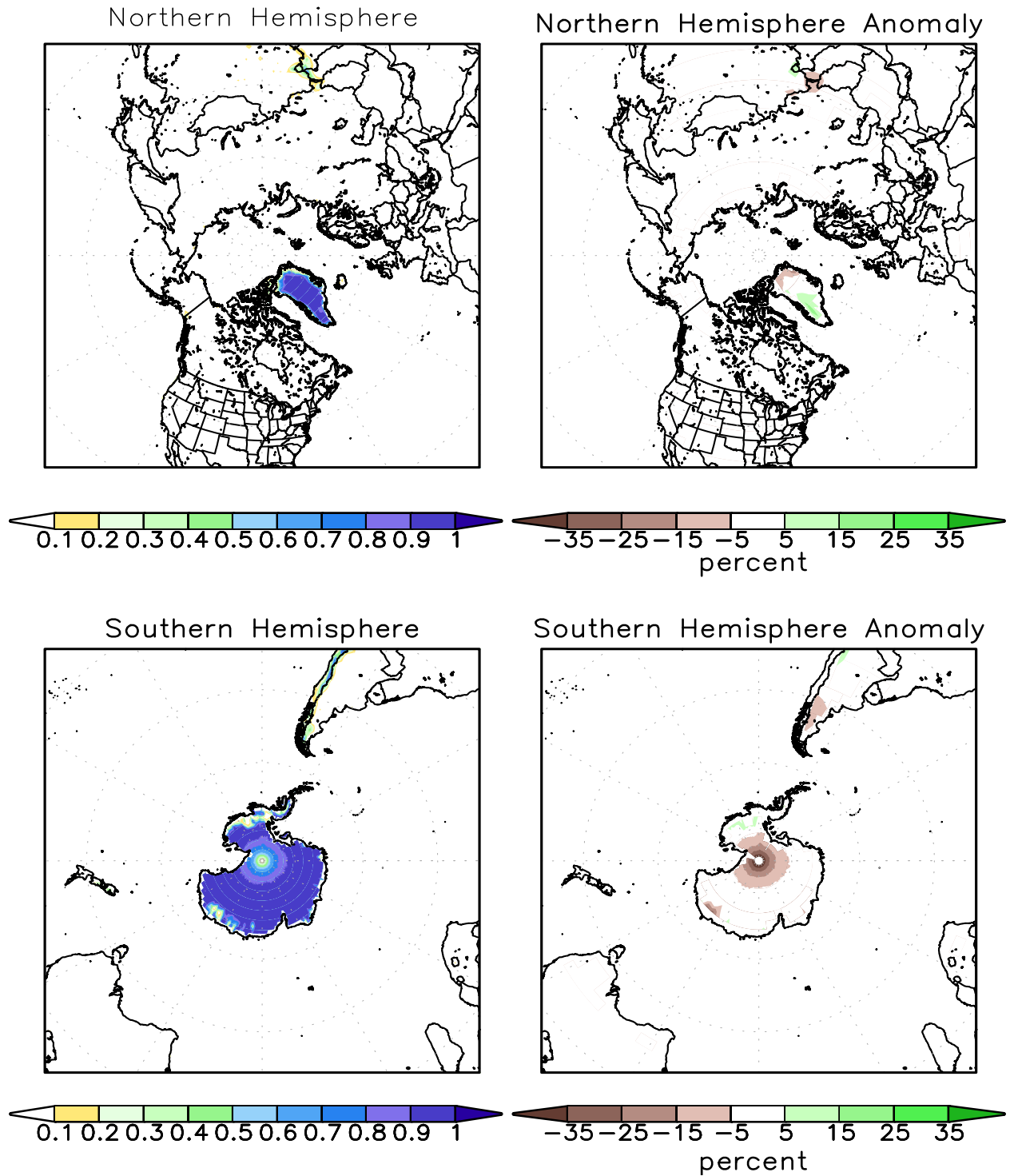
FIGURE A2.2. SSM/I derived snow cover frequency (%) (left) and snow cover anomaly (%) (right) for the month of JUL 2015 based on 1987 - 2010 base period for the Northern Hemisphere (top) and Southern Hemisphere (bottom). It is generated using the algorithm described by Ferraro et. al, 1996, Bull. Amer. Meteor. Soc., vol 77, 891-905.
