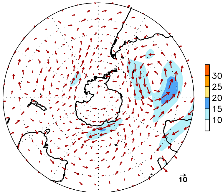
FIGURE E16. Southern Hemisphere mean (left) and anomalous (right) 300-hPa vector wind (CDAS/Reanalysis) for JUL 2015. Mean (anomaly) isotach contour interval is 10 (5) \text{ms}^{-1} . Values greater than 30 \text{ms}^{-1} (left) and 10 \text{ms}^{-1} (rights) are shaded. Anomalies are departures from the 1981-2010 base period monthly means.
