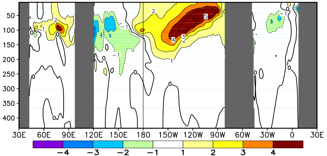
FIGURE T17. Equatorial depth–longitude section of ocean temperature (top) and ocean temperature anomalies (bottom) for JUL 2015. Contour interval is 1°C. Dashed contours in bottom panel indicate negative anomalies. Data are derived from the NCEP’s global ocean data assimilation system version 2 which assimilates oceanic observations into an oceanic GCM (Xue, Y. and Behringer, D.W., 2006: Operational global ocean data assimilation system at NCEP, to be submitted to BAMS). Anomalies are departures from the 1981–2010 base period means.
