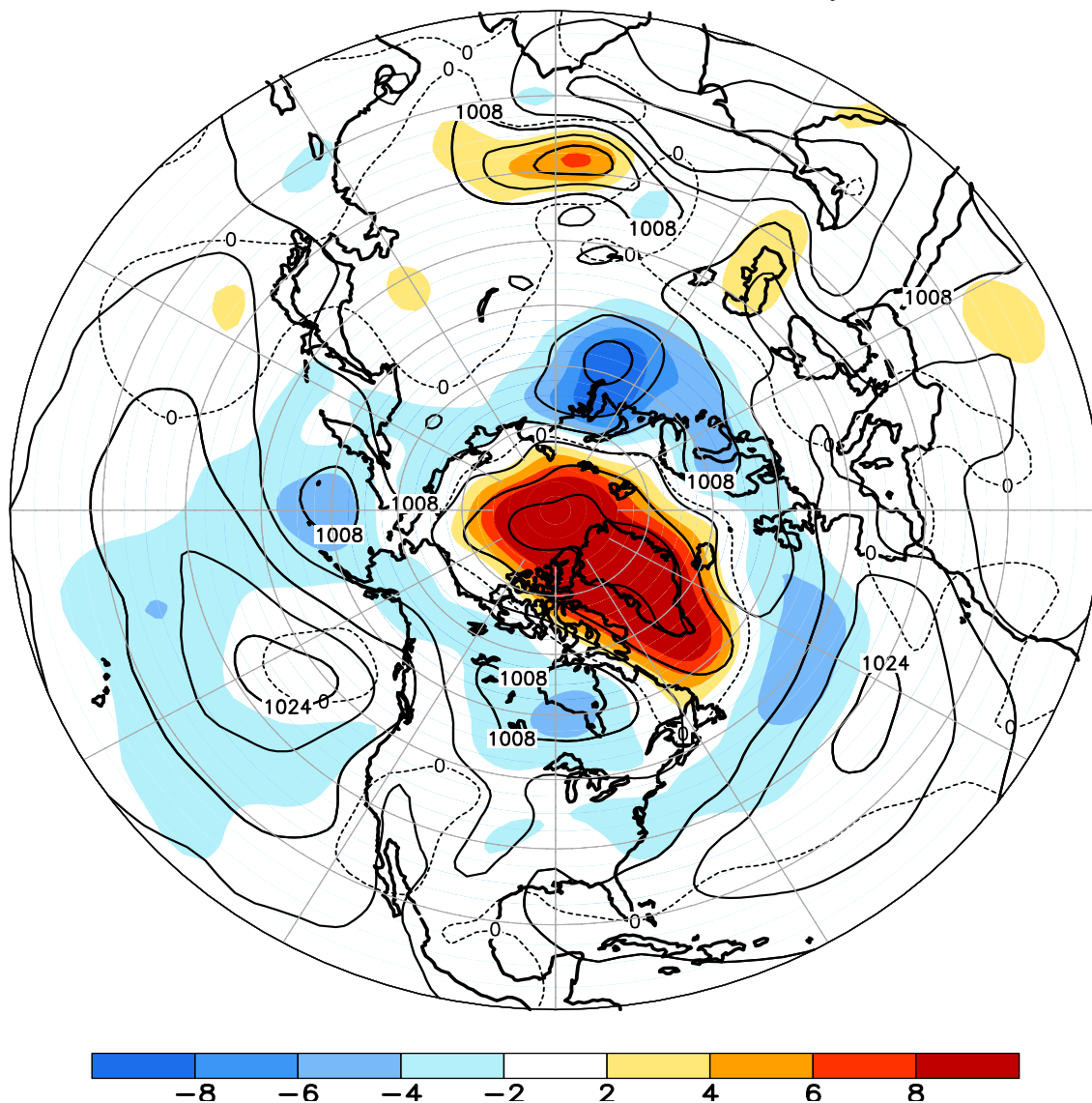
FIGURE E8. Northern Hemisphere mean and anomalous sea level pressure (CDAS/Reanalysis) for JUL 2015. Mean values are denoted by solid contours drawn at an interval of 4 hPa. Anomaly contour interval is 2 hPa with values less (greater) than -2 hPa (2 hPa) indicated by dark (light) shading. Anomalies are calculated as departures from the 1981-2010 base period monthly means.
