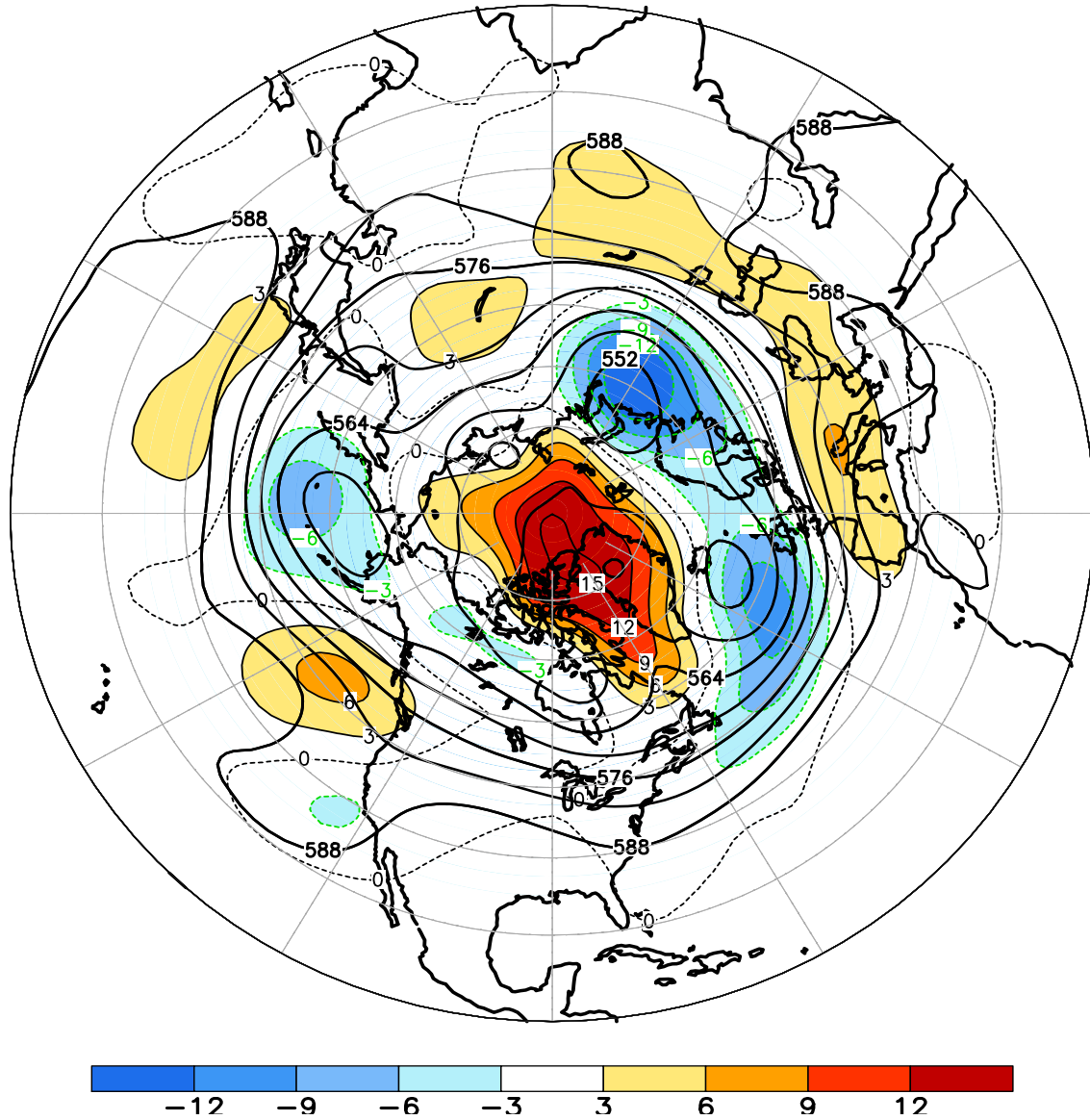
FIGURE E9. Northern Hemisphere mean and anomalous 500-hPa geopotential height (CDAS/Reanalysis) for JUL 2015. Mean heights are denoted by solid contours drawn at an interval of 6 dam. Anomaly contour interval is 3 dam with values less (greater) than -3 dam (3 dam) indicated by dark (light) shading. Anomalies are calculated as departures from the 1981-2010 base period monthly means.
