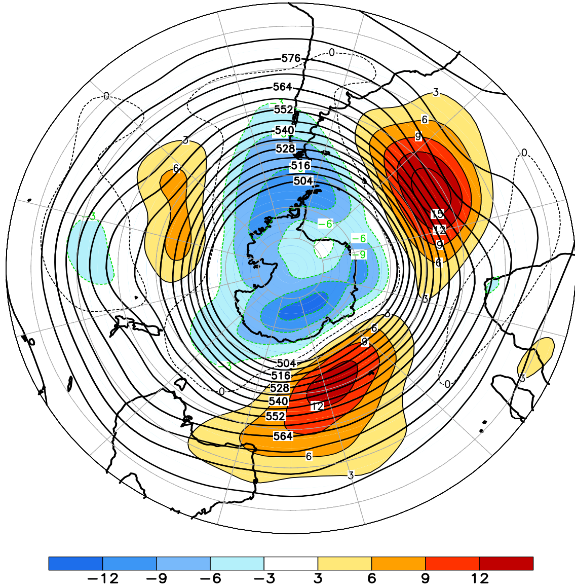
FIGURE E15. Southern Hemisphere mean and anomalous 500-hPa geopotential height (CDAS/Reanalysis) for JUL 2015. Mean heights are denoted by solid contours drawn at an interval of 6 dam. Anomaly contour interval is 3 dam with values less (greater) than -3 dam (3 dam) indicated by dark (light) shading. Anomalies are calculated as departures from the 1981-2010 base period monthly means.
